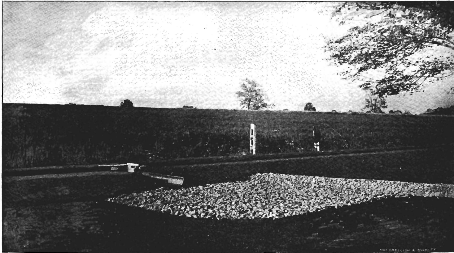
FIGURE 2—Branch Opening with Gates for Directing the Flow, and with a Broken Stone Apron to Check Velocity.
