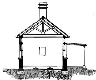
SECTION ON LINE A.A.
