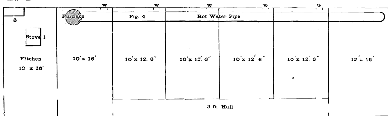
CROSS SECTION OF GROUND FLOOR OF ISOLATION HOSPITAL
