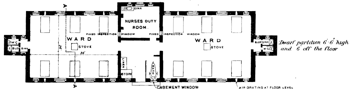
PLAN OF A WARD PAVILION FOR 12 BEDS
