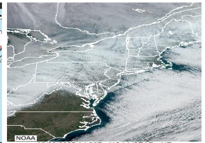
Satellite
