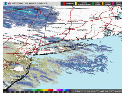
Local Radar
