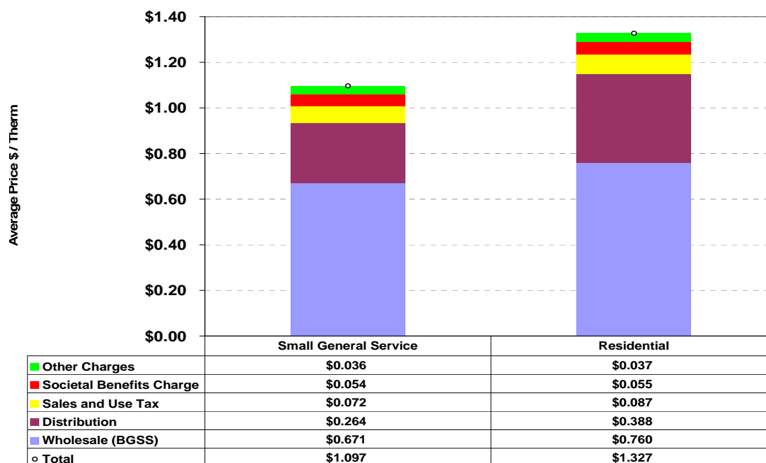
Figure 33. Average LDC 2010 Rate Components
