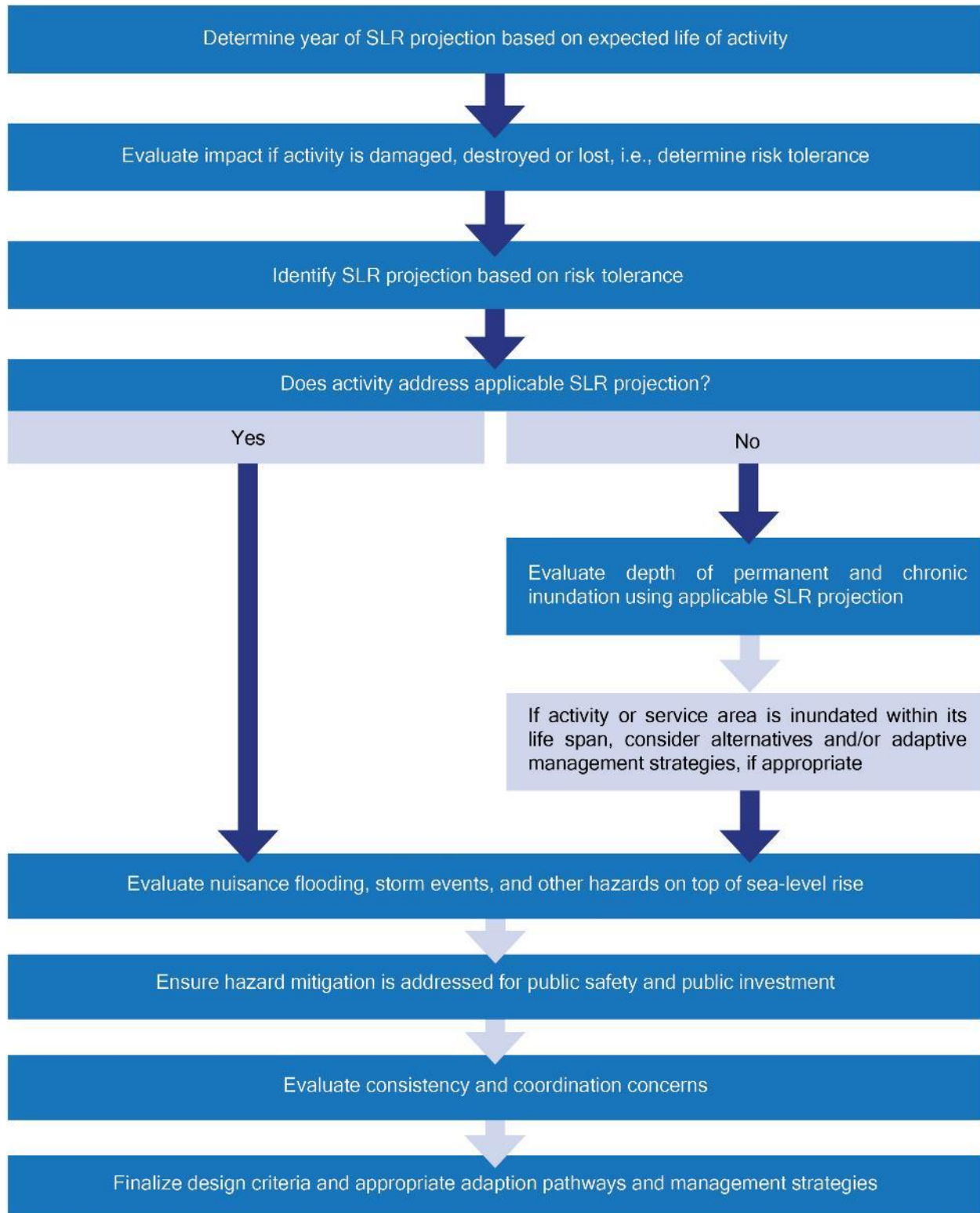
Figure 2. Diagram of method to determine appropriate SLR projection for an activity
