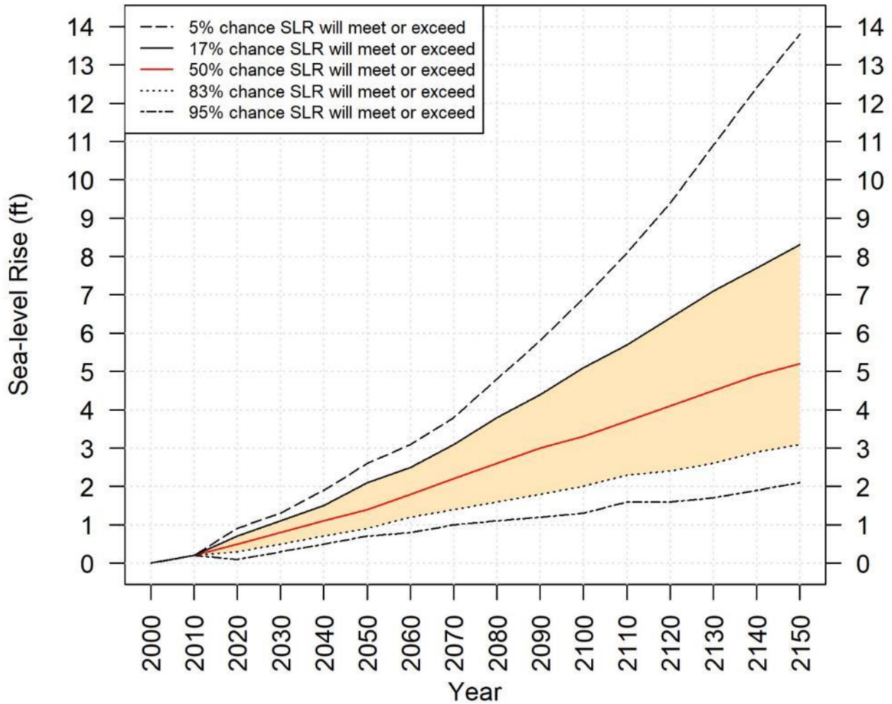
Figure 1. Diagram of sea-level rise projections curve under moderate emissions scenario SLR projections for New Jersey from 2000 to 2150 under the moderate emissions scenario. The likely range (colored area) represents the range of projections between which there is a 66% chance that sea-level rise will occur. This figure is adopted from values presented in Table 1. (Kopp et al. 2019a)
