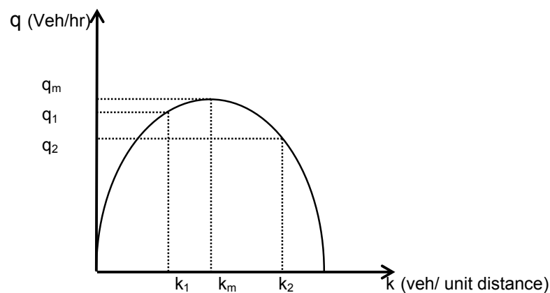
Figure A-1. Flow-density relationship
