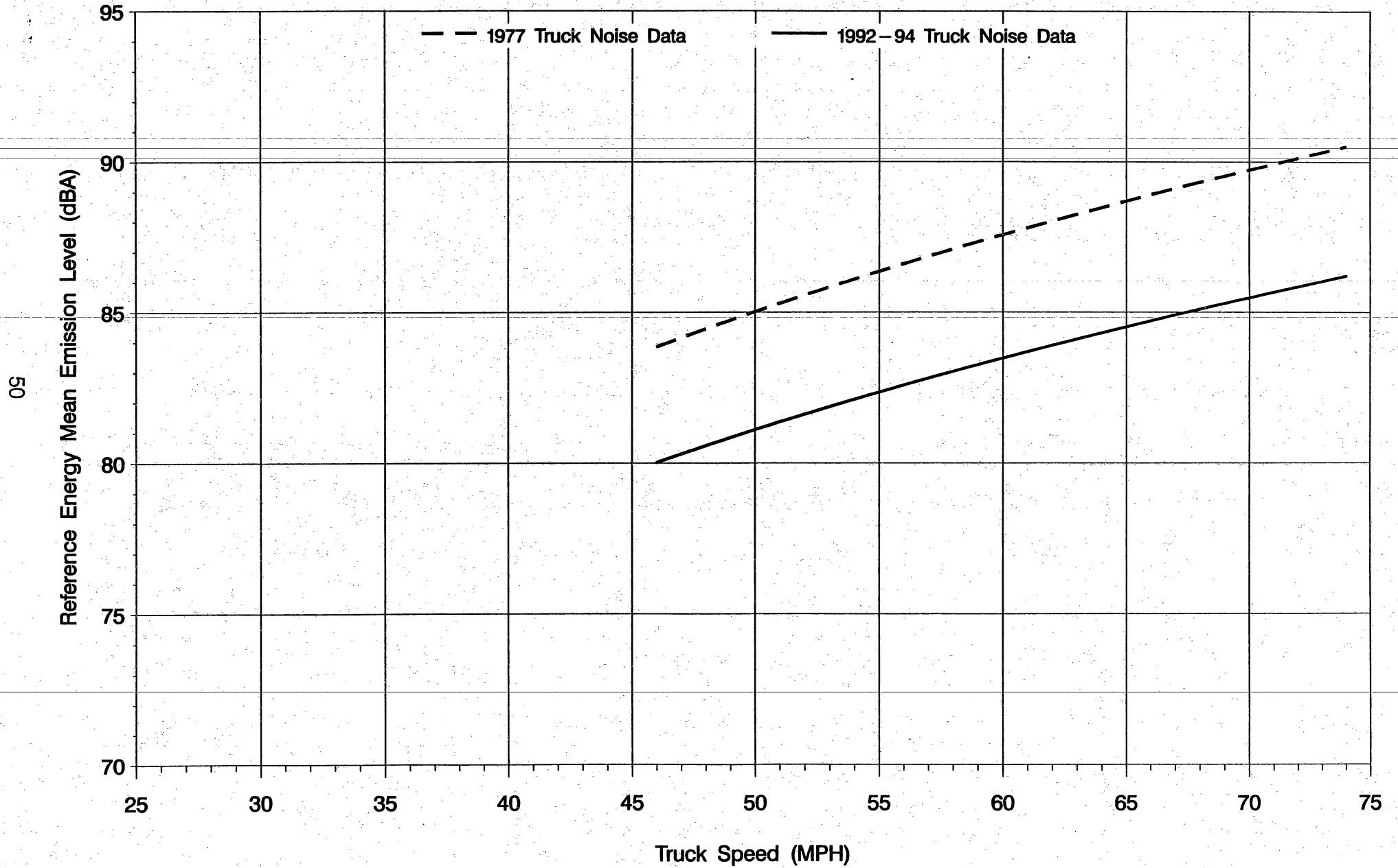
Figure 13: REMEL vs. Truck Speed ROADWAY TYPE 3 (Controlled Access, Downgrade) – HEAVY TRUCKS
