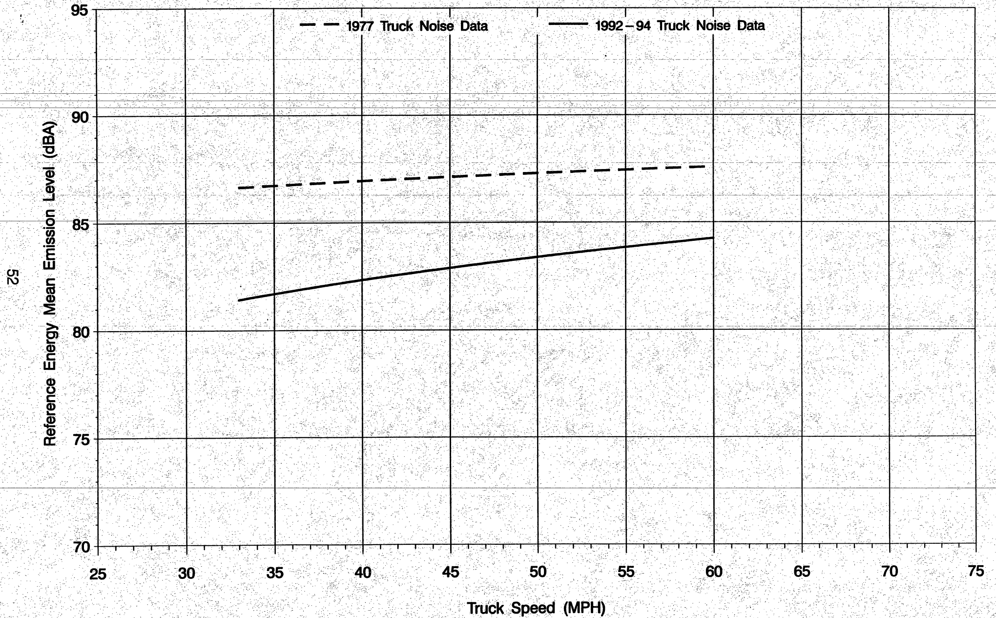
Figure 15: REMEL vs. Truck Speed ROADWAY TYPE 5 (Non-Controlled Access, Upgrade) – HEAVY TRUCKS
