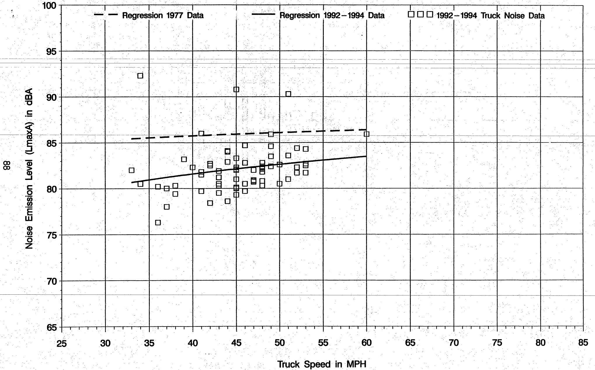
Figure B-11: Noise Emission Level (LmaxA) vs. Truck Speed ROADWAY TYPE 5 (Non-Controlled Access, Upgrade) - HEAVY TRUCKS
