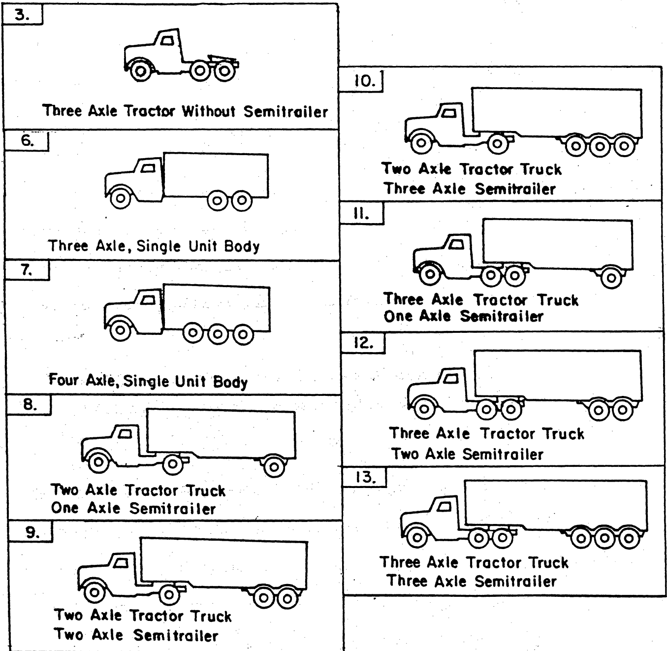
Figure 3. TRUCK CLASS 2 HEAVY TRUCKS
