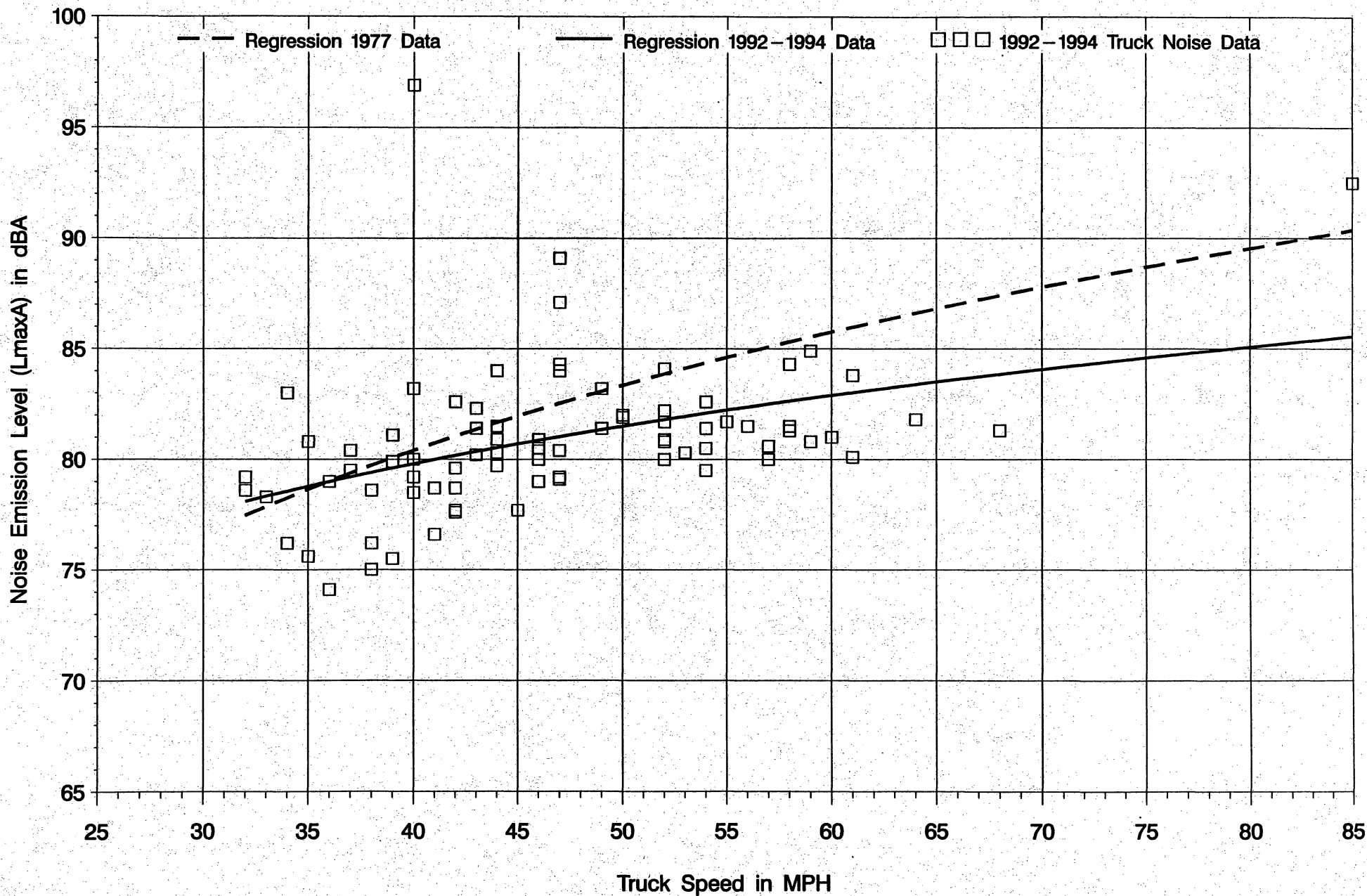
Figure B-12: Noise Emission Level (LmaxA) vs. Truck Speed ROADWAY TYPE 6 (Non-Controlled Access, Downgrade) – HEAVY TRUCKS
