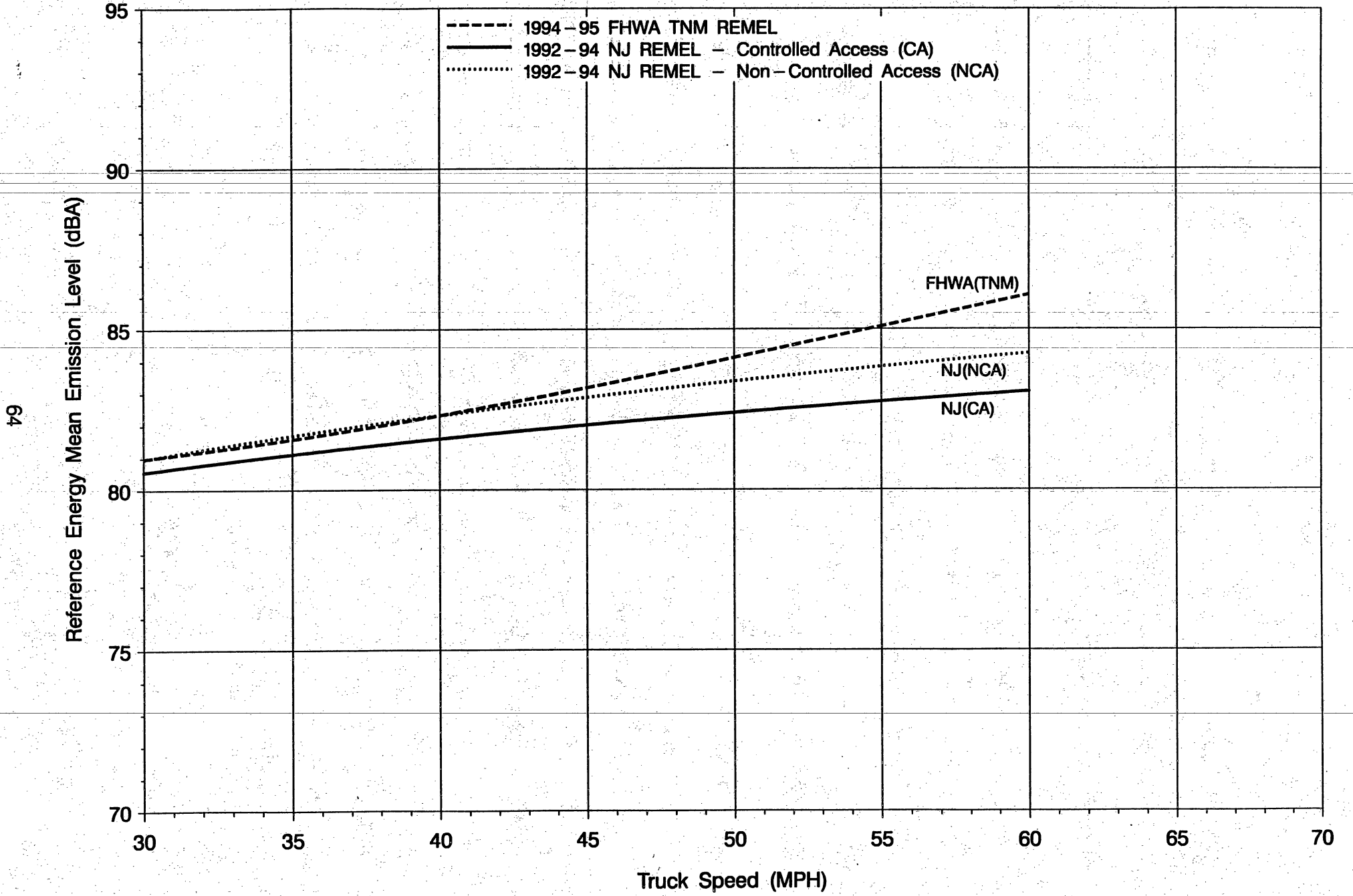
Figure 20: NJ REMELS VS. FHWA TNM REMELS – HEAVY TRUCKS, UPGRADES
