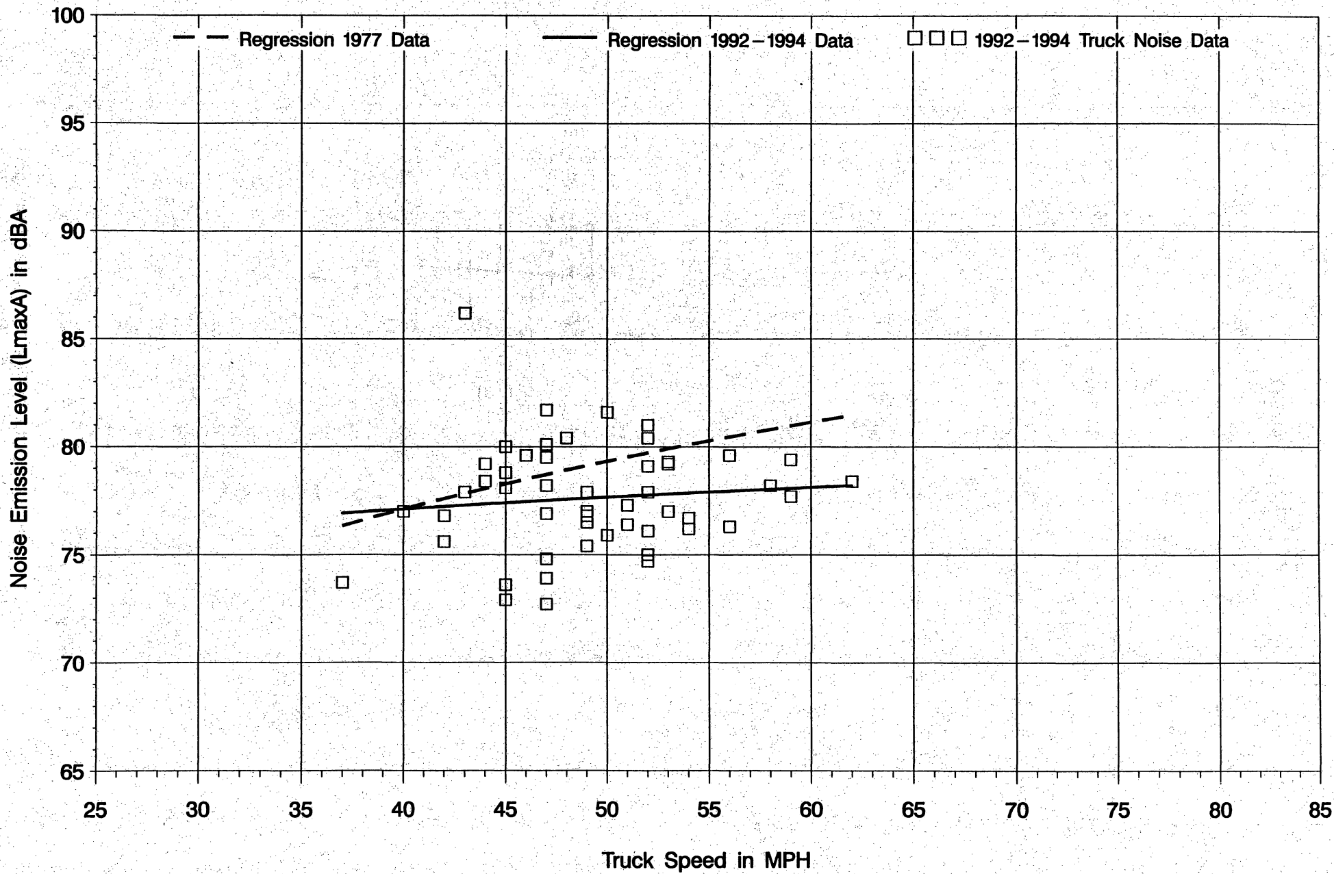
Figure B-4: Noise Emission Level (LmaxA) vs. Truck Speed ROADWAY TYPE 4 (Non-Controlled Access, Level) - MEDIUM TRUCKS & BUSES
