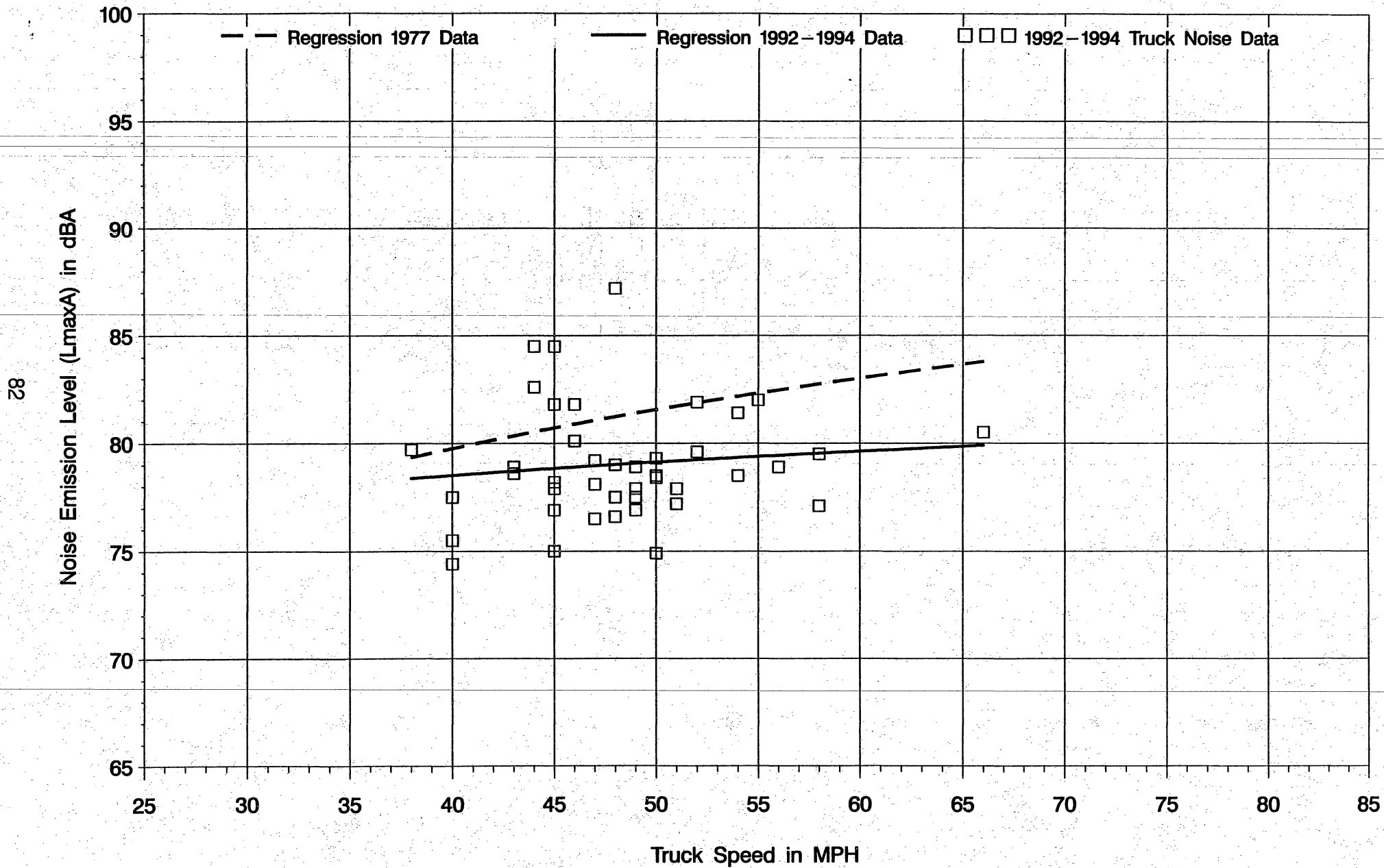
Figure B-5: Noise Emission Level (LmaxA) vs. Truck Speed ROADWAY TYPE 5 (Non-Controlled Access, Upgrade) – MEDIUM TRUCKS & BUSES
