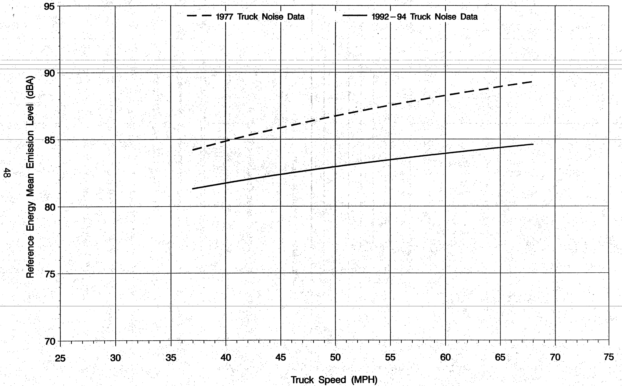
Figure 11: REMEL vs. Truck Speed ROADWAY TYPE 1 (Controlled Access, Level) – HEAVY TRUCKS
