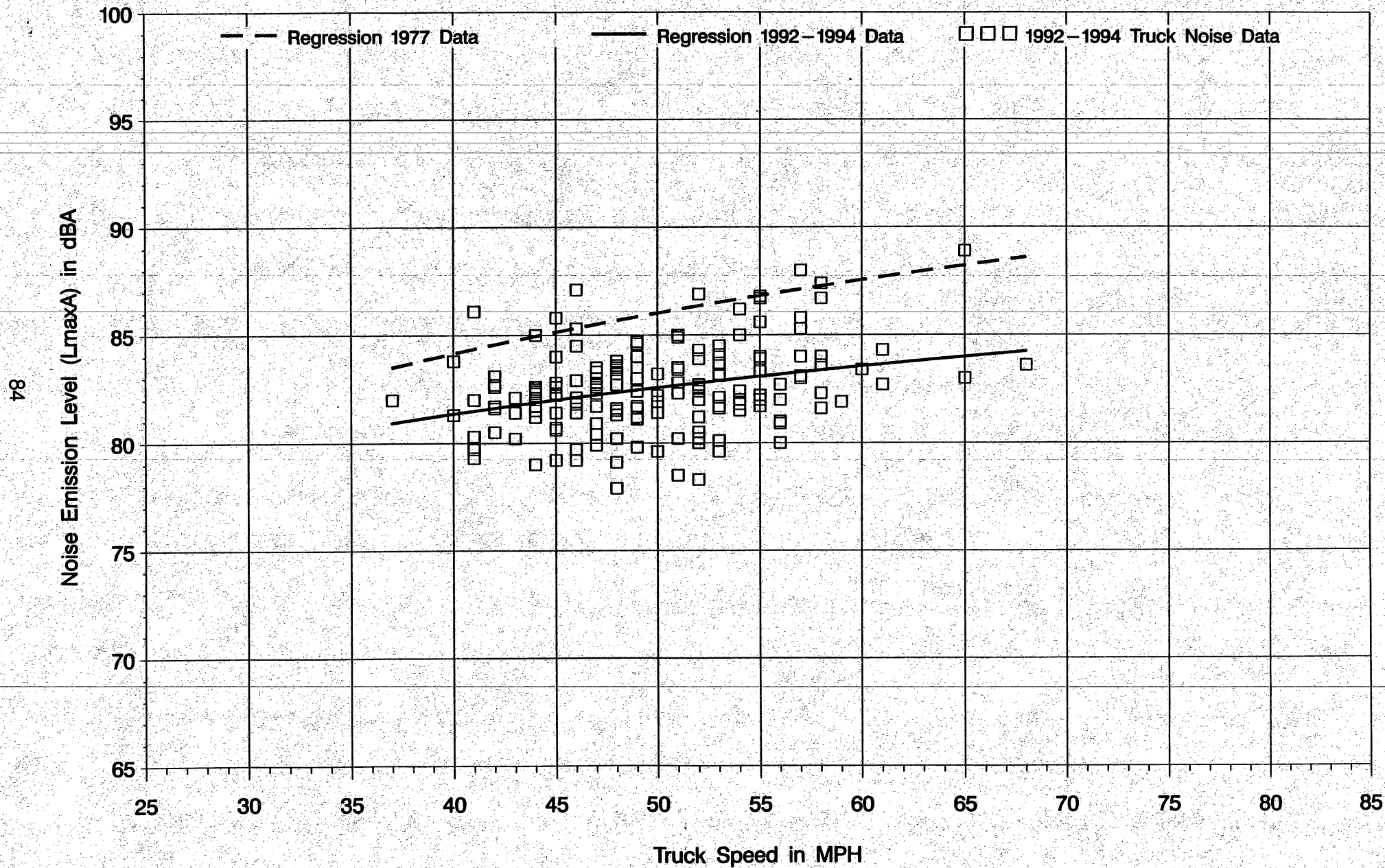
Figure B-7: Noise Emission Level (LmaxA) vs. Truck Speed ROADWAY TYPE 1 (Controlled Access, Level) – HEAVY TRUCKS
