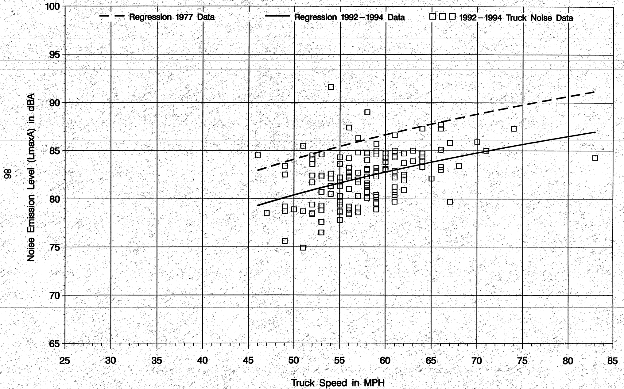
Figure B-9: Noise Emission Level (LmaxA) vs. Truck Speed ROADWAY TYPE 3 (Controlled Access, Downgrade) – HEAVY TRUCKS
