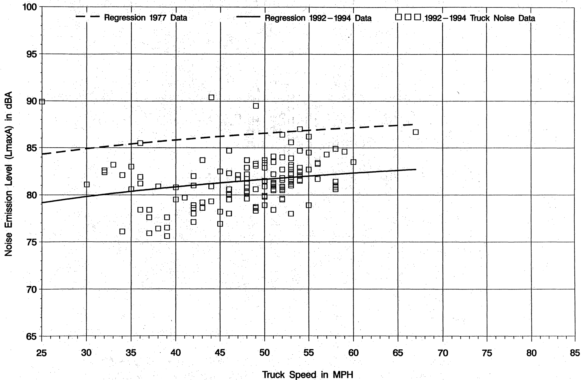
Figure B-8: Noise Emission Level (LmaxA) vs. Truck Speed ROADWAY TYPE 2 (Controlled Access, Upgrade) – HEAVY TRUCKS
