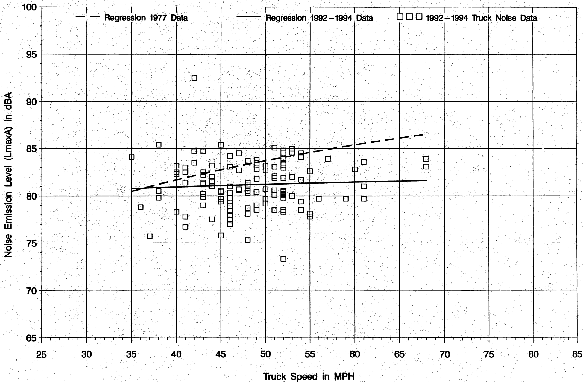
Figure B-10: Noise Emission Level (LmaxA) vs. Truck Speed ROADWAY TYPE 4 (Non-Controlled Access, Level) - HEAVY TRUCKS
