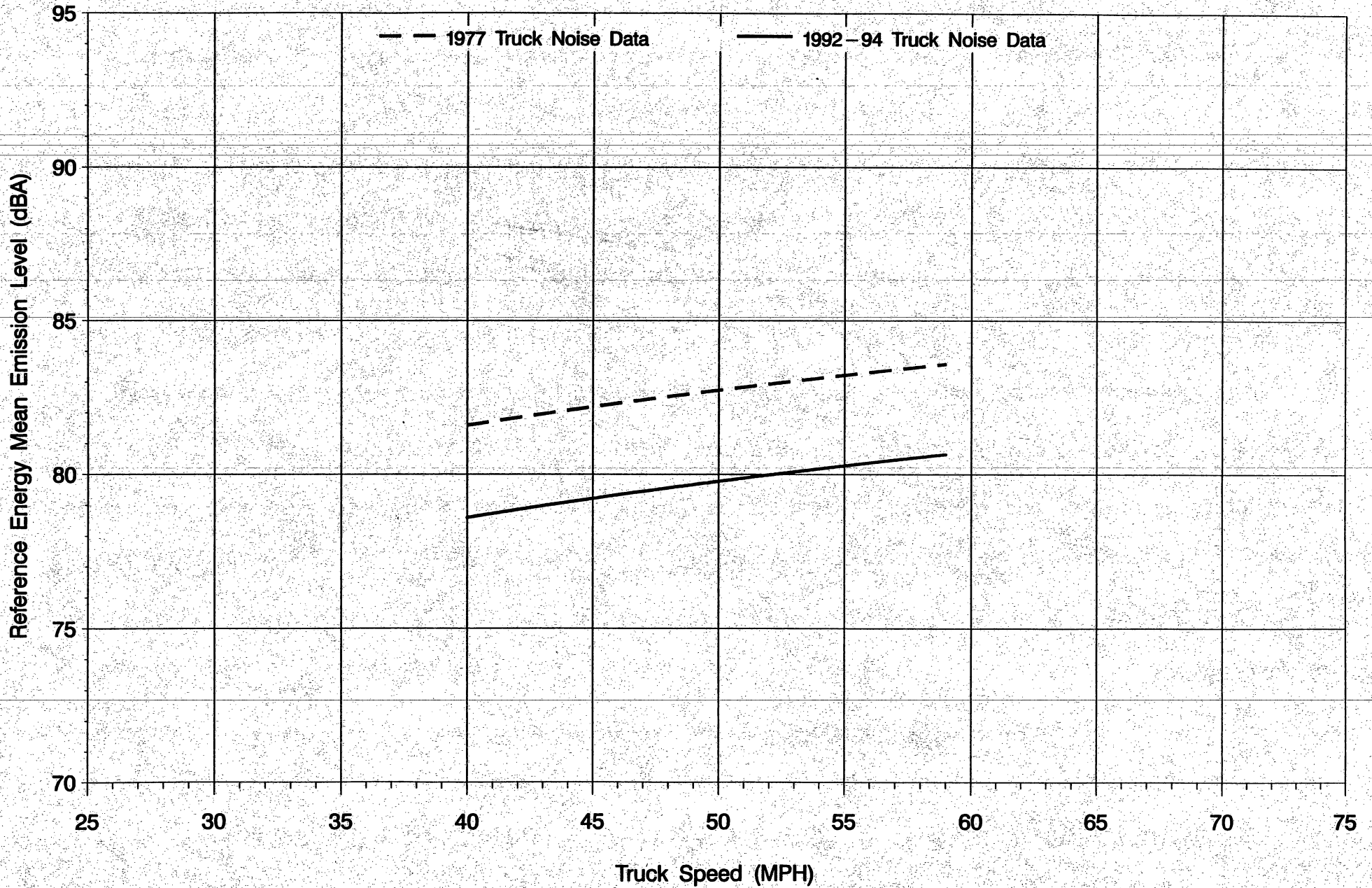
Figure 6: REMEL vs. Truck Speed ROADWAY TYPE 2 (Controlled Access, Upgrade) – MEDIUM TRUCKS & BUSES
