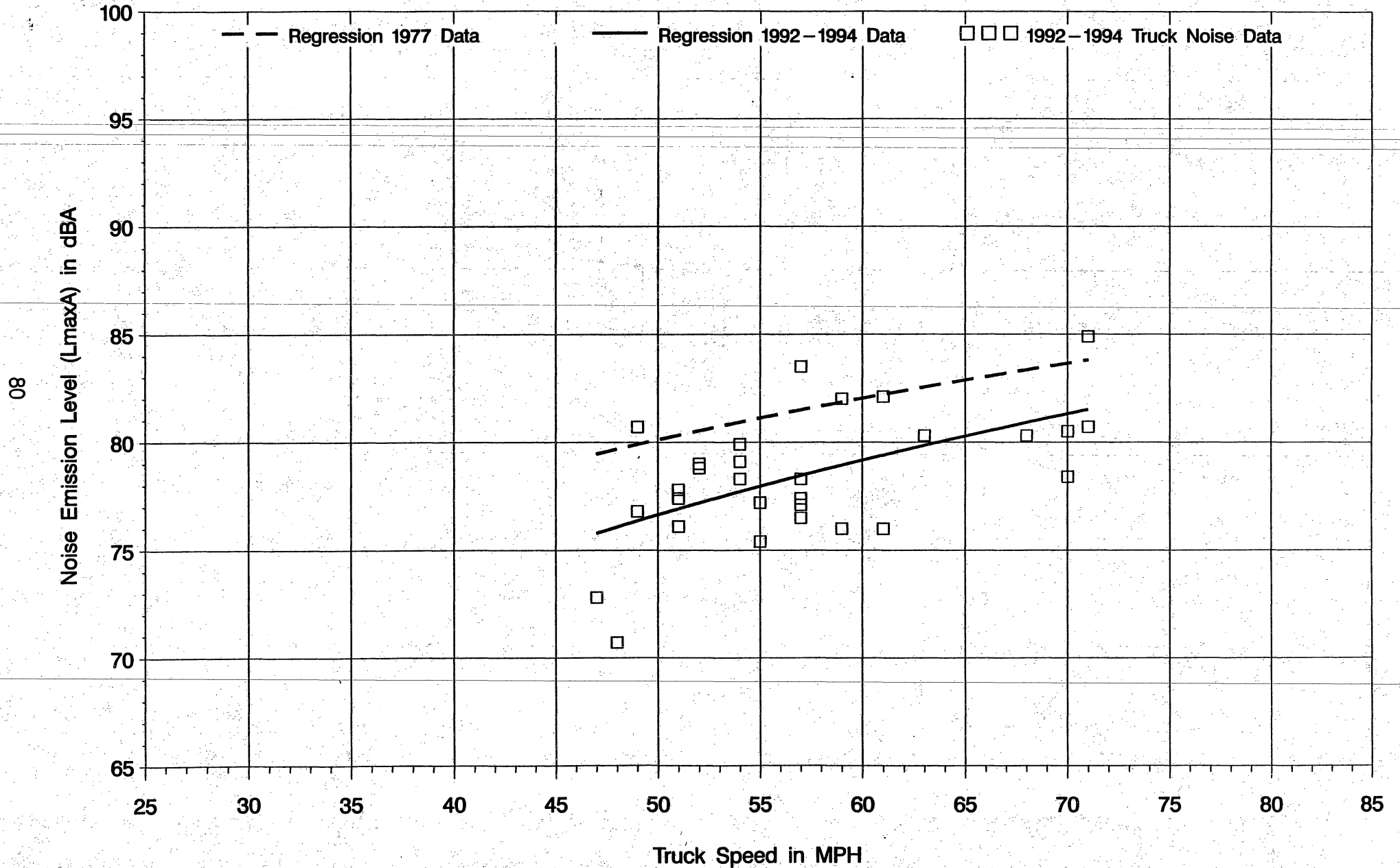
Figure B-3: Noise Emission Level (LmaxA) vs. Truck Speed ROADWAY TYPE 3 (Controlled Access, Downgrade) – MEDIUM TRUCKS & BUSES
