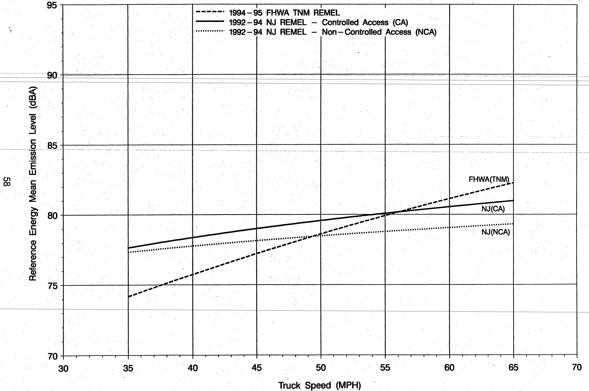
Figure 17: NJ REMELS VS. FHWA TNM REMELS – MEDIUM TRUCKS, LEVEL
