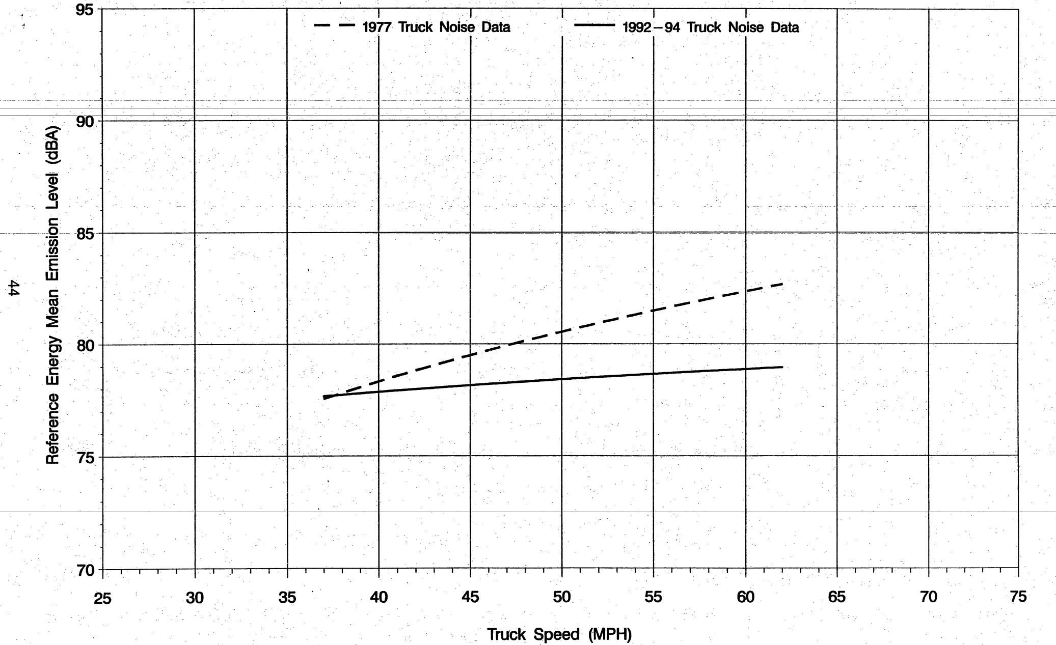
Figure 8: REMEL vs. Truck Speed ROADWAY TYPE 4 (Non – Controlled Access, Level) – MEDIUM TRUCKS & BUSES
