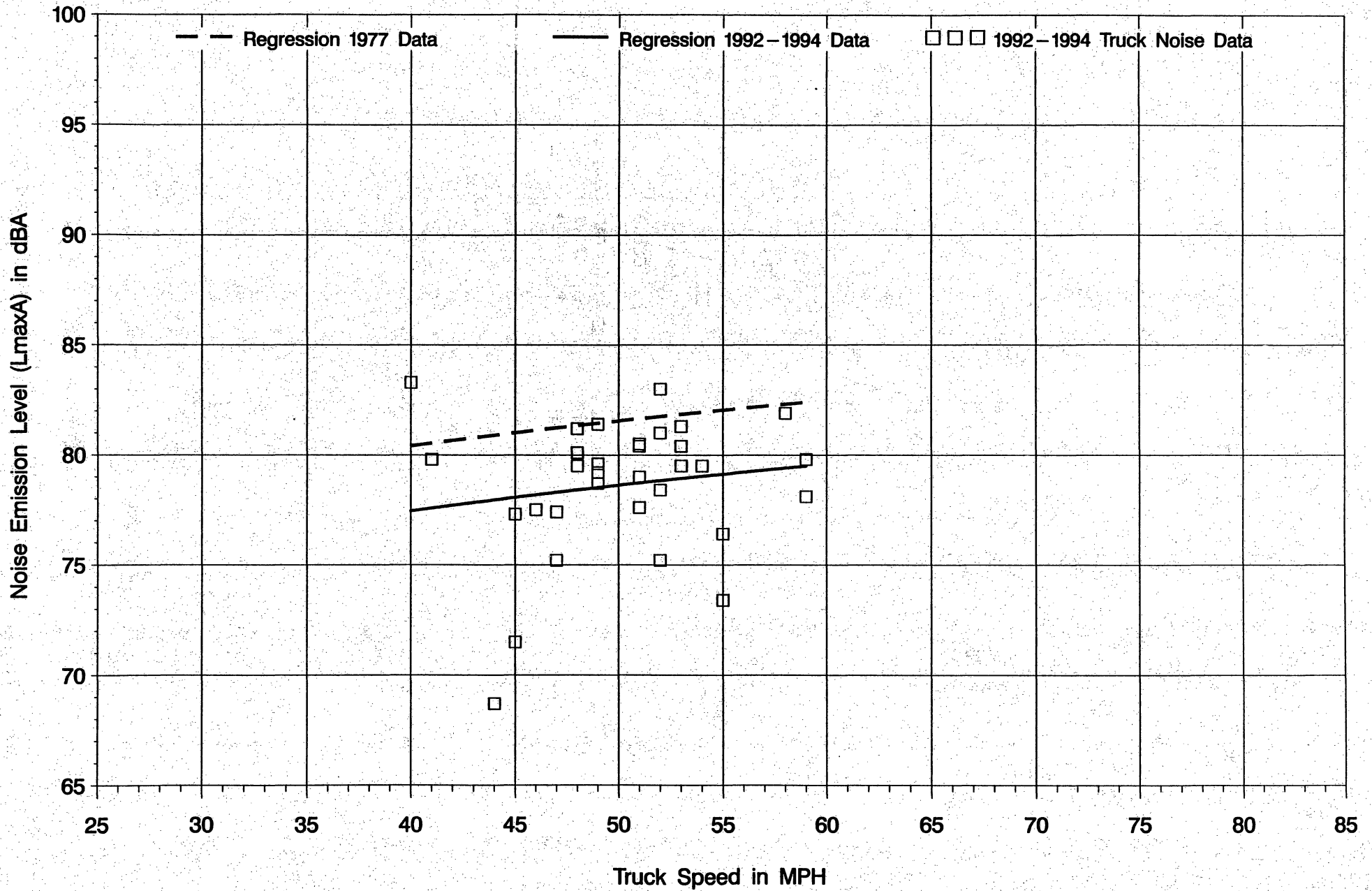
Figure B-2: Noise Emission Level (LmaxA) vs. Truck Speed ROADWAY TYPE 2 (Controlled Access, Upgrade) – MEDIUM TRUCKS & BUSES
