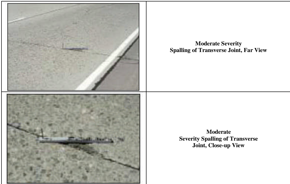
Figure 24. Illustration of Spalling of Transverse Joints
