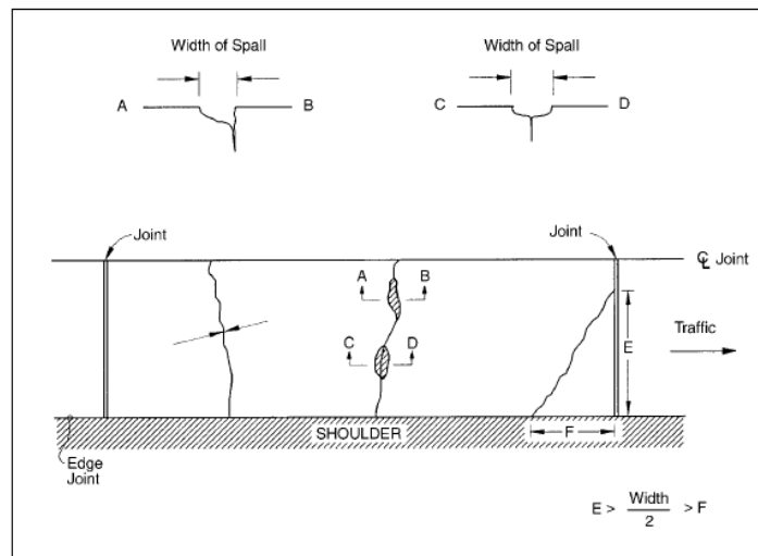
Figure 17. Transverse Cracking
