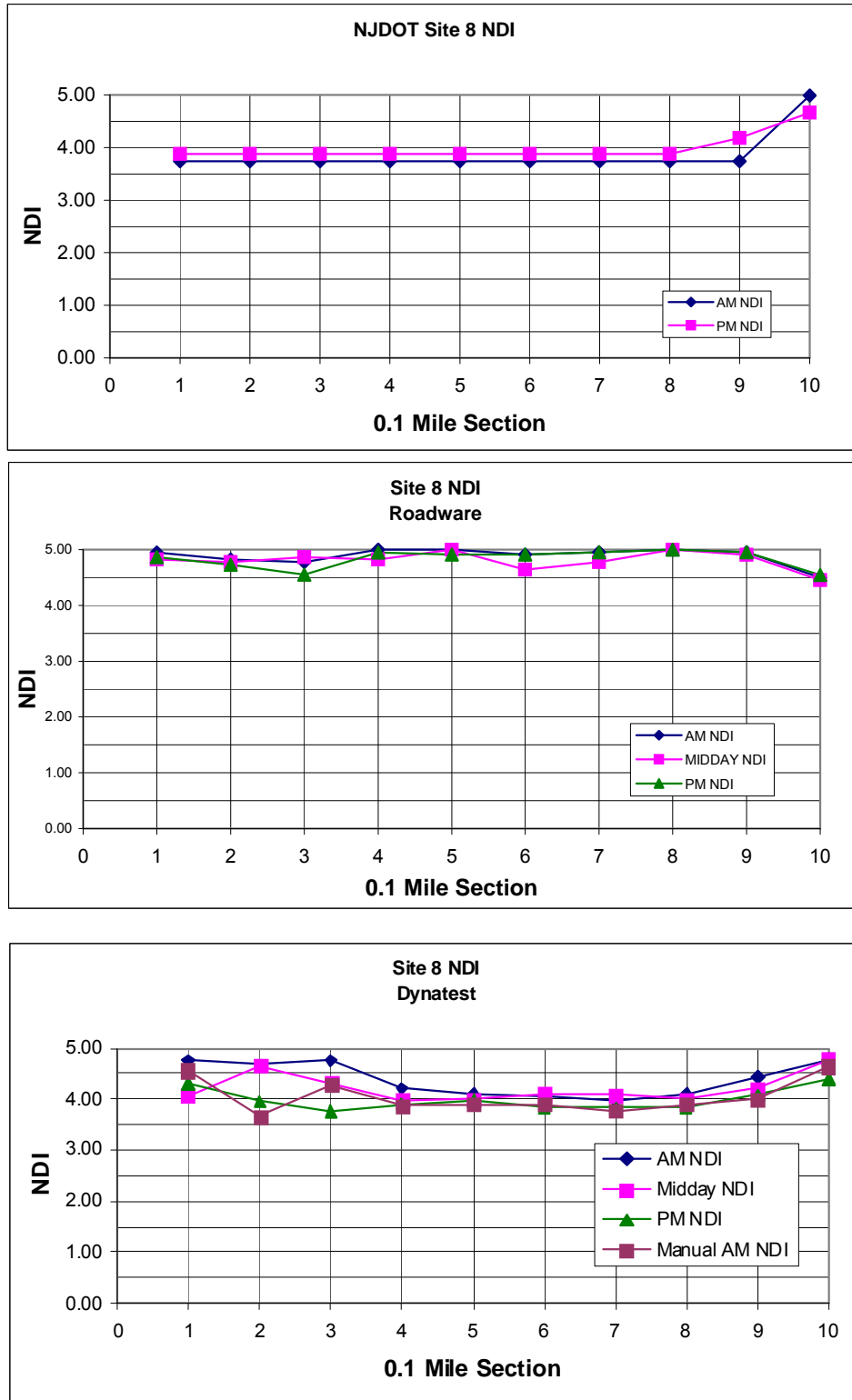
FIGURE 15. Site 8 Comparison of NDI
