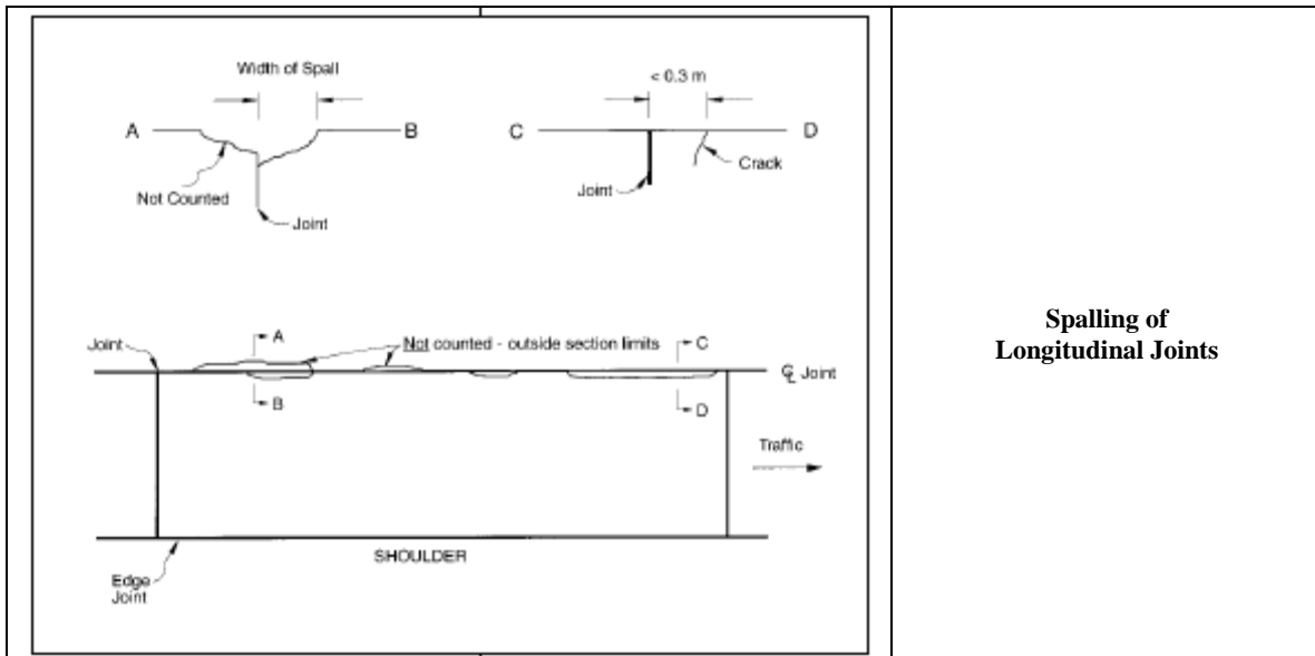
Figure 21. LONGITUDINAL JOINT SPALLING DAMAGE
