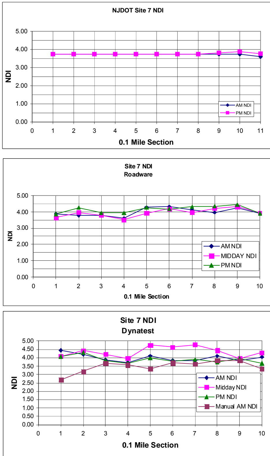
FIGURE 14. Site 7 Comparison of NDI
