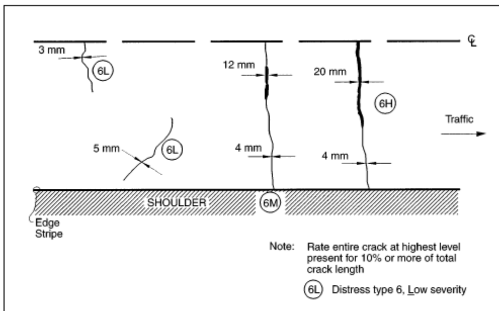
Figure 7. Transverse Cracking
