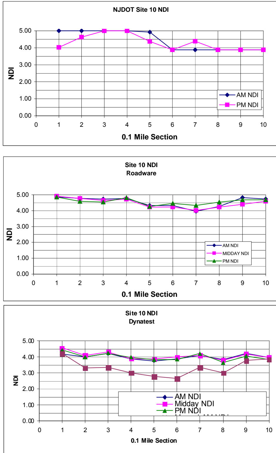
FIGURE 17. Site 10 Comparison of NDI
