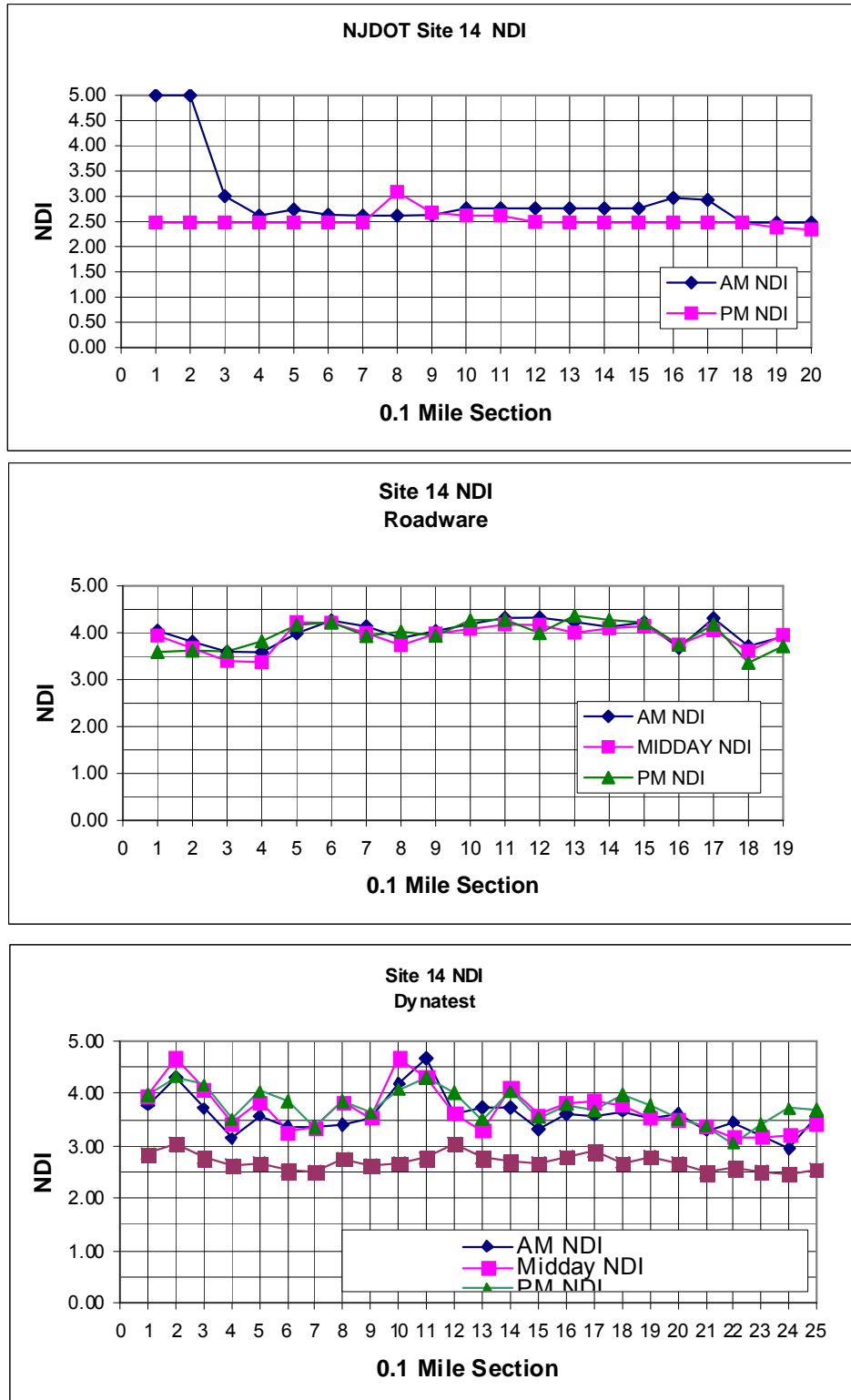
FIGURE 21. Site 14 Comparison of NDI
