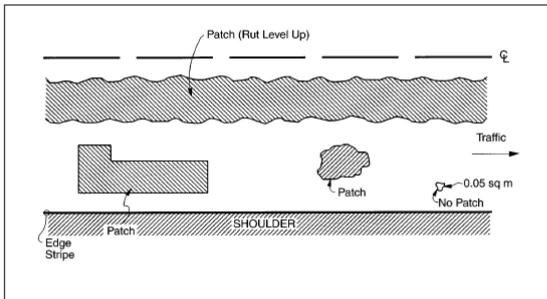
Figure 9. Patching
