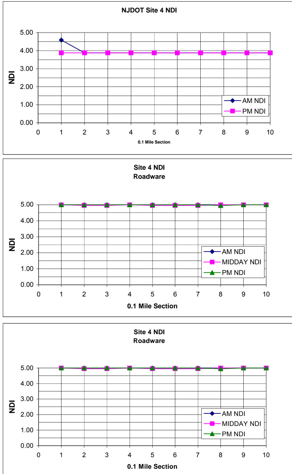
FIGURE 11. Site 4 Comparison of NDI
