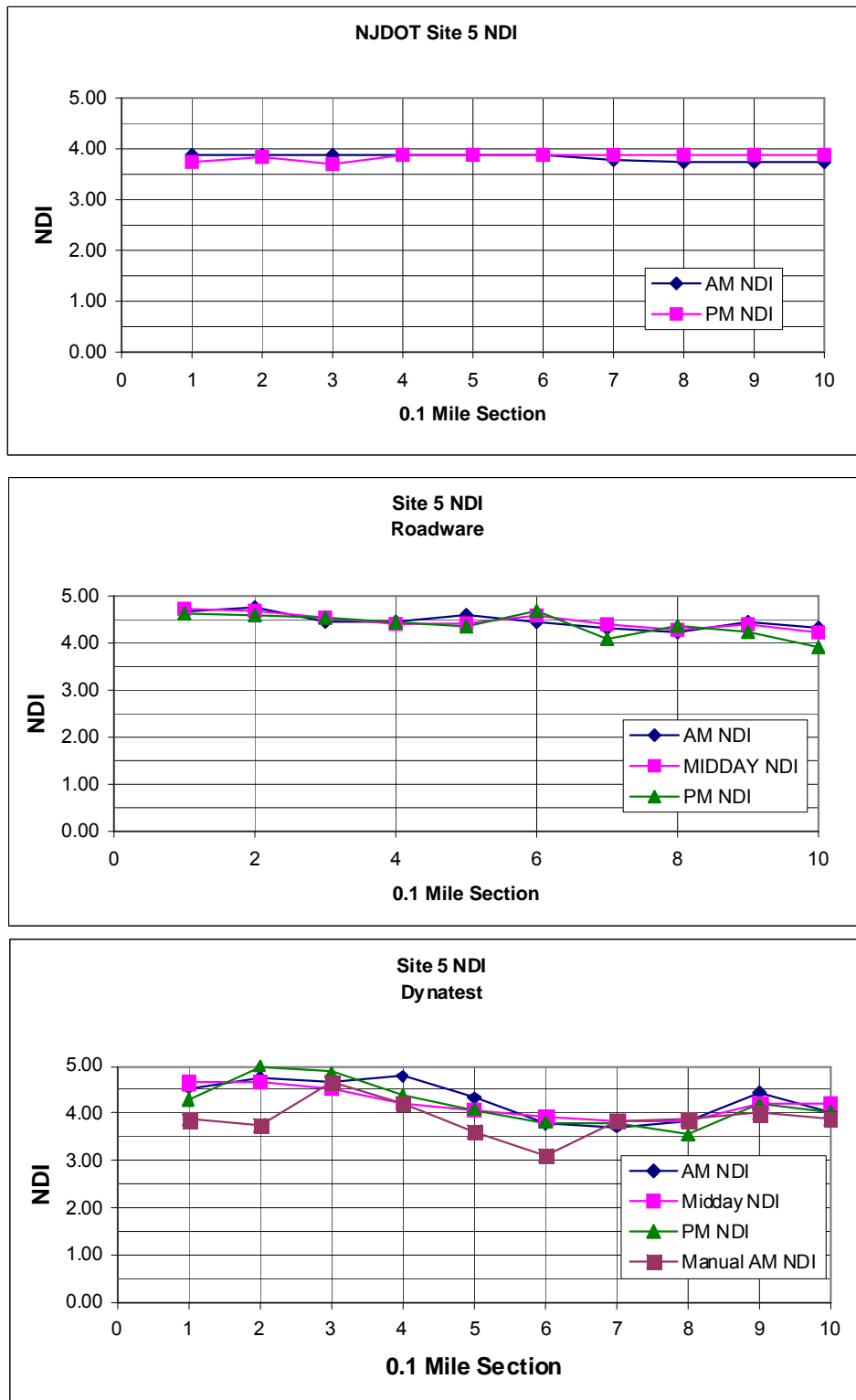
FIGURE 12. Site 5 Comparison of NDI
