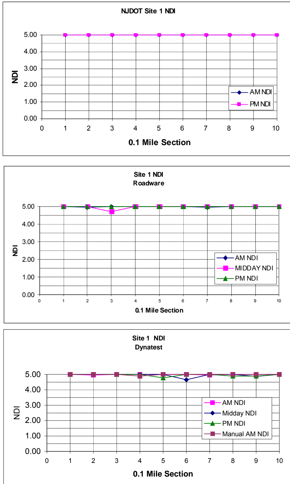
Figure 10. Site 1 Comparison of NDI
