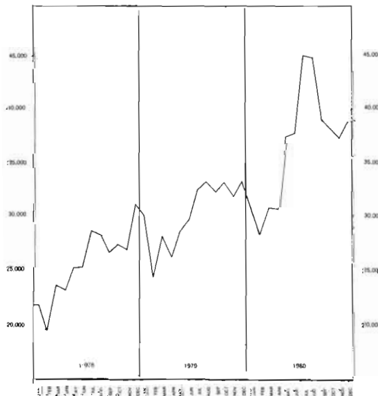
Violent Crime By Month 1978-1979-1980
