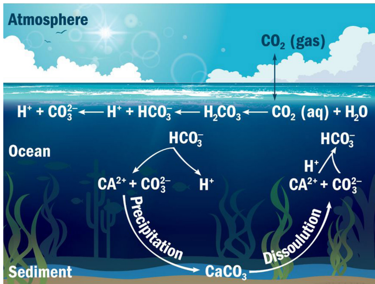
Figure 4.9. Process Contributing to Ocean Acidification. The Chemical Reaction That Leads to Ocean Acidification with the Introduction of CO 2 Into the Ocean.
