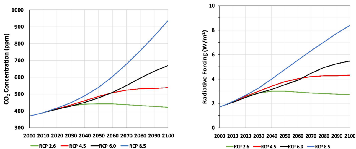
Figure 1.2. Projections of atmospheric CO 2 concentration and total radiative forcing through 2100 based on each RCP scenario. Data are available from the RCP Database (Version 2.0). Scenarios and projections follow (van Vuuren et al. 2011).
