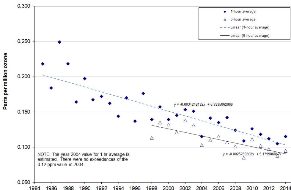
Figure 5.6. Maximum Ozone Concentrations per Year at All Monitoring Sites in New Jersey (1985 – 2014). The solid and dashed lines represent statistically significant linear trends with time (NJDEP, 2016).
