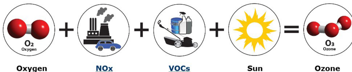
Figure 5.2. How Smog is Formed. Ground-level ozone, also known as smog, is formed when oxides of nitrogen (NO x ) and volatile organic compounds (VOCs) react in the presence of sunlight (NJDEP 2020d).
