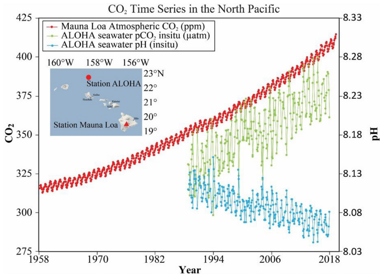
Data: Mauna Loa ( ftp://aftp.cmdl.noaa.gov/products/trends/co2/co2_mm_mlo.txt ) ALOHA ( http://hahana.soest.hawaii.edu/hot/products/HOT_surface_CO2.txt ) Ref: J.E. Dore et al, 2009. Physical and biogeochemical modulation of ocean acidification in the central North Pacific. Proc Natl Acad Sci USA 106 :12235-12240.
