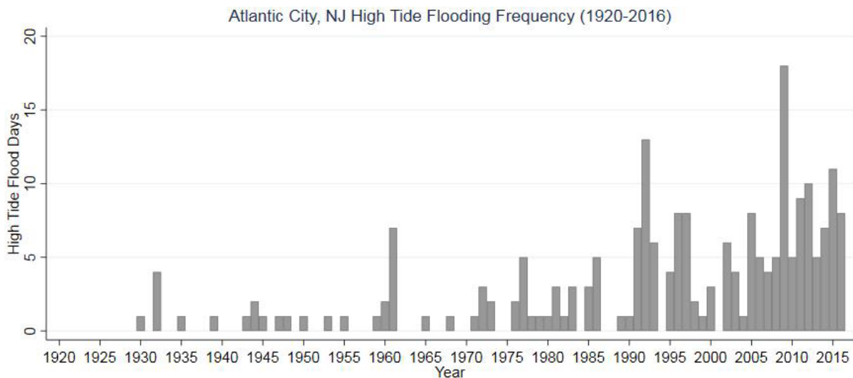
Figure 4.7. Historical High Tide Flooding Frequency (number of Flood Days) for Atlantic City, New Jersey. The number of high-tide flooding days has continued to rise in Atlantic City, NJ since 1930 (Kopp et al. 2019).
