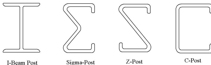
Figure 6. Various Post Designs. The I-beam post is the most commonly used post; however, it also poses the greatest threat to motorcycles. The \Sigma -, Z-, and C- posts have a more rounded shape and less harsh edges, making them safer for motorcyclists (Adapted from [30]).
