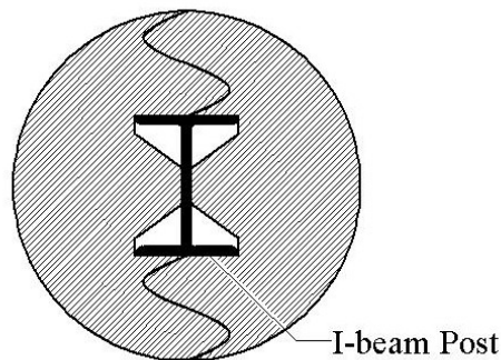
Figure 5. Sample Impact Attenuator. Impact attenuators surround posts, creating a larger surface area for impact as well as protecting motorcyclists from the sharp edges of posts (Adapted from FEMA, 2000).
