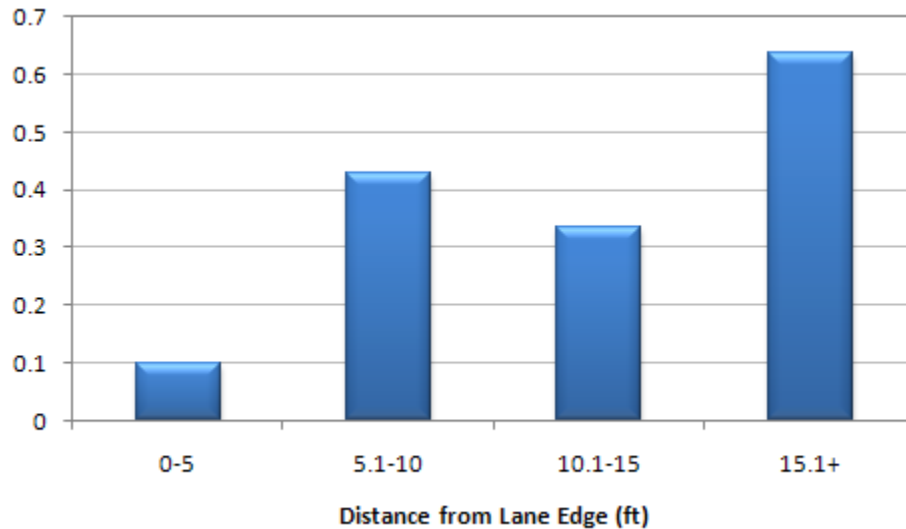
Figure 51. Risk of severe injury from fixed object as a function of distance from the lane edge
