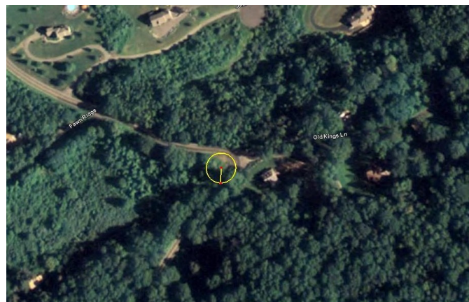
Figure 47. Radius measurement of example site. The radius of the curve was measure to be 49 feet.
