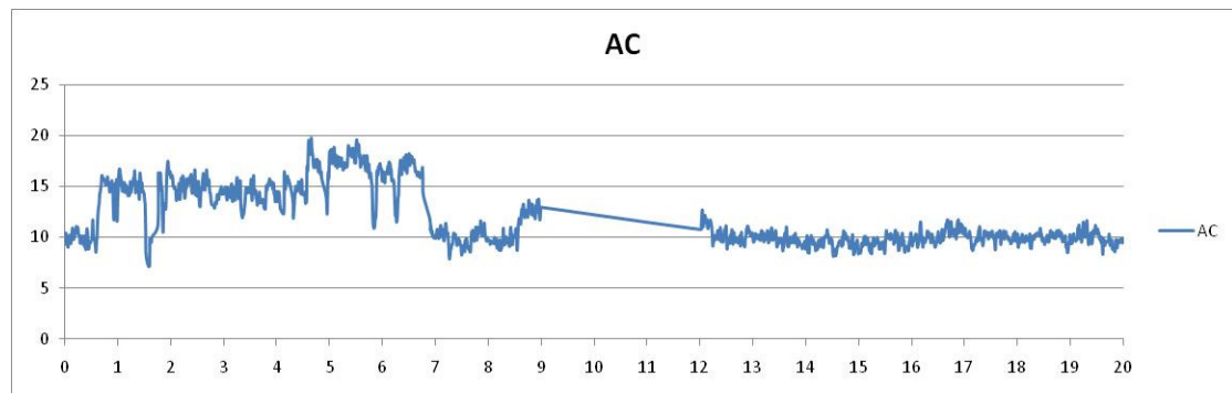
Figure 5a. Pavement layer profile – AC only - GPR.
