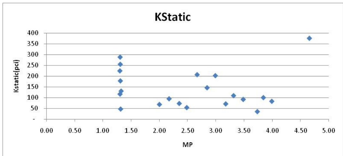
Figure 11. Kstatic profile.
