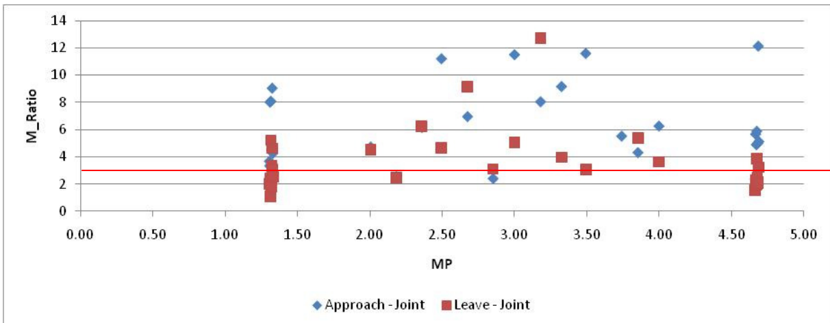
Figure 18. Calculated M-Ration
