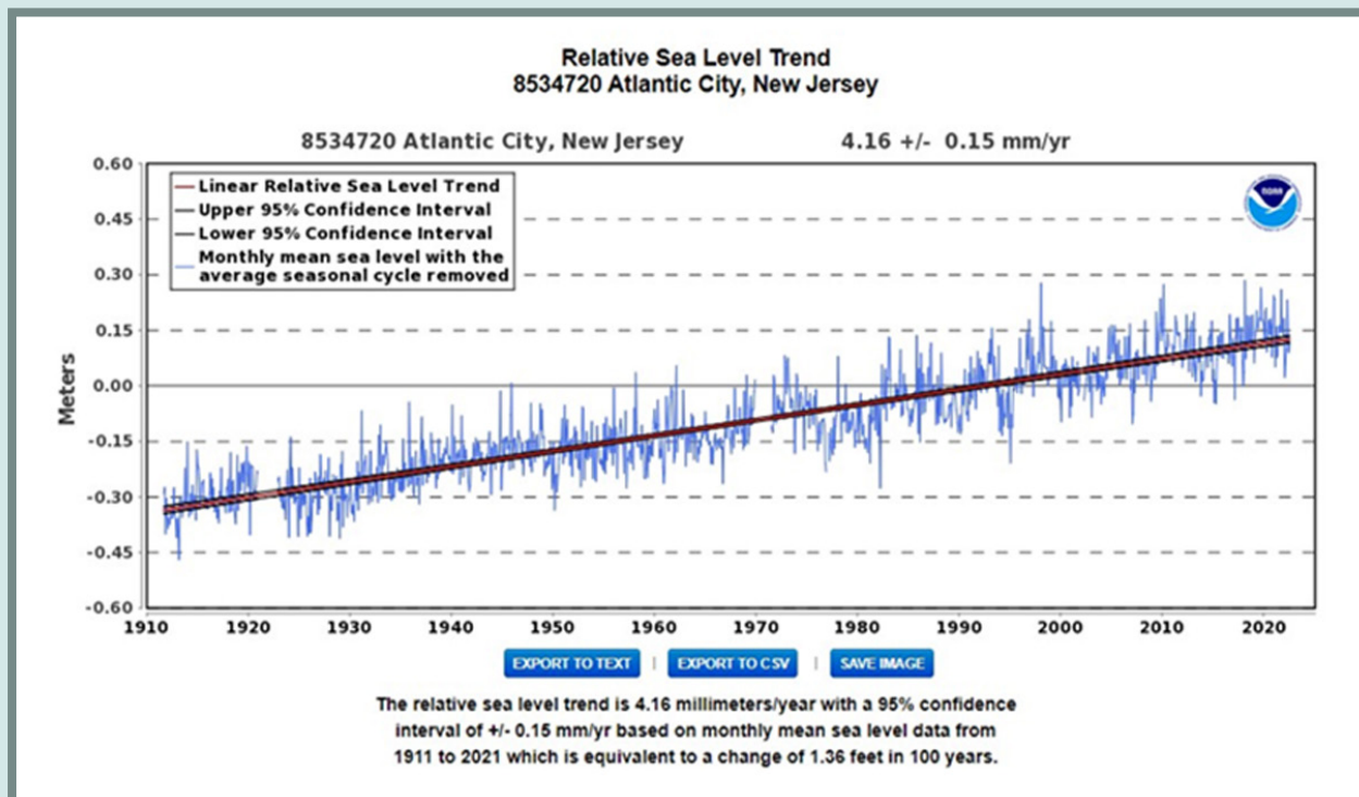
Figure 3.3a Sea level Trend for Atlantic City (NOAA).
