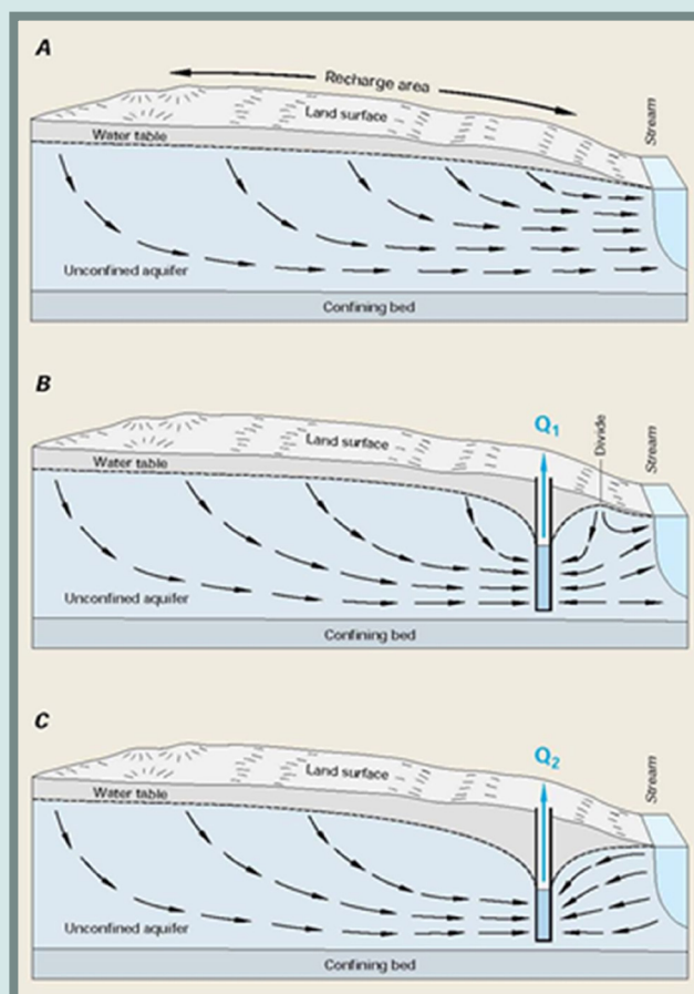
Figure 2.3 Unconfined Groundwater and Stream Flow: (a) natural conditions; (b) diverted by a pumping well; and (c) as diverted by a pumping well with induced stream leakage (modified from Winter et al., 1999).
