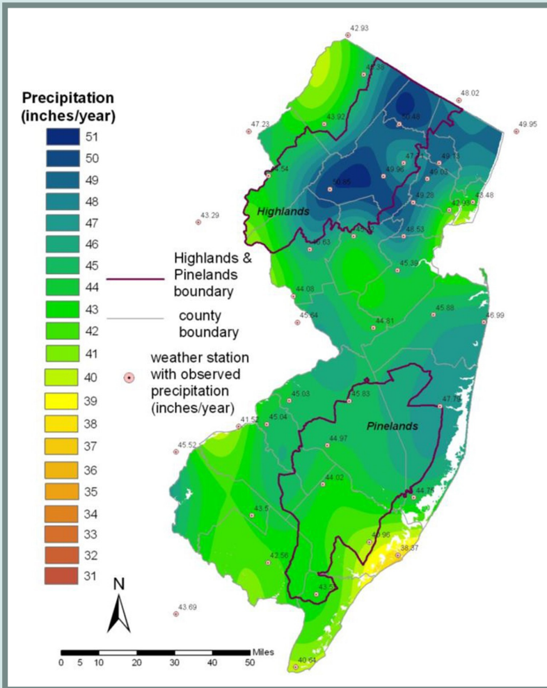
Figure 7.1 New Jersey annual average precipitation.
