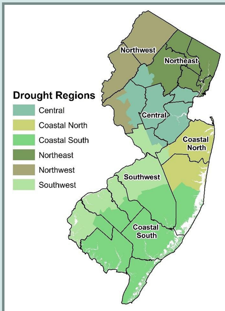
Figure 7.3 New Jersey Drought Regions.
