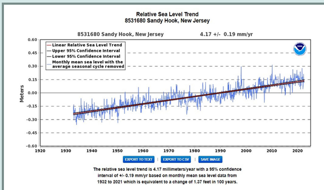
Figure 3.3b Sea level Trend for Sandy Hook (NOAA).
