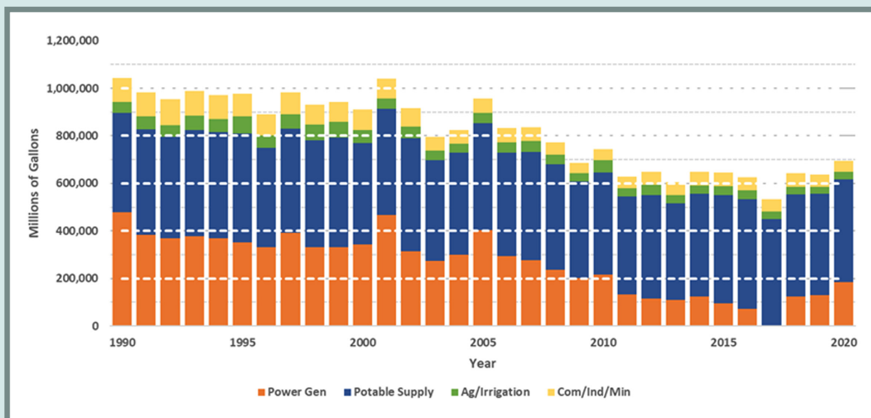
Figure 4.2 Water Withdrawals by Use Sector, 1990-2020.
