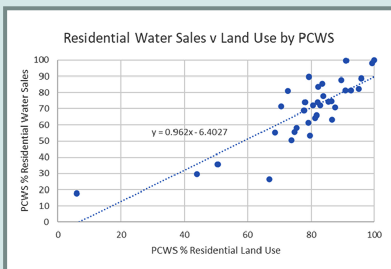
Figure 4.14 Percent PCWS Residential Demands Relative to Residential Land Use (n=210).
