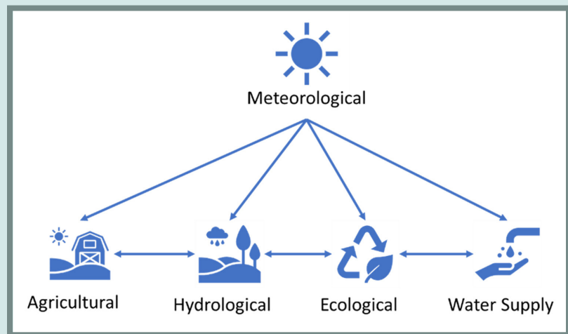
Figure 7.2 Drought type infographic.
