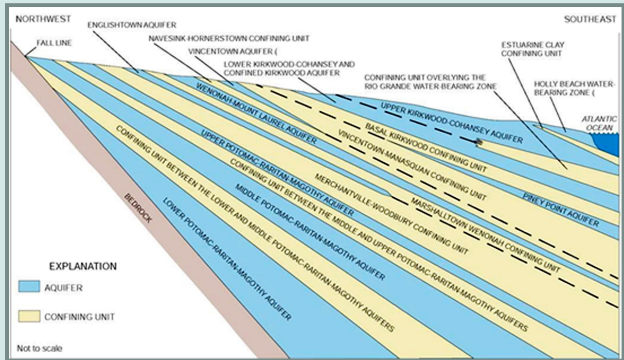
Figure 2.5 Generalized Cross Section of New Jersey's Coastal Plain Aquifer System (from Charles et al., 2011).
