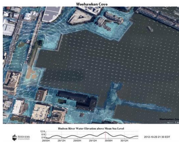
Figure 3-5: Storm Surge Modeling, Weehawken Cove, NJ.
