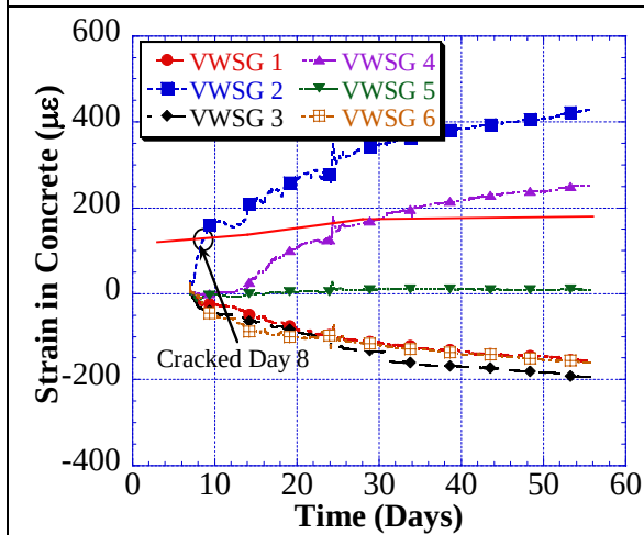
G1M1 – Specimen 1 – Concrete Strains
