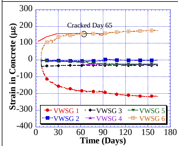
G4M4 – Specimen 1 – Concrete
