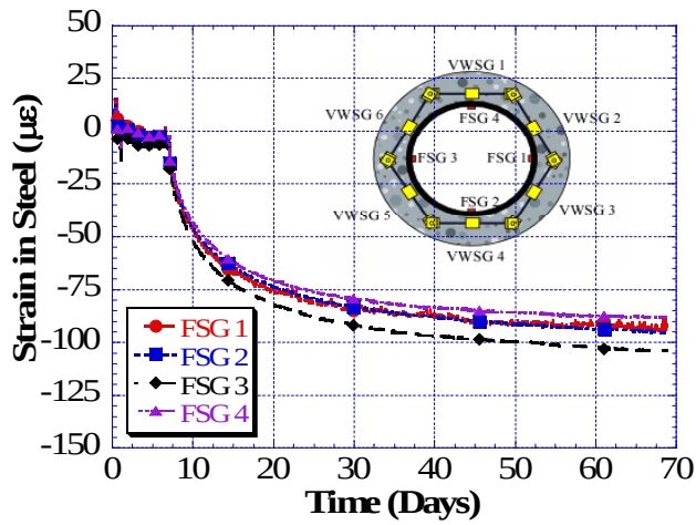
G2M5 – Specimen 1 – Steel Strains
