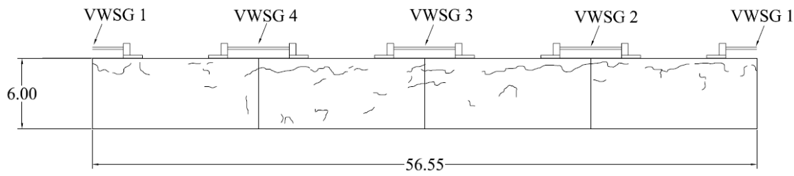
G4M3 – Ring Specimen 1 – Crack Drawings
