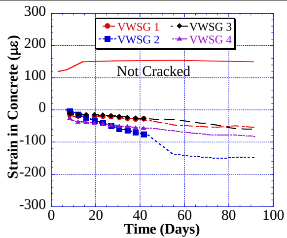
G1M3 – Specimen 2 – Concrete
