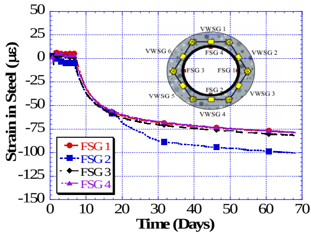
G2M6 – Specimen 1 – Steel Strains
