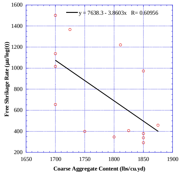
Figure 59. Coarse Aggregate Content vs. Free Shrinkage Rate for All Mixes
