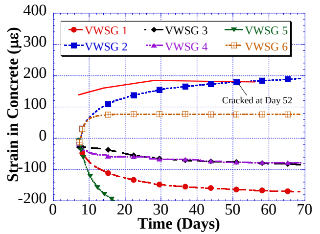
G2M5 – Specimen 2 – Concrete Strains
