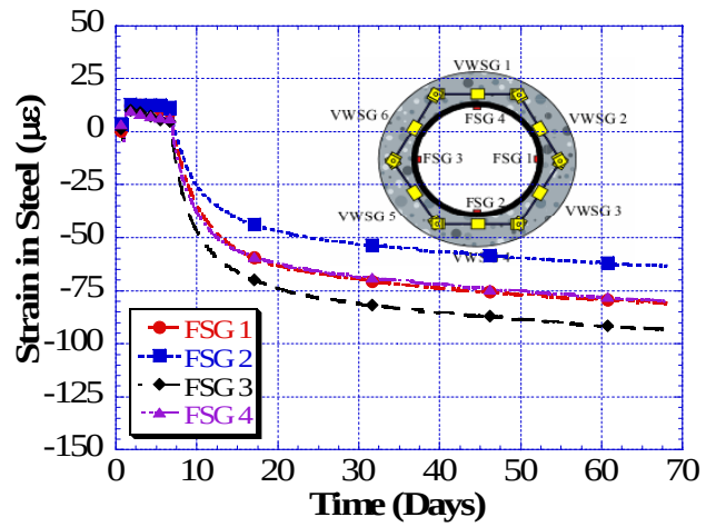
G2M6 – Specimen 2 – Steel Strains
