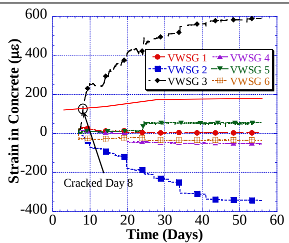
G1M1 – Specimen 2 – Concrete Strains
