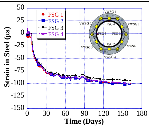
G4M4 – Specimen 2 – Steel Strains
