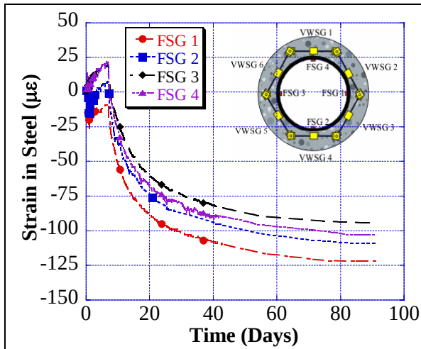
G1M3 – Specimen 1 – Steel Strains
