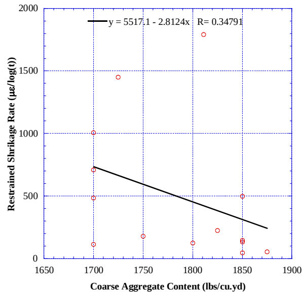
Figure 58. Coarse Aggregate Content vs. Restrained Shrinkage Rate for All Mixes
