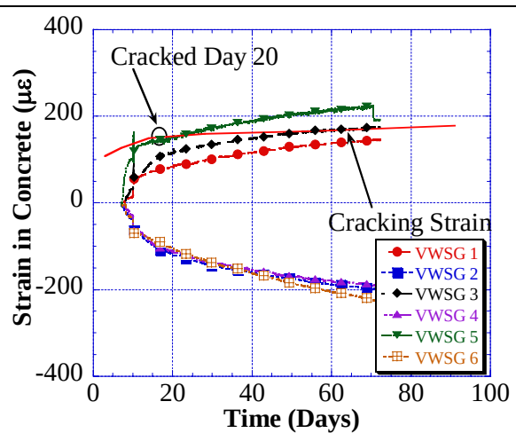
G2M4 – Specimen 2 – Concrete
