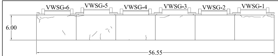
G1M3 – Ring Specimen 1 – Crack Drawings
