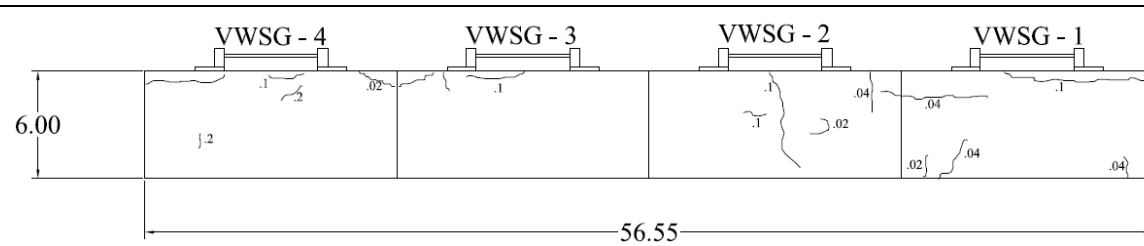
G4M2 – Ring Specimen 2 – Crack Drawings
