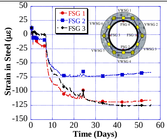
G1M1 – Specimen 2 – Steel Strains
