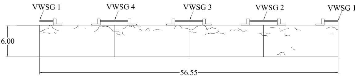
G4M3 – Ring Specimen 2 – Crack Drawings
