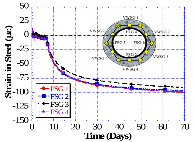
G2M5 – Specimen 2 – Steel Strains
