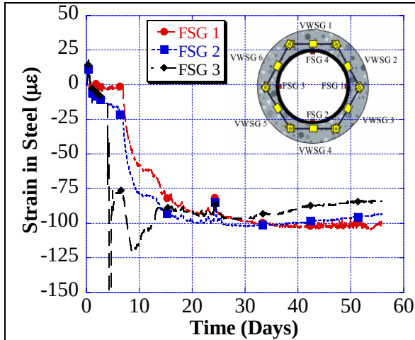
G1M1 – Specimen 1 – Steel Strains
