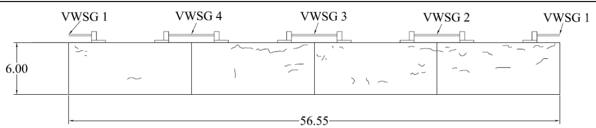
G4M1 – Ring Specimen 1 – Crack Drawings
