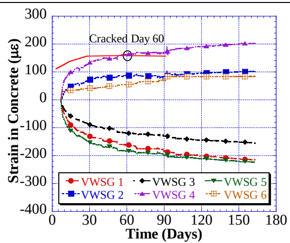
G4M4 – Specimen 2 – Concrete
