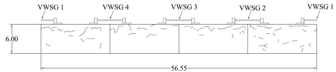
G4M1 – Ring Specimen 2 – Crack Drawings
