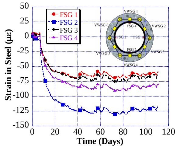
G1M3 – Specimen 2 – Steel Strains
