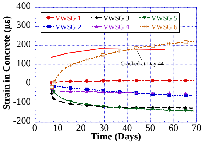
G2M5 – Specimen 1 – Concrete Strains
