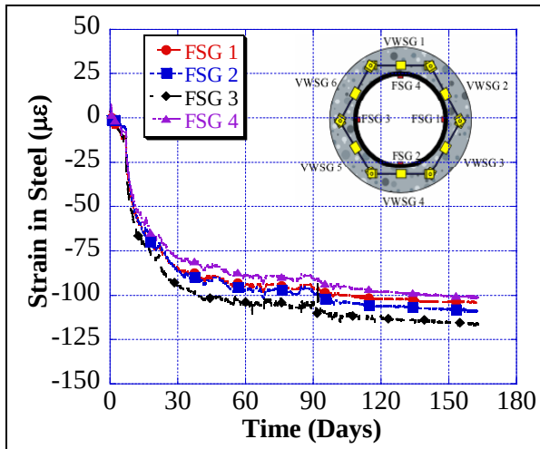
G4M4 – Specimen 1 – Steel Strains
