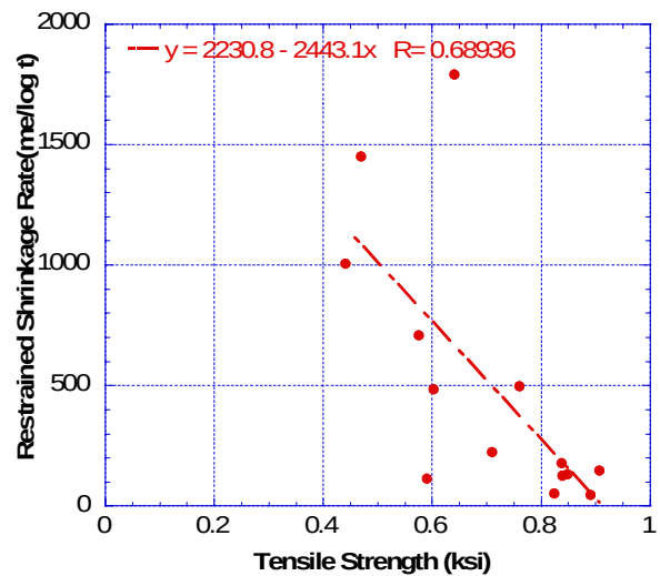
Figure 65. Restrained Shrinkage Rate versus Tensile Strength
