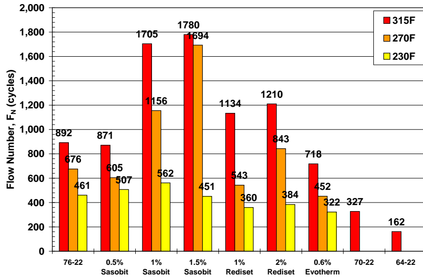
(a) – Measured Flow Number Values
