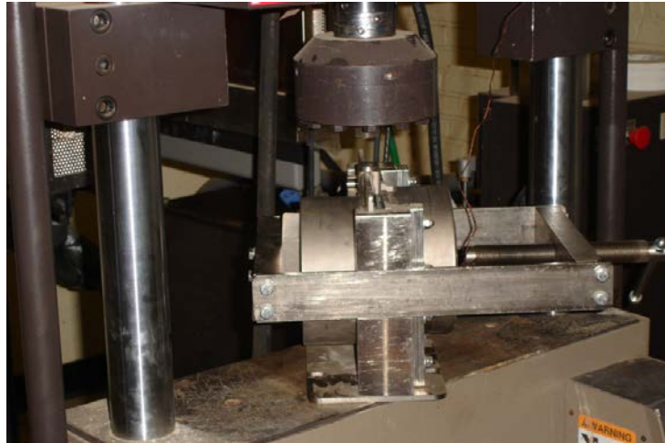
Figure 11. NCAT Bond Strength Test Device (Picture of Rutgers U. Unit)
