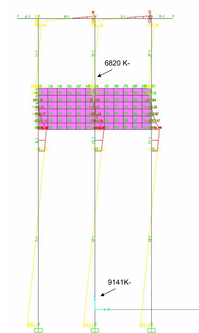
Figure VI.A.33 Model 3 Moment Distribution for Bent Subject to 1000 Kips of Transverse Loading
