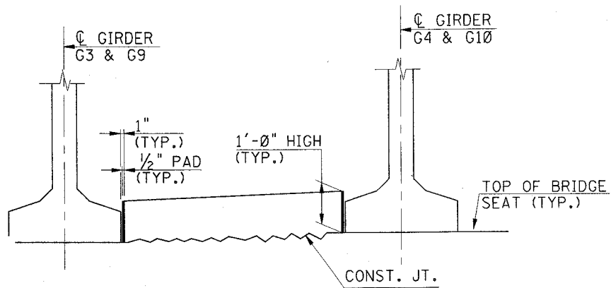
Figure VII.C.21 Keeper Block
