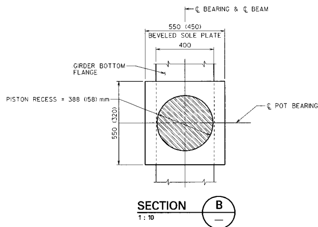
Figure VI.B.2 Fixed Pot Bearing Details
