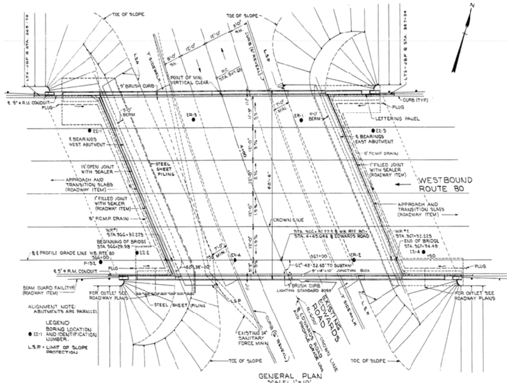
Figure 5.1 General Plan
