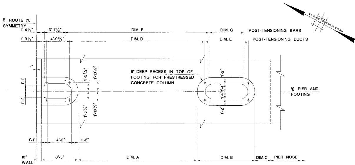
Figure VII.C.1 Pier Post - Tensioning Bars and Ducts Layout
