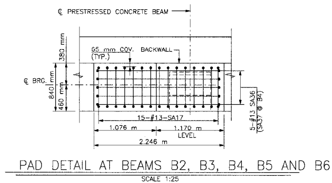
Figure VIII.C.7 South Abutment Pad Details
