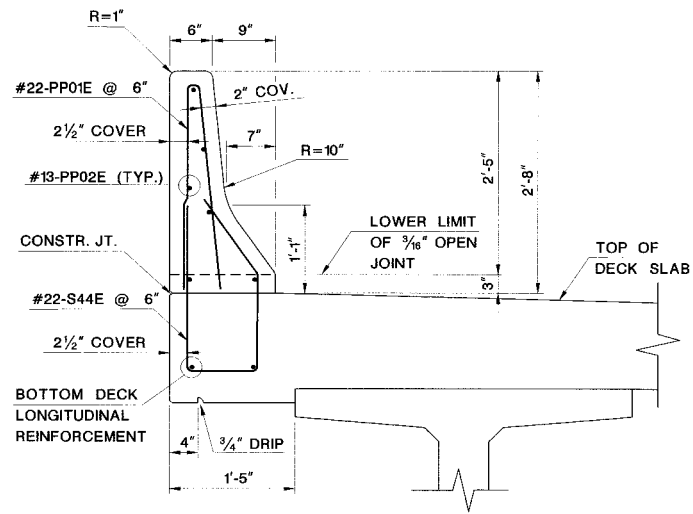
Figure VII.B.8 Typical Median Barrier Section
