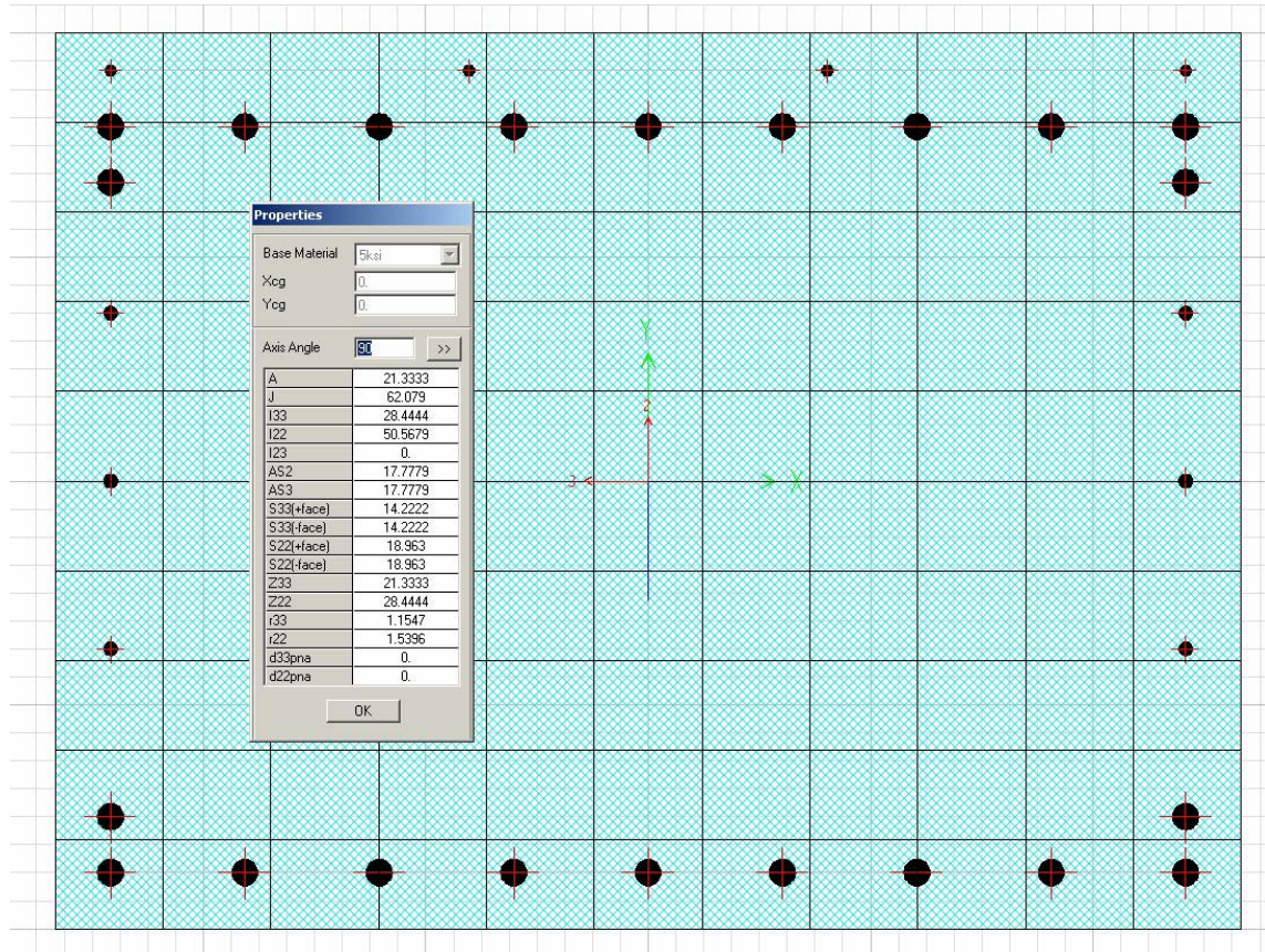
Figure VI.A.11 Bent Cap Gross Properties
