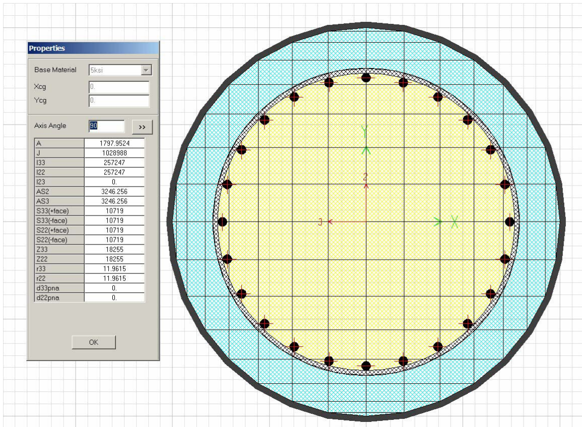
Figure VI.A.19 Column Casing Gross Properties CSE2
