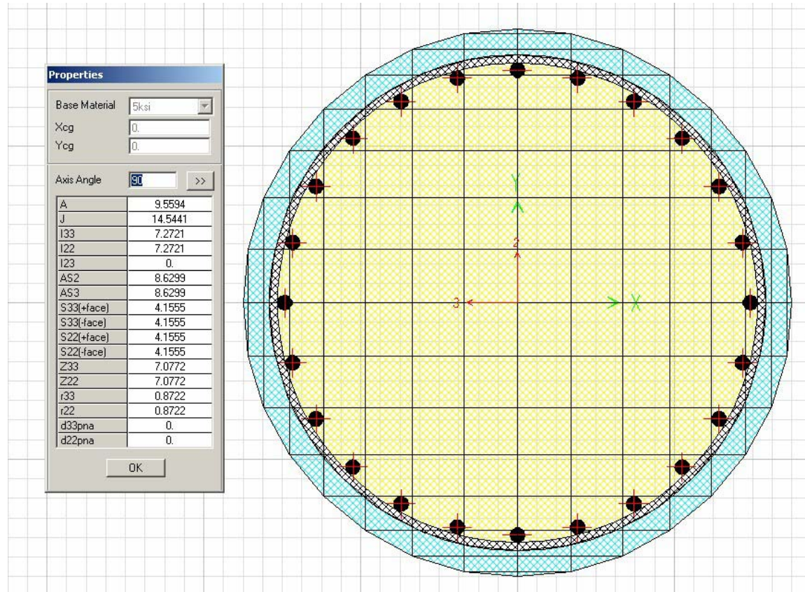
Figure VI.A.5 Column Gross Properties (CS1)
