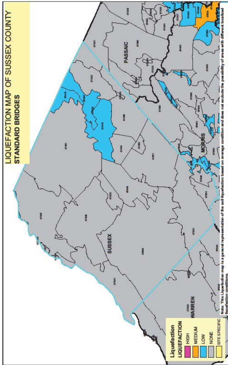
Figure III.20 Liquefaction Map for Standard Bridges in Sussex County of New Jersey
