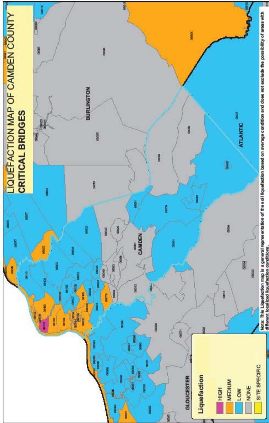
Figure III.26 Liquefaction Map for Critical Bridges in Camden County of New Jersey
