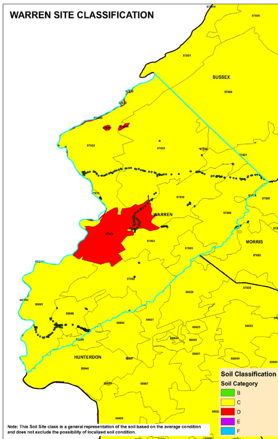
Figure II.26 Soil Site Class Map for Warren County of New Jersey
