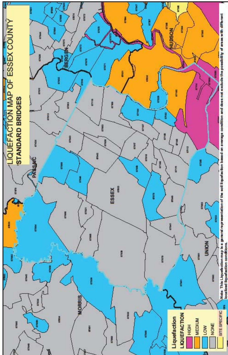
Figure III.8 Liquefaction Map for Standard Bridges in Essex County of New Jersey
