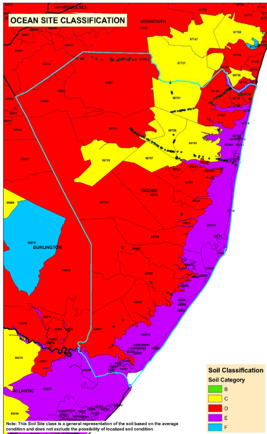
Figure II.20 Soil Site Class Map for Ocean County of New Jersey
