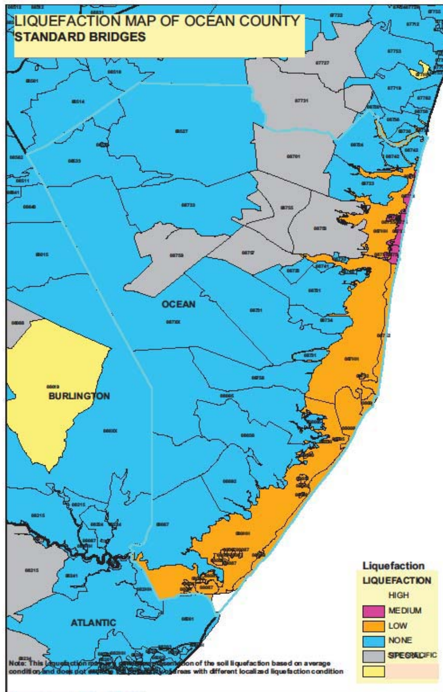
Figure III.16 Liquefaction Map for Standard Bridges in Ocean County of New Jersey
