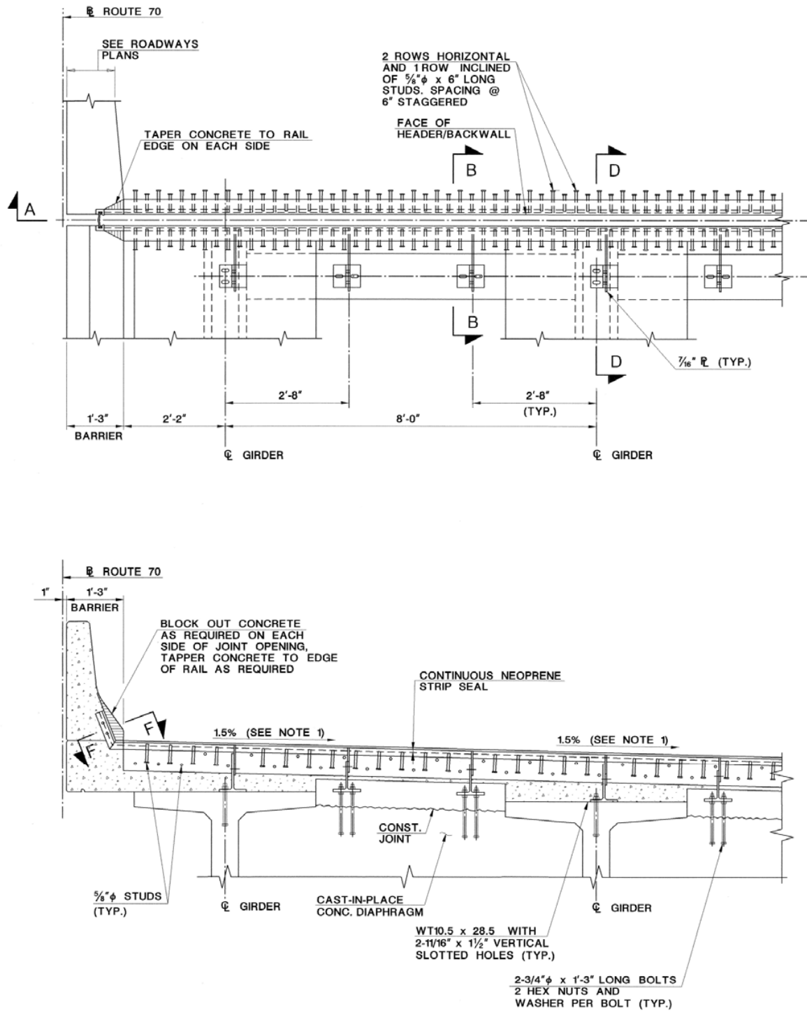
Figure VII.B.9 Expansion Joint – Plan and Elevation
