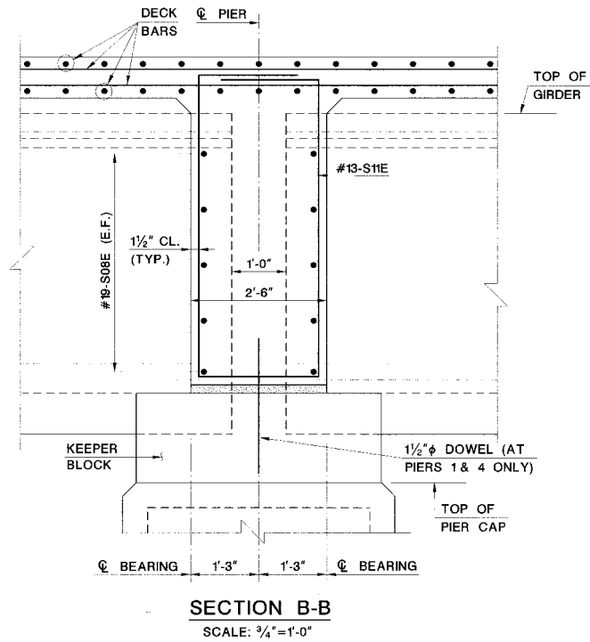
Figure VII.B.12 Diaphragm at Piers 1 and 4
