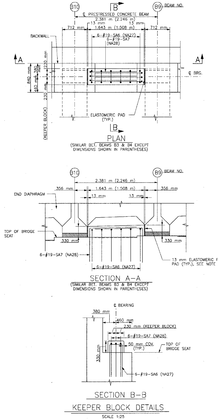
Figure VIII.C.6 South Abutment Keeper Block Details
