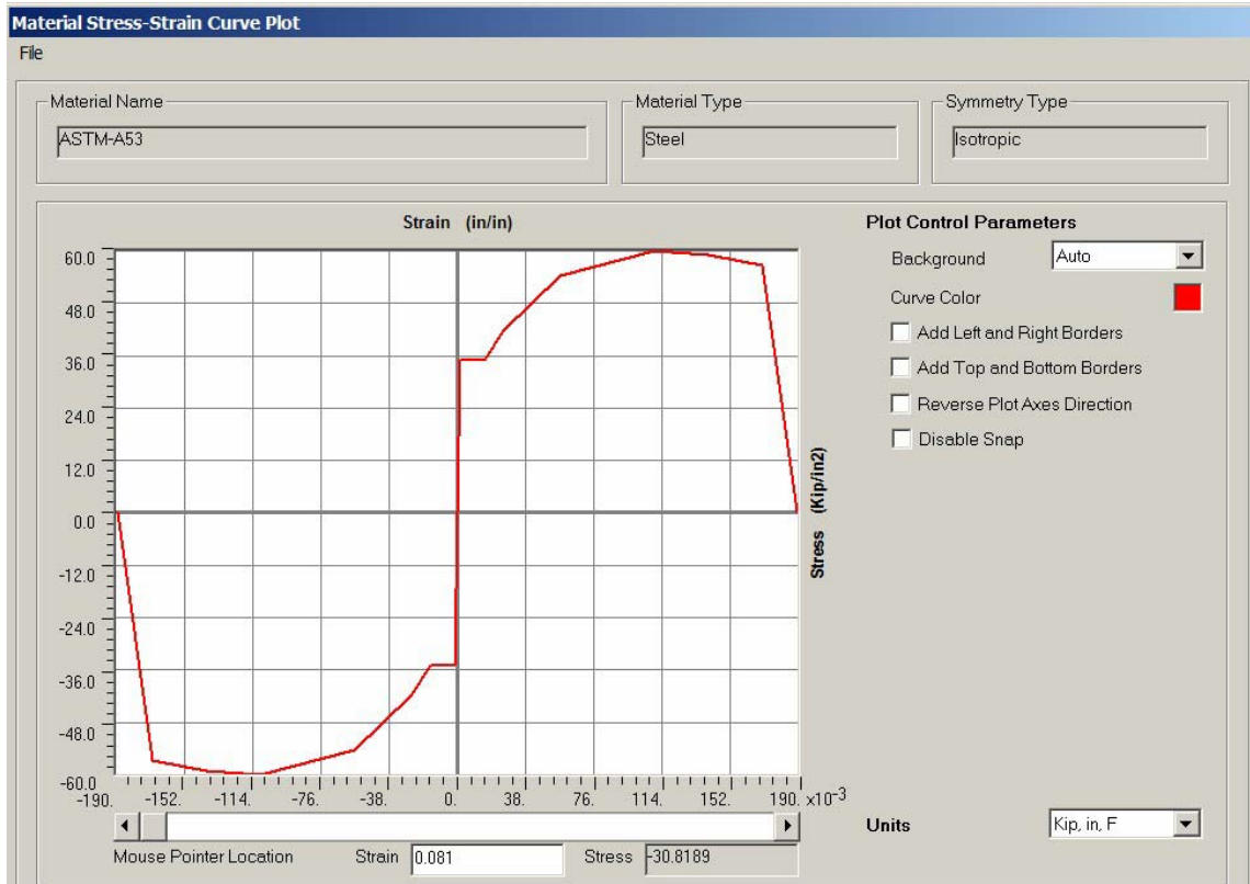
Figure VI.A.4 ASTM-A53 Grade Steel Casing Stress-Strain Model
