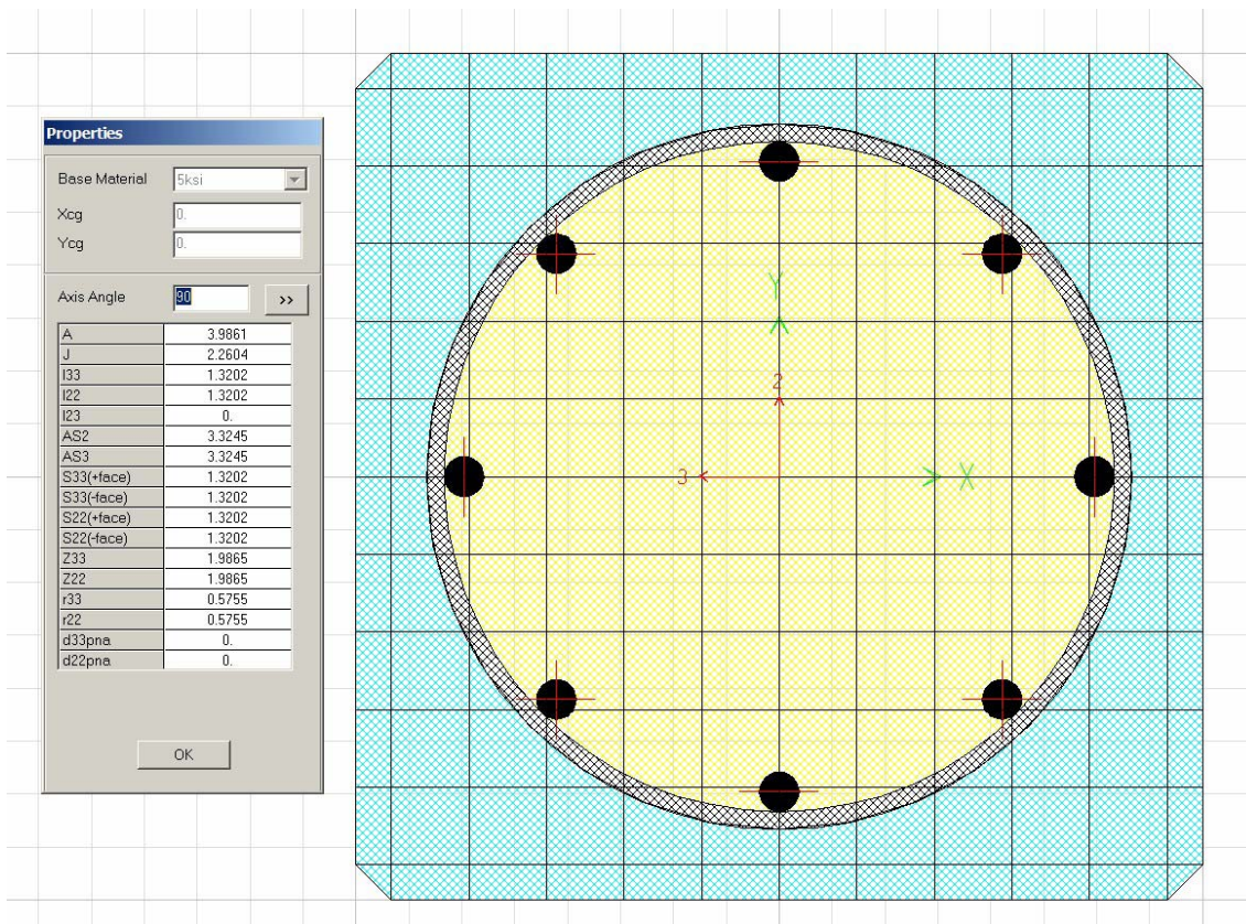
Figure VIII.A.4 Pile Gross Properties (PT)
