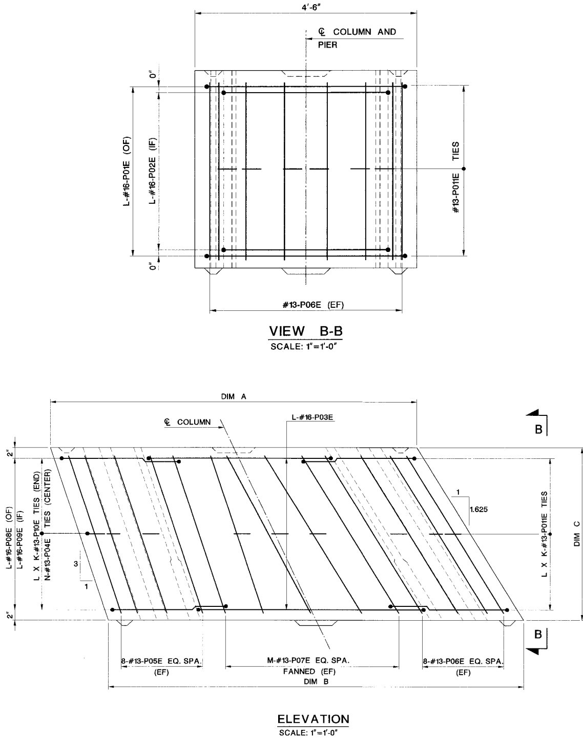
Figure VII.C.13 Outer Column Elevation and View
