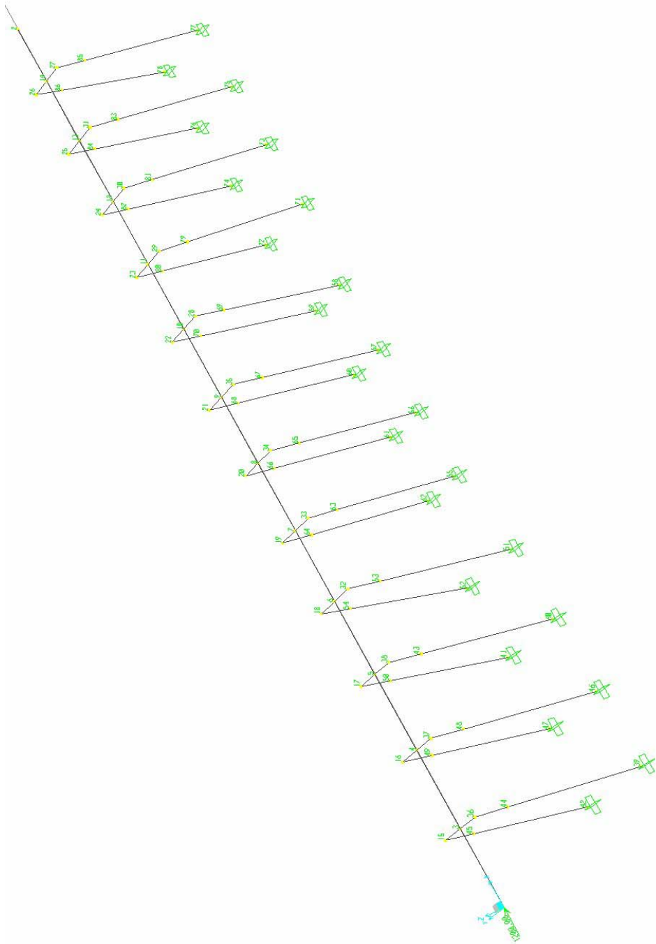
Figure VIII.A.8 CSI-SAP Model Subjected to 1200 Kips Transverse Loading.
