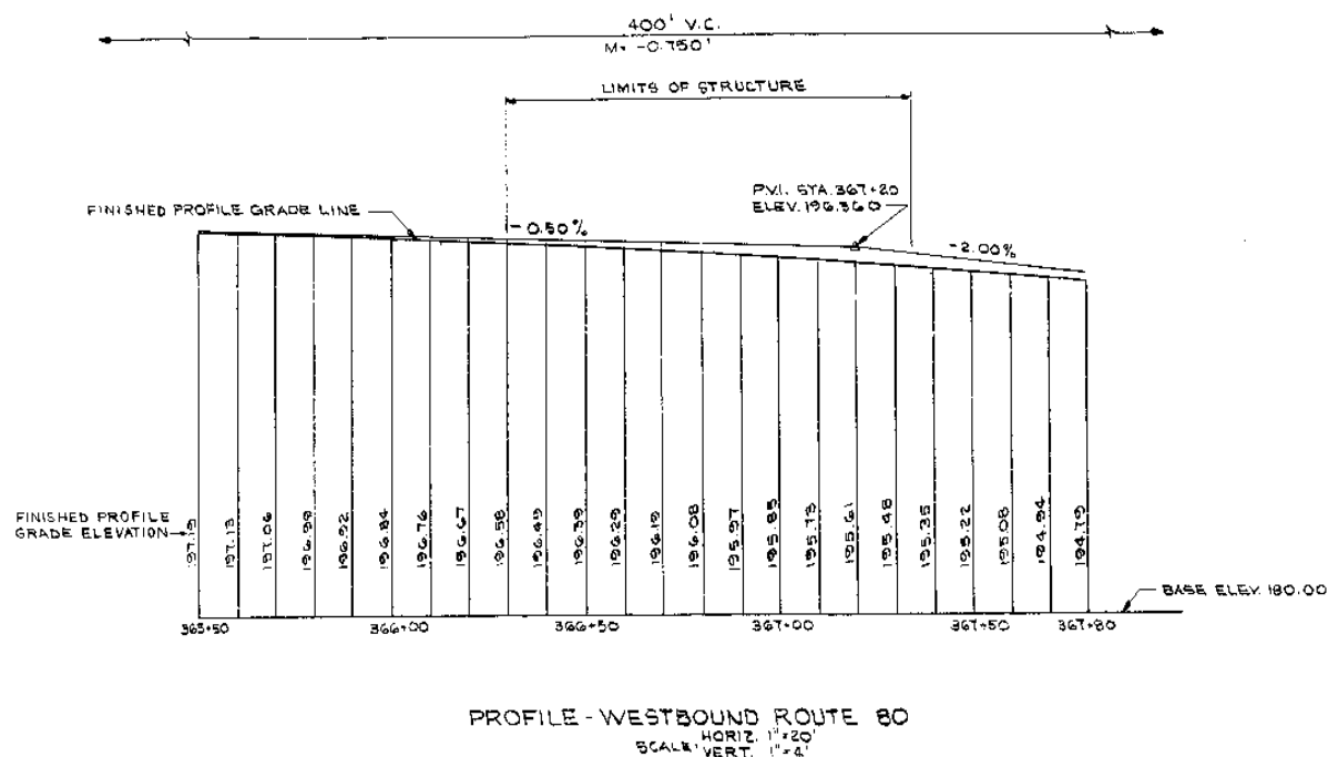
Figure 5.24 Roadway Profile
