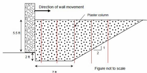
Figure IV.B.3 Schematic cross section through test specimen illustrating the shape of the excavated surface and backfill
