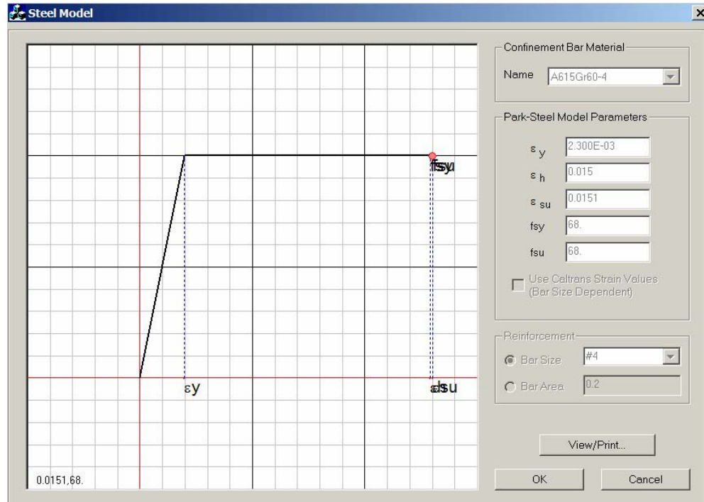
FIGURE V.3 TRANSVERSE REINFORCEMENT STRESS-STRAIN MODEL.
