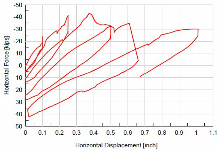
Figure IV.B.4 Load-displacement curve without backfill soil
