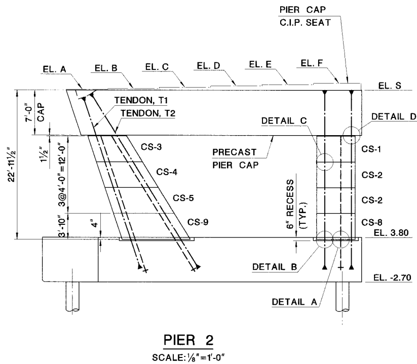
Figure VII.C.3 Piers 1 and 2 Precast Segment Elevation
