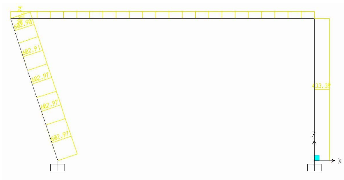
Figure VII.A.52 Pier 3 Transverse Members Shear Lateral 1
