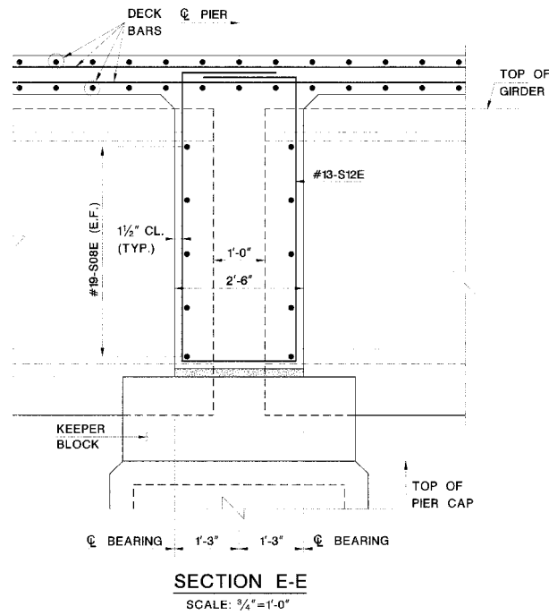
Figure VII.B.13 Diaphragm at Piers 2 and 5
