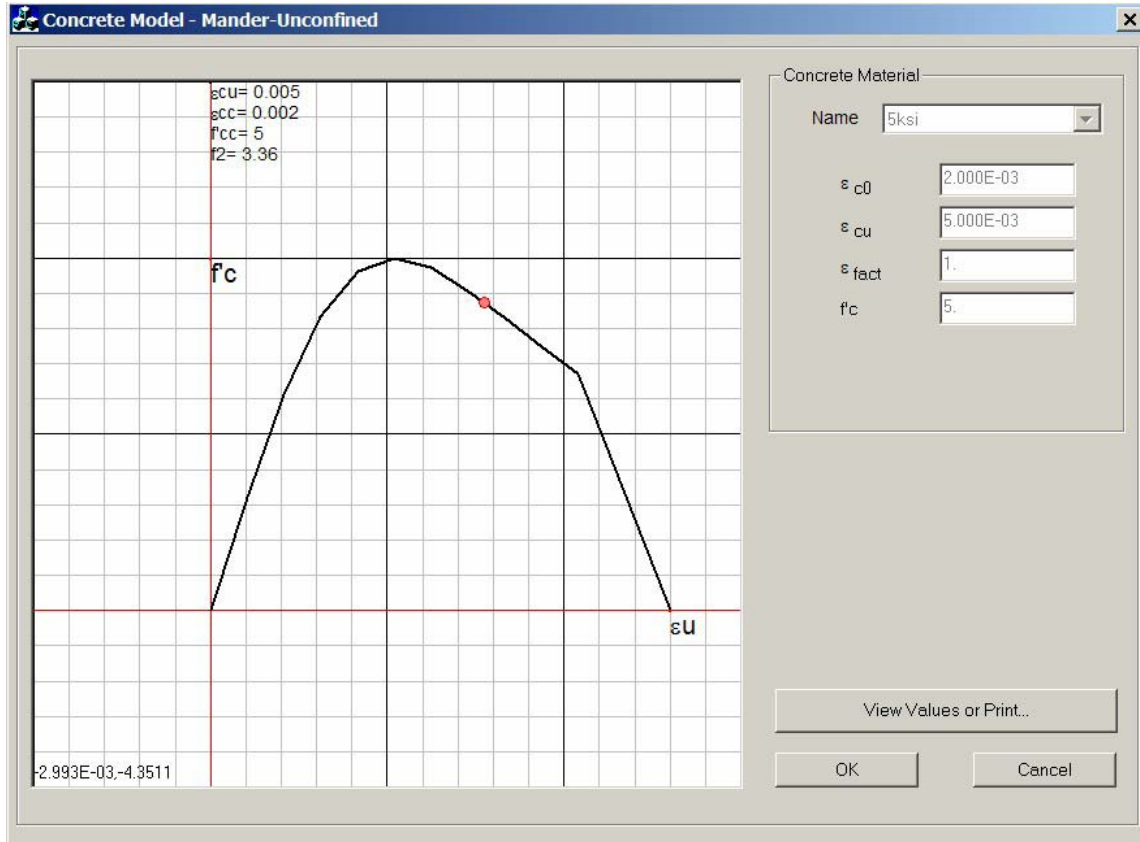
Figure VI.A.1 Unconfined Concrete Stress Strain
