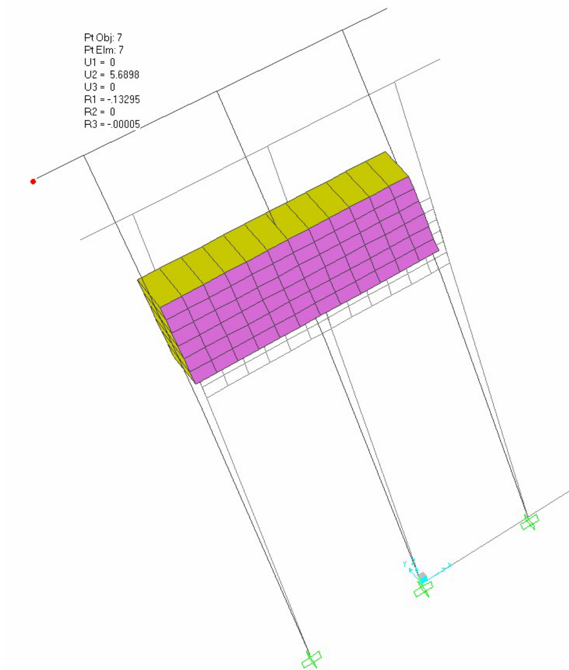
Figure VI.A.16 Response of Model 1 Subjected to 1000 Kips of Longitudinal Loading
