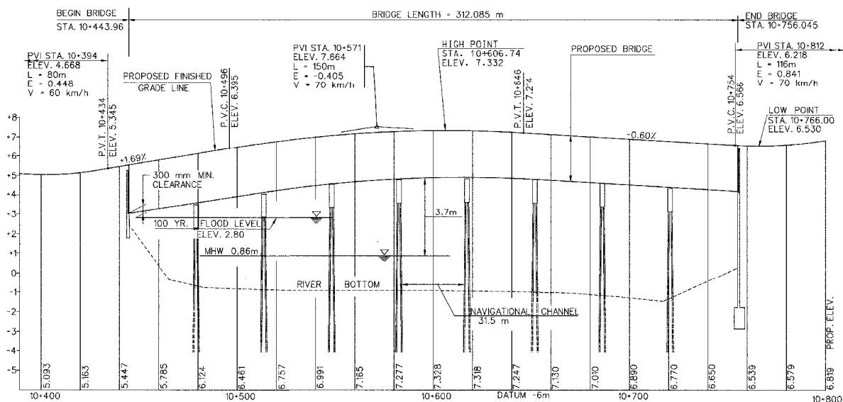
Figure 5.121 River Bottom Profile
