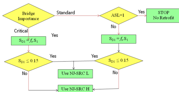
Figure 6.2 Flow Chart for Selection of NJSRC.
