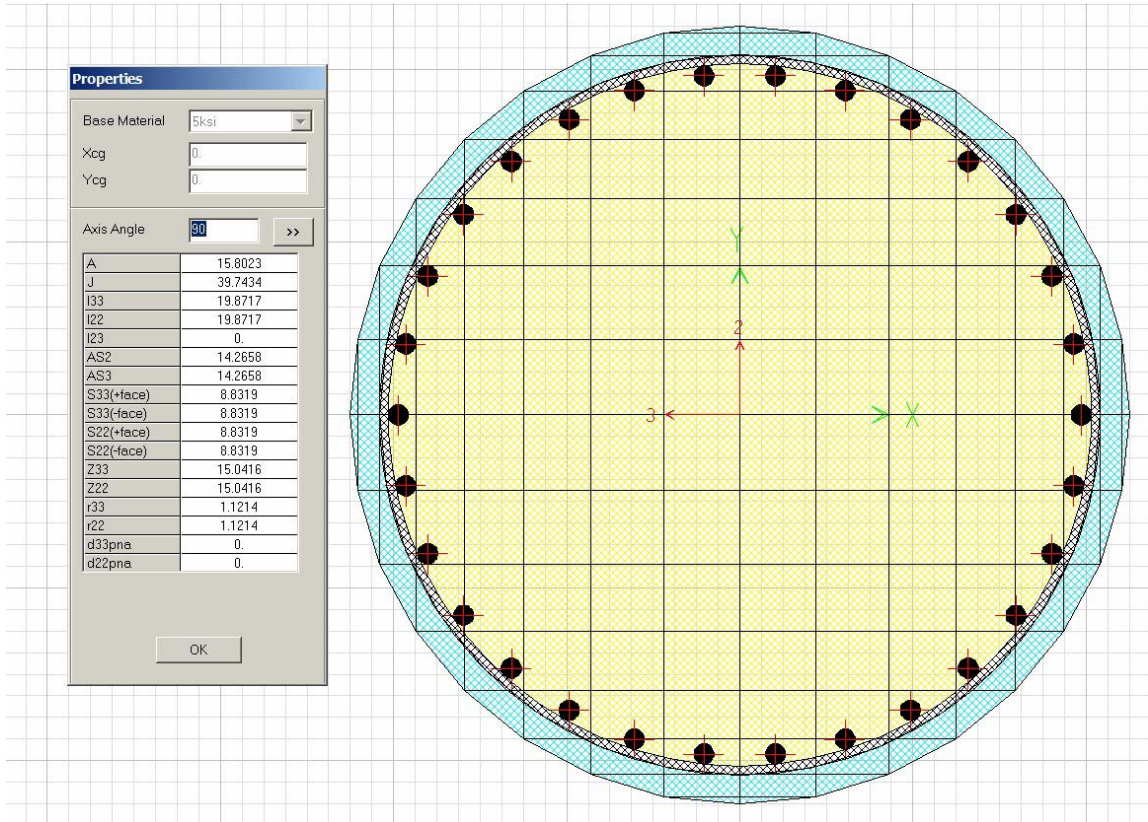
Figure VI.A.25 Column Gross Properties (CS3)
