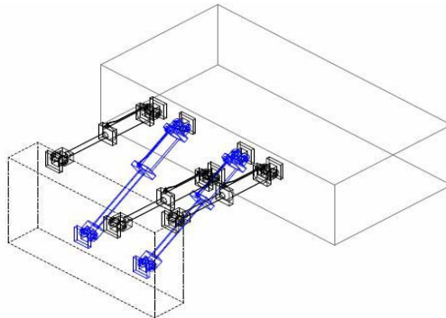
Figure IV.B.1 Actuator Configuration
