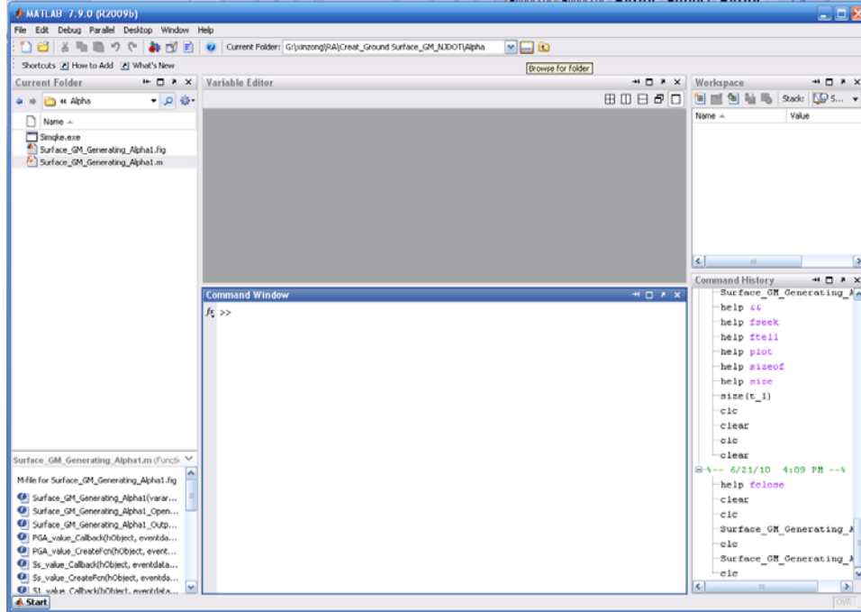
Figure III.44 Launching MATLAB
