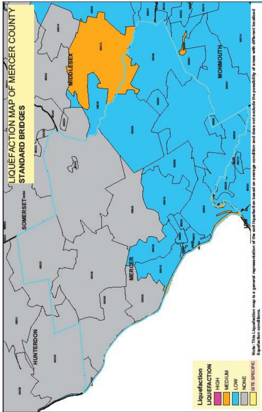
Figure III.12 Liquefaction Map for Standard Bridges in Mercer County of New Jersey
