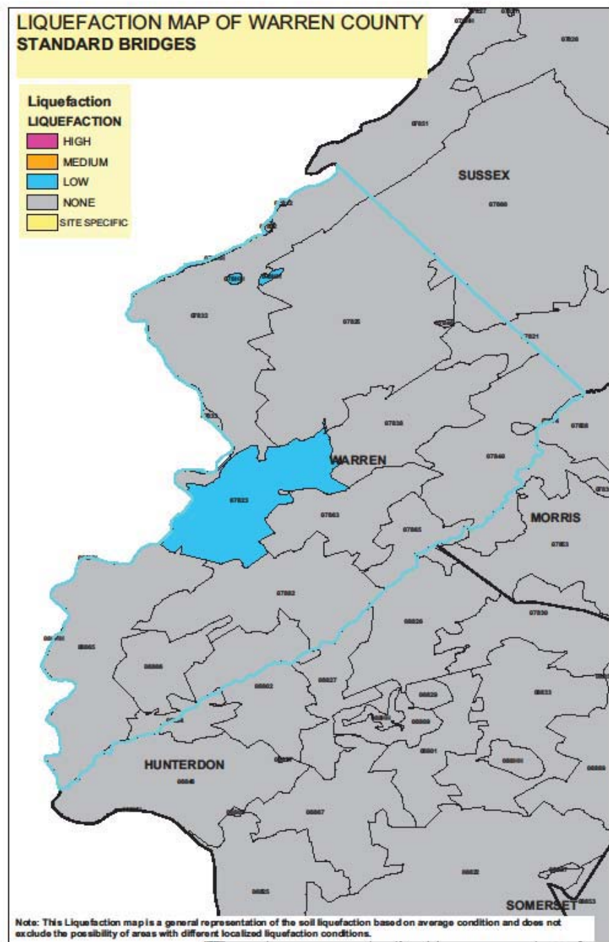
Figure III.22 Liquefaction Map for Standard Bridges in Warren County of New Jersey
