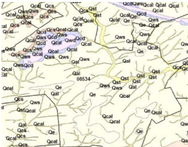
Figure II.4 Soil Condition in Zip Code 08534 in Mercer County
