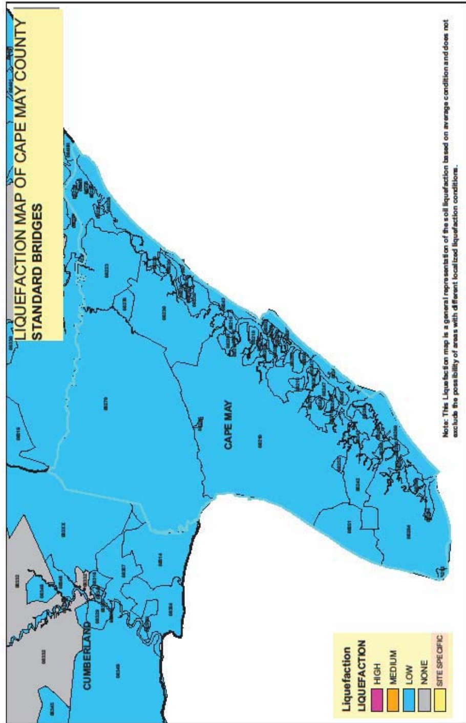
Figure III.6 Liquefaction Map for Standard Bridges in Cape May County of New Jersey
