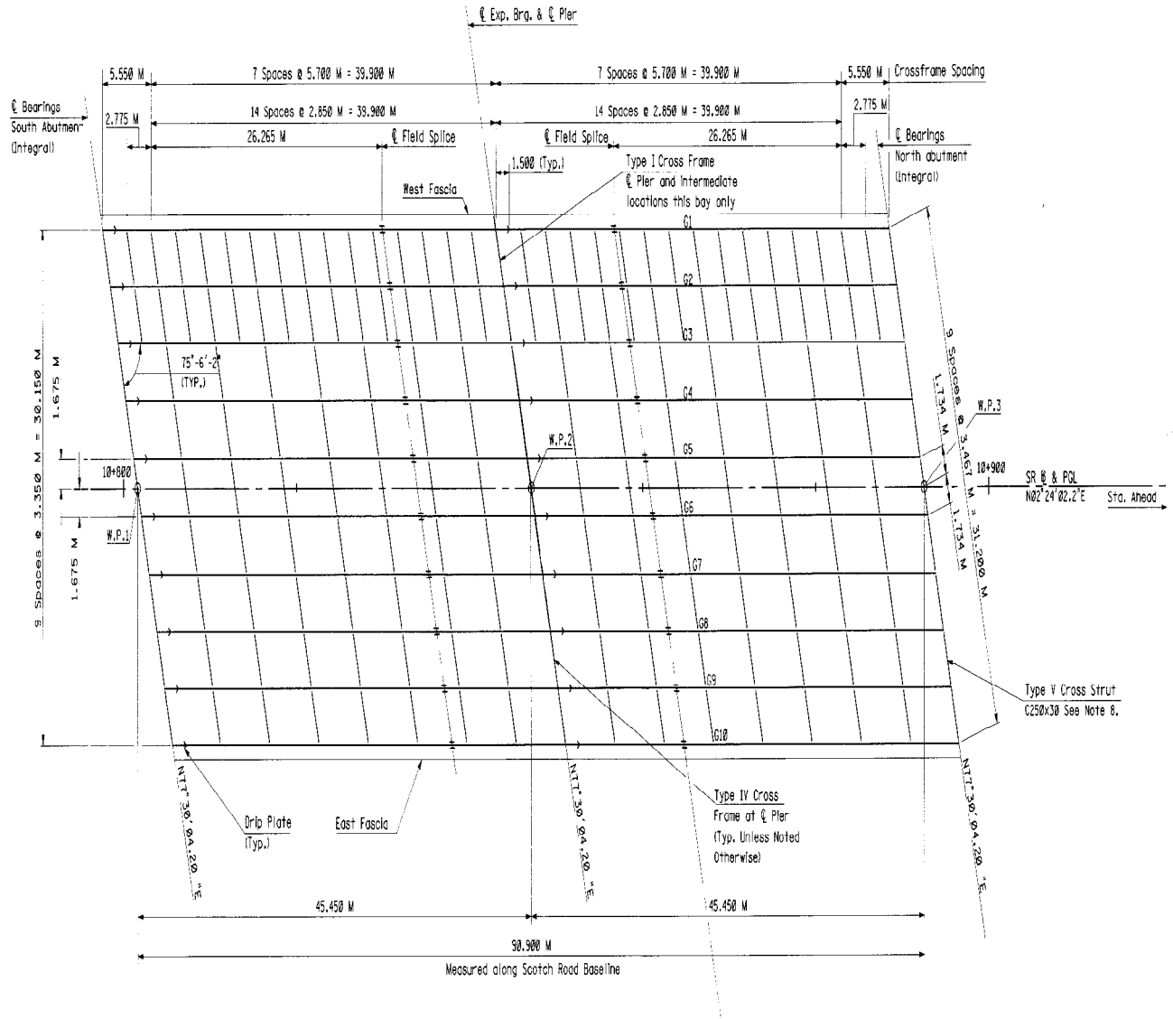
Figure 5.28 Superstructure Framing Plan
