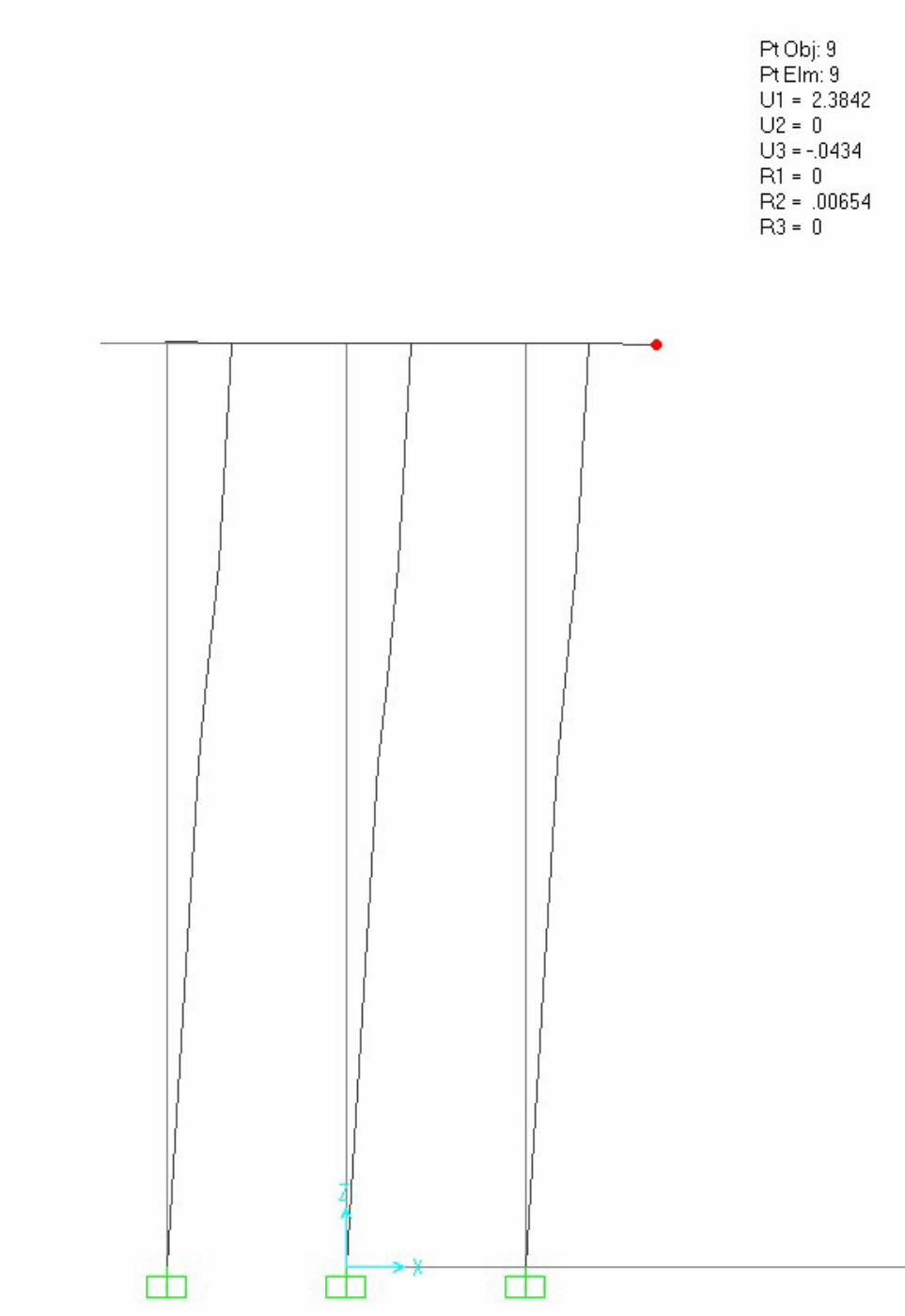
Figure VI.A.37 Response of Model 4 Subjected to 1000 Kips of Transverse Loading
