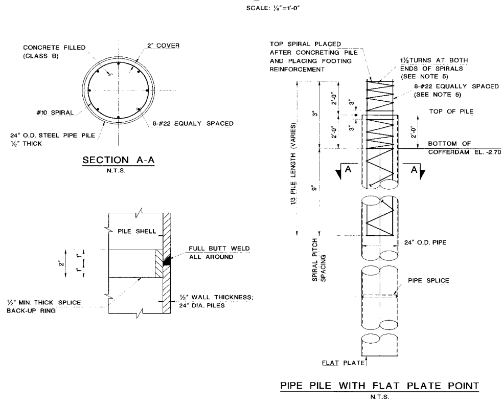
Figure VII.C.2 Pipe Pile Details
