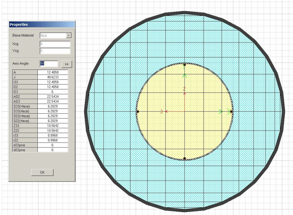
Figure VI.A.21 Shaft Casing Gross Properties (SC2)
