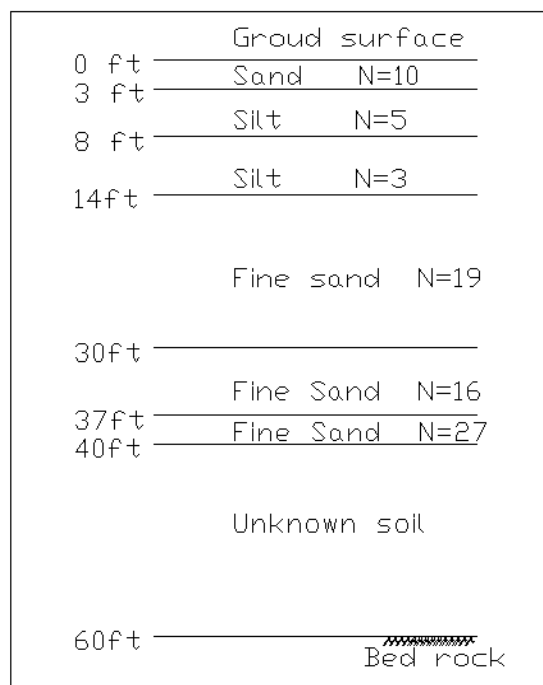
Figure II.1 Illustration of a soil profile (not to scale)
