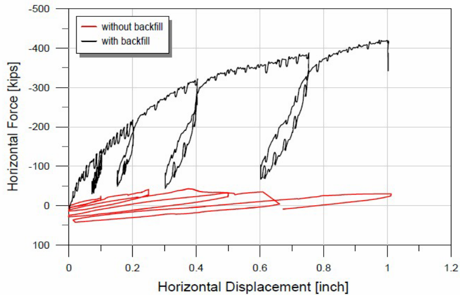
Figure IV.B.6 Load-deflection curves up to max displacement of 1.0 in with and without backfill
