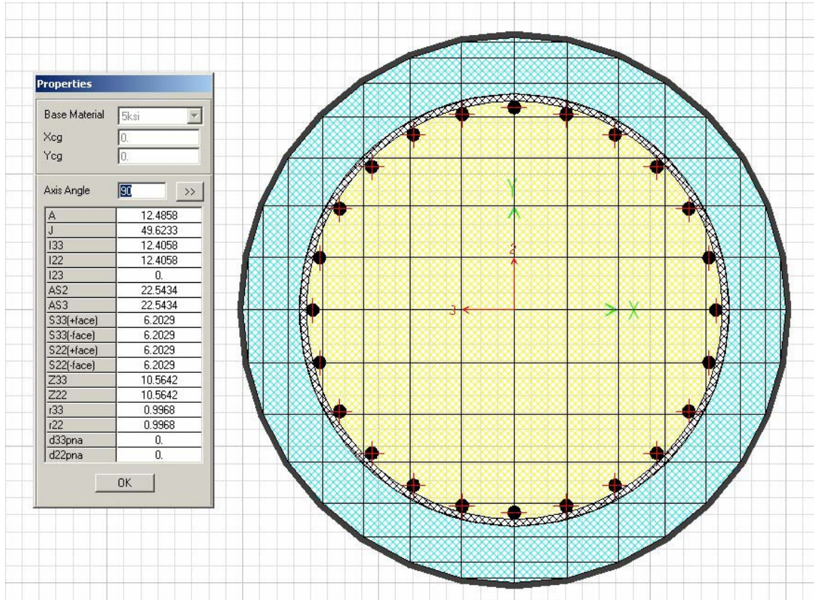
Figure VI.A.7 Column Casing Gross Properties (CSE1)
