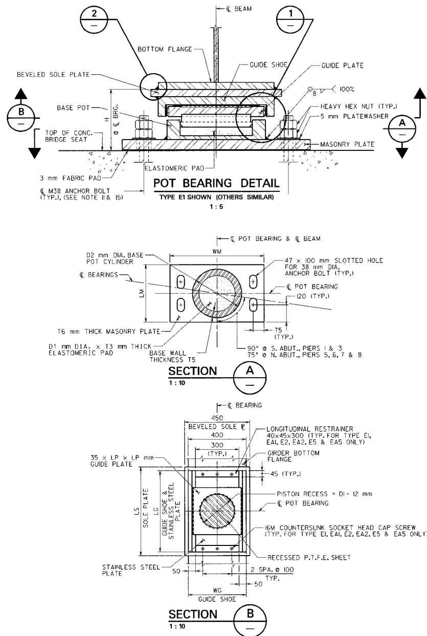
Figure VI.B.1 Expansion Pot Bearing Details
