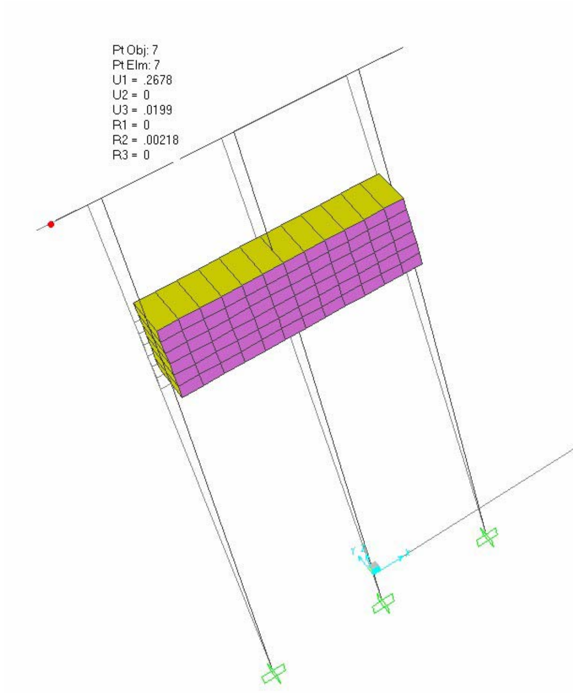
Figure VI.A.31 Response of Model 3 Subjected to 1000 Kips of Transverse Loading
