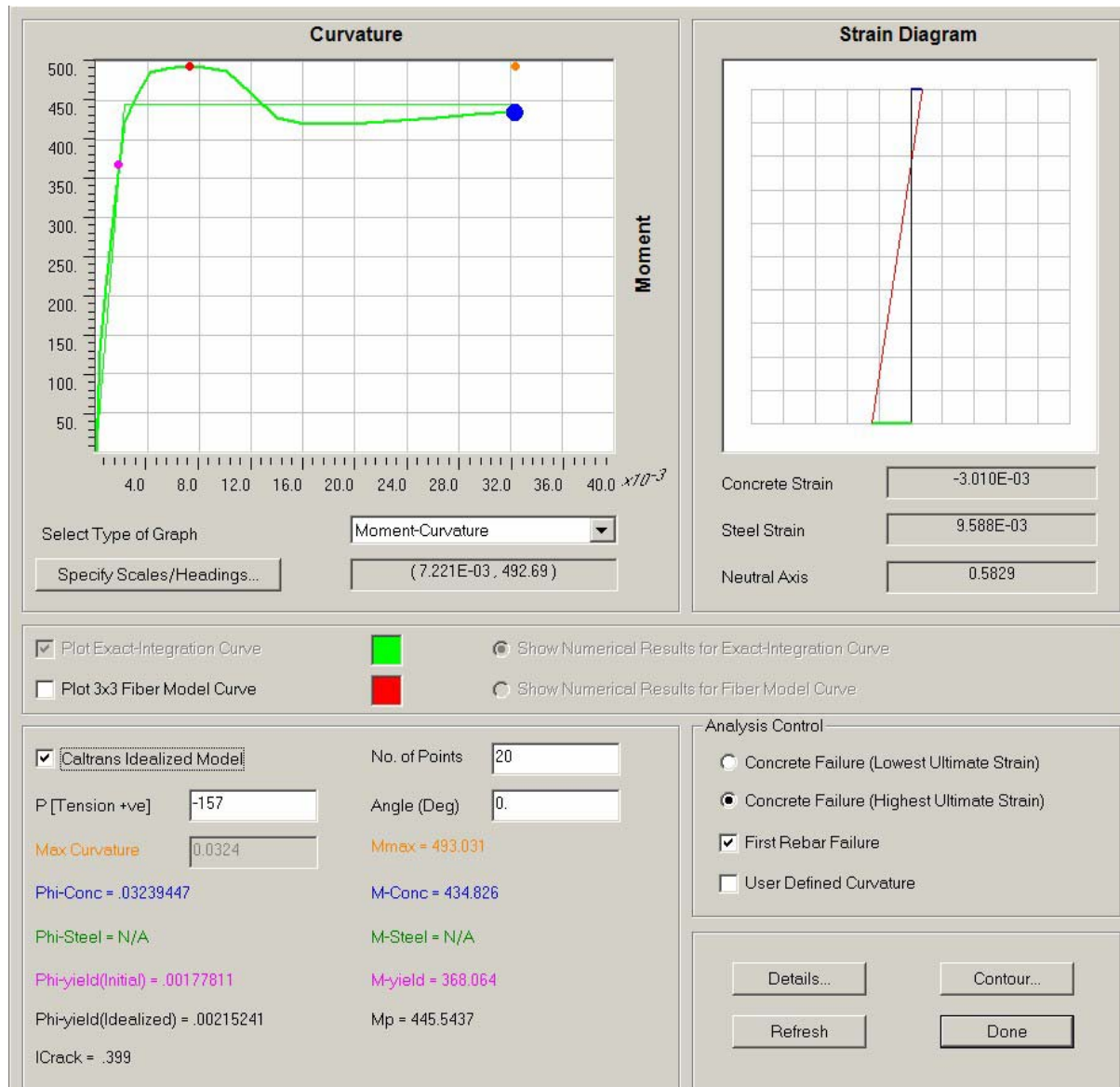
Figure VIII.A.5 Moment Curvature Analysis (PT)
