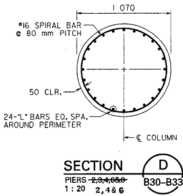
Figure VI.C.14 Column Section Pier 2, 4, and 6
