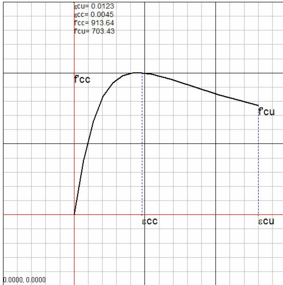
Figure VIII.A.3 Confined Concrete Stress Strain Model Section (PB)
