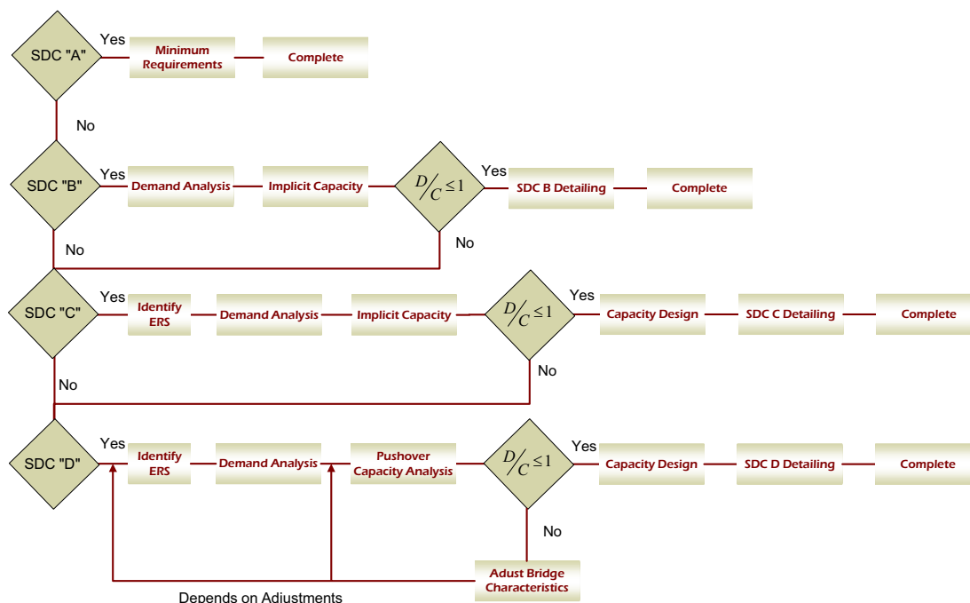
Figure 5.55 Seismic Design Category (SDC) Core Flowchart
