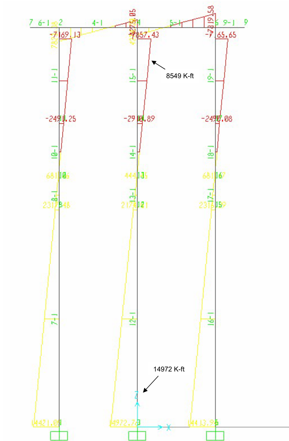
Figure VI.A.38 Model 4 Moment Distribution for Bent Subject to 1000 Kips of Transverse Loading
