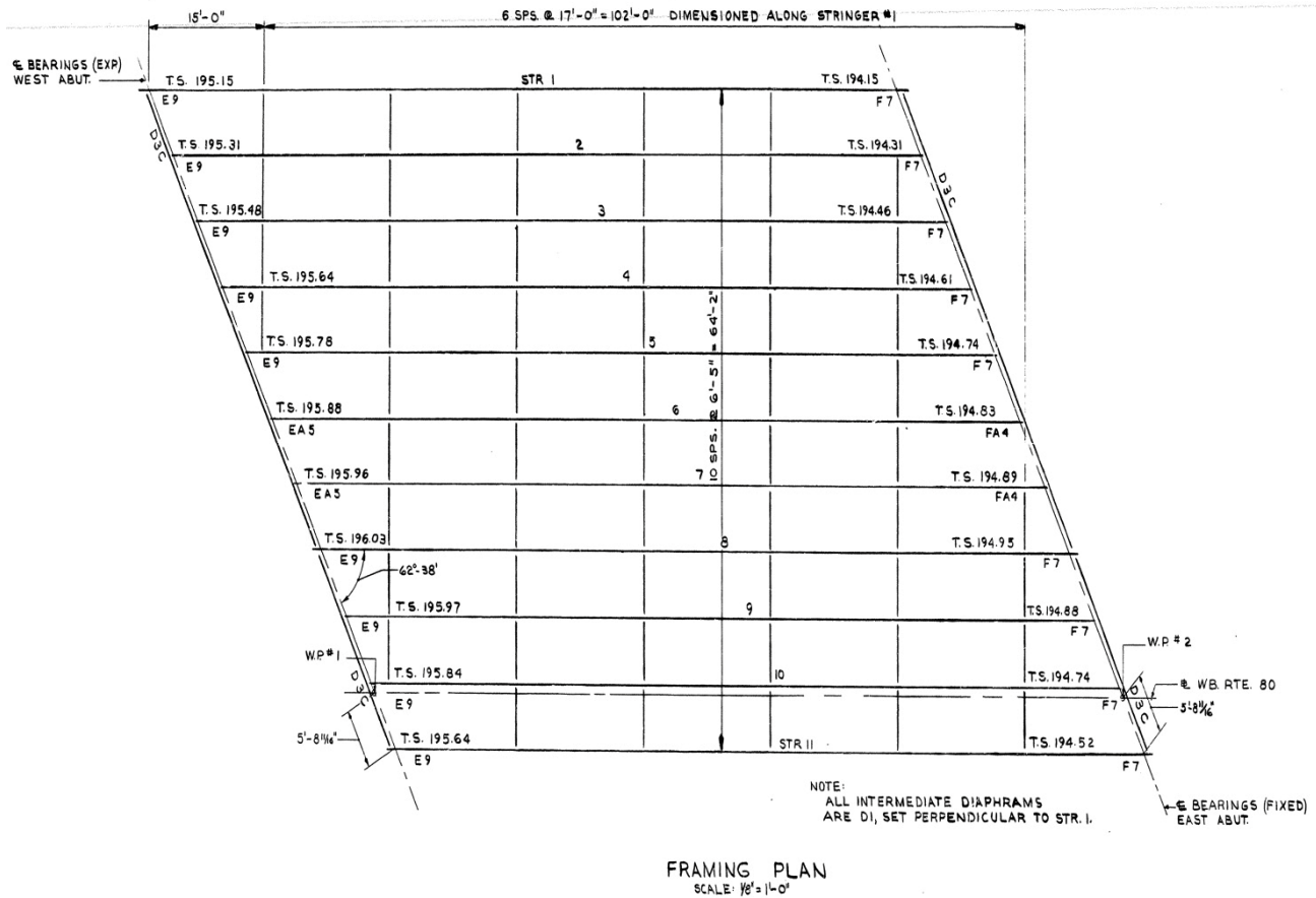
Figure 5.15 Framing Plan
