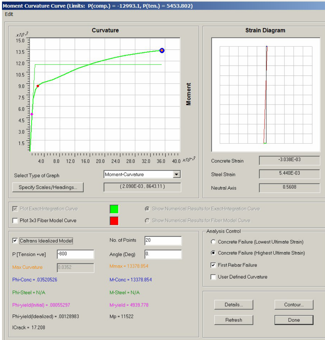
Figure VI.A.20 Moment Curvature Analysis (CSE2)
