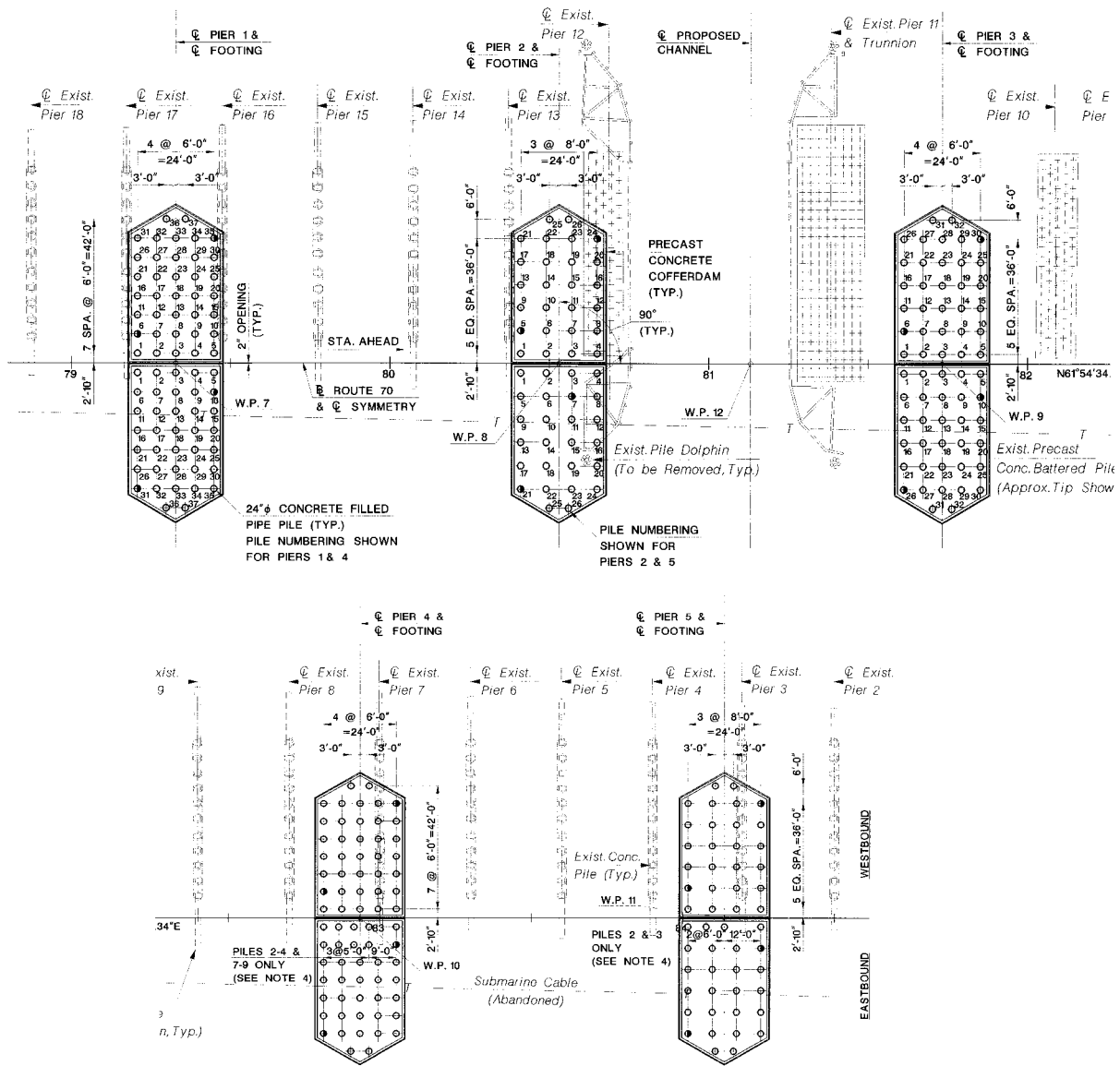
Figure VII.C.22 Footing Layout for Piers 1,2,3,4,5
