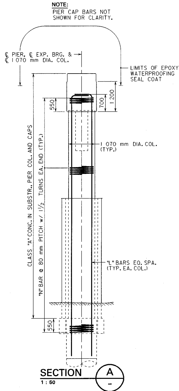
Figure VI.C.9 Section Pier 5, 7, and 8
