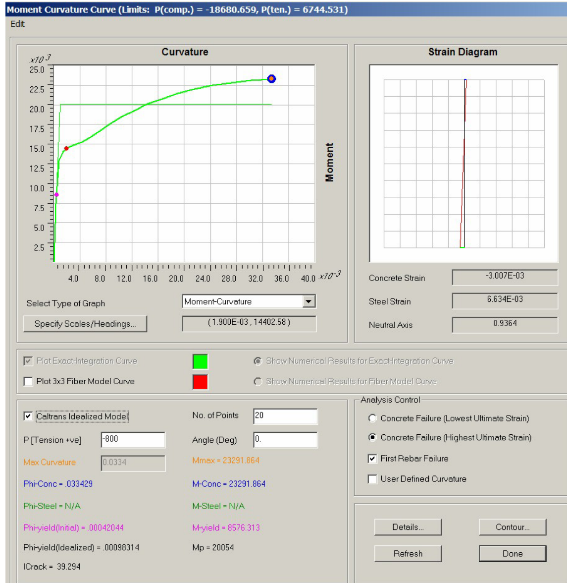
Figure VI.A.30 Moment Curvature Analysis (SC3)
