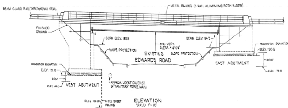
Figure 5.14 Elevation
