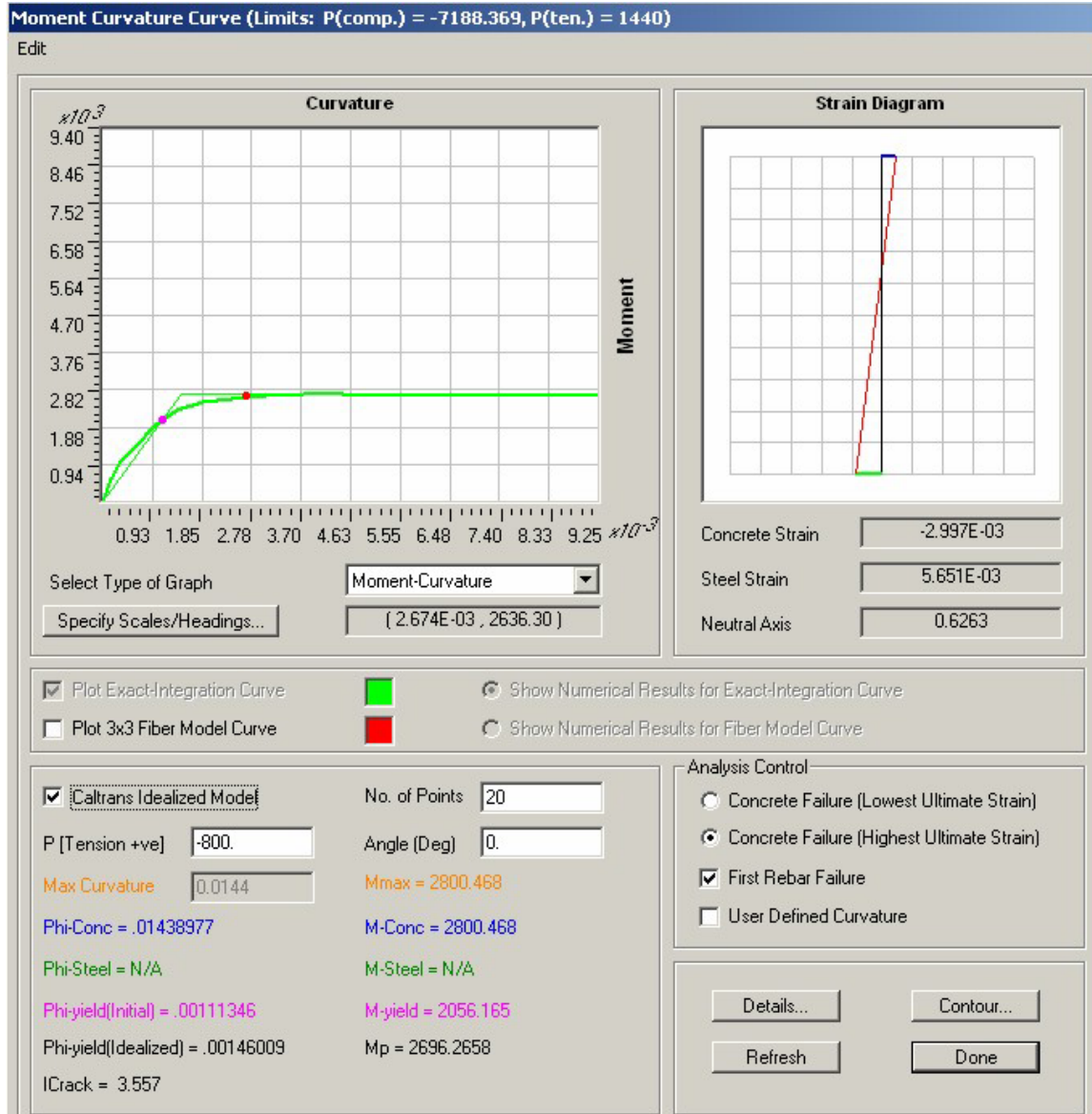
Figure VI.A.6 Moment Curvature Analysis (CS1)
