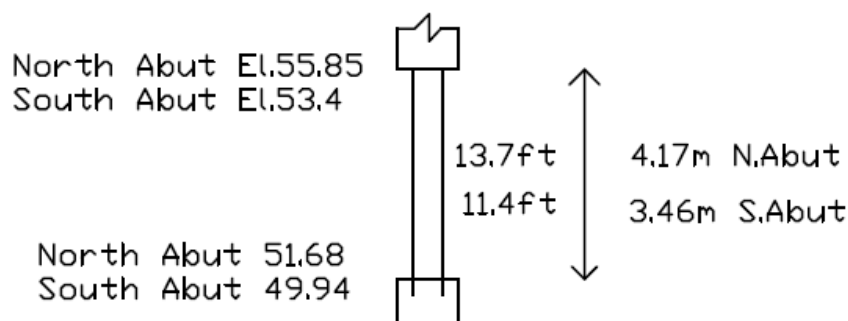
Figure 5.42 Effective Pile Length at Abutments.
