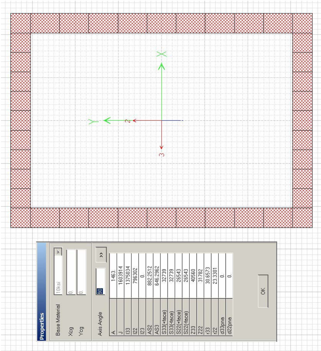
Figure VII.A.36 Bent Cap Section A-A Hollow Core
