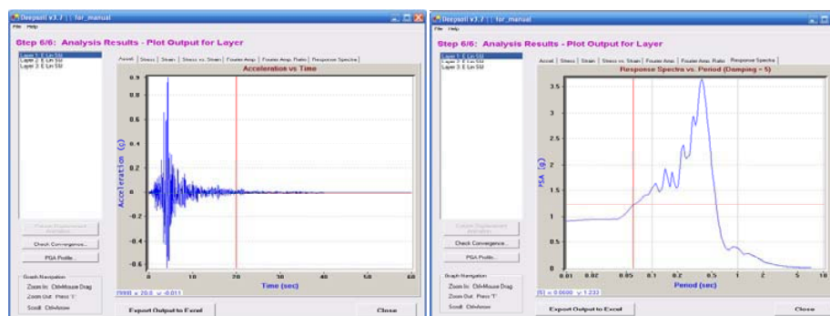
Figure III.70 Computed Surface Acceleration and Response Spectra
