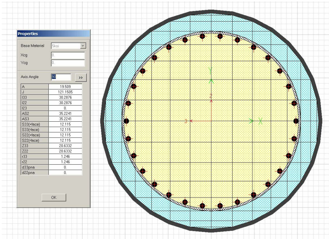
Figure VI.A.27 Column Casing Gross Properties (CSE3)
