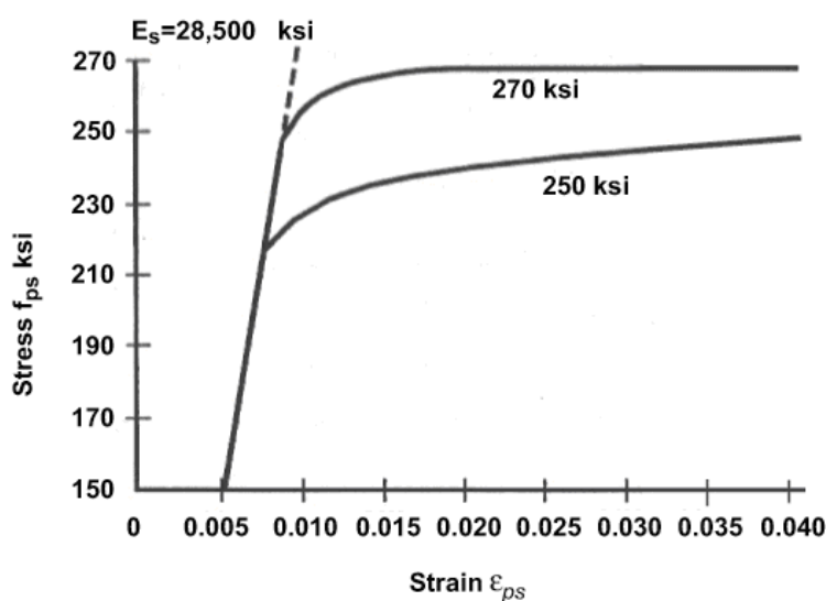
Figure VII.A.2 Prestressing Strand Stress-Strain Model.
