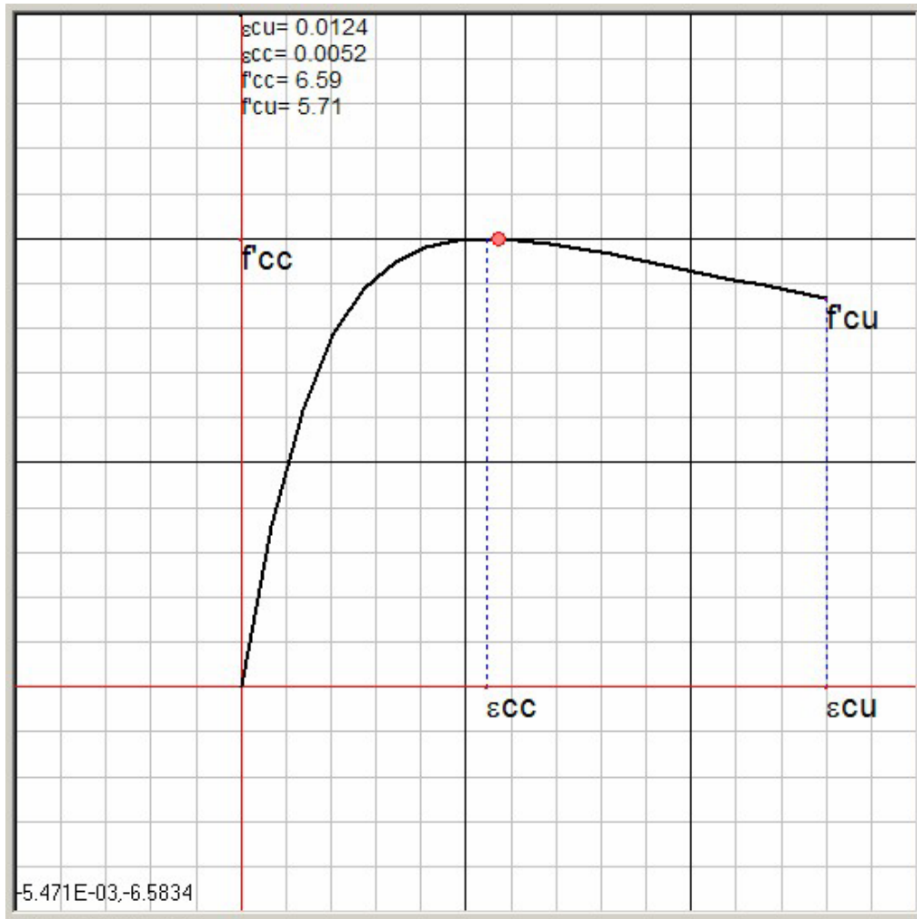
Figure VI.A.2 Confined Concrete Stress Strain Model
