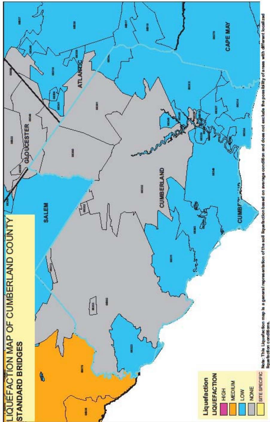
Figure III.7 Liquefaction Map for Standard Bridges in Cumberland County of New Jersey
