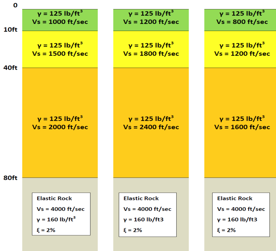
Figure III.59 Soil profiles for the example
