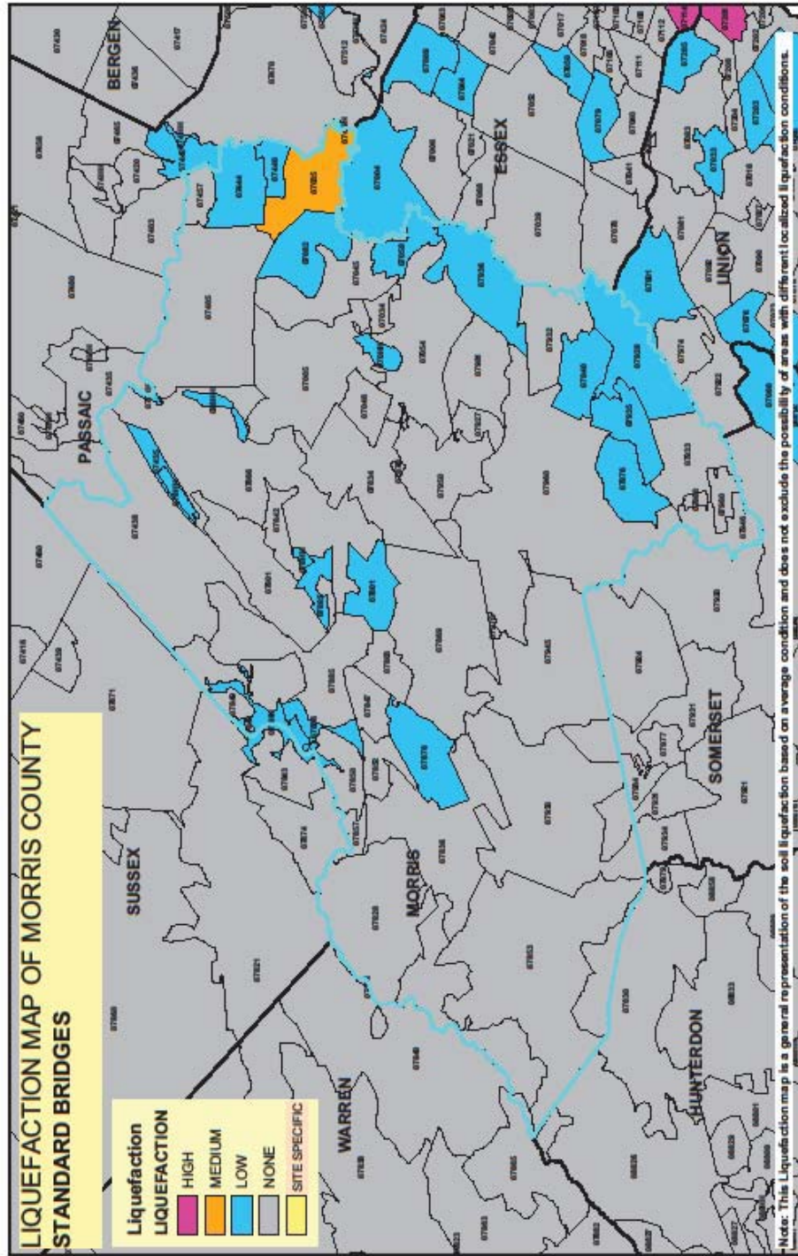
Figure III.15 Liquefaction Map for Standard Bridges in Morris County of New Jersey
