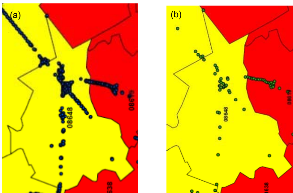
Figure II.2 (a) Available and (b) Selected Borehole Data for analysis in zip code 08648
