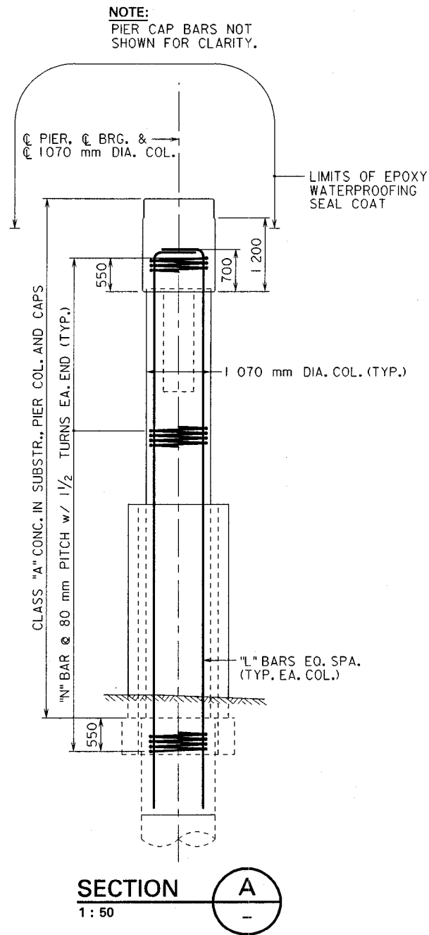
Figure VI.C.5 Section Pier 1, 2, and 4
