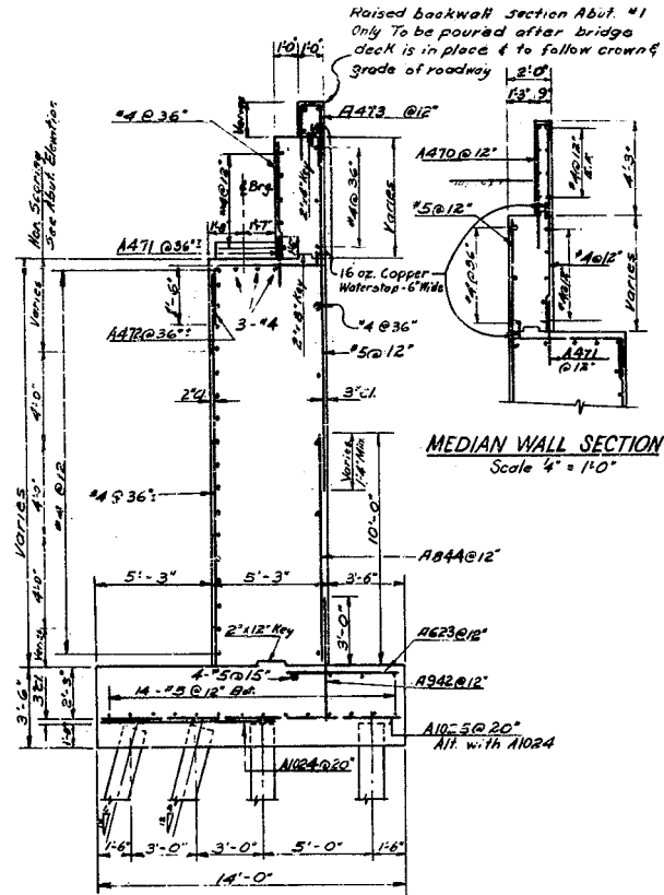
Figure 5.89 Abutment Typical Section
