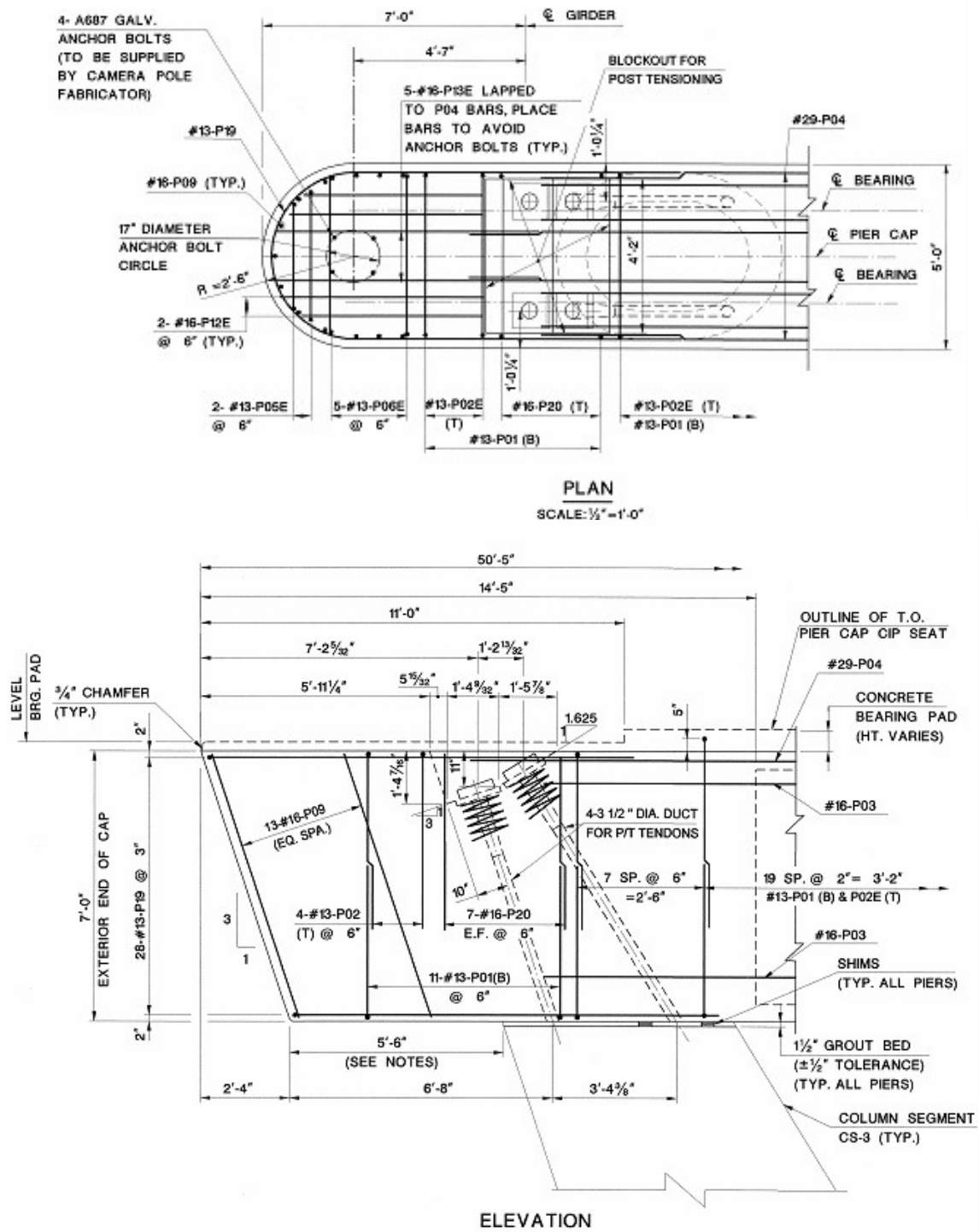
Figure VII.C.16 Pier 3 EB Cap End Details
