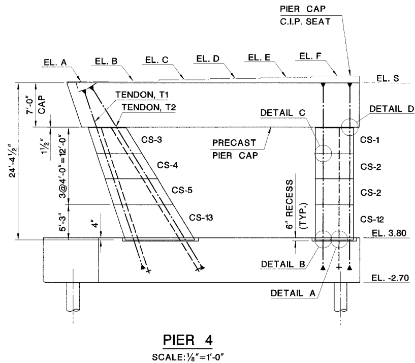
Figure VII.C.4 Piers 3 and 4 Precast Segment Elevation
