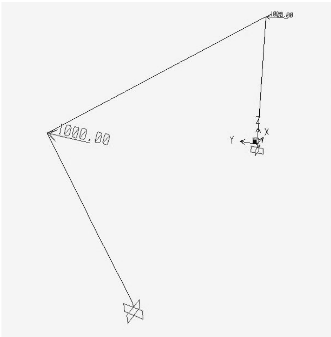
Figure VII.A.46 Pier 3 Longitudinal Loading
