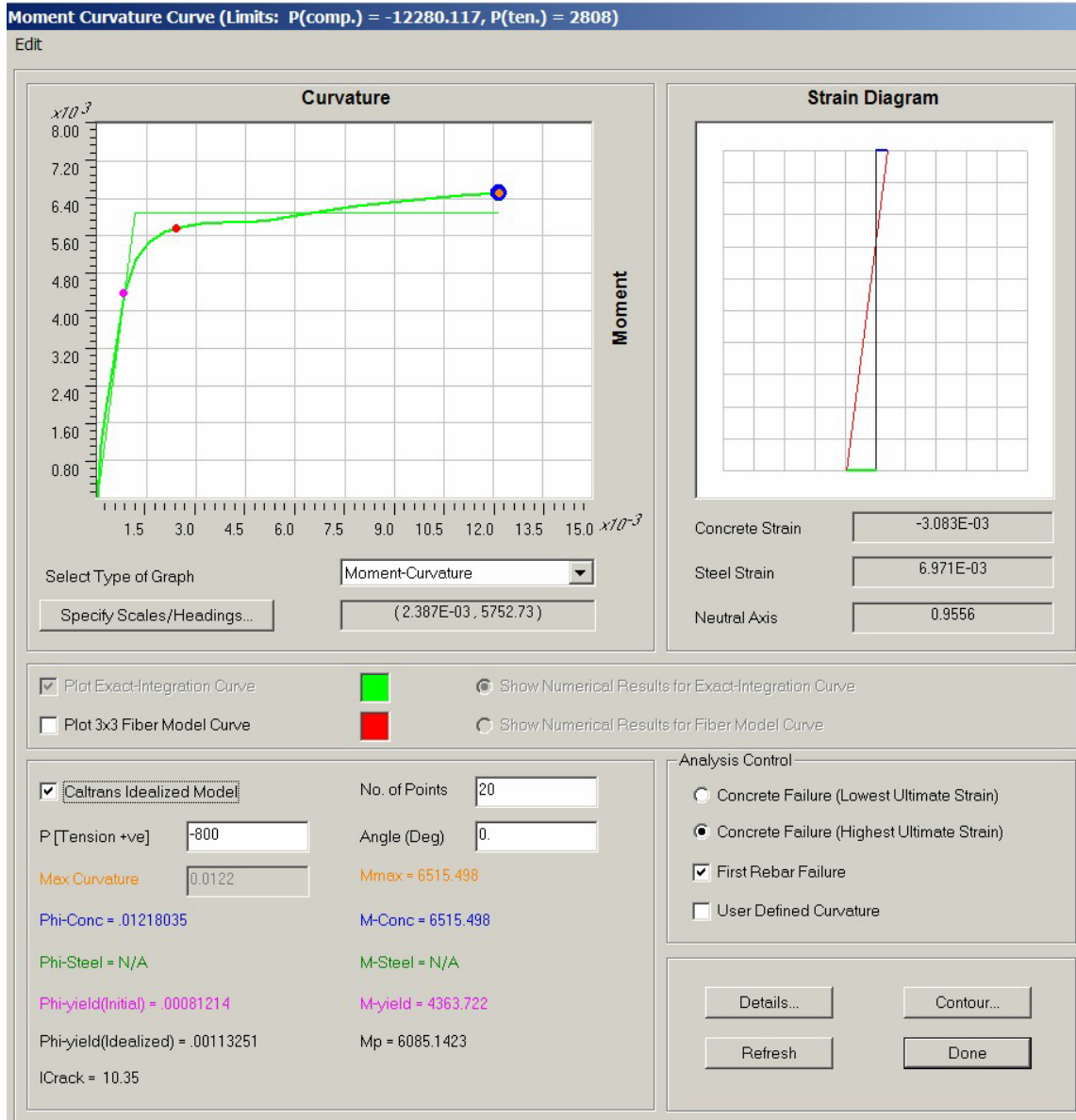
Figure VI.A.26 Moment Curvature Analysis (CS3)
