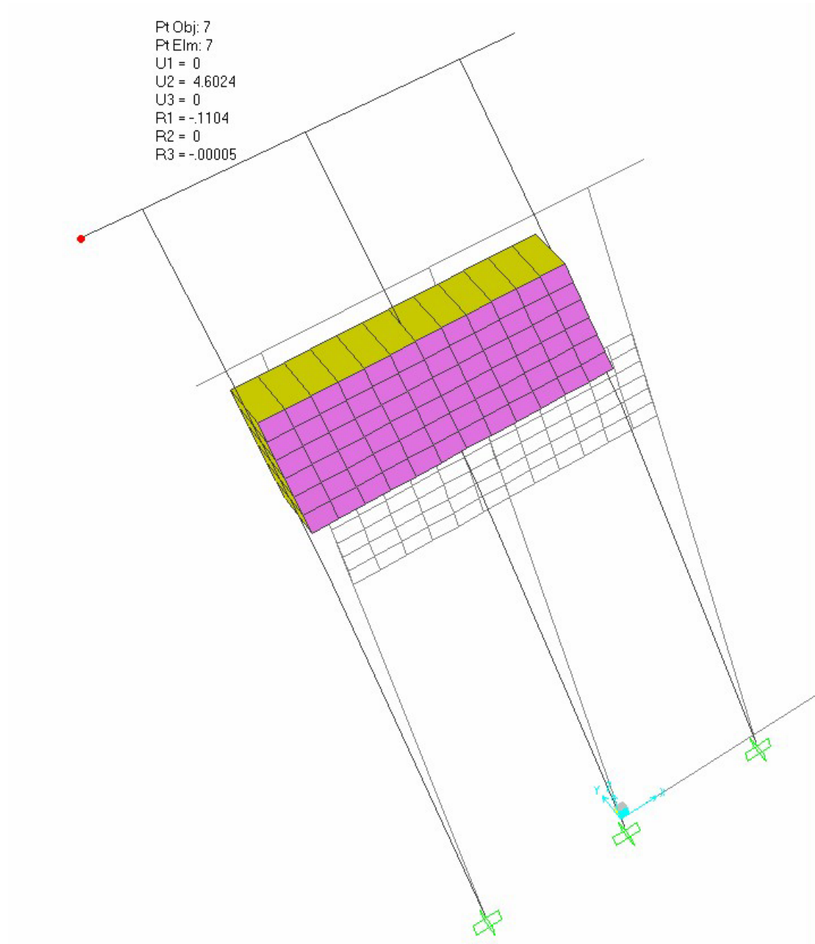
Figure VI.A.24 Response of Model 2 subjected to 1000 Kips of Longitudinal Loading
