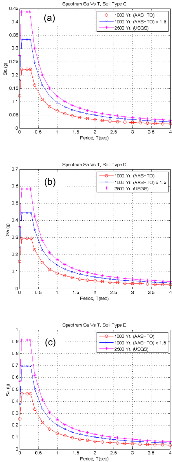
Figure 1.5 Comparison Between 1000 Yr (AASHTO-SGS), 1000 Yr. (AASHTO-SGS) \times 1.5 and 2500 Yr. (USGS for NJ) Spectra for Soil Sites C, D and E.
