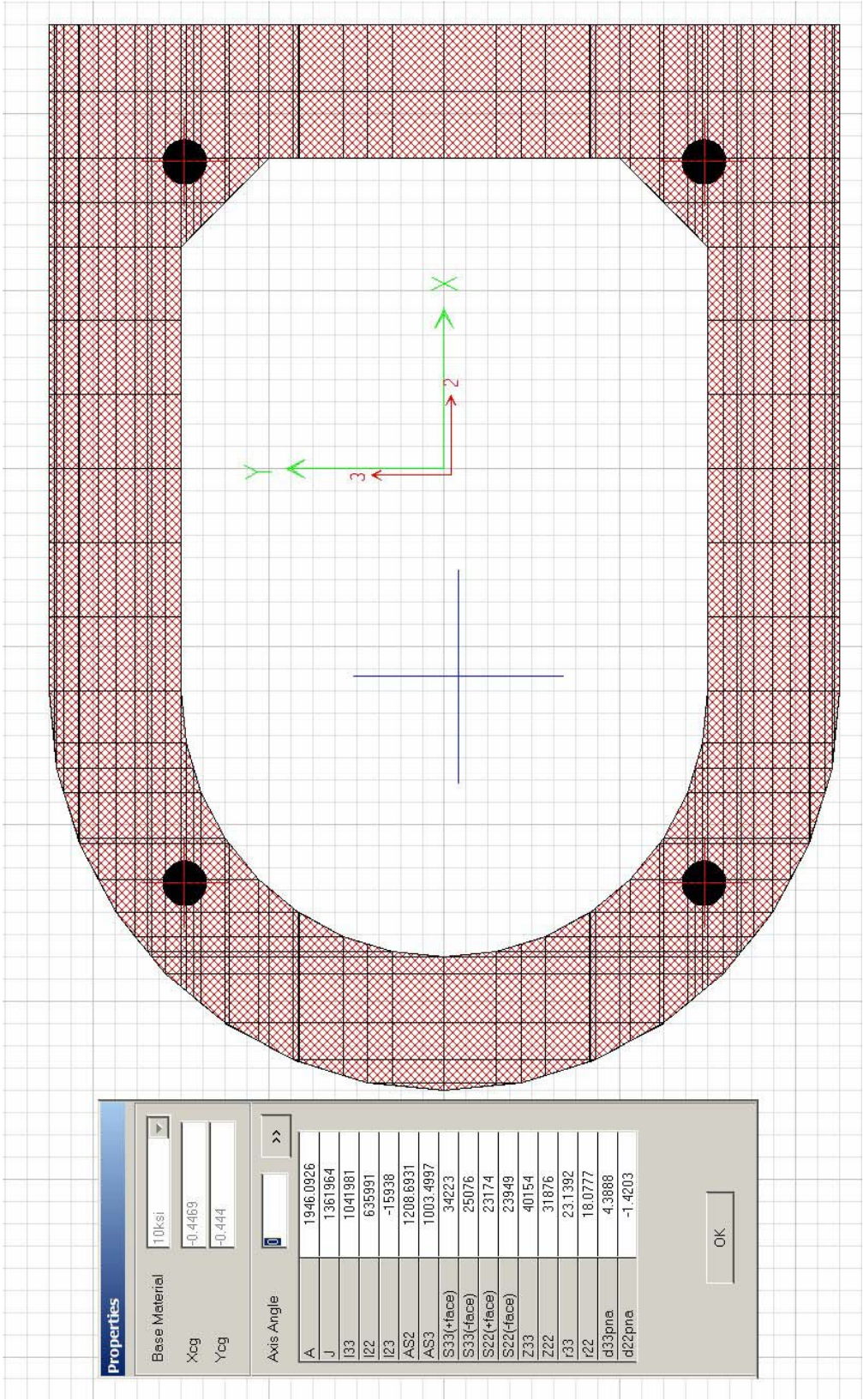
Figure VII.A.4 CS1-PS CSI-SAP Properties
