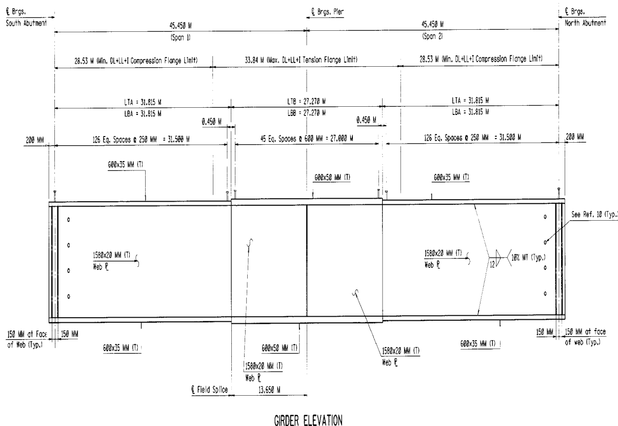
Figure 5.29 Girder Elevation
