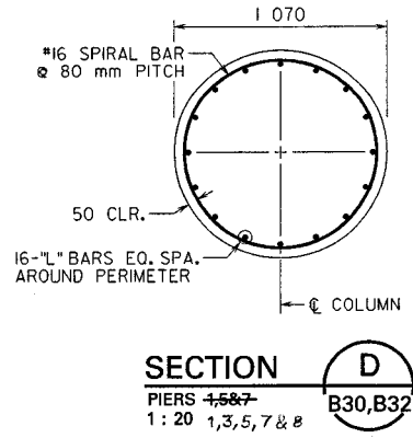
Figure VI.C.13 Column Section Pier 1, 3, 5, 7, and 8
