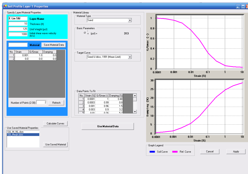
Figure III.64 Soil curves
