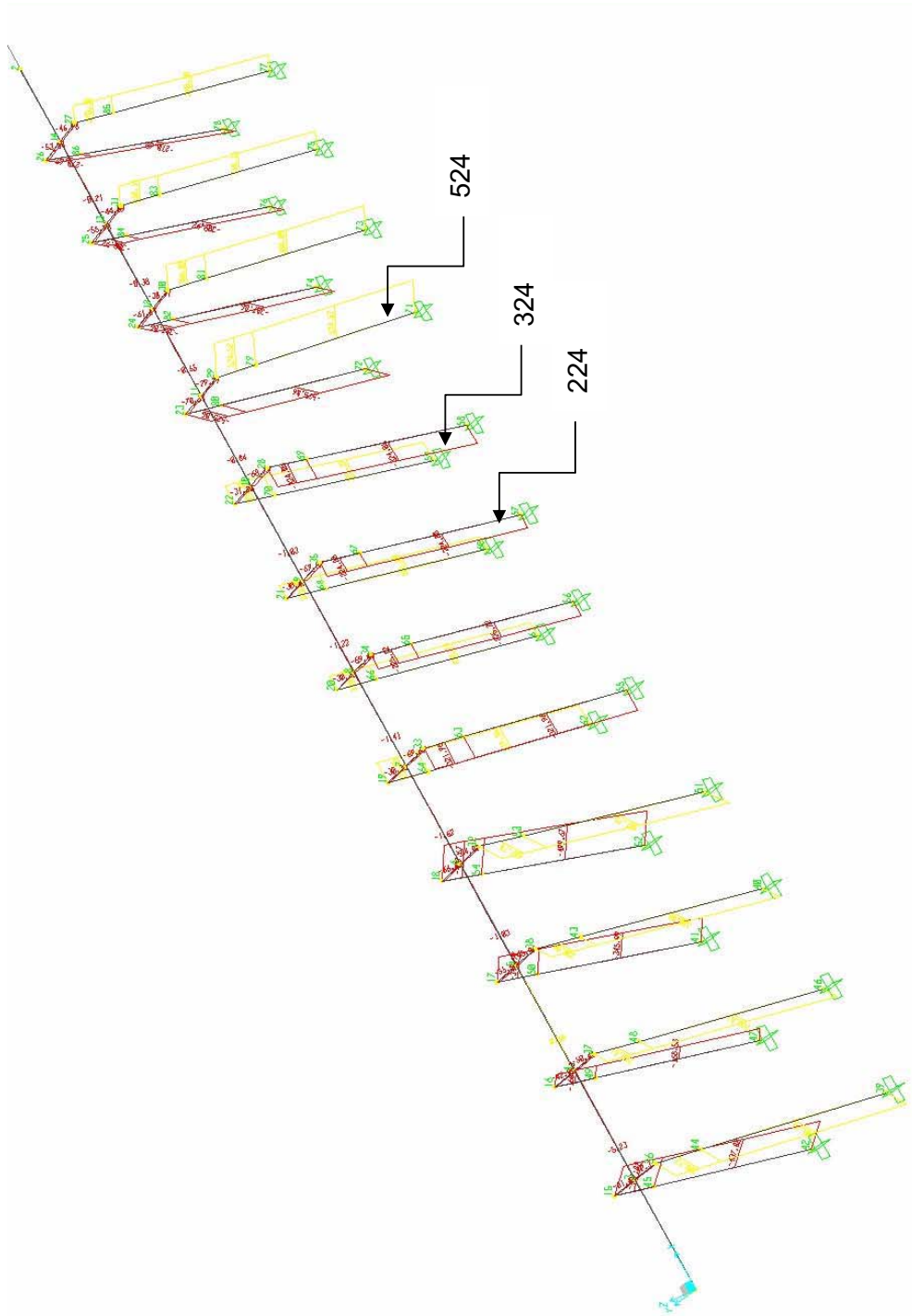
Figure VIII.A.15 Axial Force Demand Subject to 1200 Kips of Longitudinal Loading
