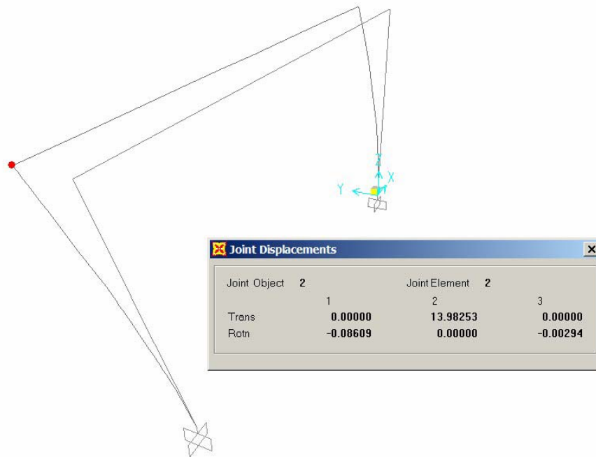
Figure VII.A.47 Pier 3 Outer Column Longitudinal Displacement
