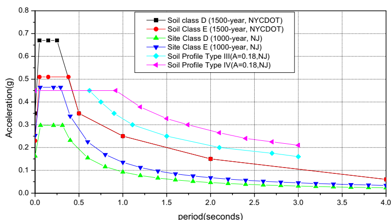
Figure 1.2 Div. 1-A, 1500 Yr. NYCDOT (2008) and 1000 Yr. AASHTO-SGS Spectra.
