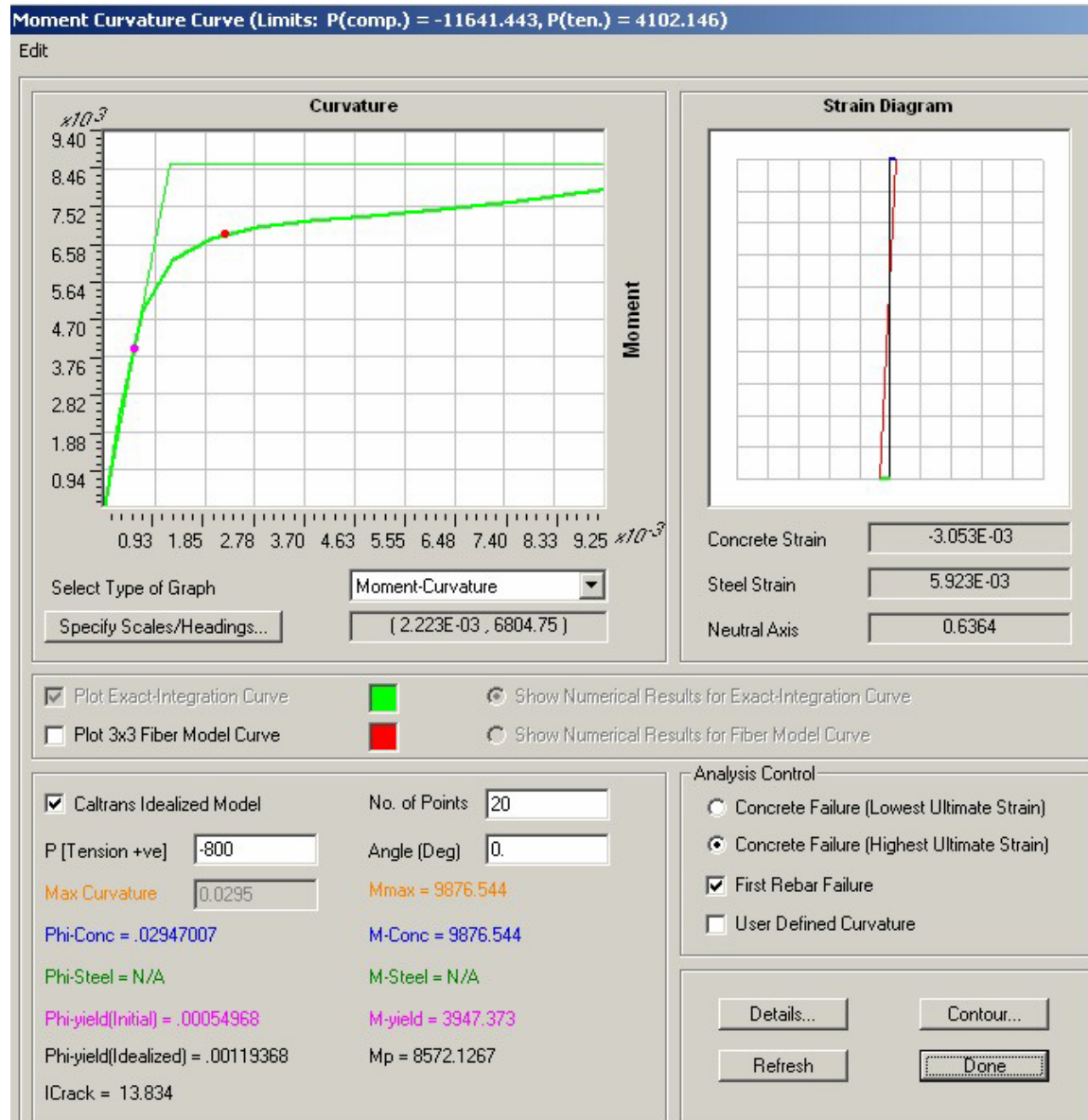
Figure VI.A.8 Moment Curvature Analysis (CSE1)
