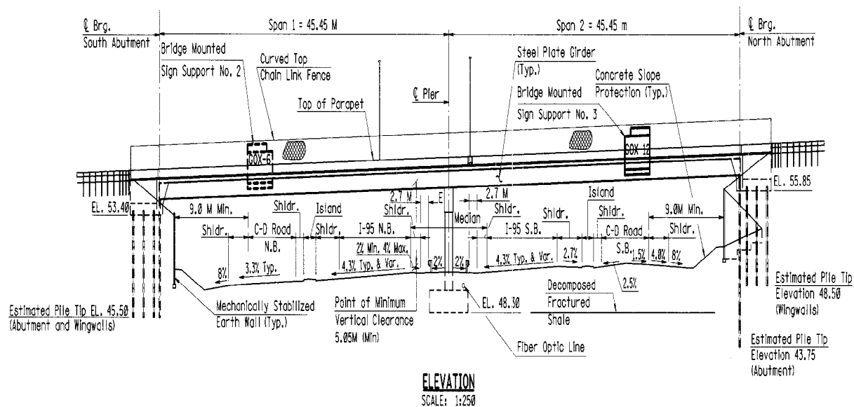
Figure 5.26 Elevation
