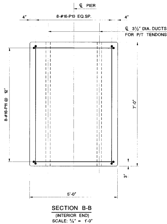
Figure VII.C.15 Bent Cap Section A-A and B-B
