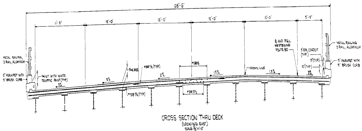
Figure 5.16 Part Section thru Deck
