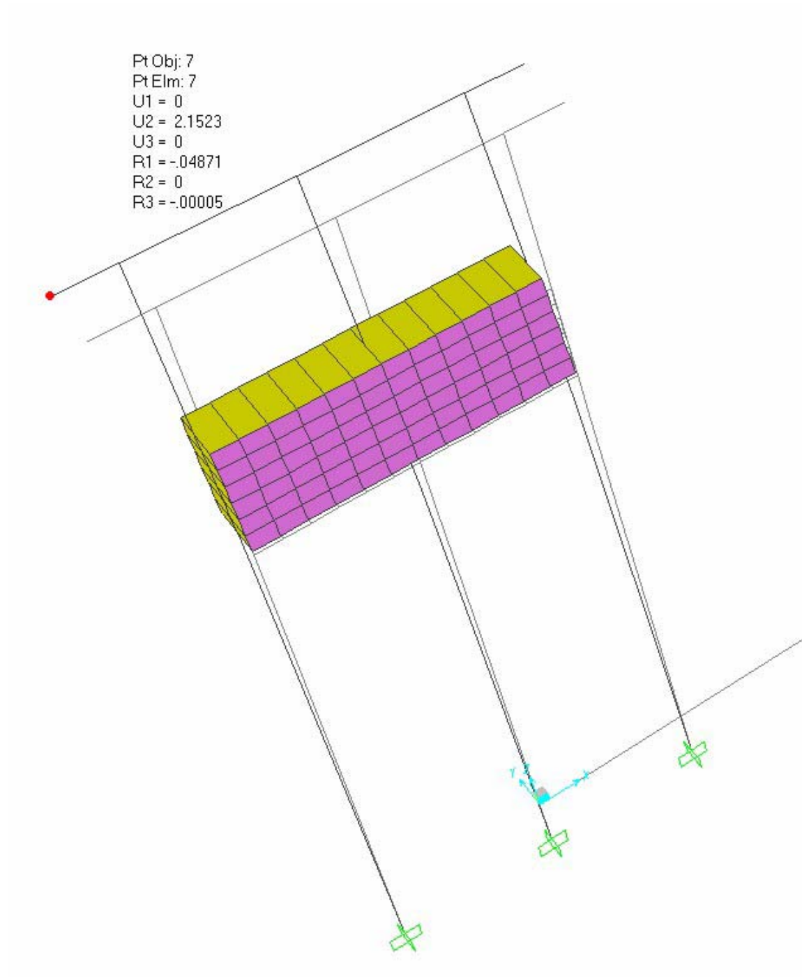
Figure VI.A.32 Response of Model 3 Subjected to 1000 Kips of Longitudinal Loading
