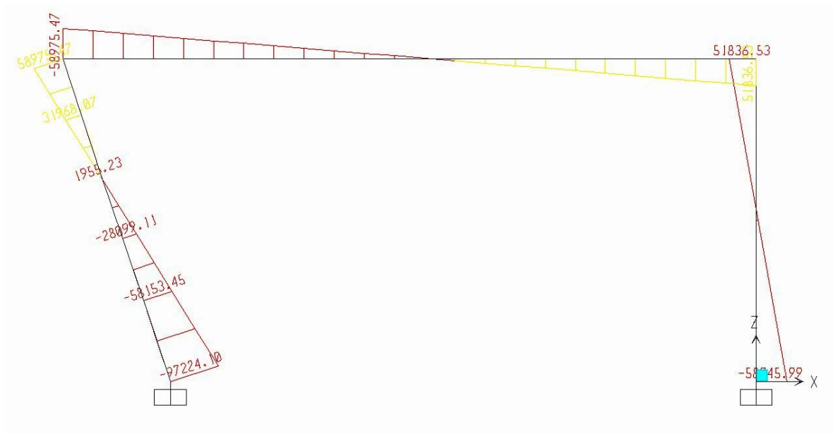
Figure VII.A.58 Pier 3 Transverse Members Moment Lateral 2
