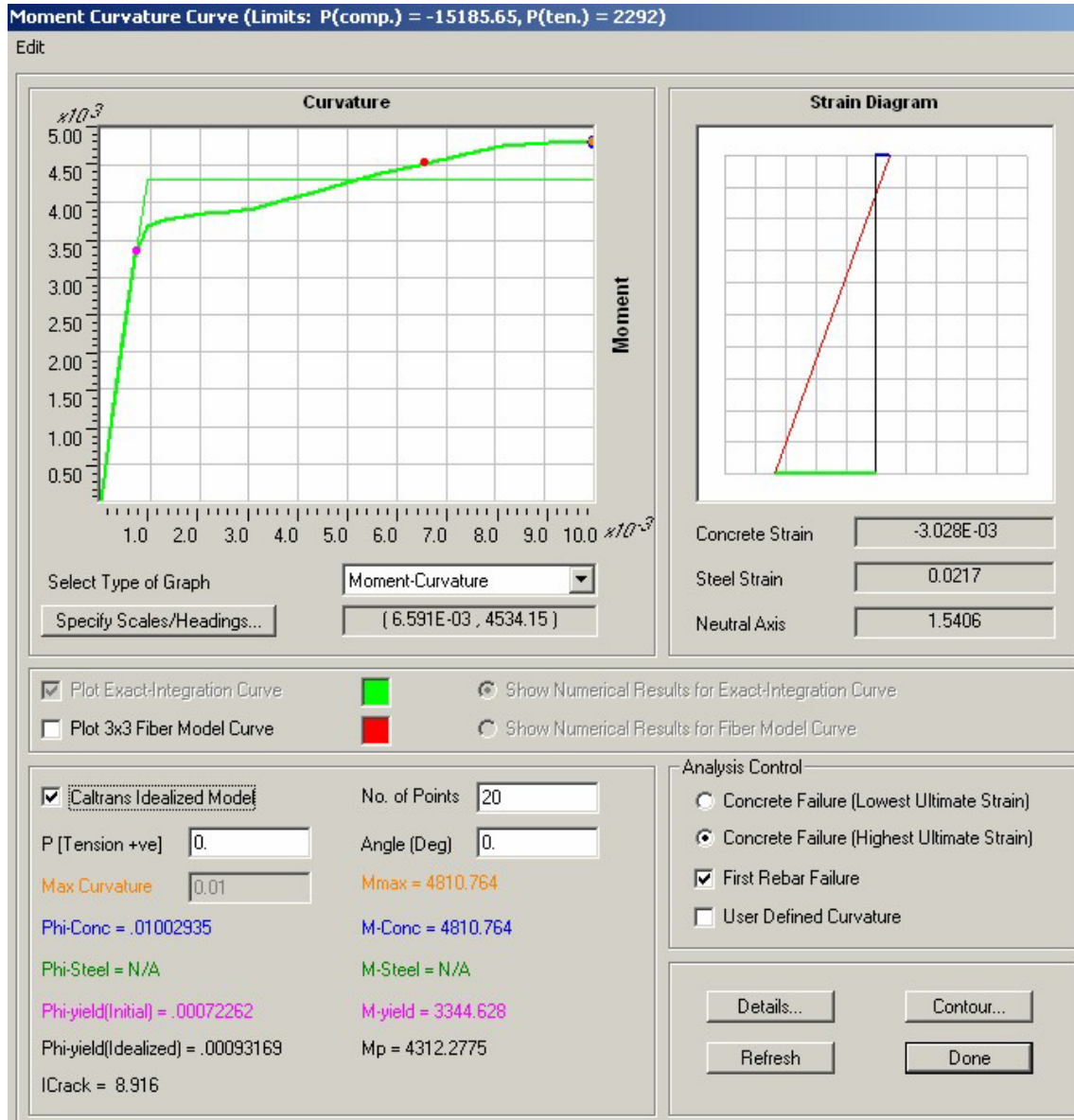
Figure VI.A.12 Bent Cap Movement Curvature Analysis
