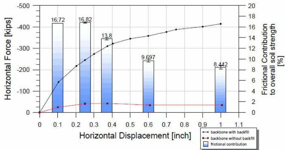
Figure IV.B. 7 Backbone curves and contribution of base friction up to 1.0 inch displacement
