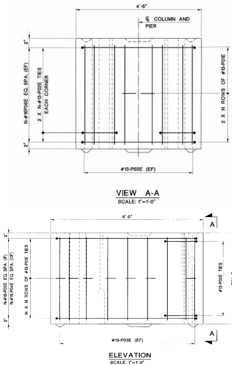
Figure VII.C.10 Inner Column Elevation and View
