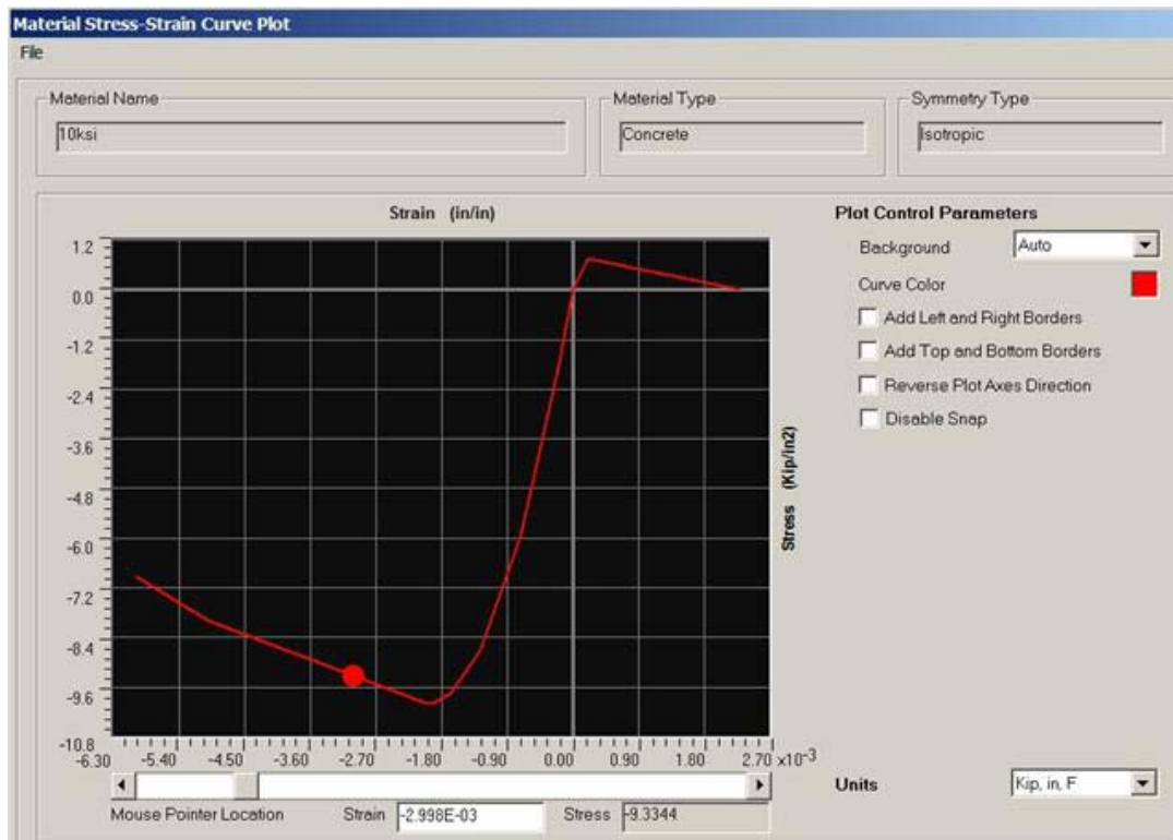
Figure VII.A.3 Concrete Stress-Strain Model
