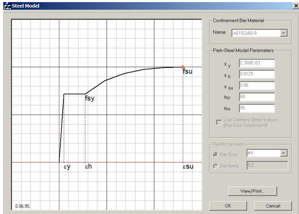
FIGURE V.4 LONGITUDINAL REINFORCEMENT STRESS-STRAIN MODEL.
