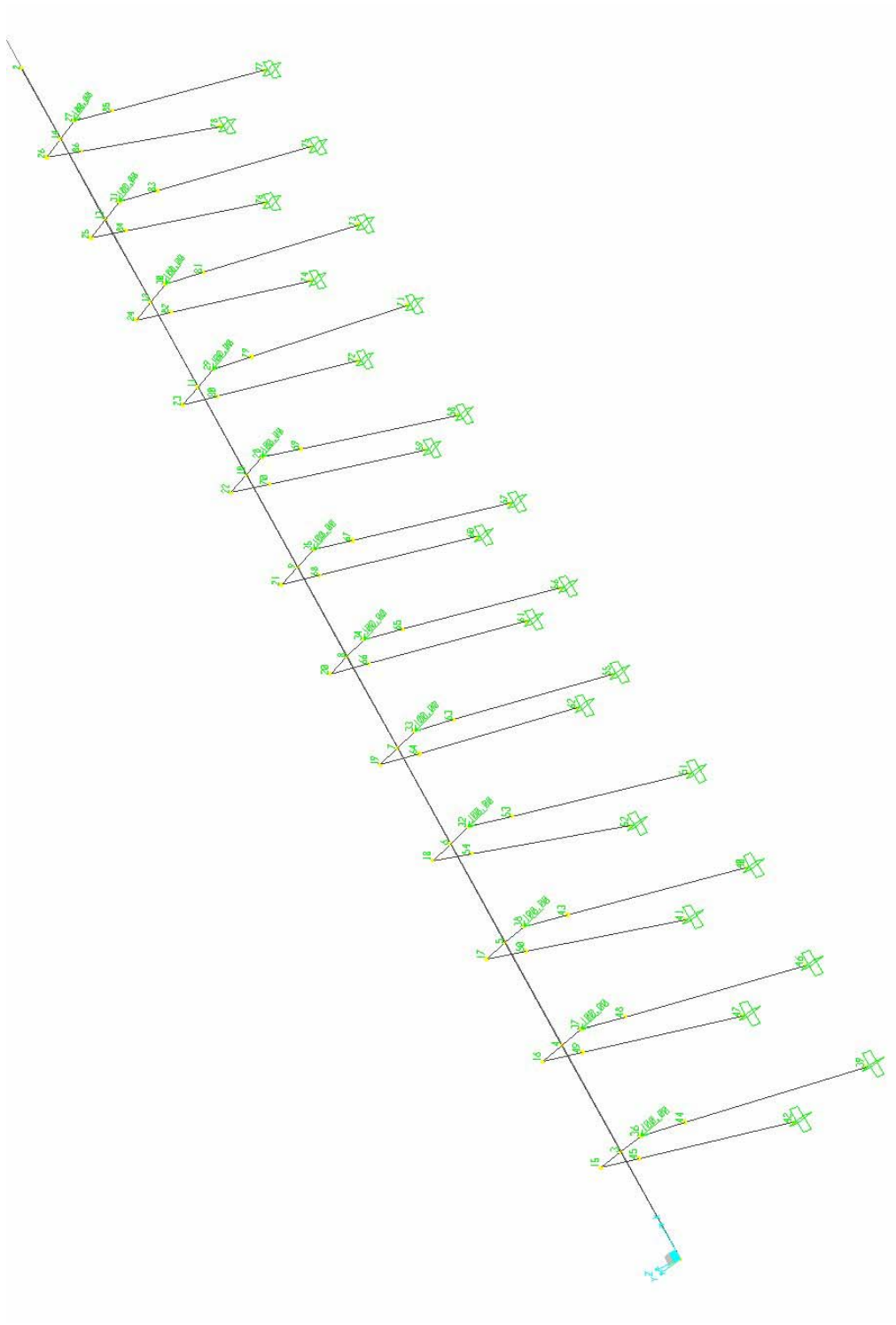
Figure VIII.A.9 CSI-SAP Model Subjected to 1200 Kips Longitudinal Loading
