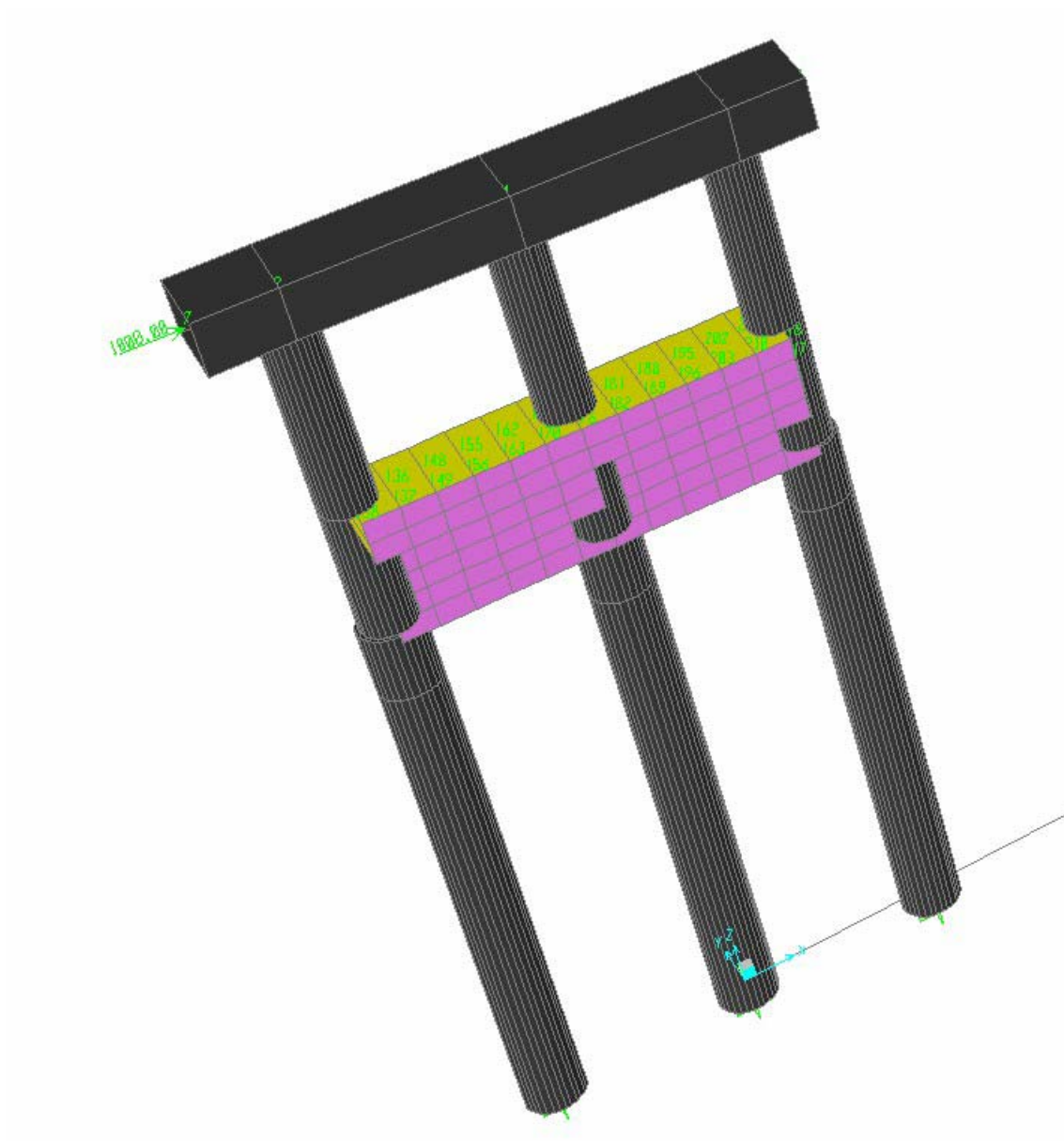
Figure VI.A.13 Model 1 Subjected to 1000 Kips Transverse Loading
