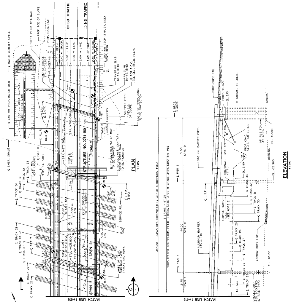
Figure 5.49: Dormeus Avenue Plan and Elevation ( 3of 3)
