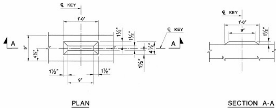
Figure VII.C.7 Typical Shear Key Detail
