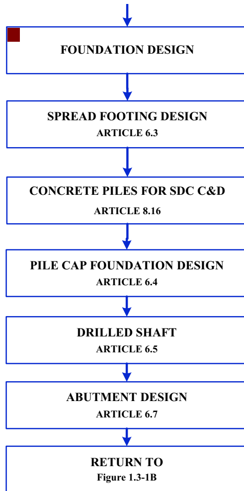
Figure 5.68 Foundation Design Flowchart 6
