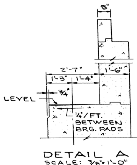
Figure 5.23 Detail A of Typical Abutment Section
