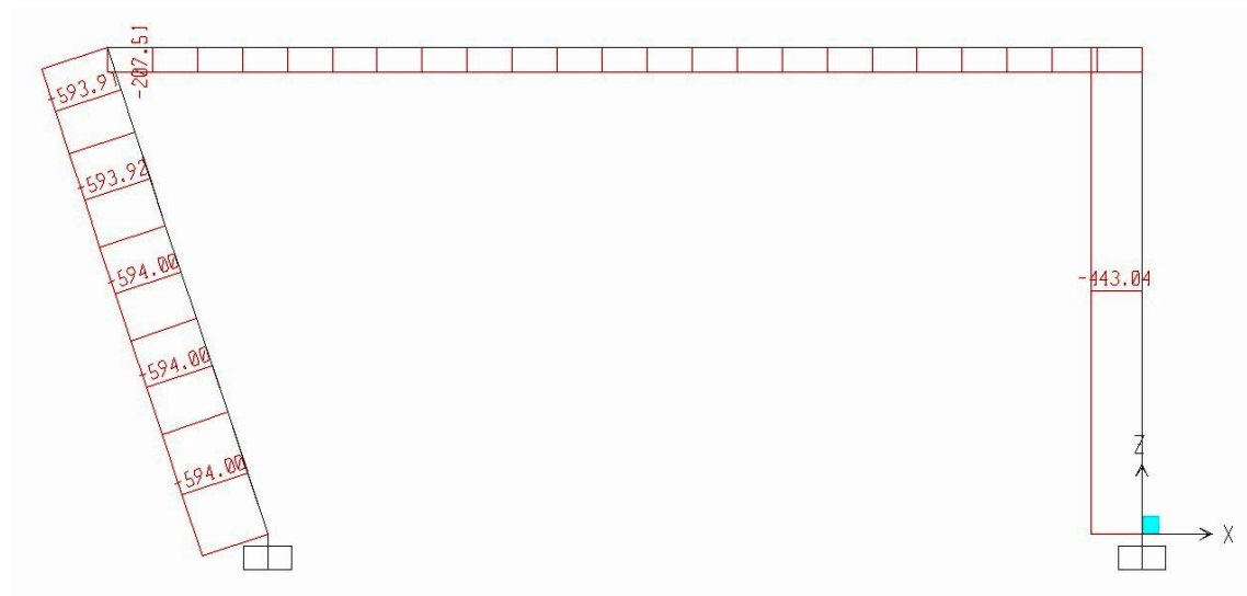
Figure VII.A.57 Pier 3 transverse Members Shear Lateral 2
