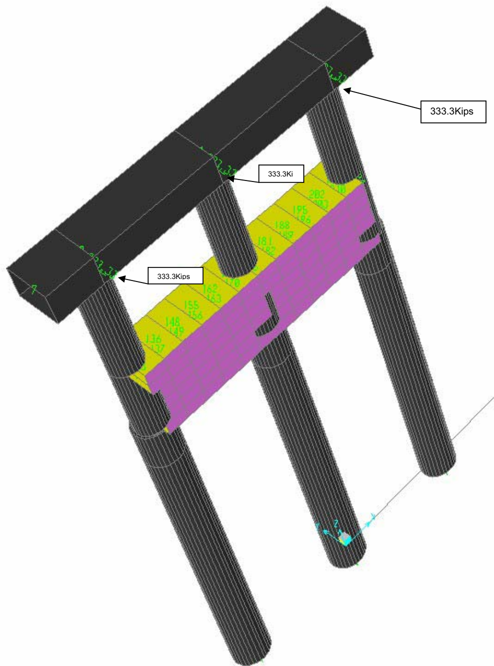
Figure VI.A.14 CSI_SAP Model 1 Subjected to 1000 Kips Longitudinal Loading
