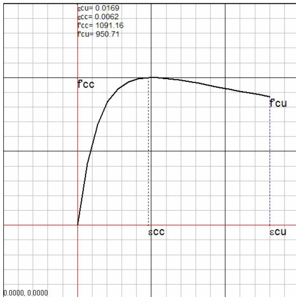
Figure VIII.A.2 Confined Concrete Stress Strain Model Section (PT)
