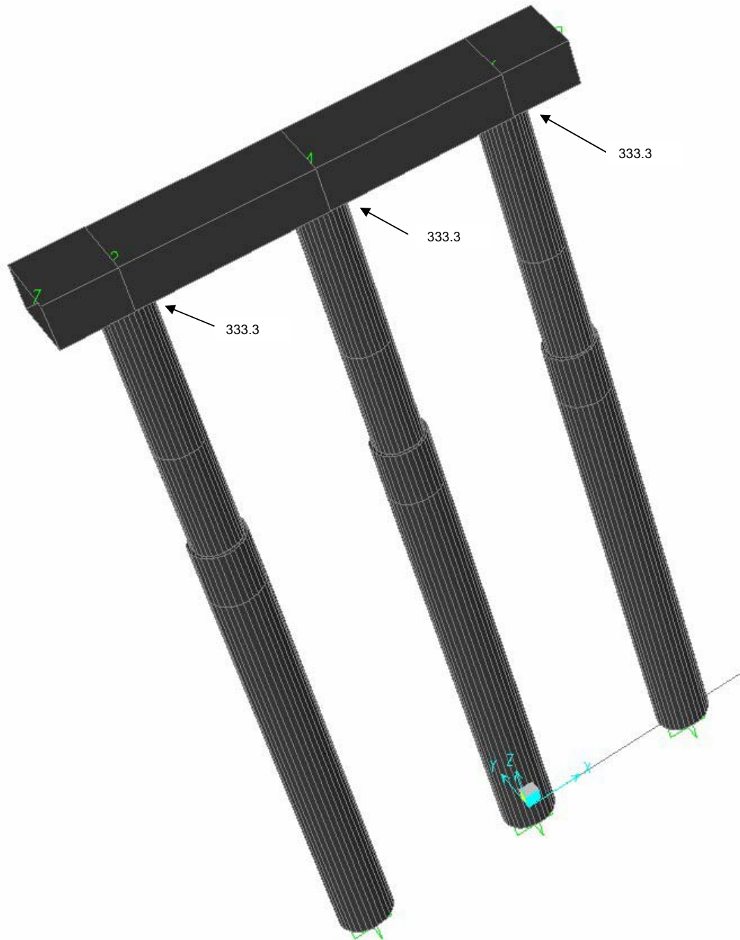
Figure VI.A.35 CSI-SAP Model 4 Subjected to 1000 Kips Longitudinal Loading
