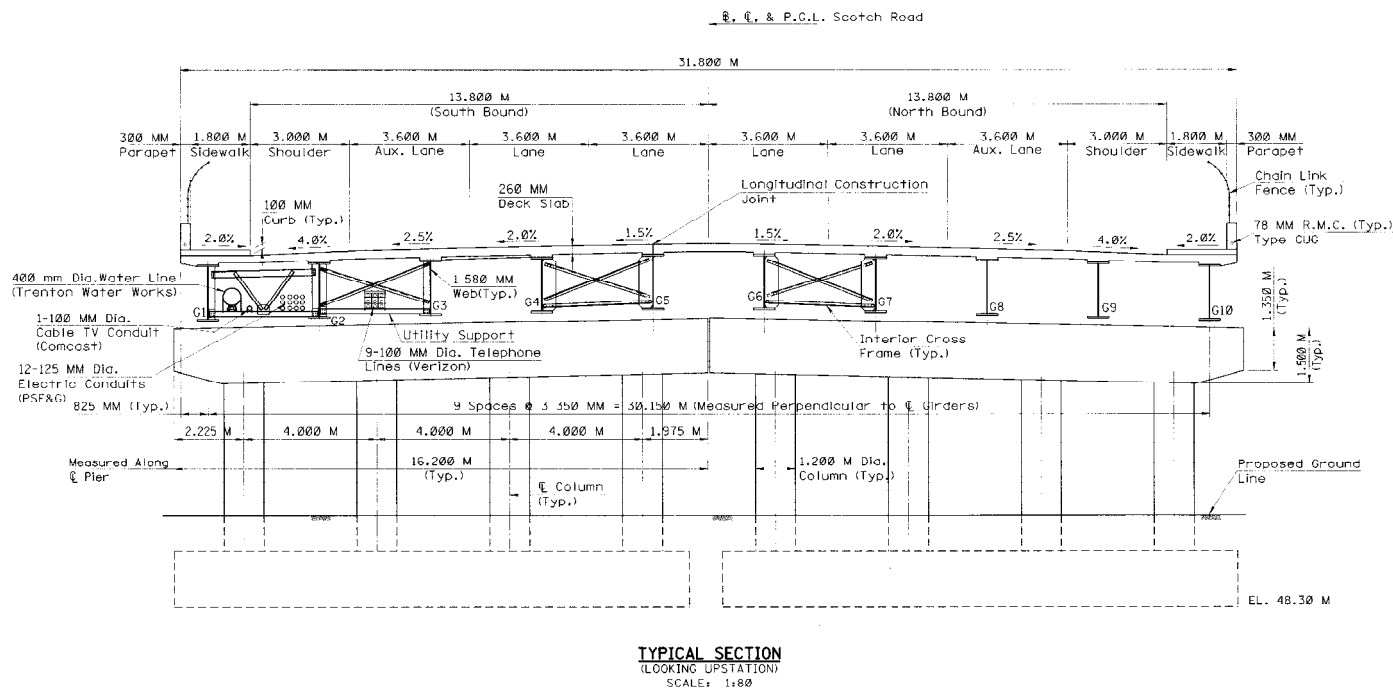
Figure 5.27 Typical Section
