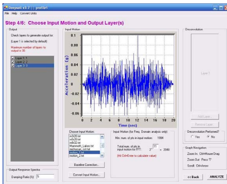
Figure III.68 Step 4 of 6
