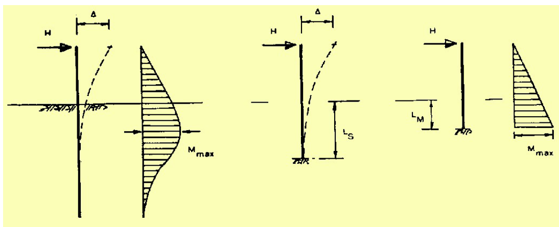
Figure 5.70 Estimated Depth to Fixity Model
