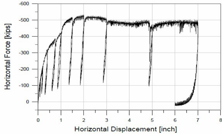
Figure 5.2. Load-displacement curve with backfill soil
