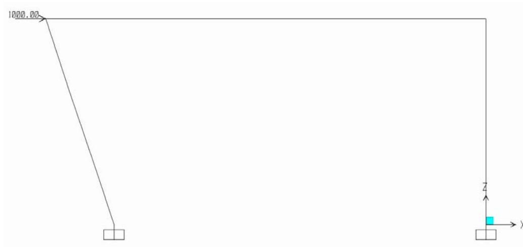
Figure VII.A.49 Pier 3 Transverse Loading Lateral 1
