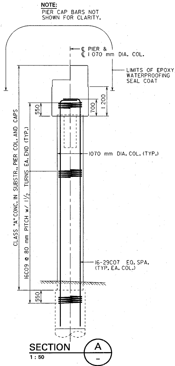
Figure VI.C.7 Section Pier 3
