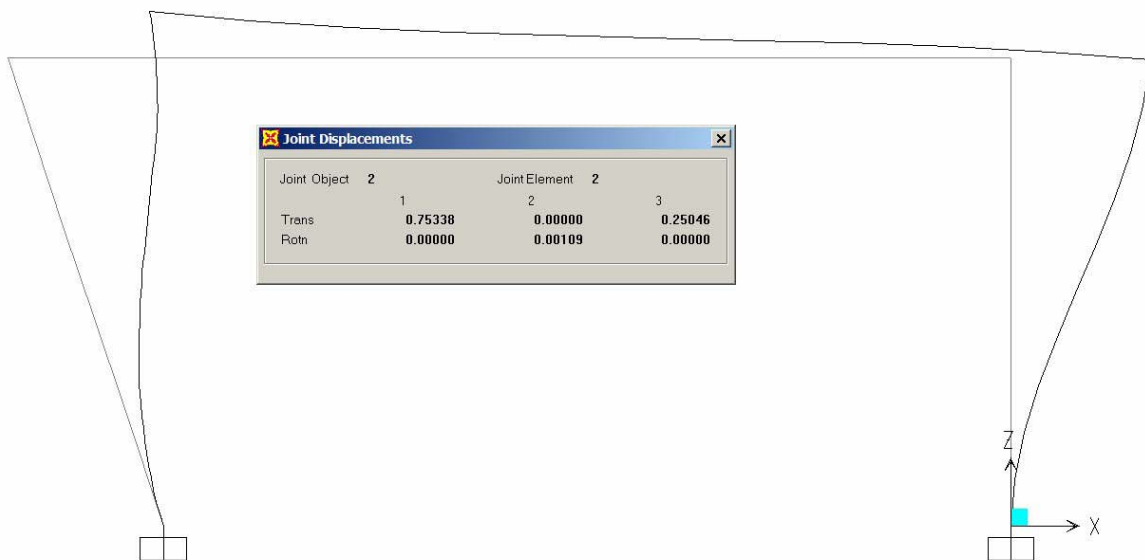
Figure VII.A.50 Pier 3 Transverse Displacement Lateral 1
