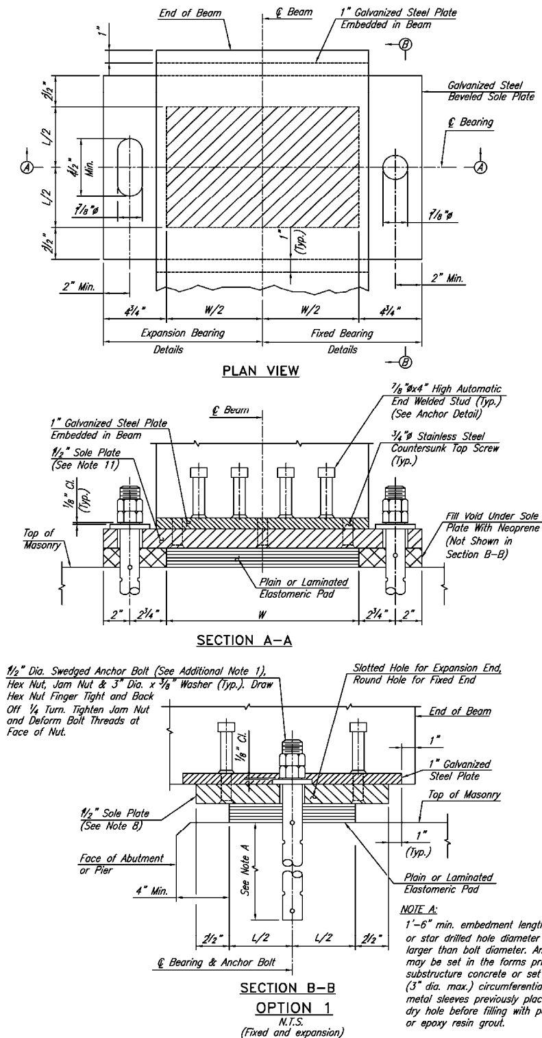
Figure 5.17 Bearing Connection Details
