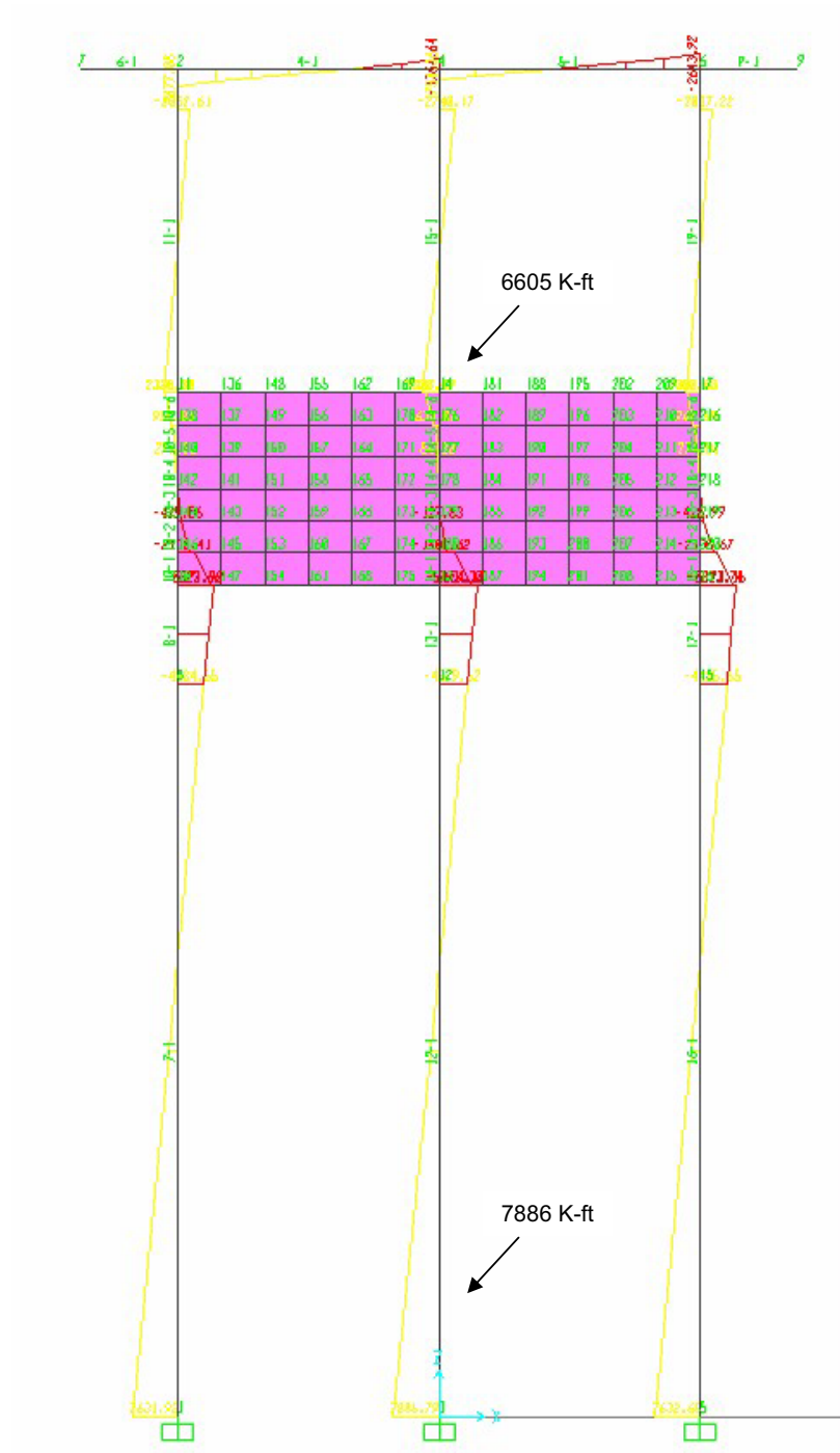
Figure VI.A.17 Model 1 Moment distribution for Bent Subject to 1000 Kips of Transverse Loading
