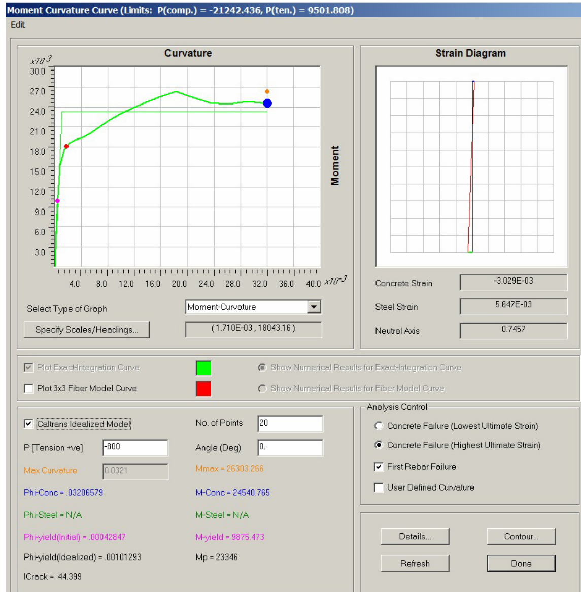
Figure VI.A.28 Moment Curvature Analysis (CSE3)
