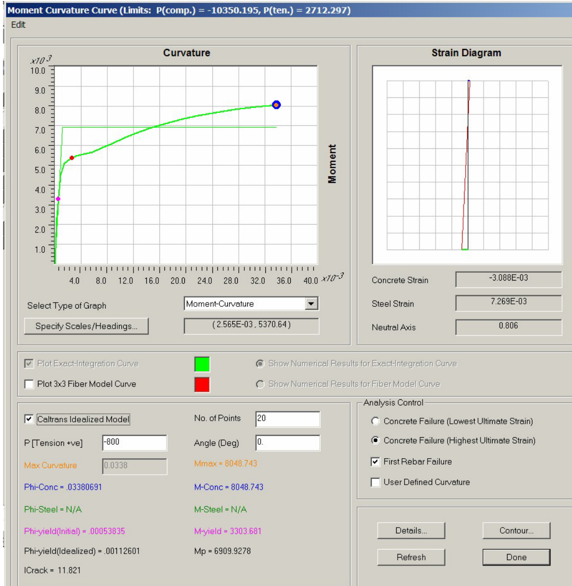
Figure VI.A.10 Movement Curvature Analysis (SC1)
