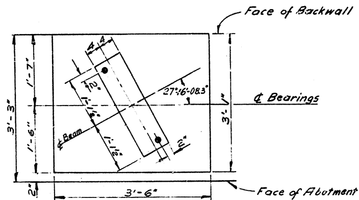
Figure 5.90 Anchor Bolts Location at Abutment Pedestals
