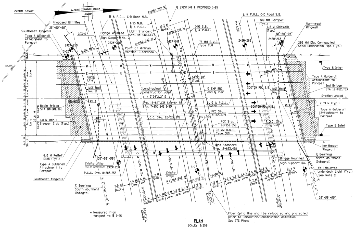
Figure 5.25 General Plan
