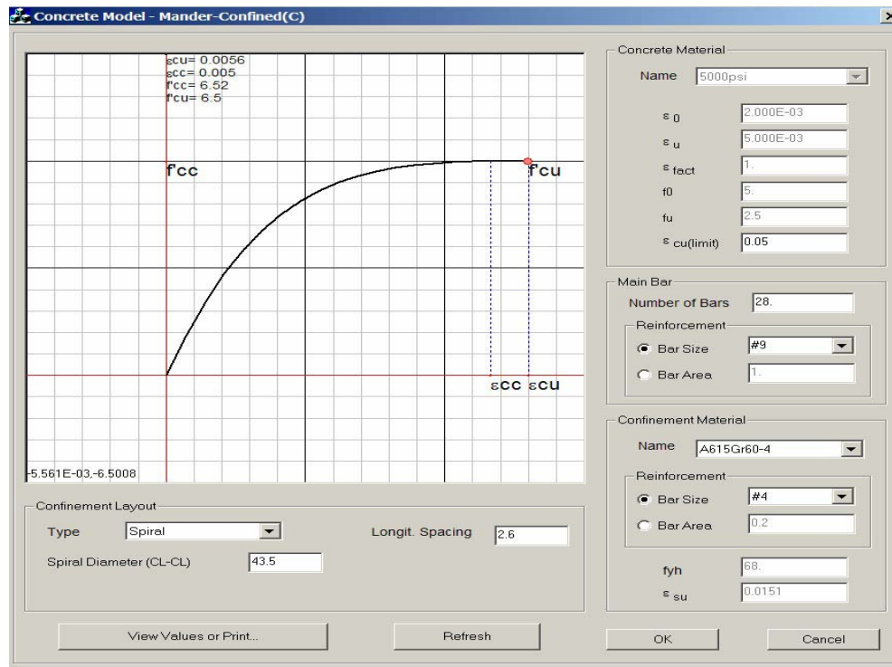
FIGURE V.5 CONFINED CONCRETE CORE.
