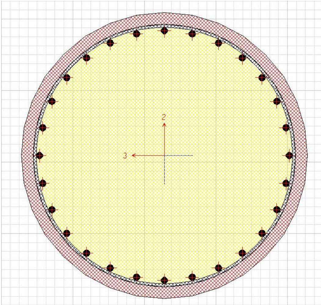
Figure V.1 Colum Section Model
