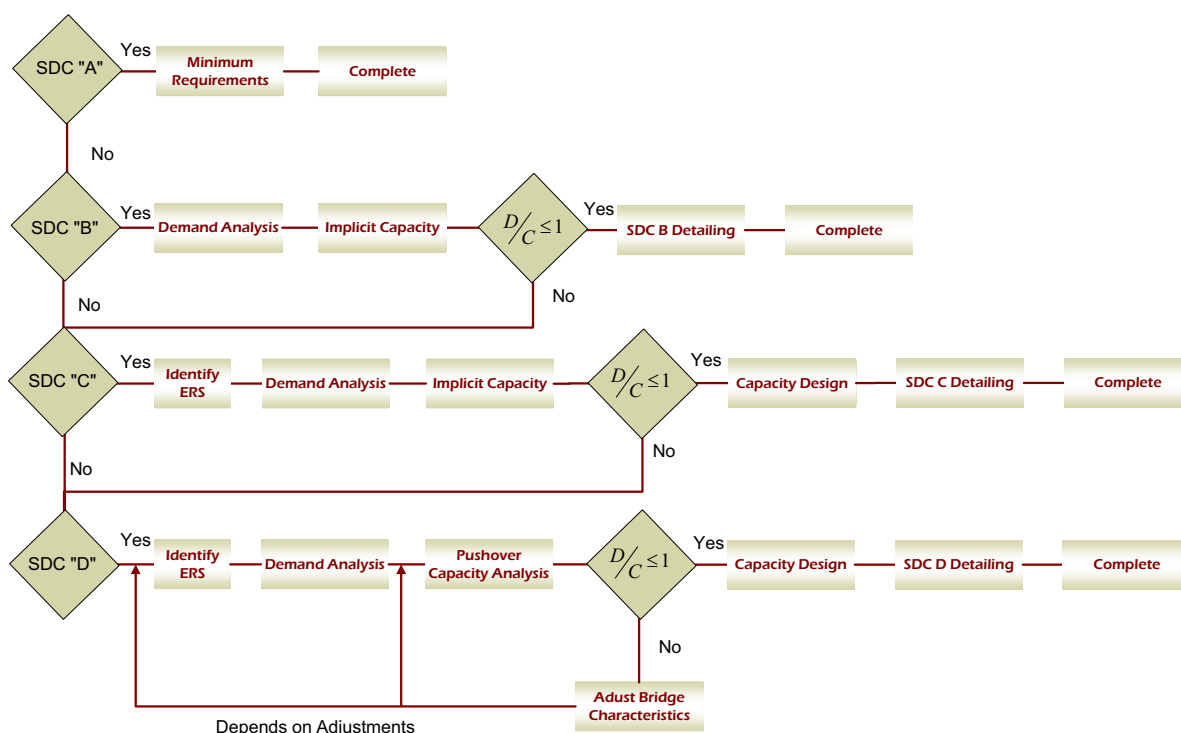
Figure 5.37 Seismic Design Category (SDC) Core Flowchart.
