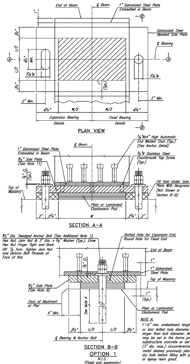
Figure 5.5 Bearing Connection Details
