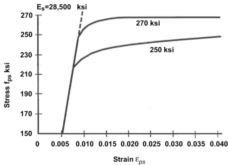
Figure VIII.A.1 Prestressing Strand Stress-Strain Model.
