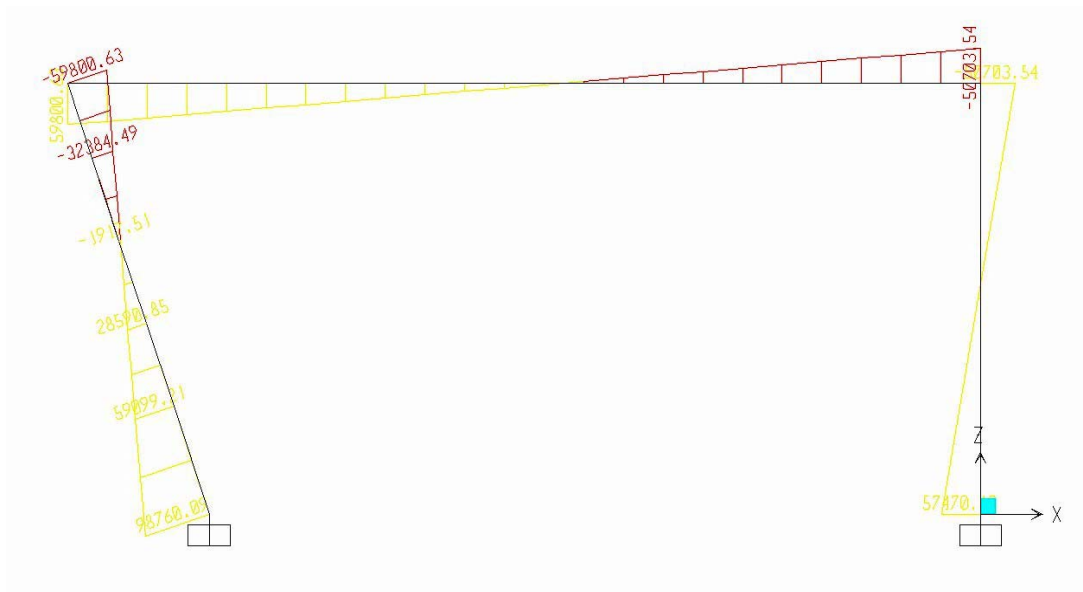
Figure VII.A.53 Pier 3 Transverse Members Moment Lateral 1
