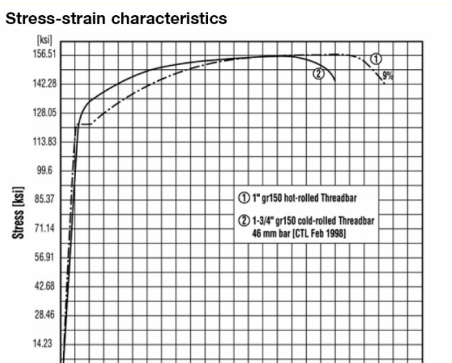
Figure VII.A.1 Stress-strain Curve for High Strength Bar
