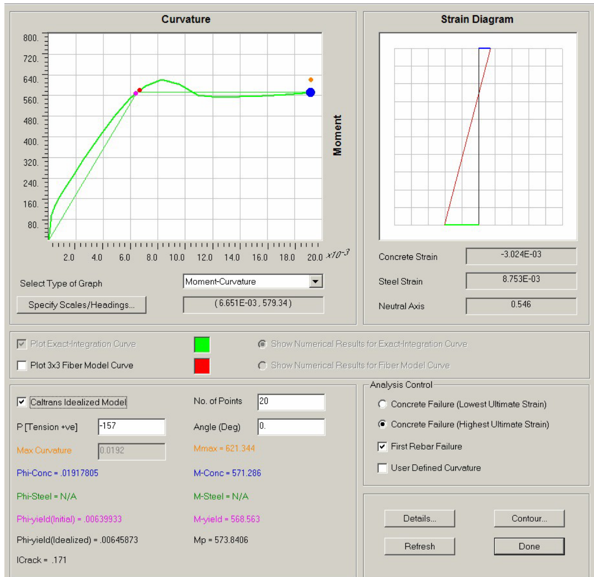
Figure VIII.A.7 Moment Curvature Analysis (PB)
