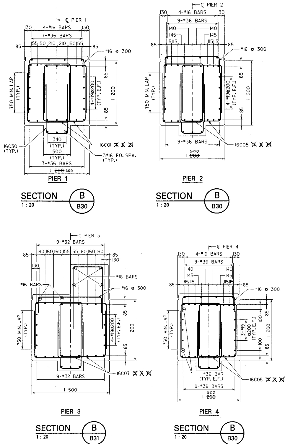
Figure VI.C.15 Bent Cap Section Piers 1, 2, 3, and 4
