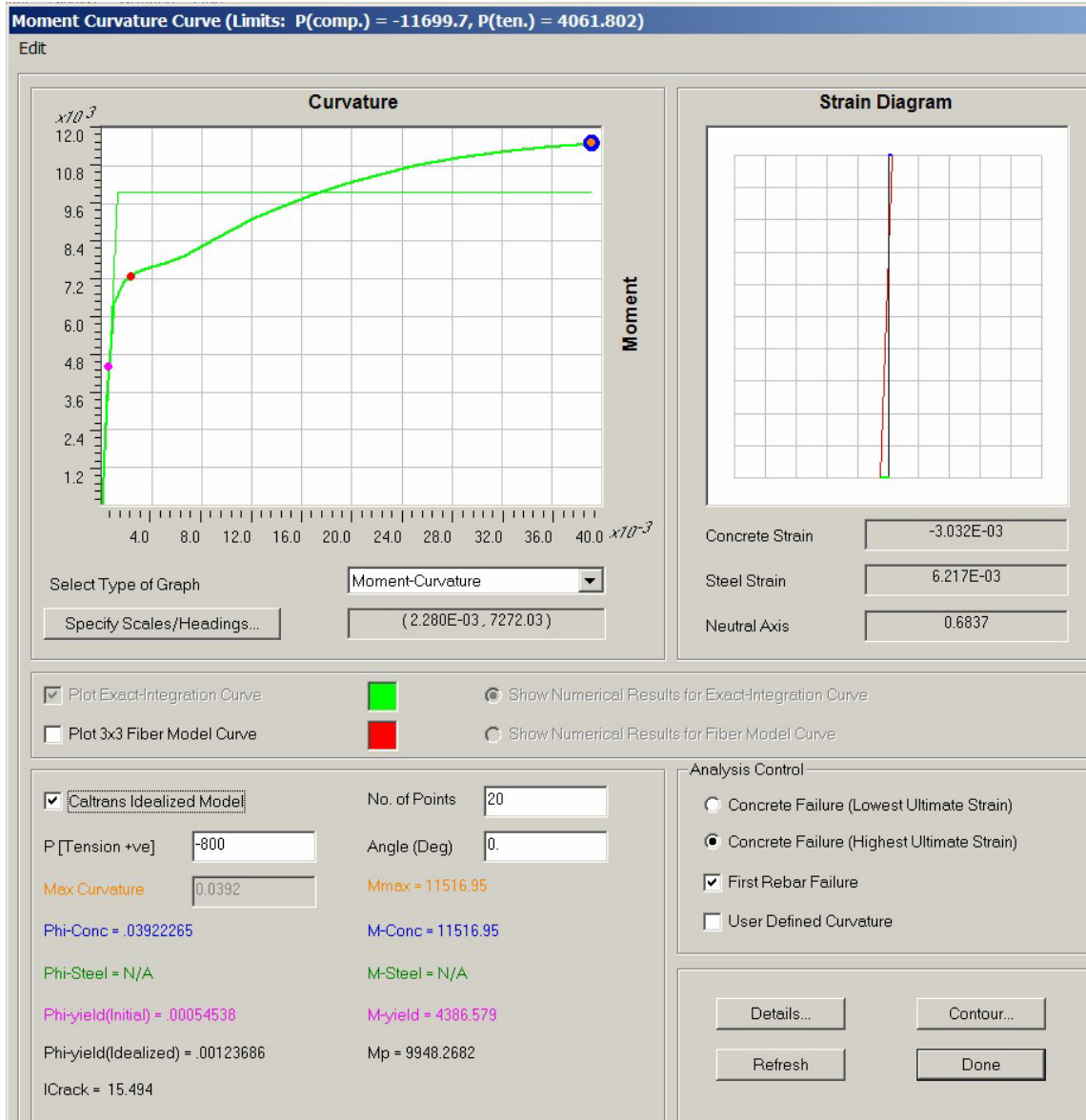
Figure VI.A.22 Moment Curvature Analysis (SC2)
