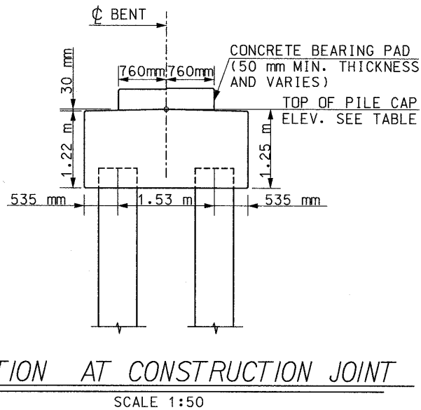
Figure VIII.C.9 Pile Bent Elevations
