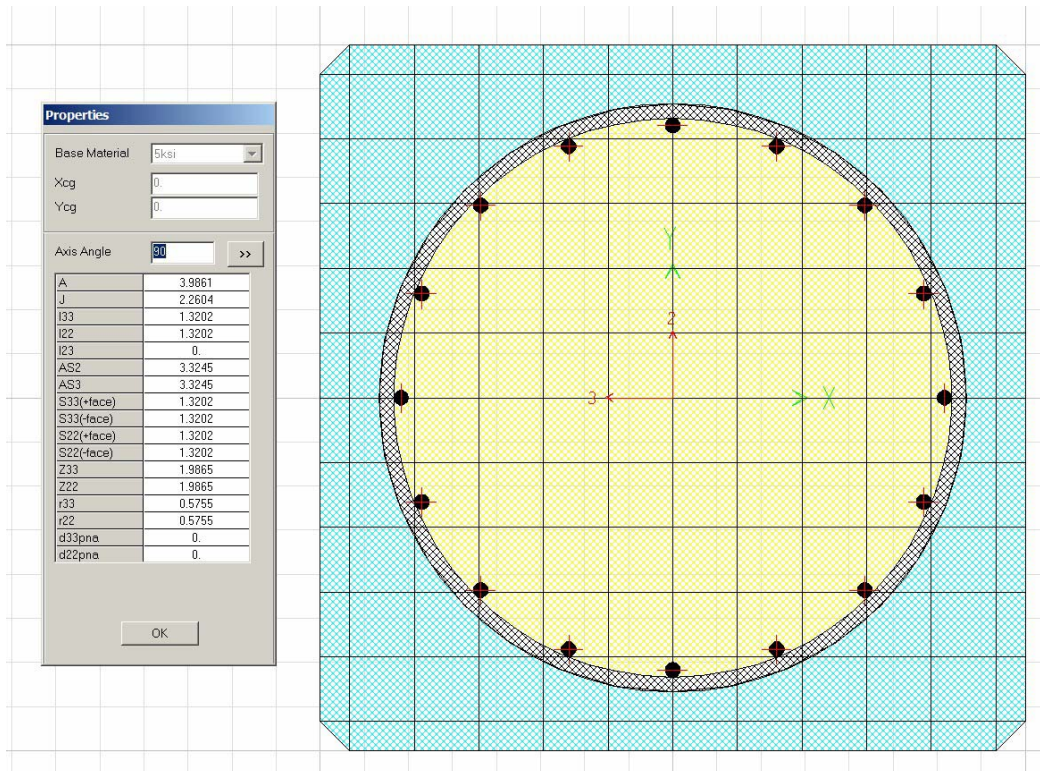
Figure VIII.A.6 Pile Gross Properties (PB)
