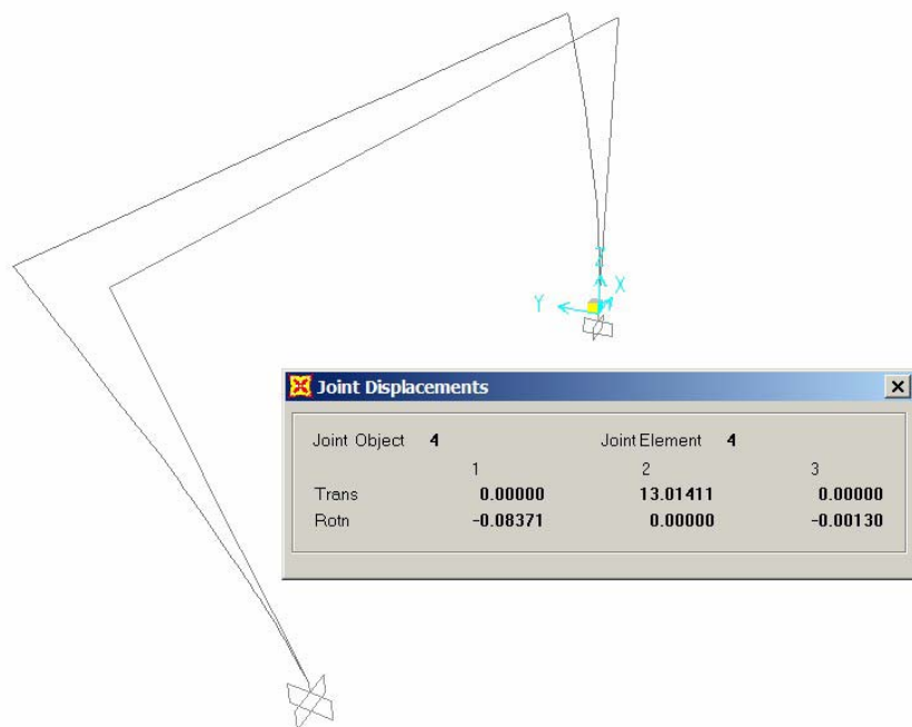
Figure VII.A.48 Pier 3 Inner Column Longitudinal Displacement
