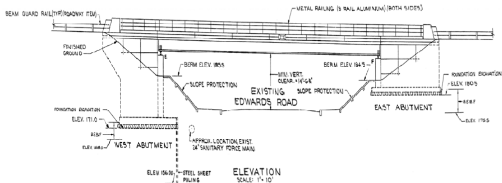
Figure 5.2 Elevation
