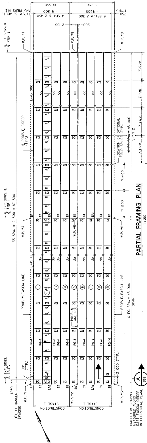
Figure VI.B.6 Partial Framing Plan Spans 1 and 2
