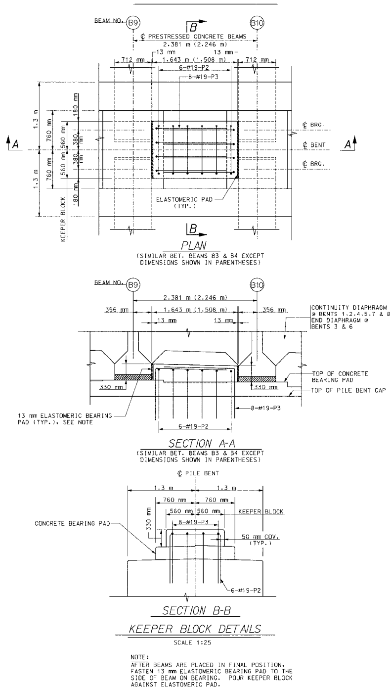
Figure VIII.C.13 Keeper Block Details at Pile Bents
