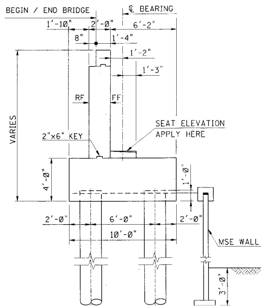
Figure VII.C.20 Abutment Section A-A
