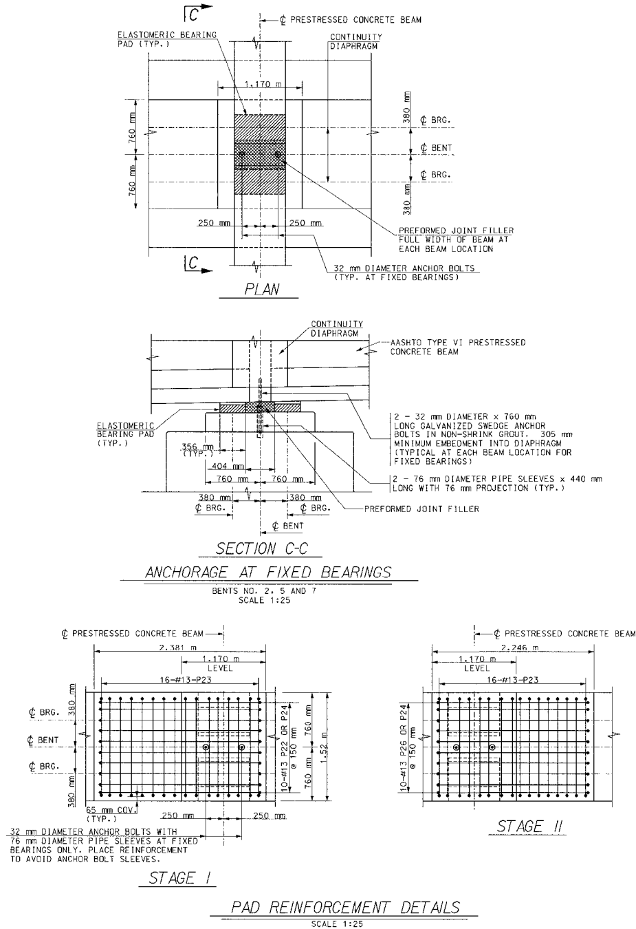
Figure VIII.C.14 Pad Reinforcement Details at Pile Bents
