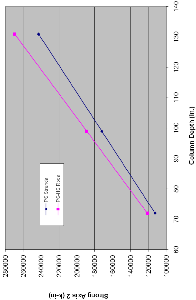
Figure VII.A.40 Strong Axis 2 Flexural Capacity CS3A, CS4B, and CS13B
