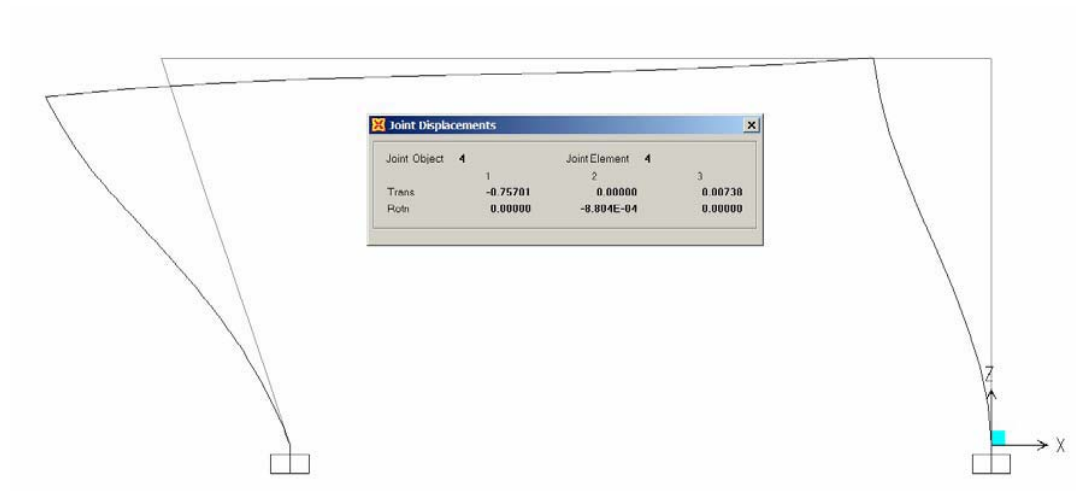
Figure VII.A.55 Pier 3 Transverse Displacement Lateral 2
