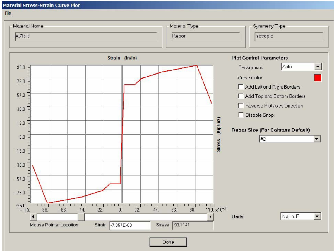
Figure VI.A.3 A615 Grade Reinforcement Stress Strain Model
