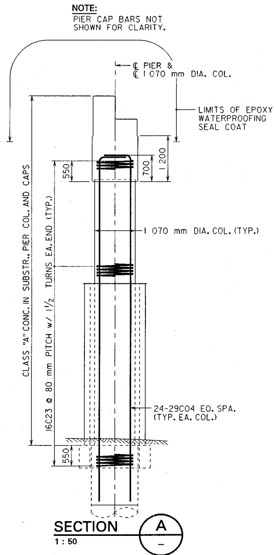
Figure VI.C.11 Section Pier 6
