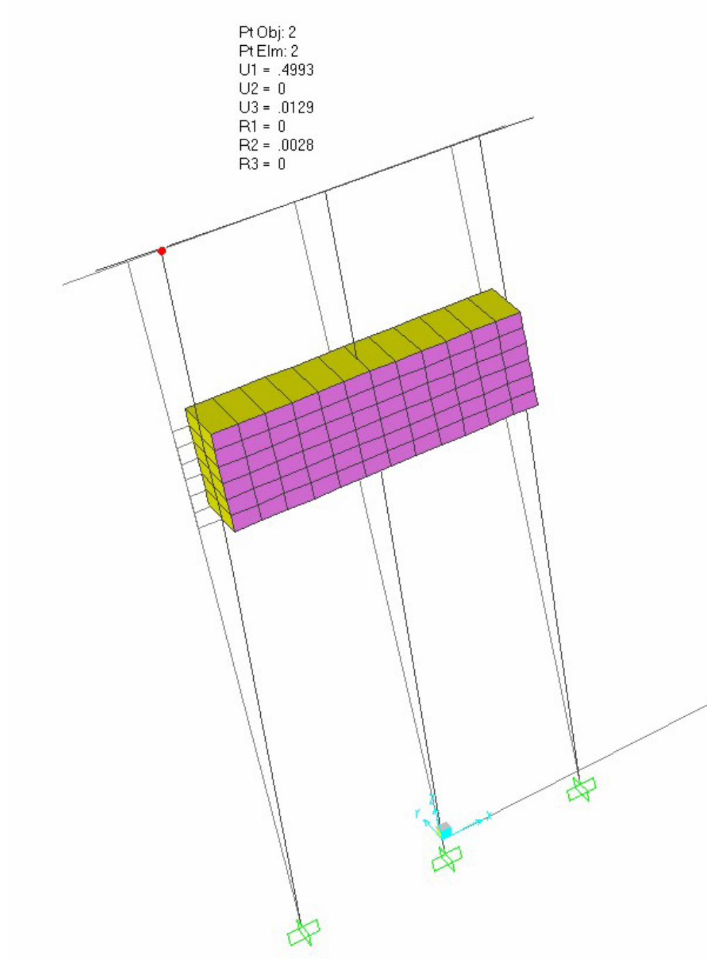
Figure VI.A.23 Response of Model 2 Subjected to 1000 Kips of Transverse Loading
