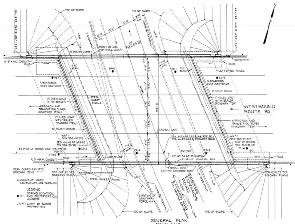
Figure 5.13 General Plan
