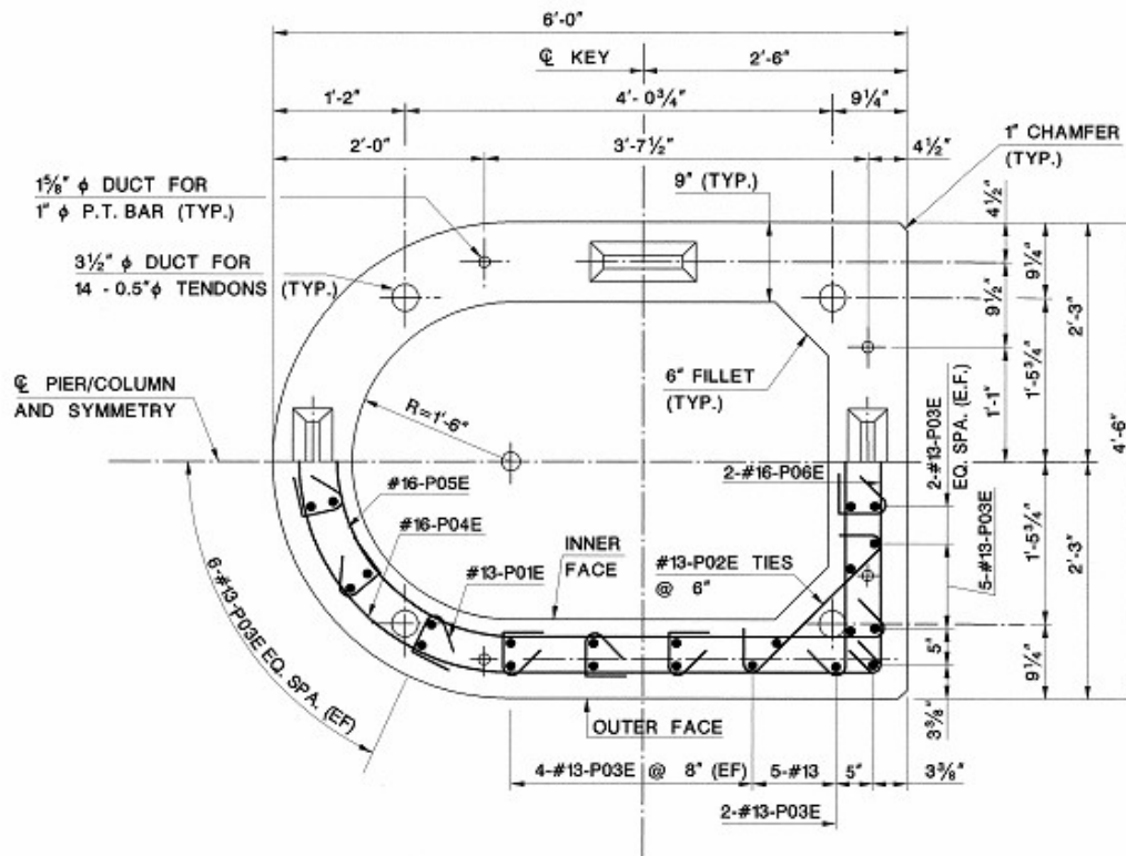
Figure VII.C.8 Inner Column Section
