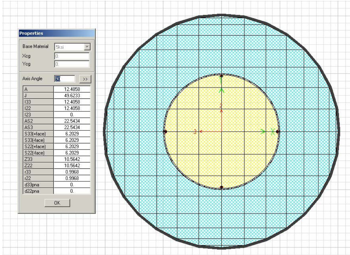
Figure VI.A.9 Shaft Casing Gross Properties (SC1)
