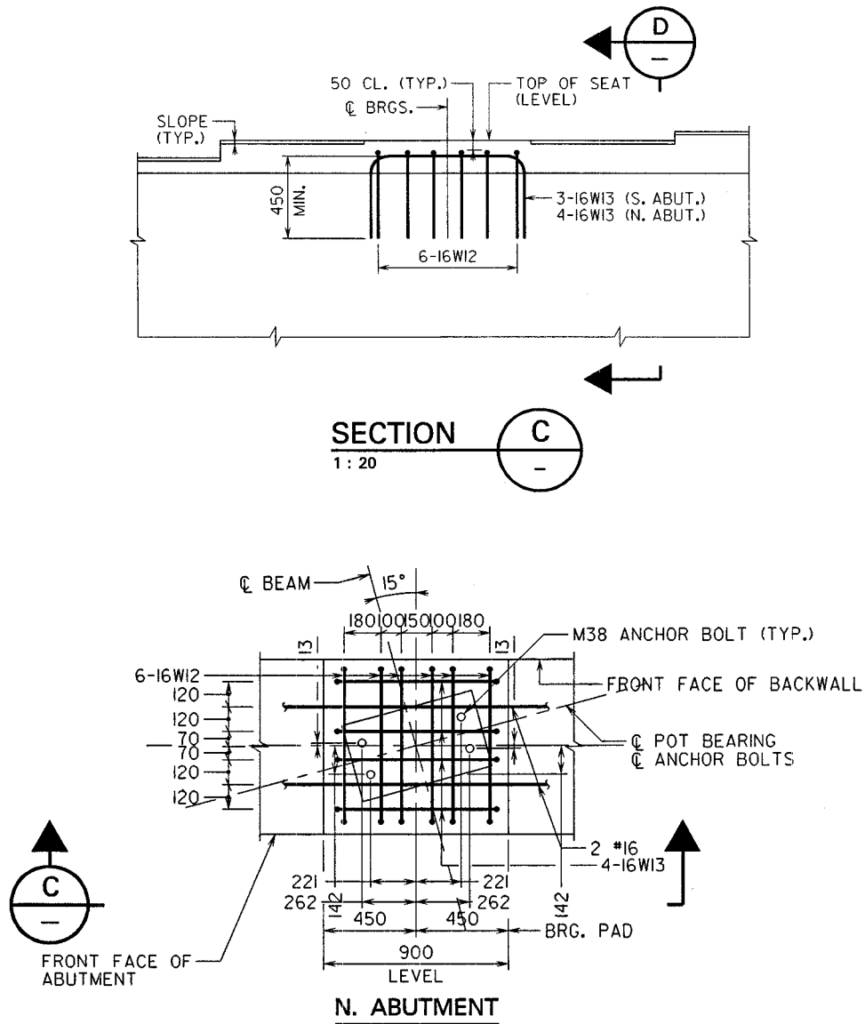
Figure VI.C.3 Bearing Pedestal Plan and Section
