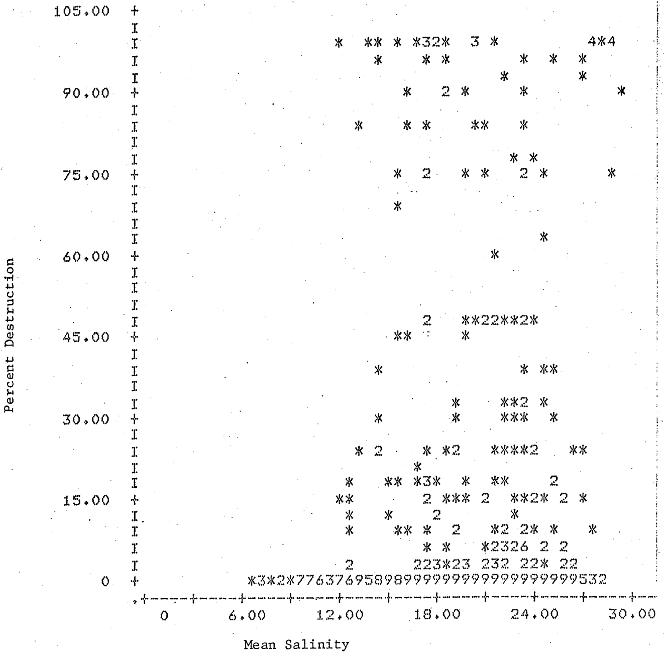
FIGURE A-9. PERCENT DESTRUCTION VERSUS MEAN SALINITY FOR EACH 6-MONTH EXPOSURE PANEL REMOVED FROM DECEMBER, 1975, THROUGH NOVEMBER, 1978
