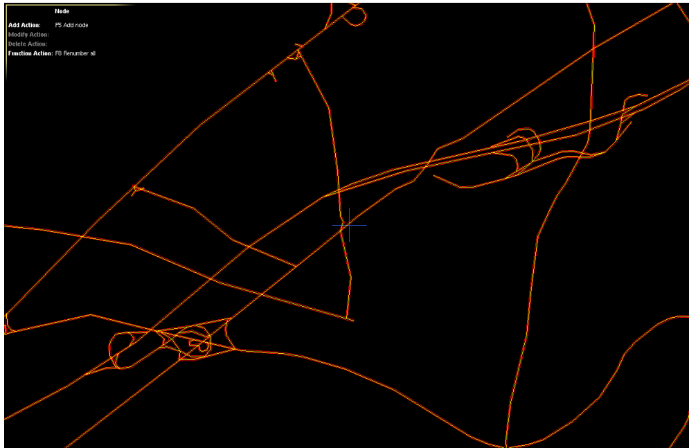
Figure 9. Paramics network
