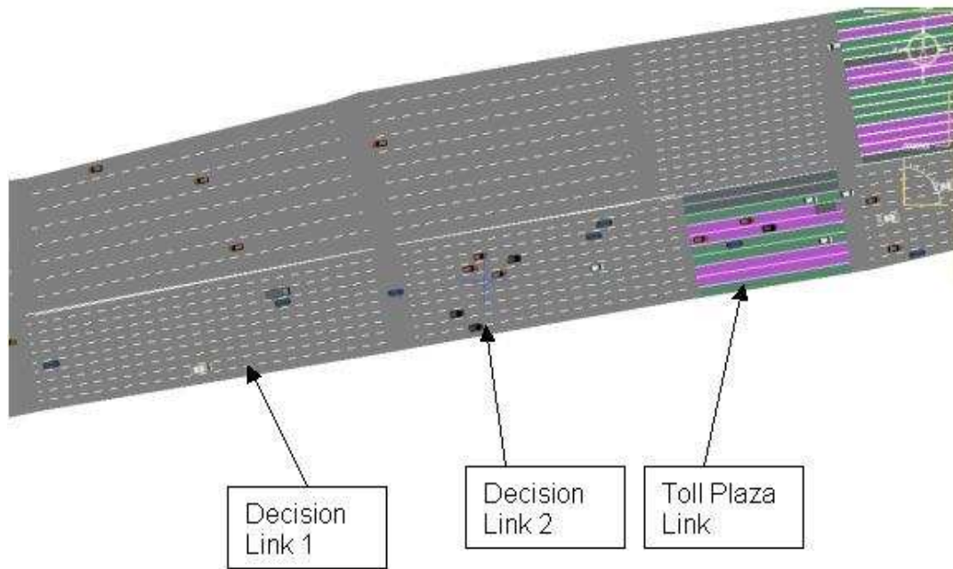
Figure 15. Graphical depiction of toll plaza lane changing behavior
