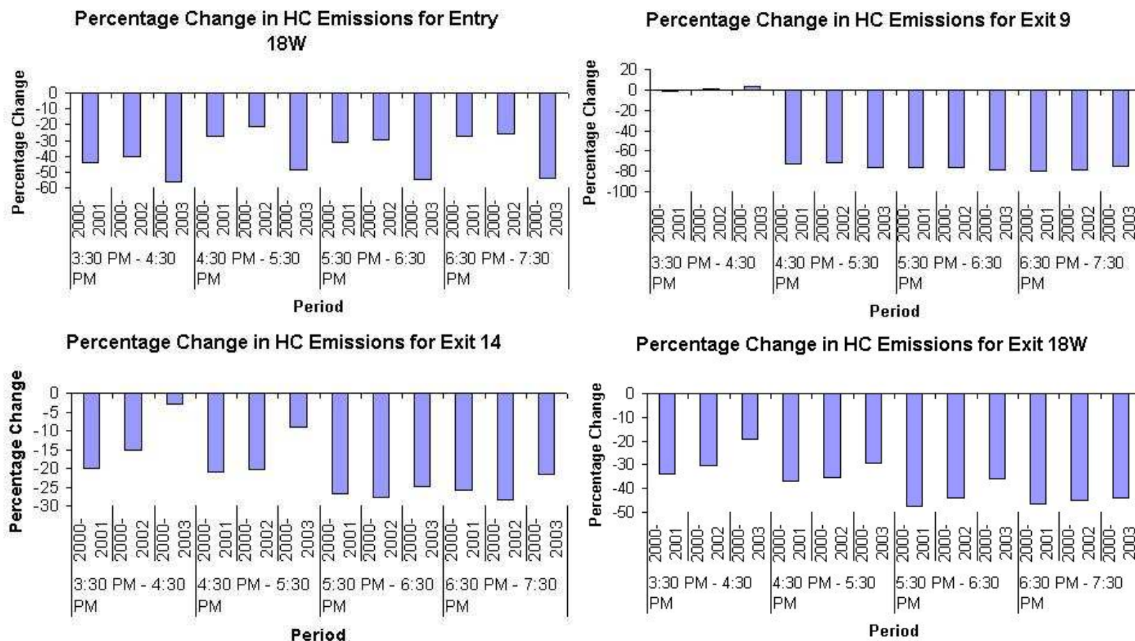
Figure 50. Percent change in emissions at the exit toll plazas (9, 14, 18W) Entry 18W for various periods during the PM period
