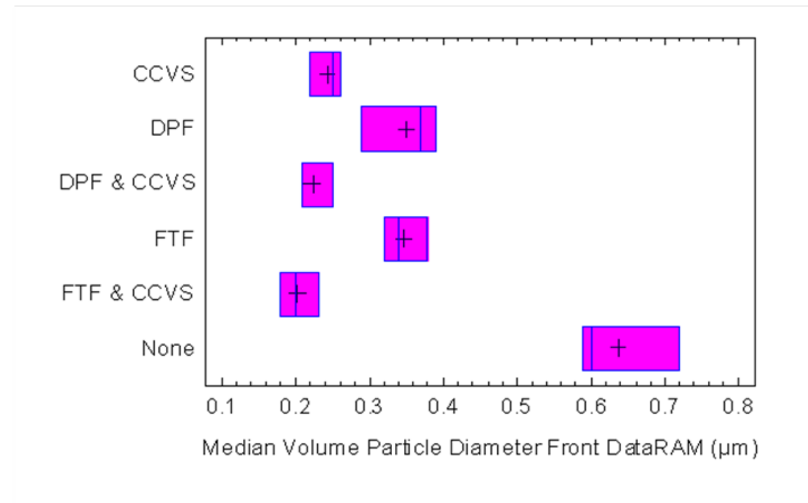
Figure 53: Box and whisker plot for particle size results from the DataRAM located in the front of the bus.
