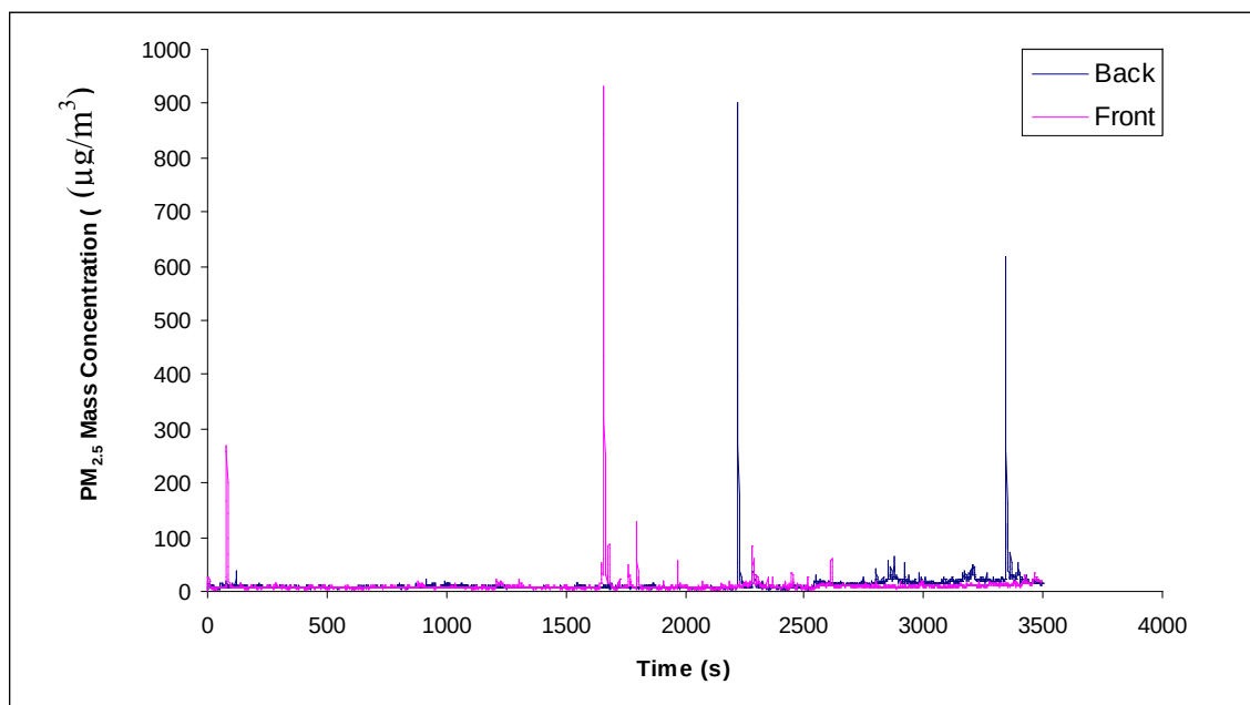
Figure 66 Run 33, Idle test with DPF & CCF windows closed PM2.5 mass concentration, May 14-07.
