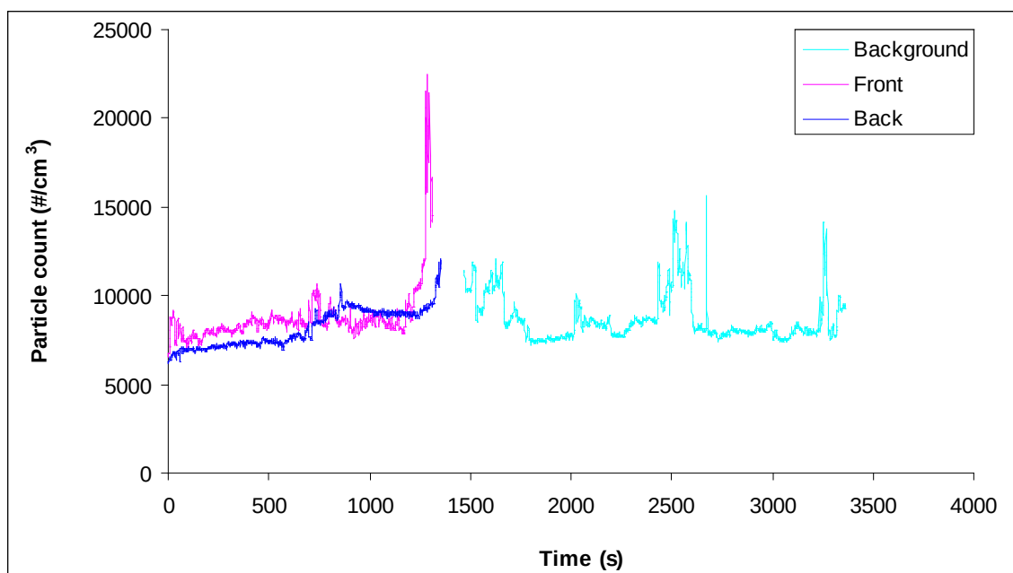
Figure 67 Run 33, Idle test with DPF & CCF windows closed Particle Count, May 14-07.
