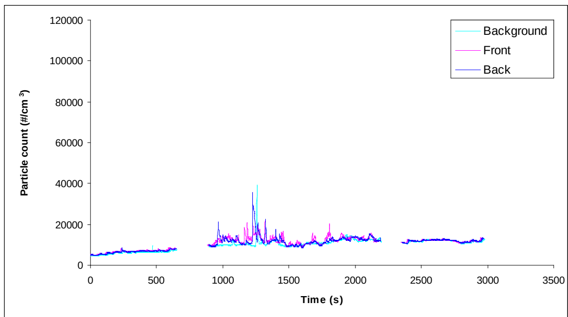
Figure 93 Run 46, FTF windows open Particle Count, May 21.
