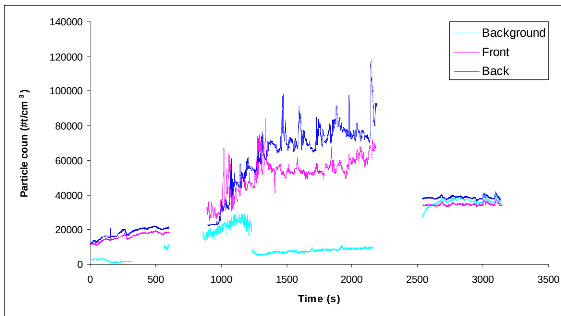
Figure 77 Run 38, FTF & CCF windows closed Particle Count, May 17.
