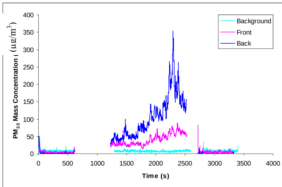
Figure 30 Run 15, CCF windows closed PM 2.5 mass concentration, April 18-07. Run had particle size >1.0µm, and build up of >20µg/m 3 before the run
