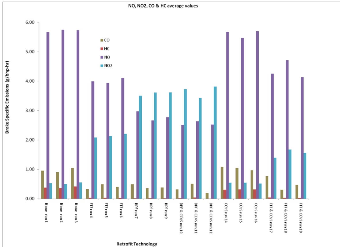
Figure 49: Gas emissions results for new set of runs with average NO, NO 2 , CO, and HC values. Note: the NO x values for all the technologies resulted in a 4% coefficient of variation.
