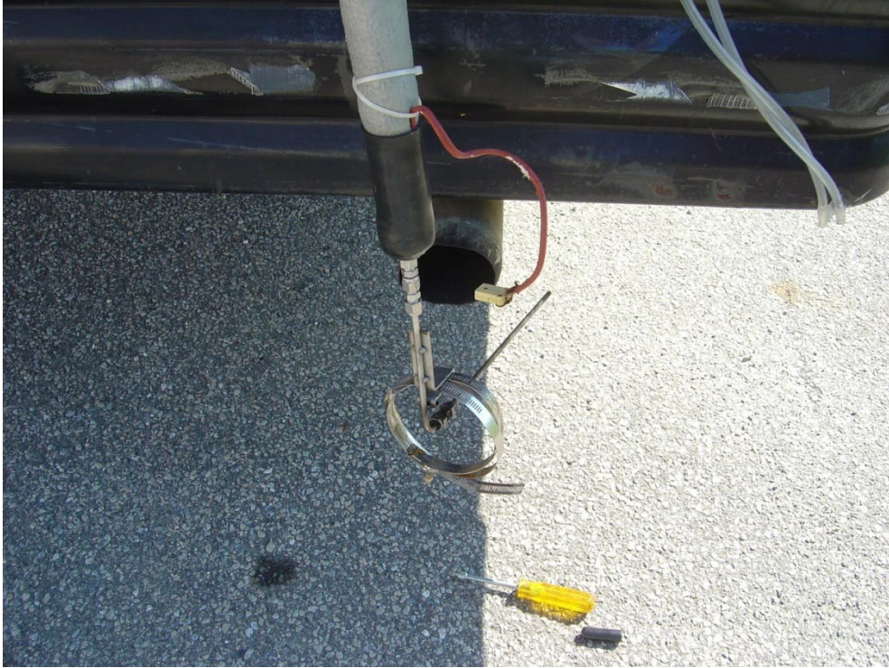
Figure 21: SEMTECH-D sampling tip before being inserted and secured to the tailpipe. Picture of the system taken for the final set of runs.
