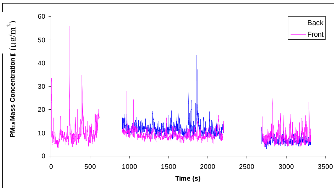
Figure 68 Run 34, DPF & CCF windows closed PM 2.5 mass concentration, May 14.
