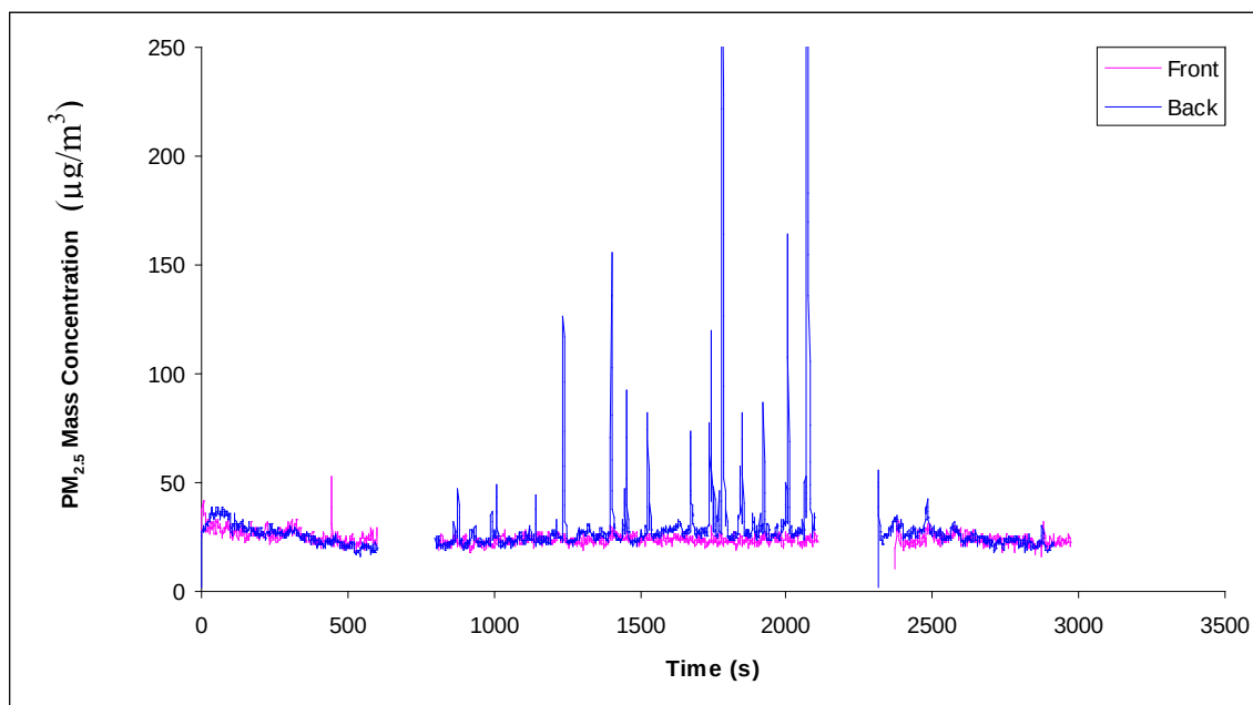
Figure 122 Run 61, DPF windows closed PM2.5 mass concentration, June 13.
