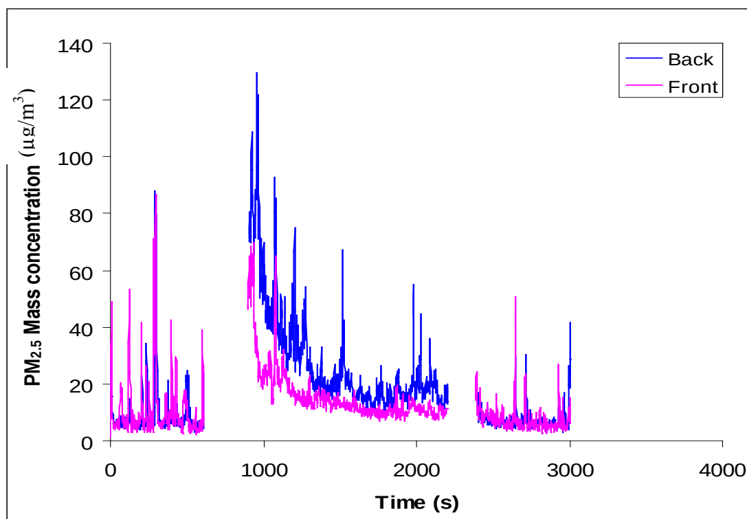
Figure 46 Run 23, DPF & CCF windows closed, May 7-07. DR1 Back , DR2 Front of bus Initial build up of concentration before the test started. Particle size for Back instrument during run = 1.30\mu\text{m}
