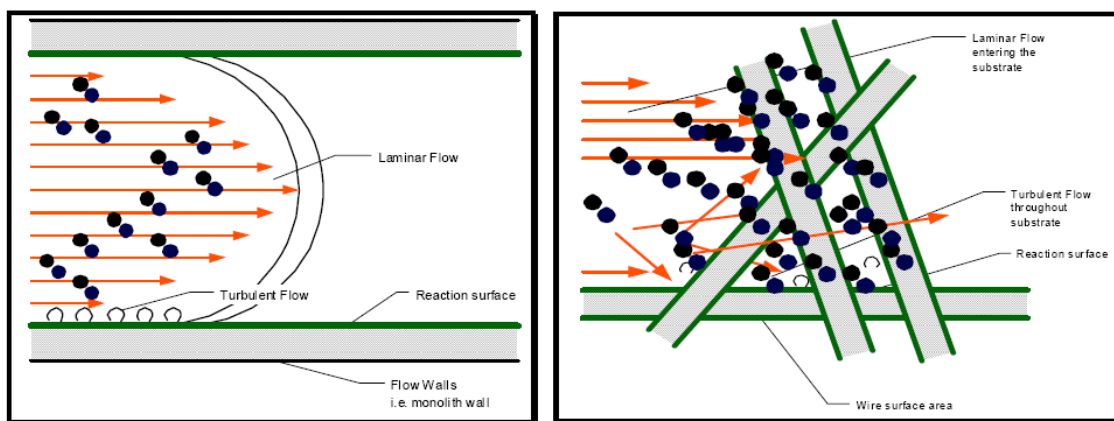
Figure 11: Representation of exhaust laminar flow through a diesel oxidation catalyst (left) and the ESW Particulate Reactor ® (right). Source: M.J. Bradley & Associates, Inc. (2006) 13 .
