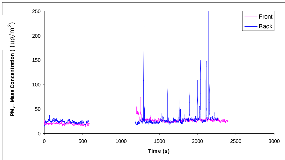
Figure 112 Run 56, DPF & CCF windows closed, June 7. Ran out of fuel with about 3 minutes left.
