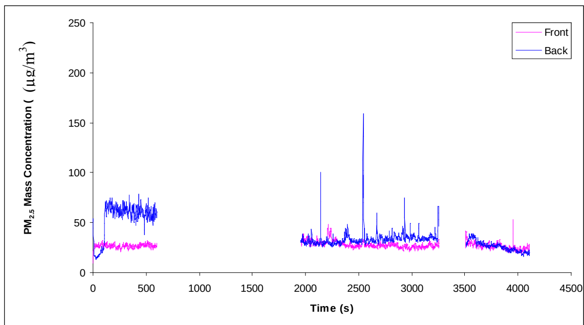
Figure 120 Run 60, DPF windows closed PM 2.5 mass concentration, June 13. Particle size: Back Pre= 3.584 \mu\text{m}
