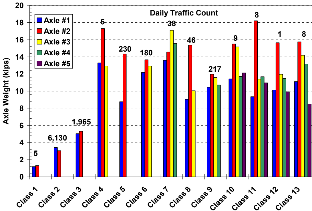
Figure 31 – Axle Load Spectra (ALS) for Rt. 34N in New Jersey
