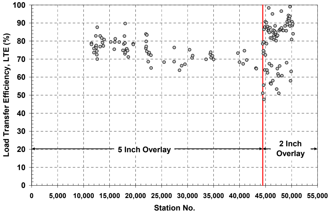
Figure 54 – Load Transfer Efficiency (LTE) at PCC Joint/Crack
