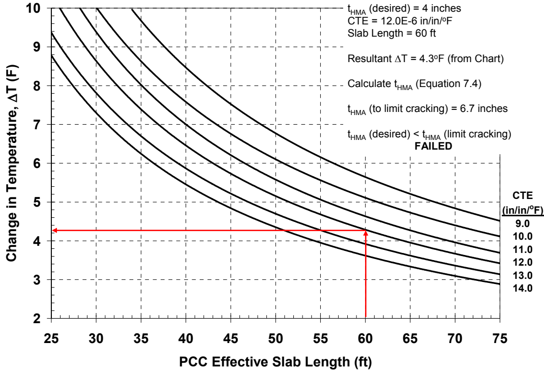
Figure 99 – Example of Using Proposed Guideline to Limit Horizontal Deformation-Related Fatigue Cracking – Required Asphalt Overlay Thickness
