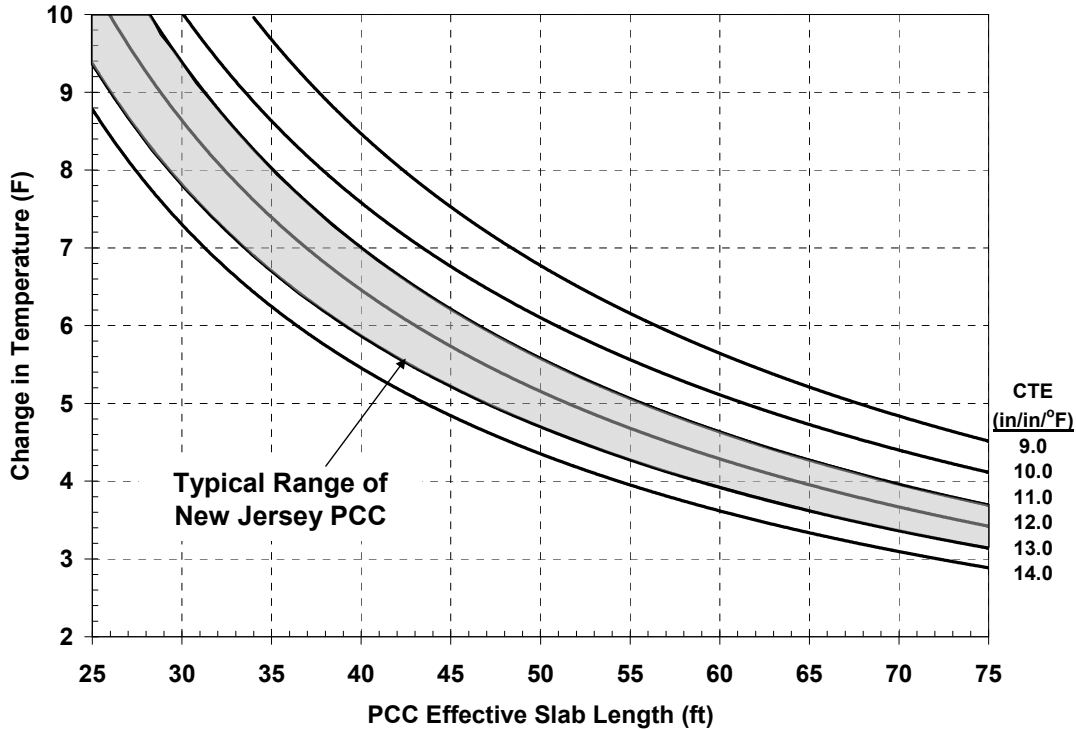
Figure 98 – Proposed Guideline to Limit Horizontal Deformation-Related Fatigue Cracking
