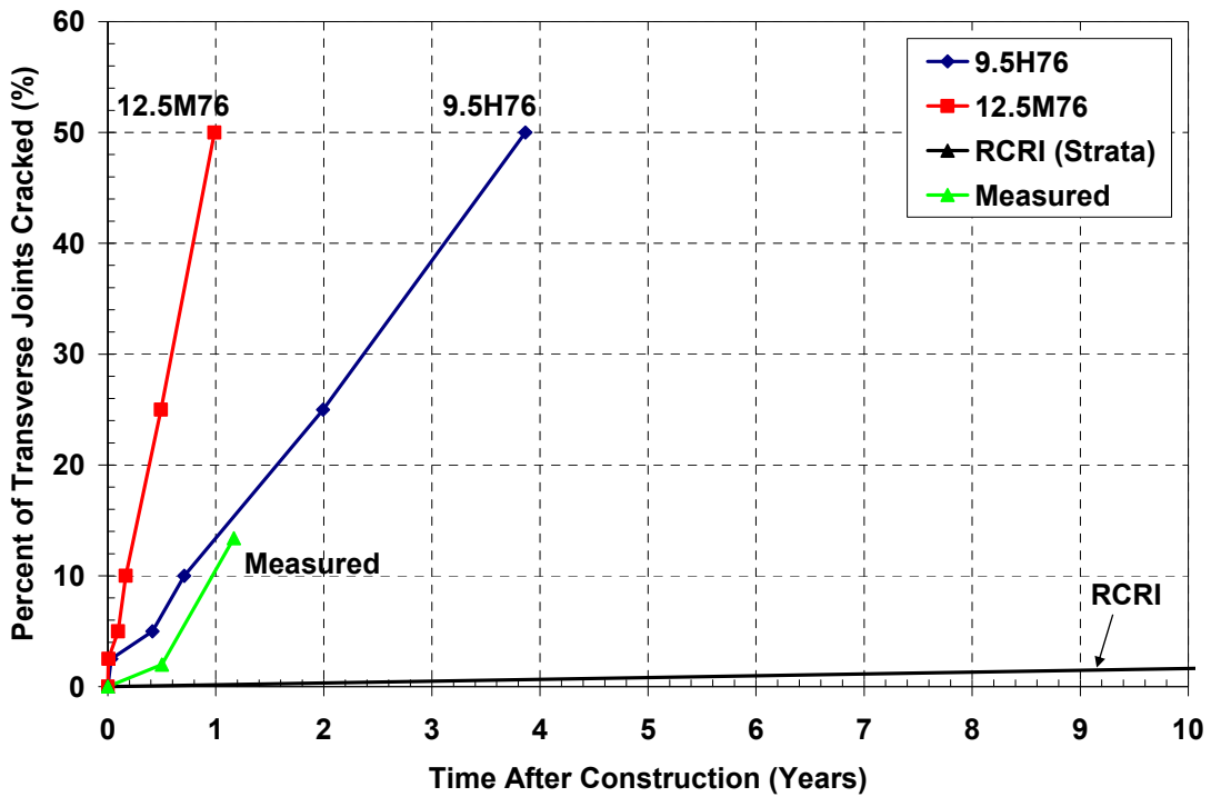
Figure 85 – Predicted versus Measured Reflective Cracking of Test Section #3 on Rt 34N New Jersey
