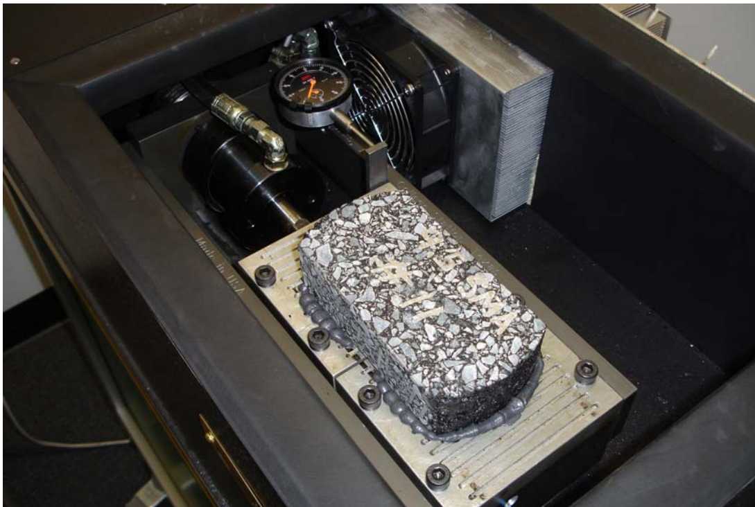
Figure 24 – Overlay Tester Device
