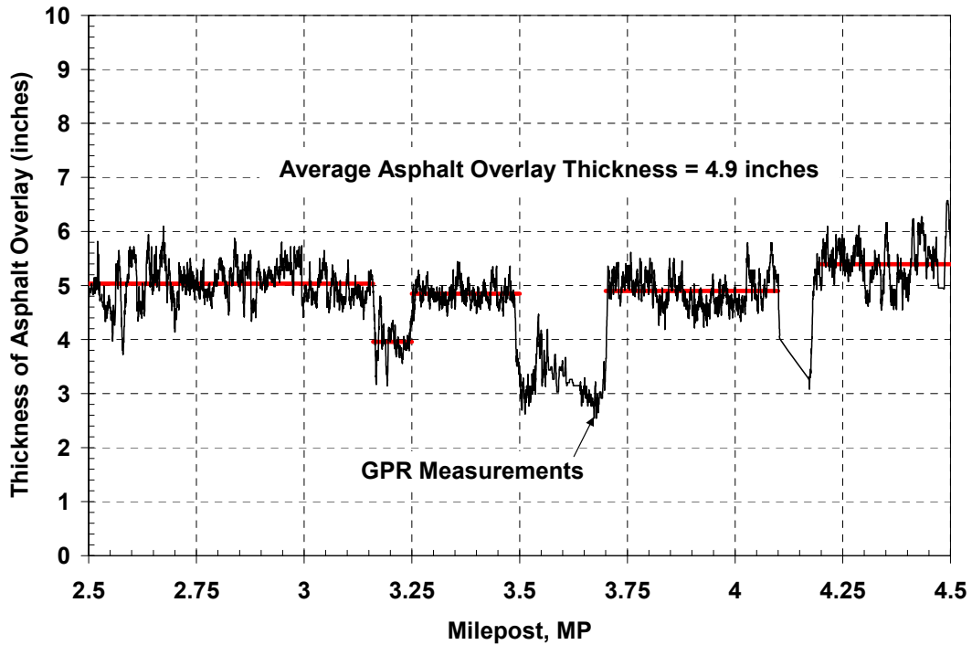
Figure 80 – Ground Penetrating Radar (GPR) Test Results for Section #2 of Rt 34N New Jersey
