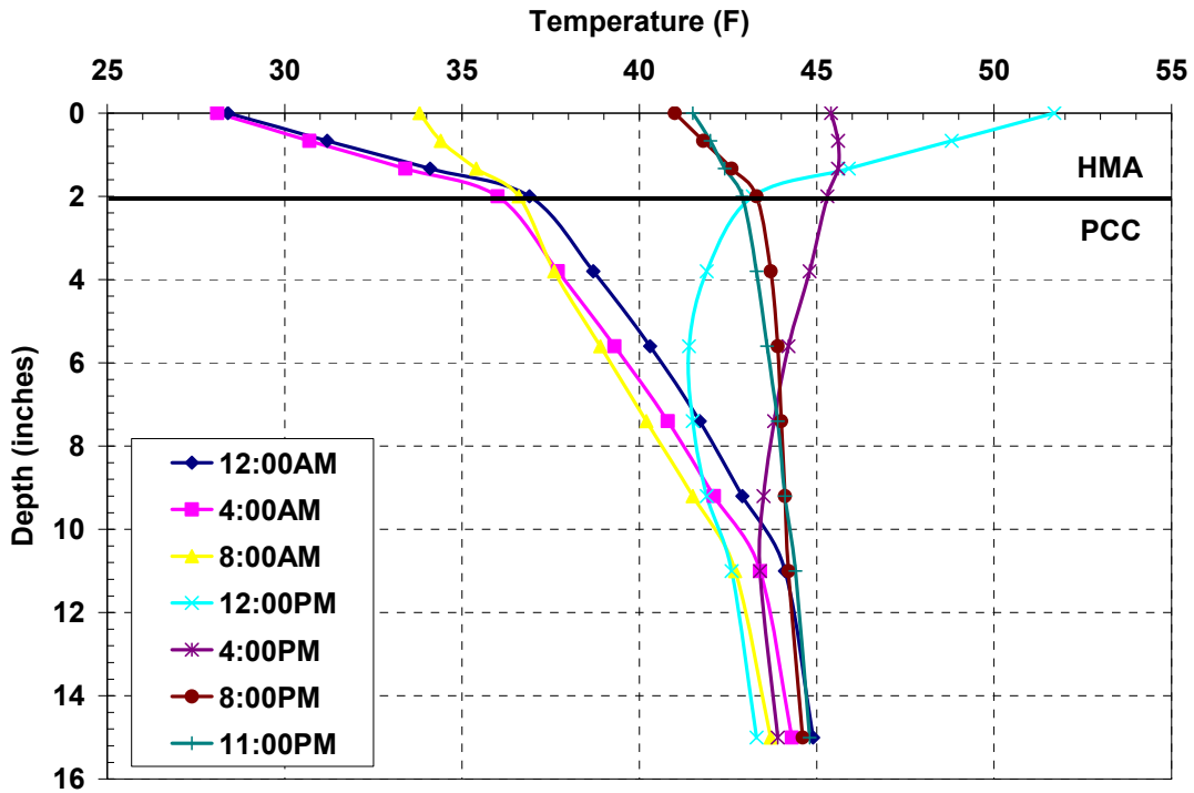
Figure 57 – Predicted Temperature Profiles for 2-Inch Overlay on I-495 MA
