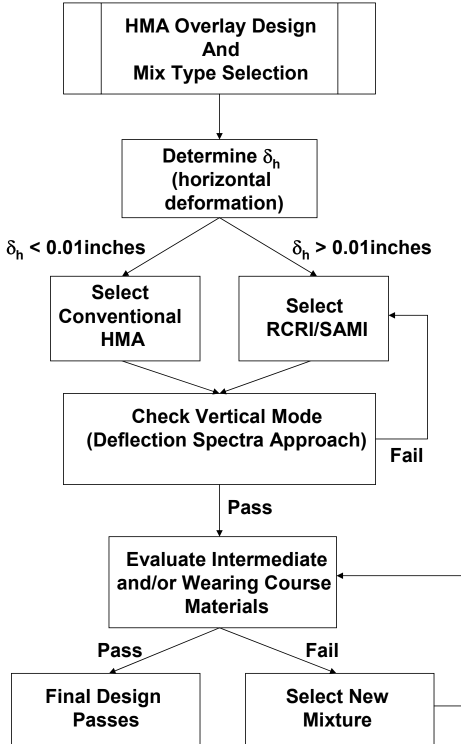
Figure 102 – Flowchart for Hot Mix Asphalt Overlay Design and Mixture Selection
