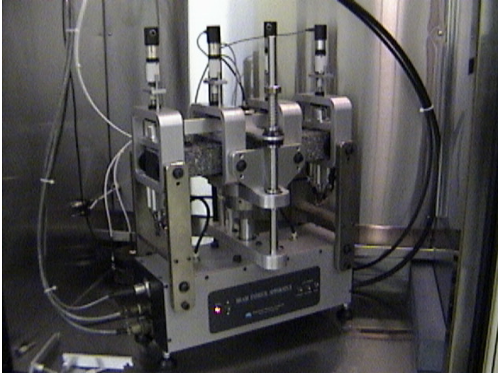
Figure 62 – Flexural Beam Fatigue Device for AASHTO T321
