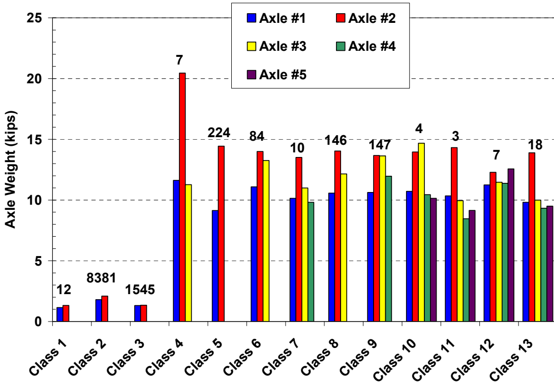
Figure 43 – Axle Load Spectra for Rt 202S
