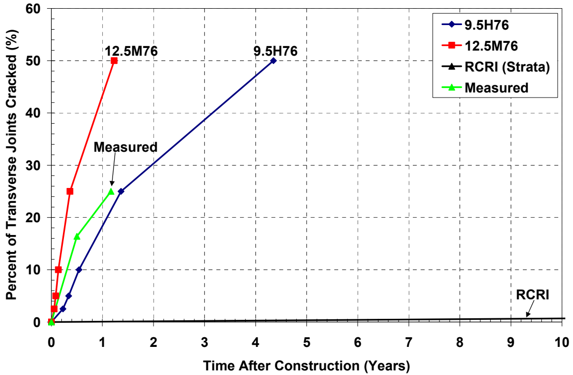
Figure 83 – Predicted versus Measured Reflective Cracking of Test Section #1 on Rt 34N New Jersey
