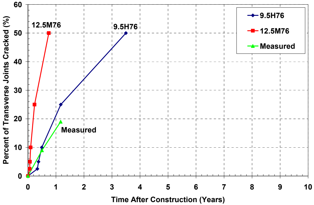
Figure 84 – Predicted versus Measured Reflective Cracking of Test Section #2 on Rt 34N New Jersey
