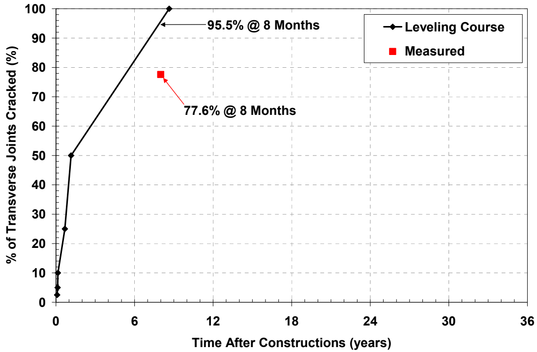
Figure 92 – Predicted versus Measured Reflective Cracking of the 2-Inch Overlay Test Section on I495 in Massachusetts
