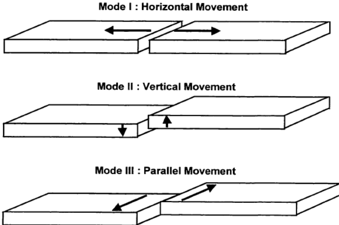
Figure 2 – Movements in Underlying Pavement Layers that Contribute to Reflective Cracking (After Mukhtar and Dempsey, 1996)
