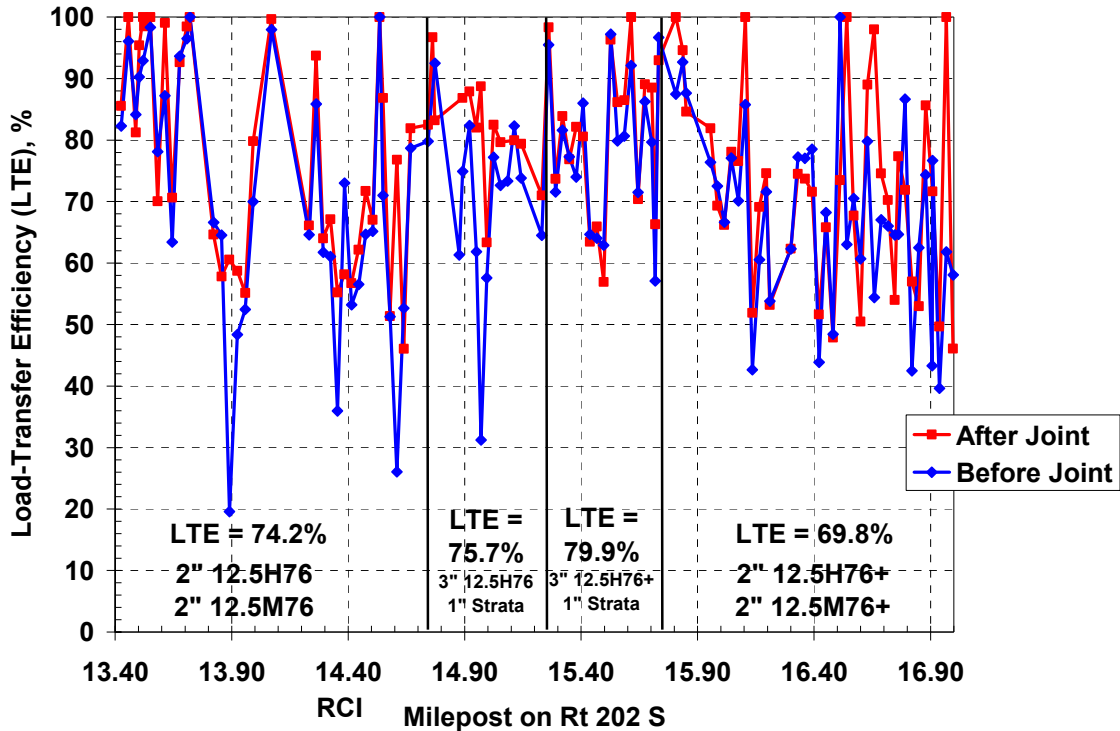
Figure 45 – Load Transfer Efficiency (LTE) of the Different Test Sections on Rt. 202S
