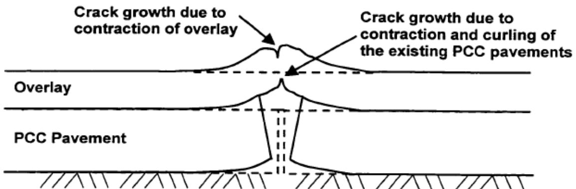
Figure 4 – Crack Growth in HMA Overlay Due to Excessive Curling Forces (After Kohale and Lytton, 2000)
