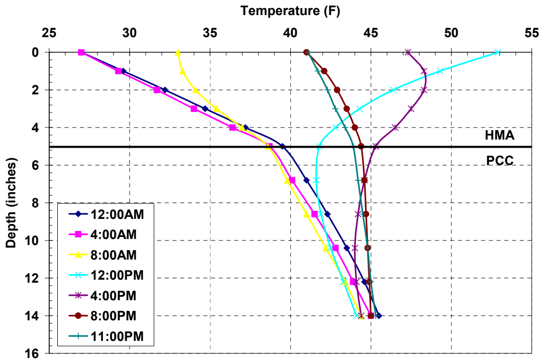
Figure 58 – Predicted Temperature Profiles for 5-Inch Overlay on I-495 MA
