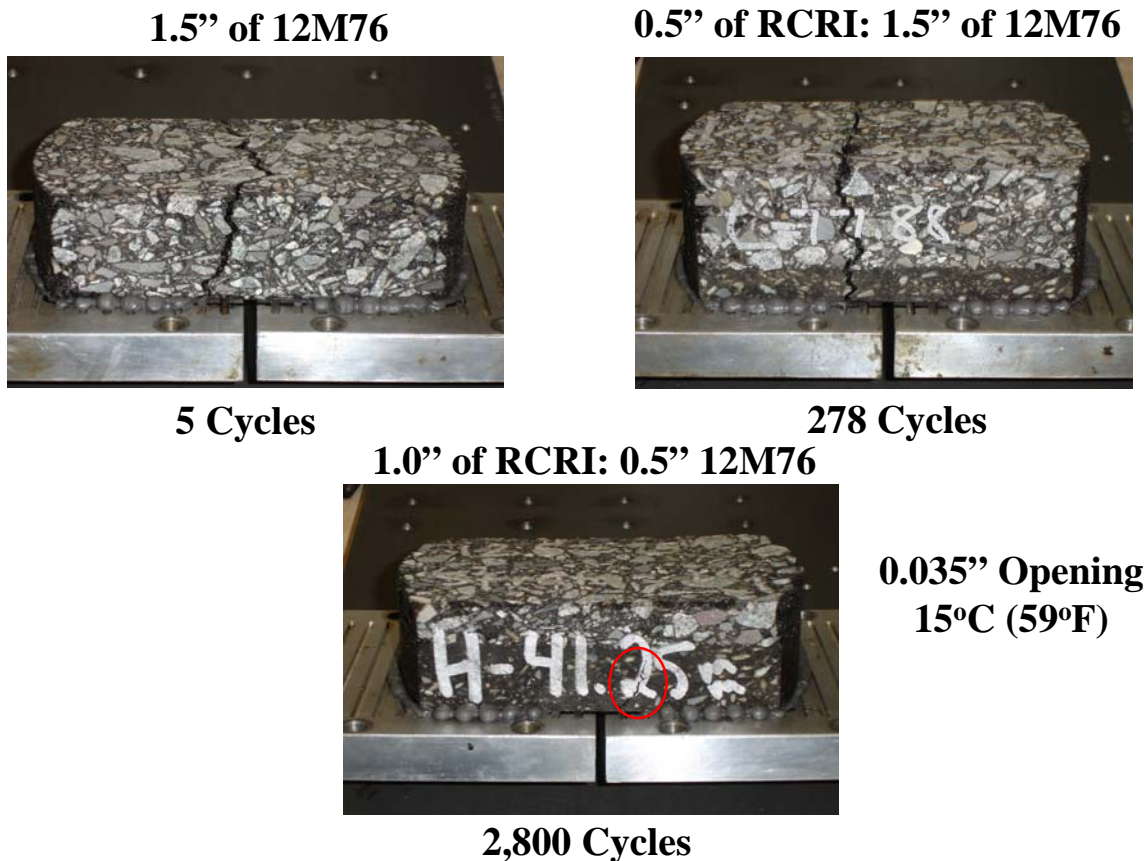
Figure 101 - Assessing RCRI Horizontal Strain Absorption and Thickness Impact on Fatigue Life Using the TTI Overlay Tester
