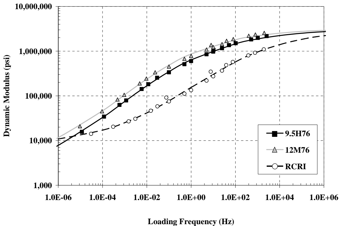
Figure 73 – Dynamic Modulus Test Results of Asphalt Mixtures on Rt 34N, New Jersey
