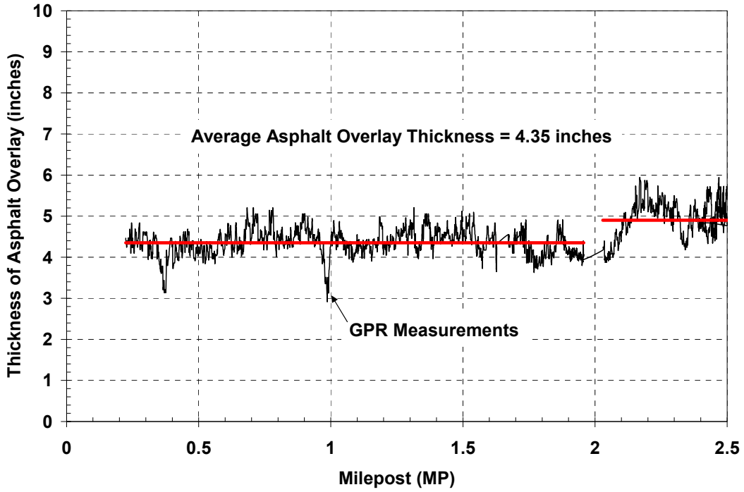
Figure 79 – Ground Penetrating Radar (GPR) Test Results for Section #1 of Rt 34N New Jersey
