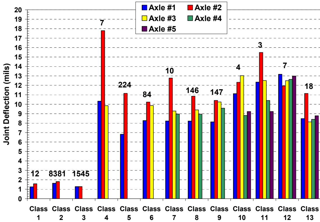
Figure 47 – PCC Vertical Joint Deflection Spectra for Test Section #2 (Rt 202S)
