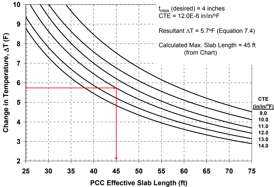
Figure 100 – Example of Using Proposed Guideline to Limit Horizontal Deformation-Related Fatigue Cracking – Determining Maximum Slab Length
