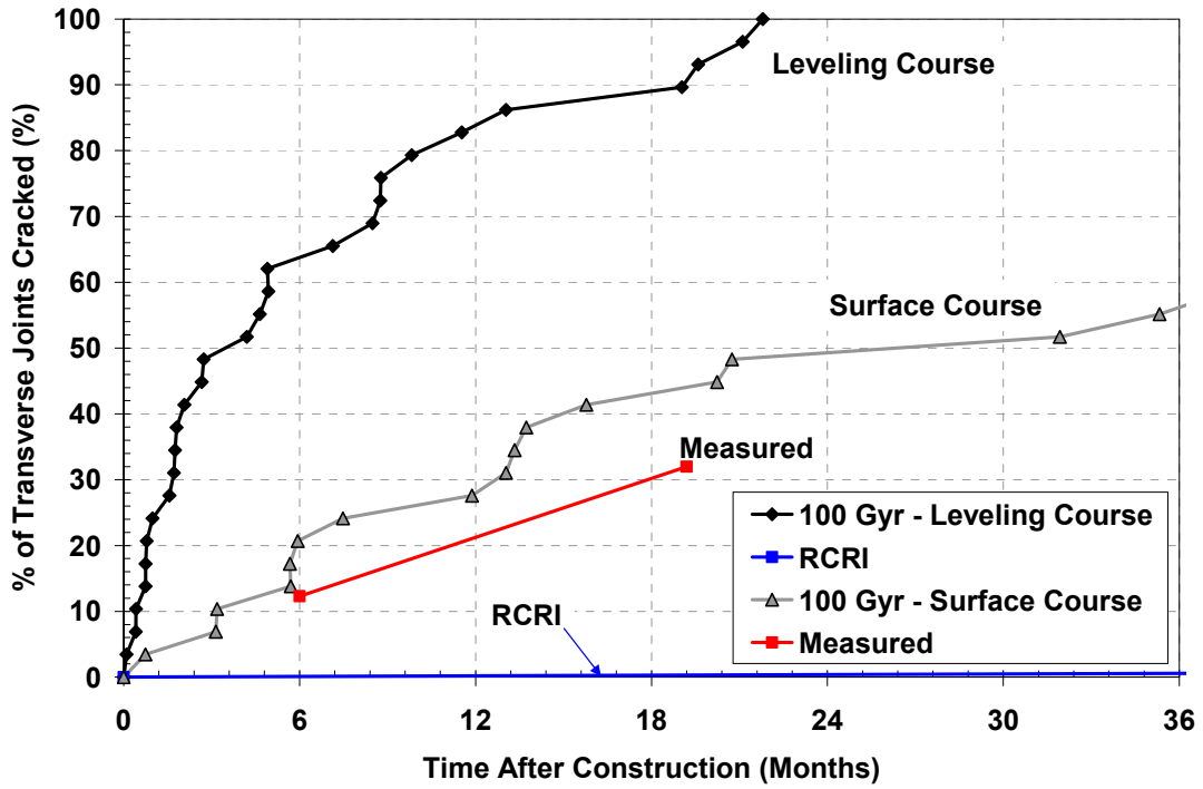
Figure 95 – Predicted versus Measured Reflective Cracking of the 100 Gyration Surface Course Mix on I476 in Pennsylvania
