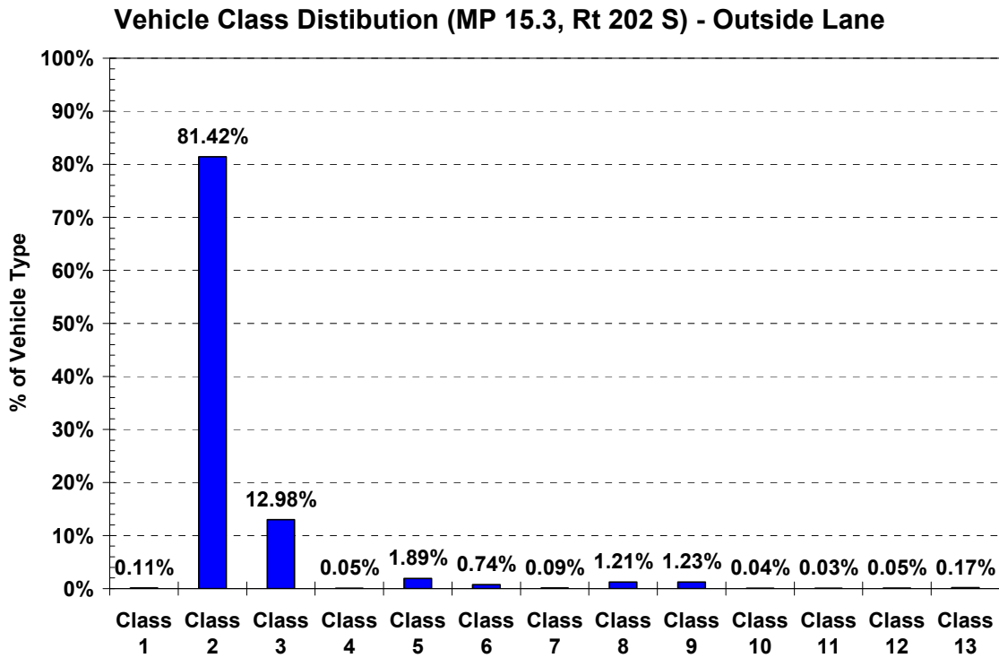
Figure 41 – Vehicle Class Distribution for Rt 202S
