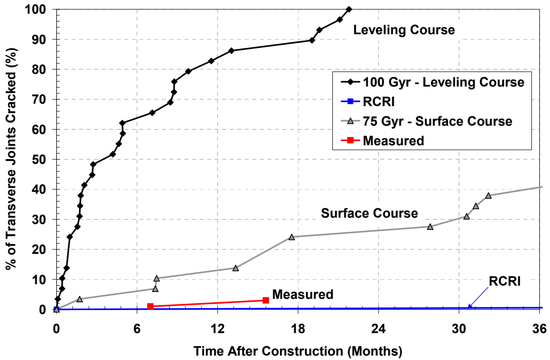
Figure 96 – Predicted versus Measured Reflective Cracking of the 75 Gyration Surface Course Mix on I476 in Pennsylvania
