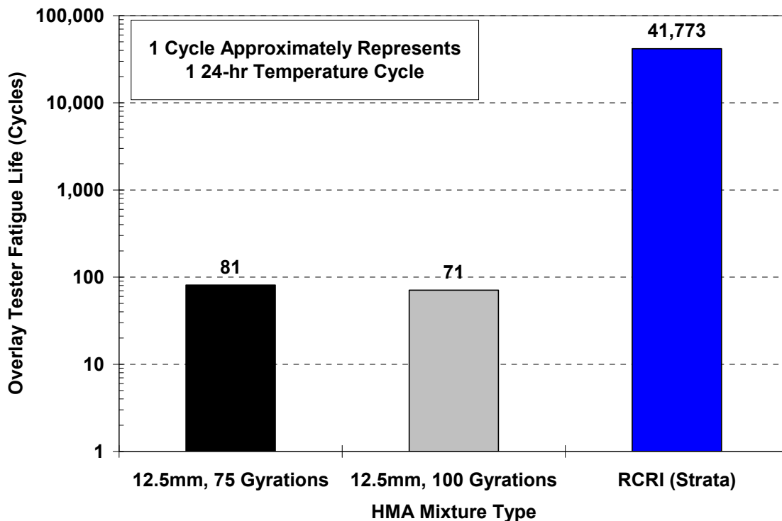
Figure 71 – TTI Overlay Tester Results for HMA Mixtures on I476, Pennsylvania
