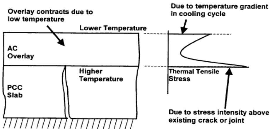
(b) Contraction Effect of AC Overlay
