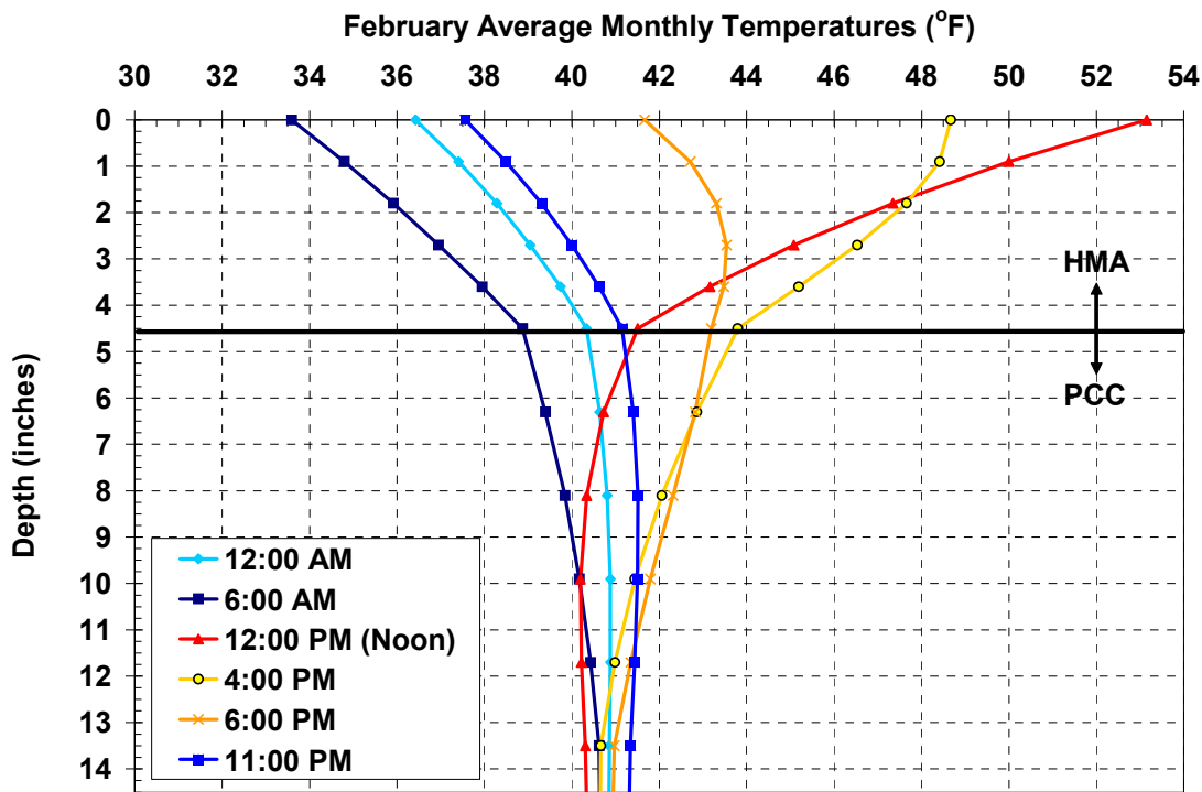
Figure 37 – An Example of the Predicted Thermal Distribution on Rt 34N in New Jersey
