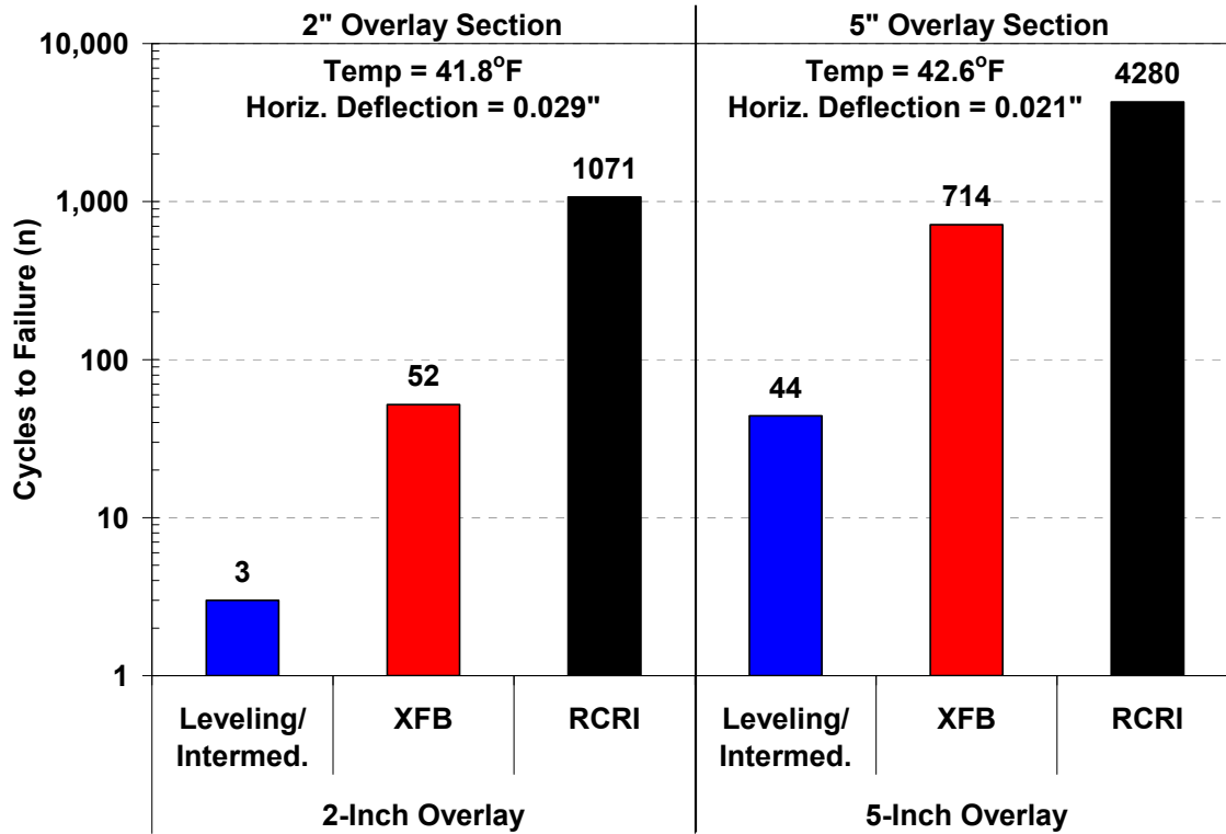
Figure 70 – Overlay Tester Test Results for 2” and 5” Overlay Sections
