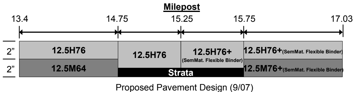
Figure 86 – Cross Section of Research Test Sections on Rt. 202S in New Jersey
