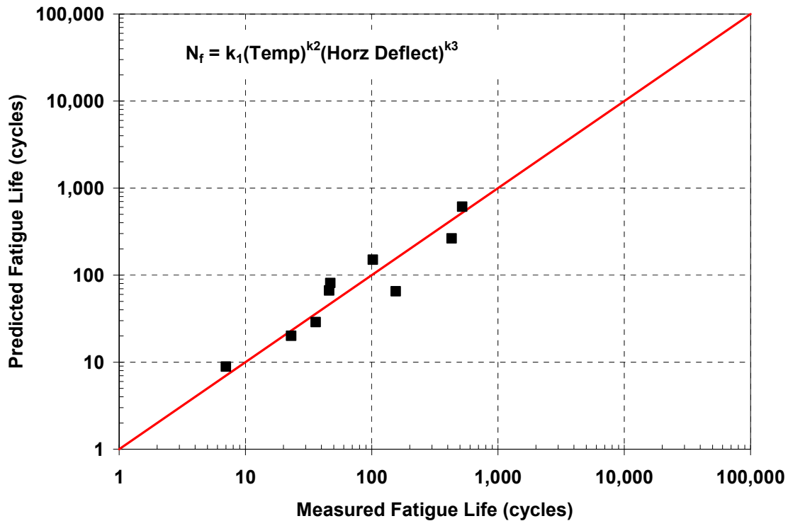
Figure 72 – Example of Horizontal Fatigue Life Determined in the TTI Overlay Tester
