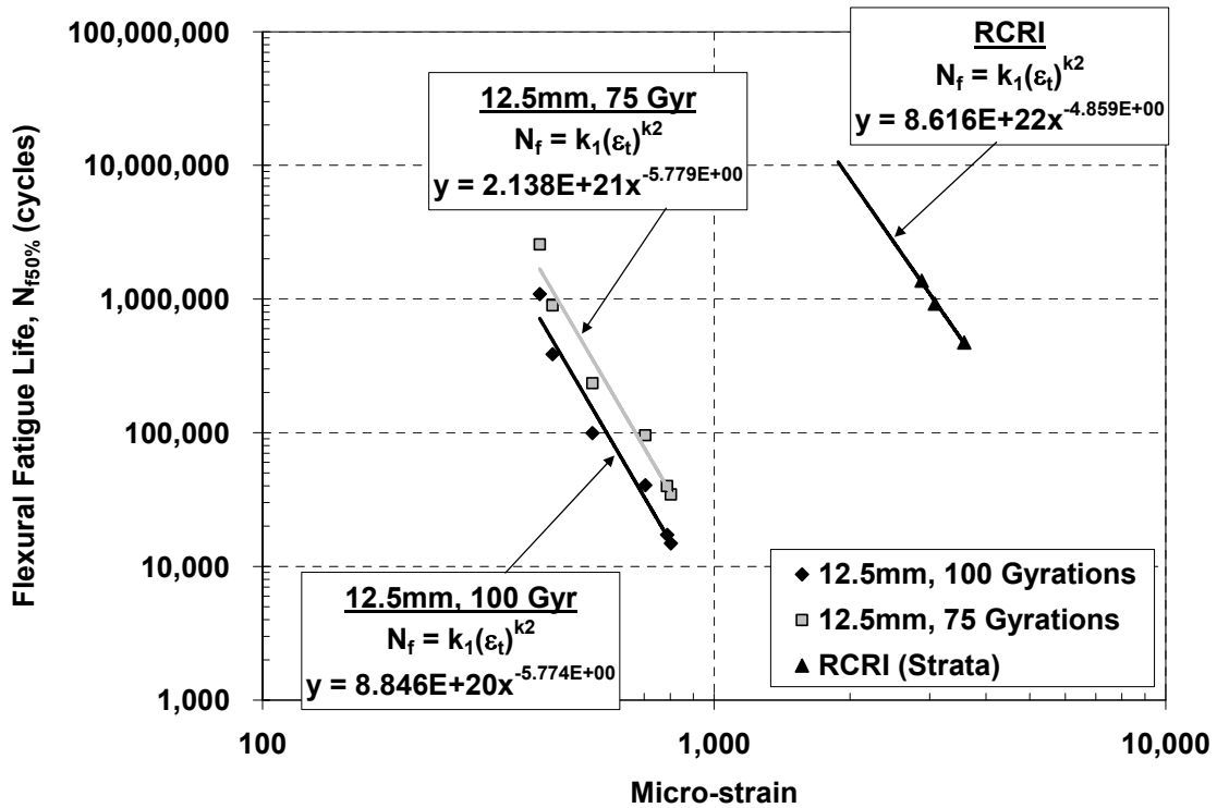
Figure 66 – Flexural Beam Fatigue Life of Asphalt Mixtures from I476, Pennsylvania
