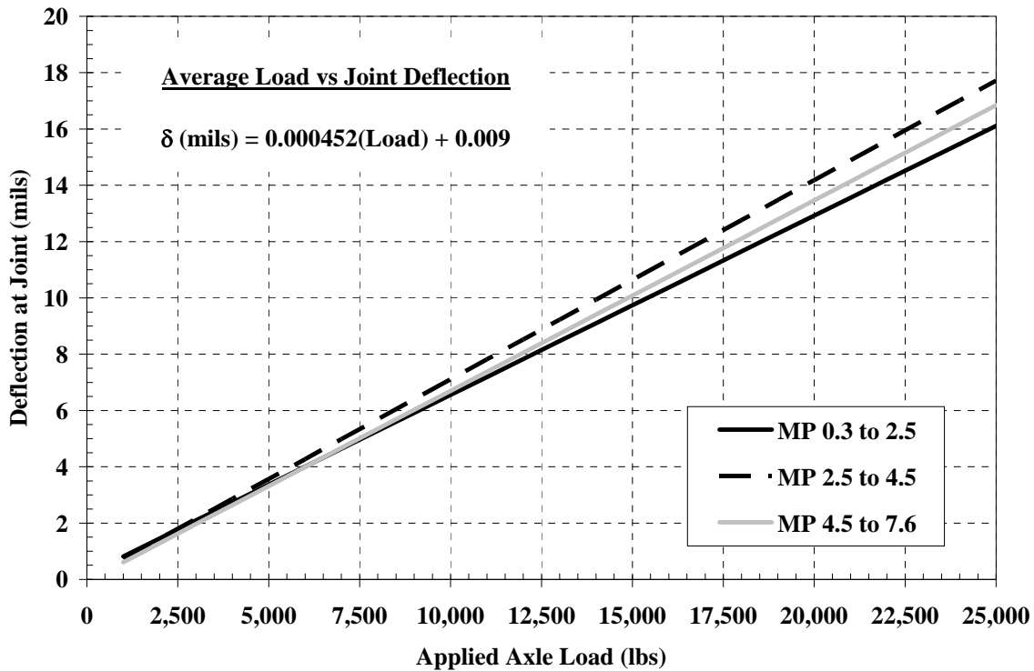
Figure 76 – Relationship Between FWD Load Magnitude and Vertical Deflection at PCC Joint for Rt 34N New Jersey Test Section
