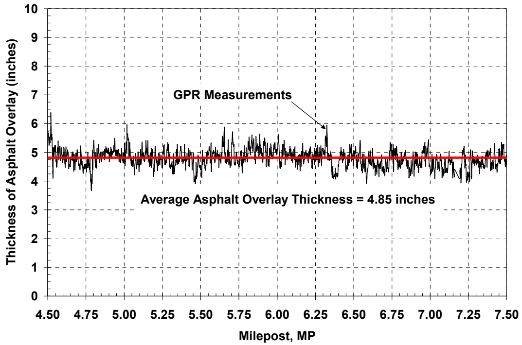
Figure 81 – Ground Penetrating Radar (GPR) Test Results for Section #3 of Rt 34N New Jersey
