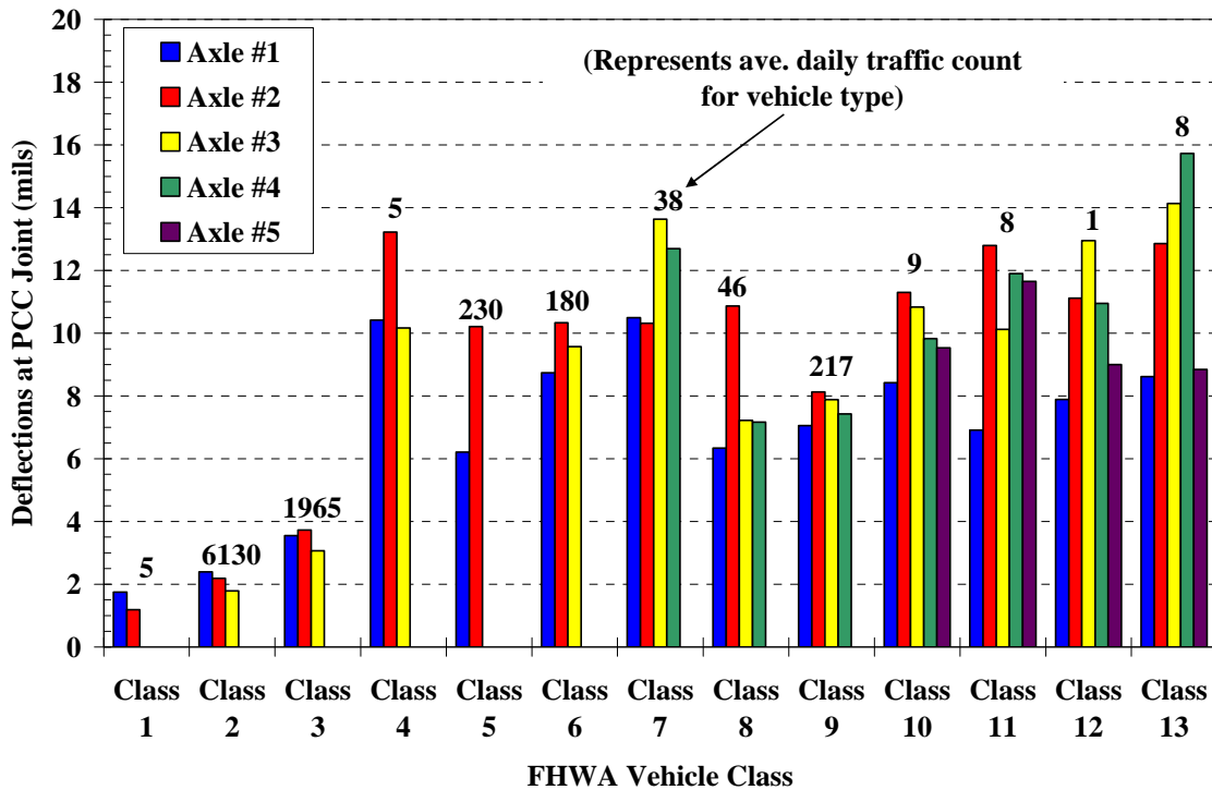
Figure 77 – PCC Vertical Joint Deflection Spectra for Test Section #1
