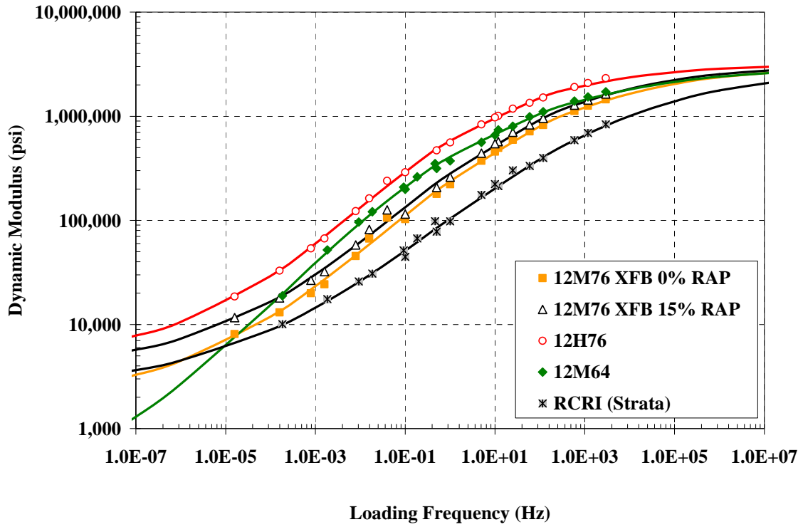
Figure 75 – Master Stiffness Curves of Asphalt Mixtures from the Rt 202S New Jersey Test Section
