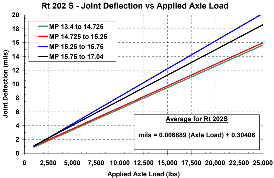
Figure 46 – PCC Joint Deflection vs Applied Axle Load for Rt 202S in New Jersey
