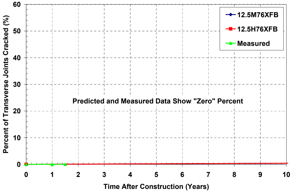
Figure 91 – Predicted versus Measured Reflective Cracking of Test Section MP 15.75 to 17 of Rt 202S New Jersey
