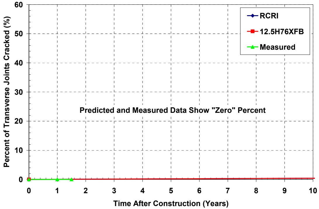
Figure 90 – Predicted versus Measured Reflective Cracking of Test Section MP 15.25 to 15.75 of Rt 202S New Jersey
