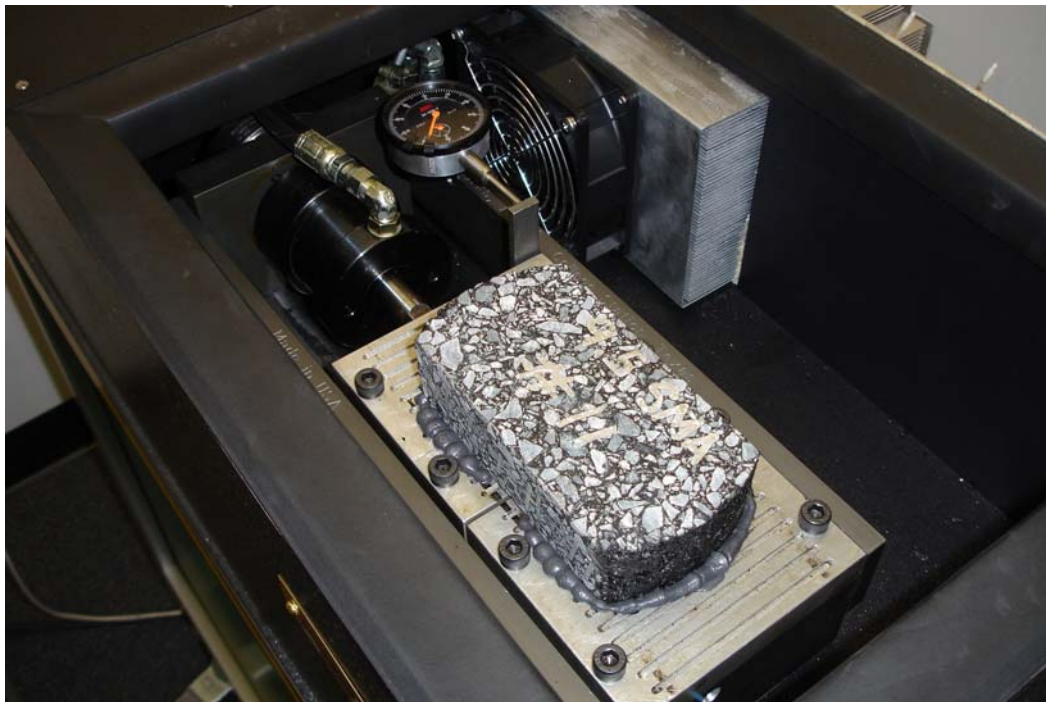
Figure 67 – Photo of the TTI Overlay Tester
