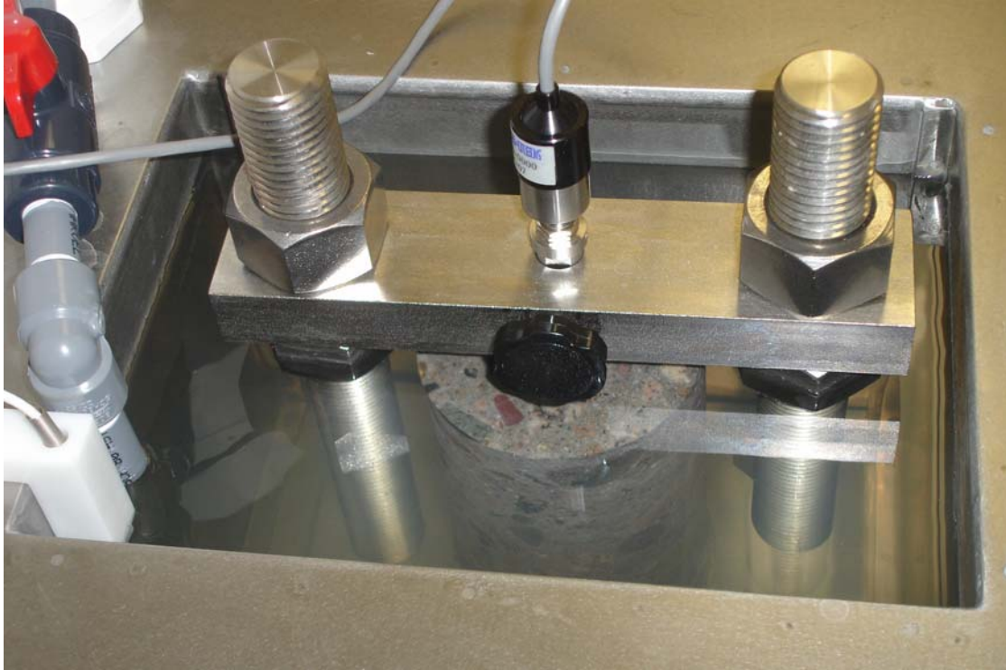
Figure 25 – Coefficient of Thermal Expansion Test Device
