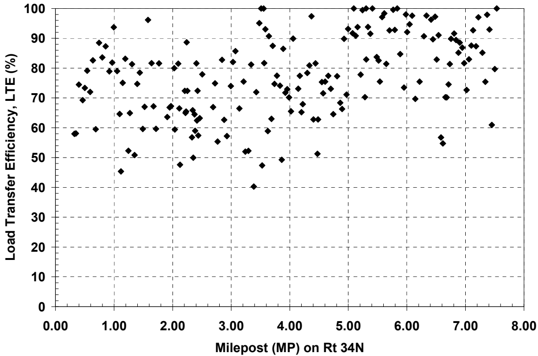
Figure 33 – Load Transfer Efficiency for Rt 34N in New Jersey
