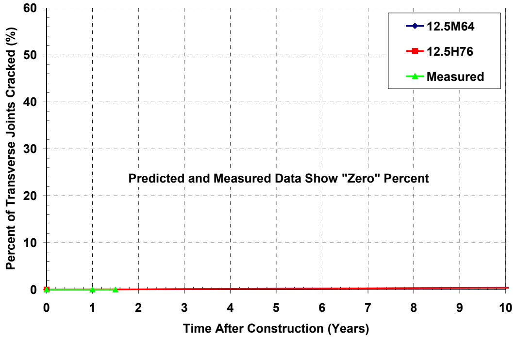
Figure 88 - Predicted versus Measured Reflective Cracking of Test Section mp 13.4 to 14.75 of Rt 202S New Jersey
