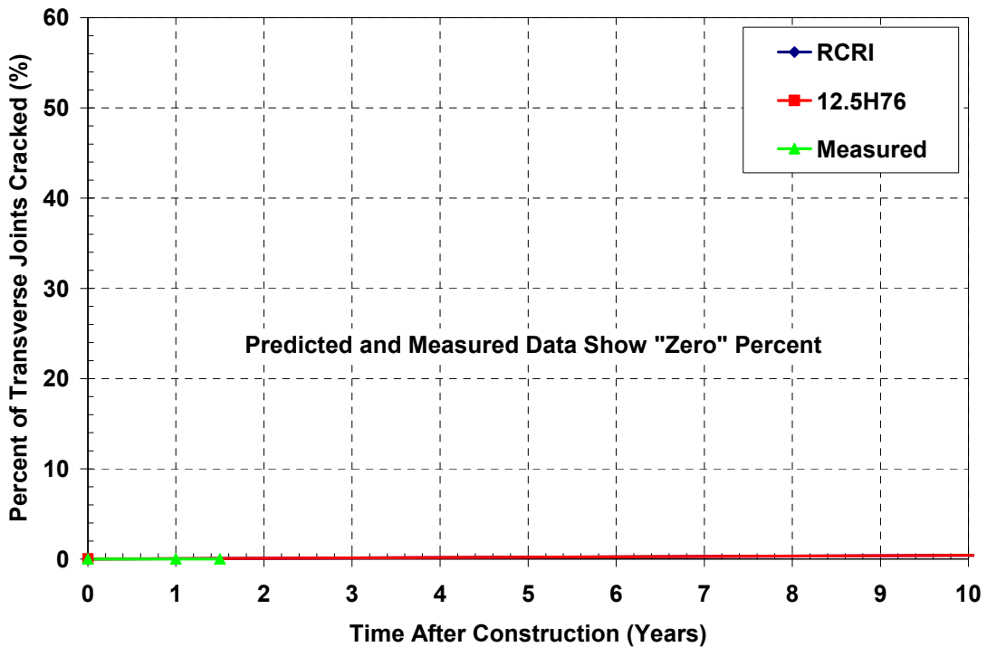
Figure 89 – Predicted versus Measured Reflective Cracking of Test Section MP 14.75 to 15.25 of Rt 202S New Jersey
