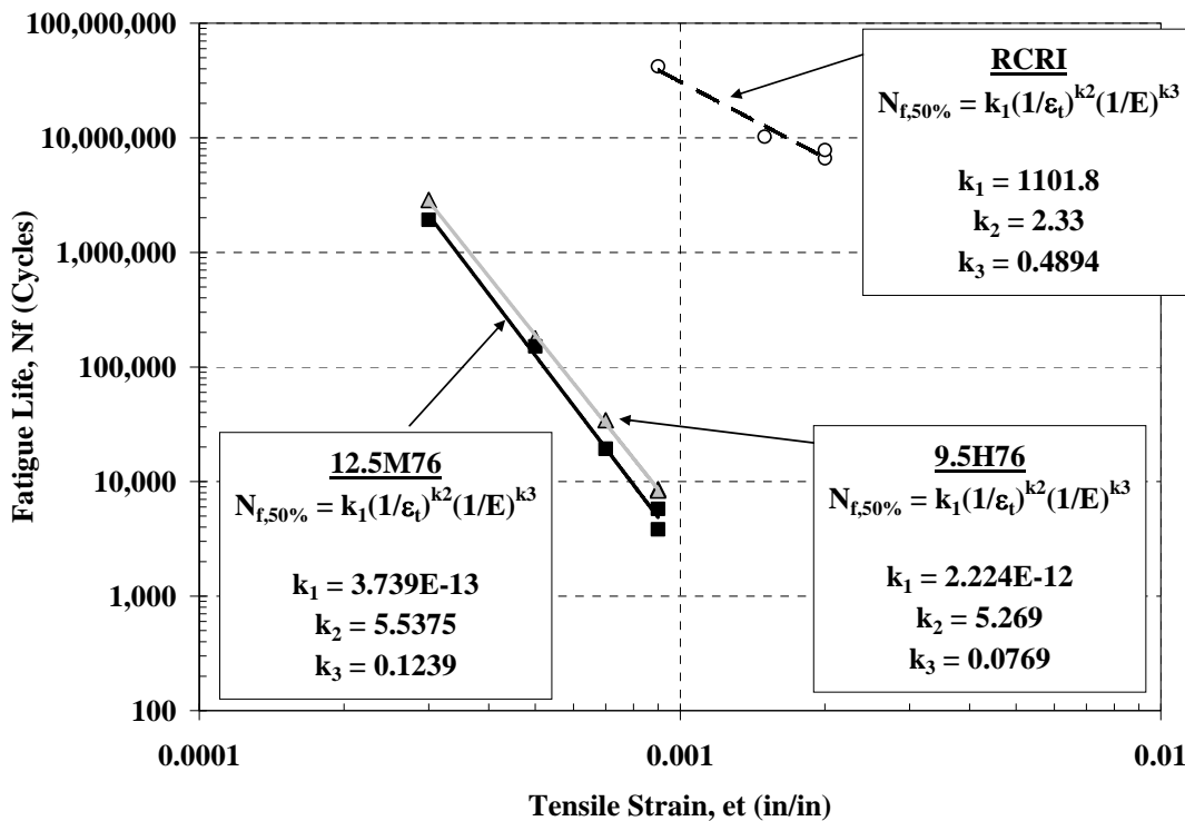
Figure 63 – Flexural Beam Fatigue Life of Asphalt Mixture from Rt 34N, New Jersey
