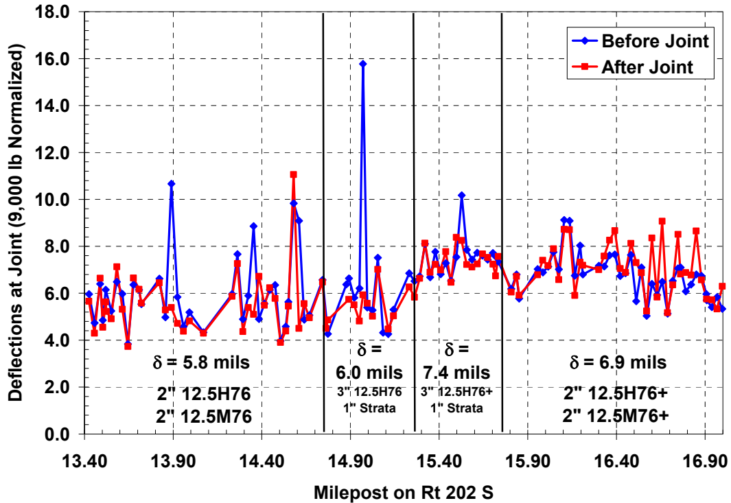
Figure 44 – Vertical Deflection at the PCC Joint/Crack Normalized to 9,000 lbs
