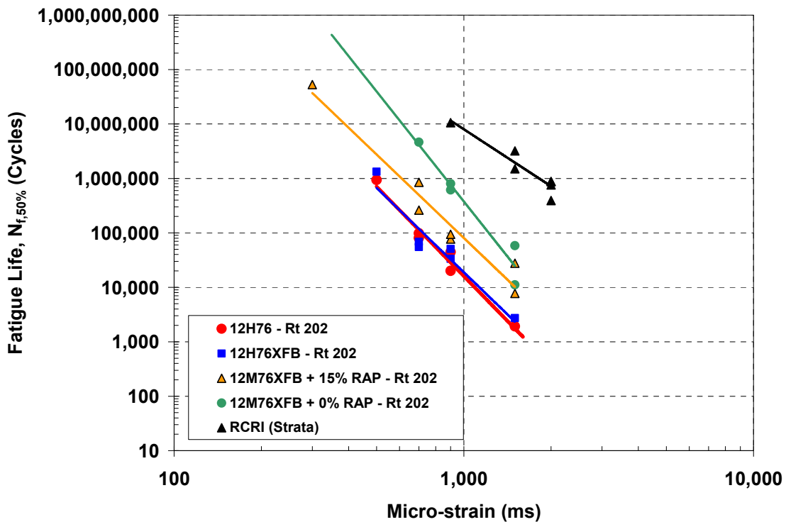
Figure 64 – Flexural Beam Fatigue Life of Asphalt Mixture from Rt 202S, New Jersey
