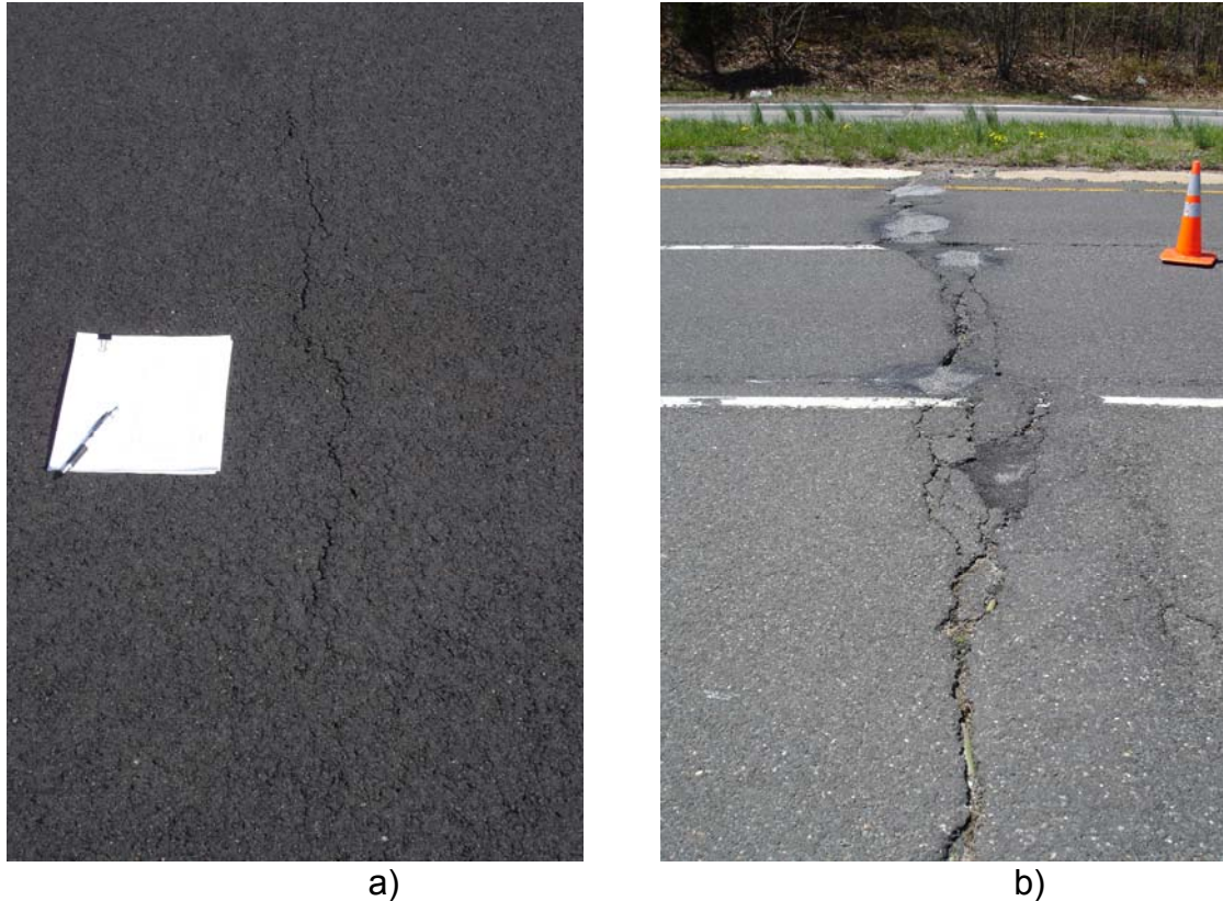
Figure 1 – Reflective Cracking on Existing Composite Pavement, a) Early Reflective Cracking and b) Reflective Cracking After 8 Years of Service
