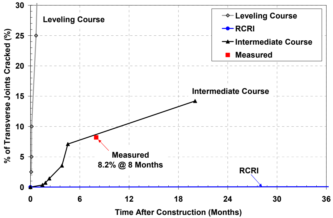
Figure 93 – Predicted versus Measured Reflective Cracking of the 5-Inch Overlay Test Section on I495 in Massachusetts
