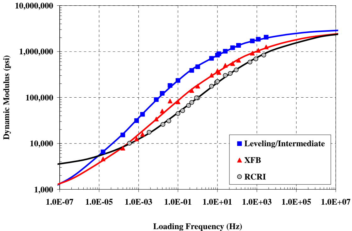
Figure 74 – Master Stiffness Curves of the Asphalt Mixtures from I495 Massachusetts Test Section
