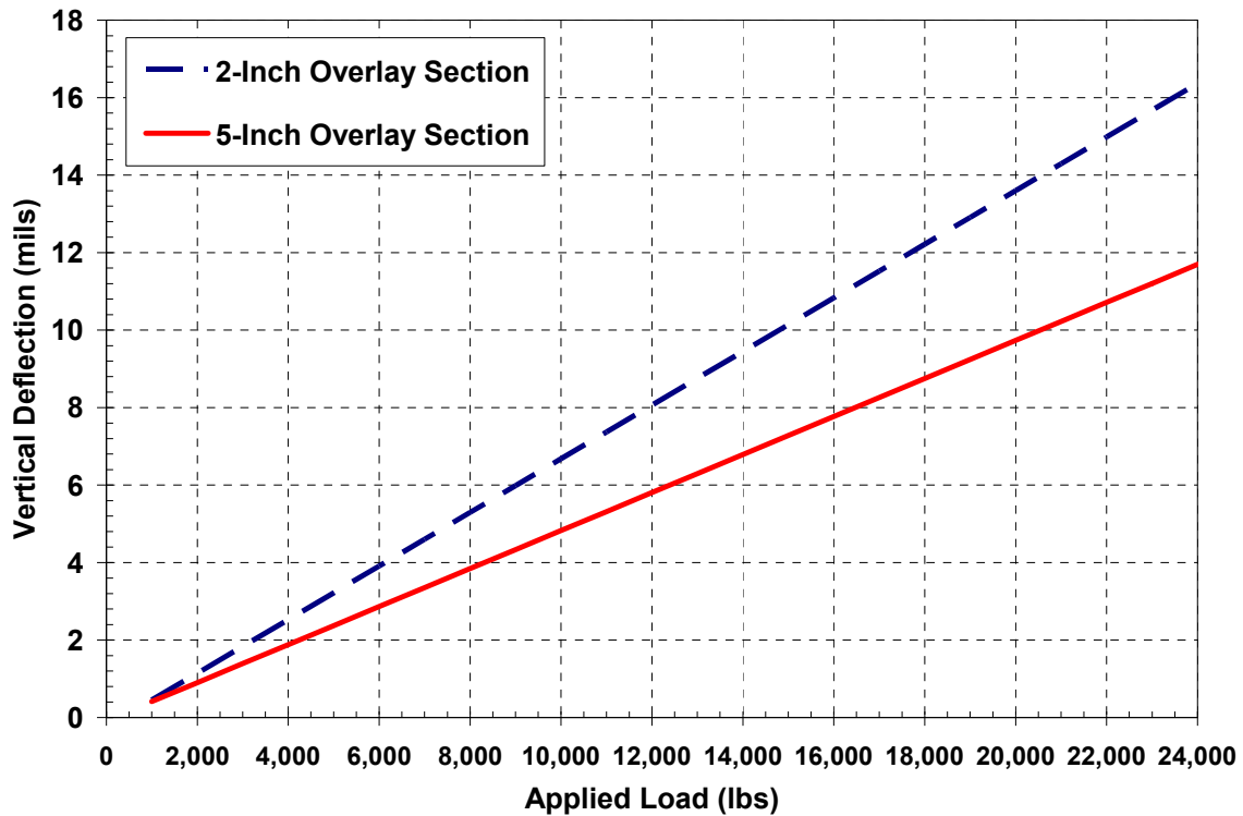
Figure 55 – Applied Load vs PCC Vertical Deflection Relationship for Interstate 495
