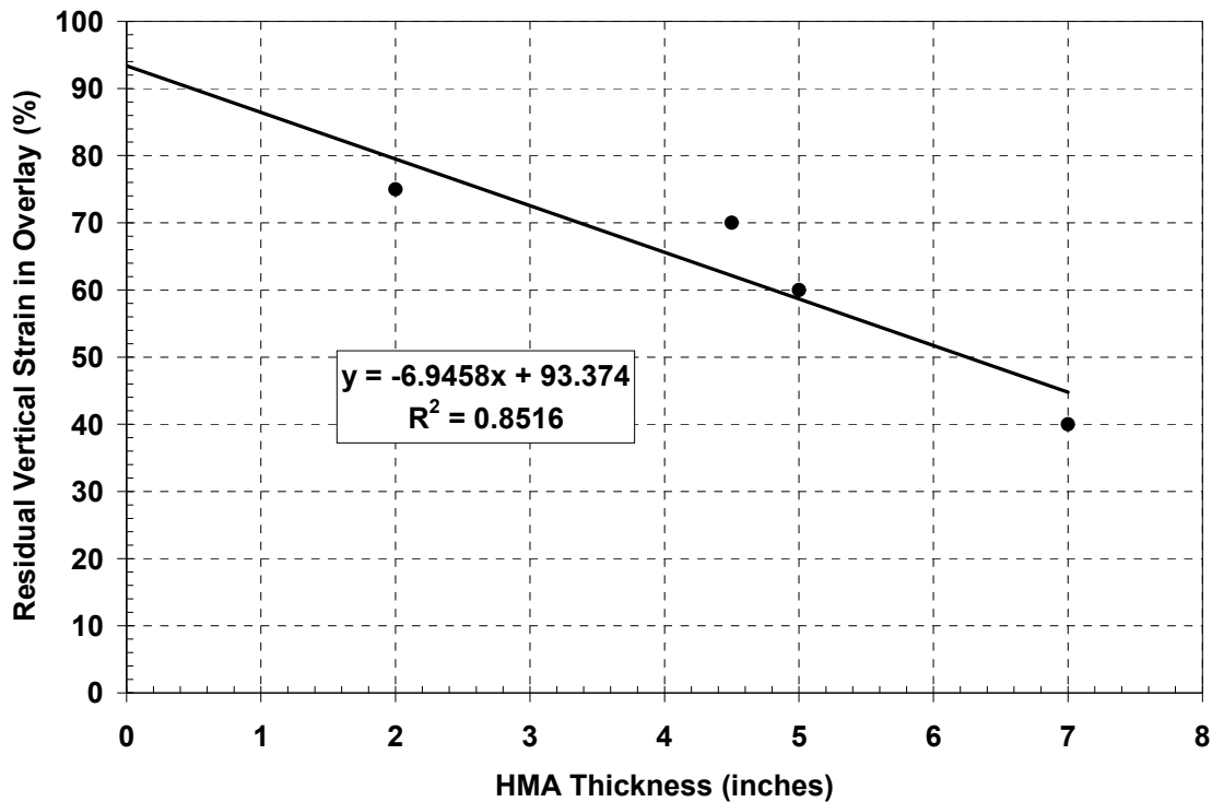
Figure 78 – Determination of Residual Vertical Strain from FWD Field Testing
