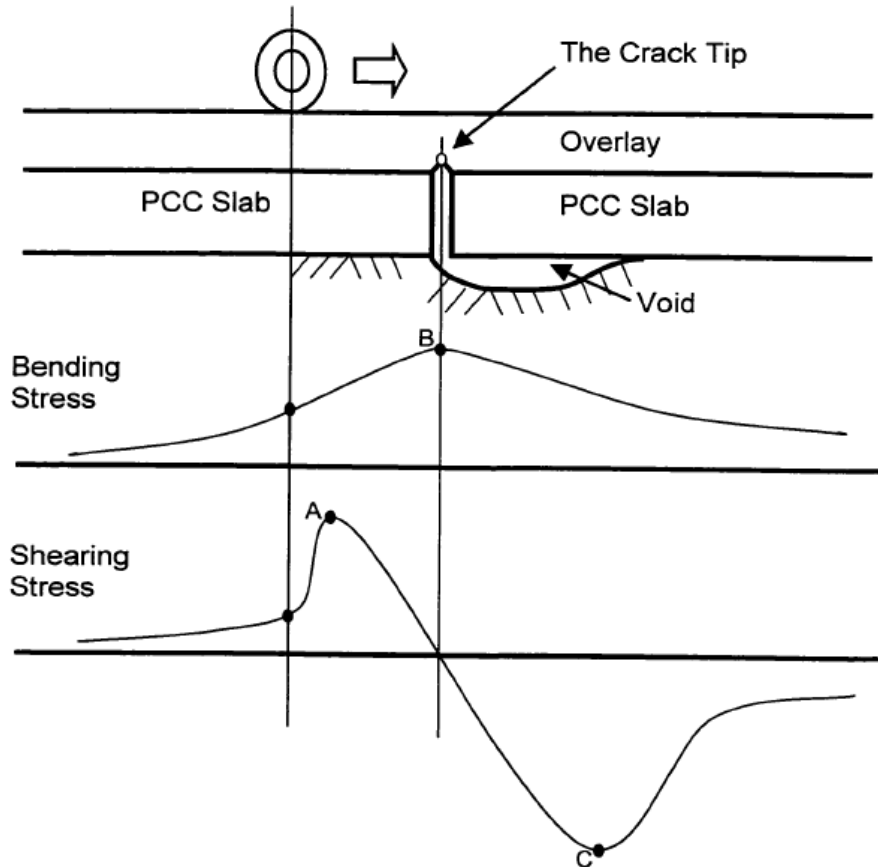
Figure 8 – Stresses Developed in the Joint/Crack Area Due to Traffic Loading (After Kohale and Lytton, 2000)
