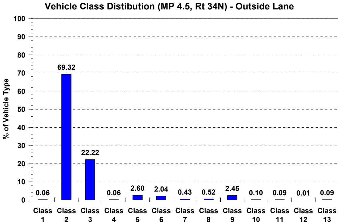
Figure 29 – Vehicle Class Distribution (VCD) for Rt 34N in New Jersey
