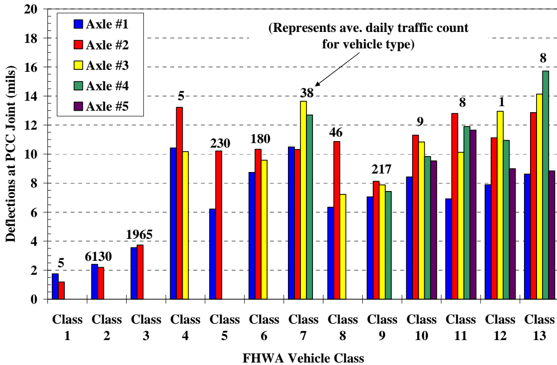
Figure 35 – PCC Vertical Joint Deflection Spectra for Test Section #1
