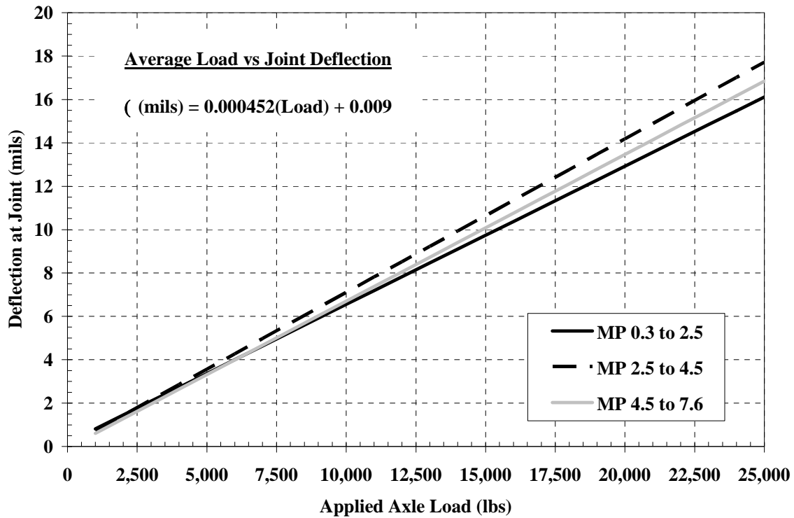
Figure 34 – Applied Load vs Resultant PCC Joint/Crack Vertical Deflection
