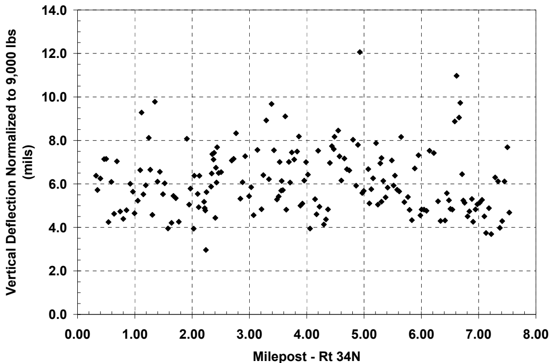
Figure 32 – Vertical Deflections at PCC Joint/Crack
