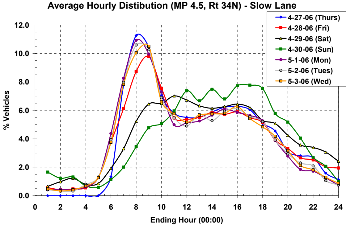
Figure 30 – Hourly Distribution on Rt. 34N in New Jersey
