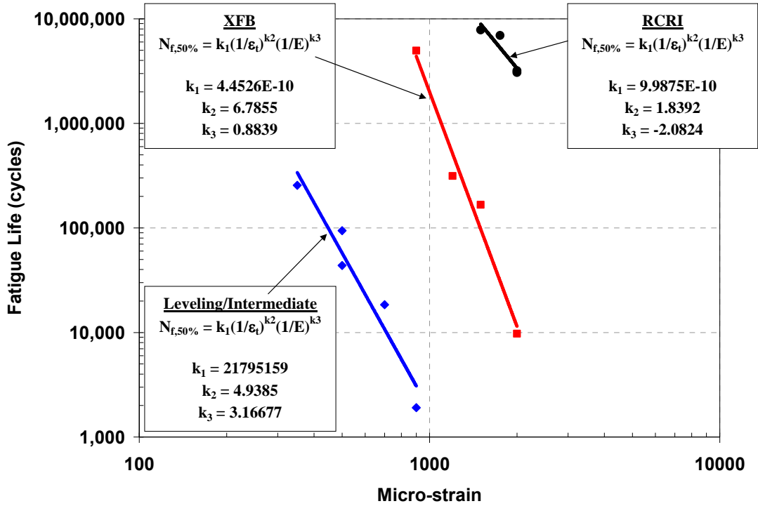
Figure 65 – Flexural Beam Fatigue Life of Asphalt Mixture from I495, Massachusetts
