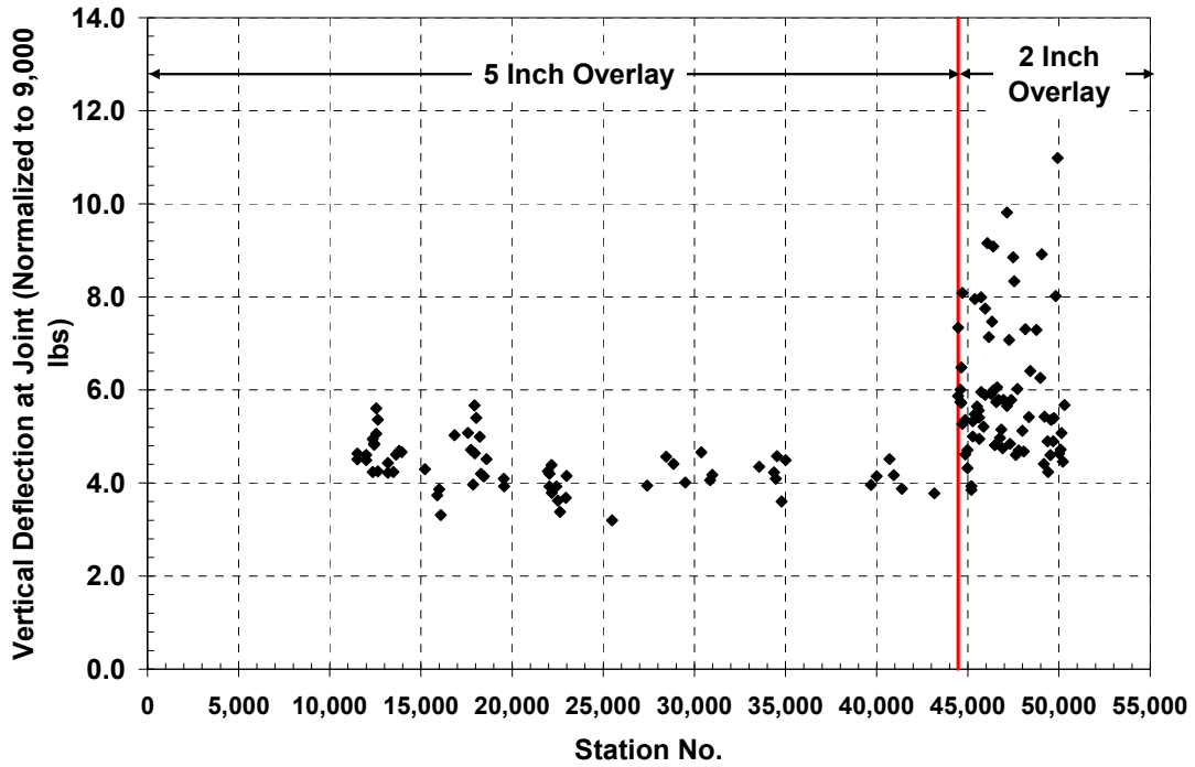
Figure 53 – Vertical Deflection at PCC Joint/Crack Normalized to 9,000 lbs
