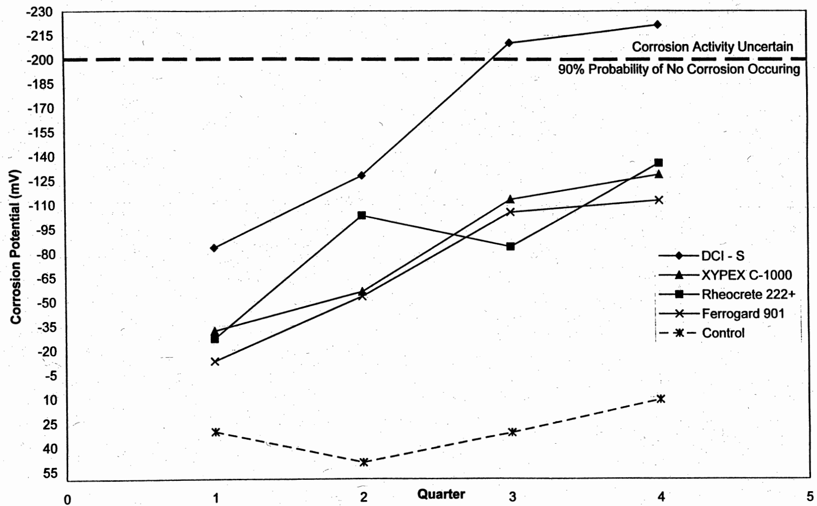
Fig. 4.39: Comparison of Corrosion Inhibitors GECOR 6 Average Corrosion Potential (mV)
