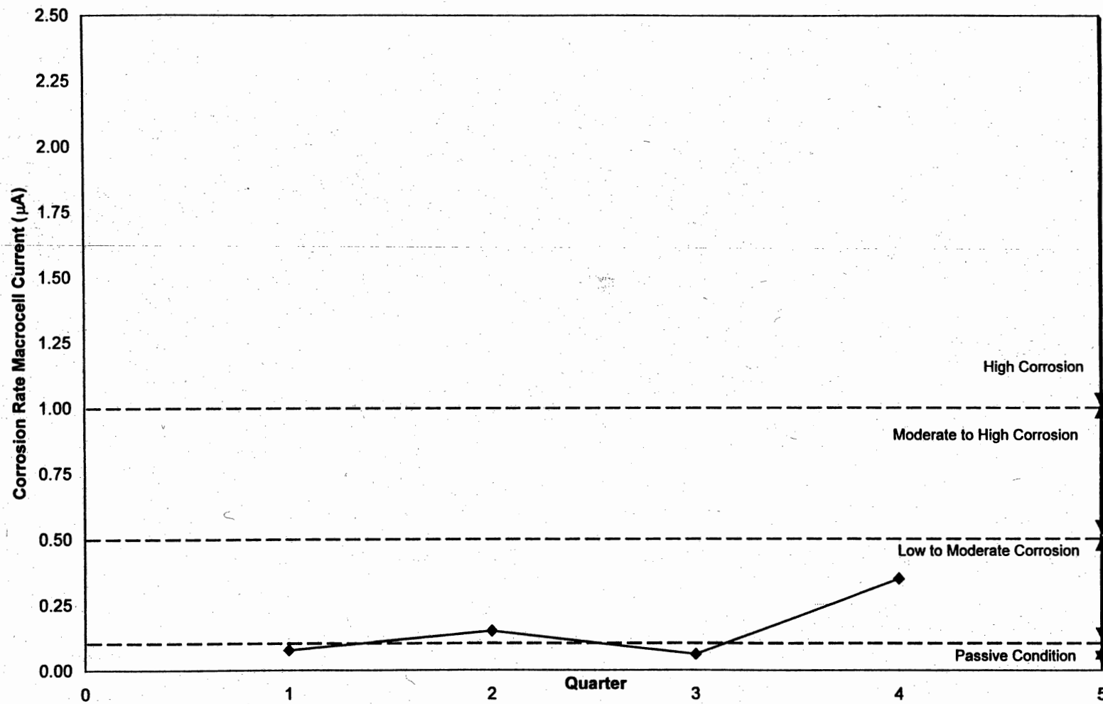
Fig. 4.17: Wyckoff Road Westbound GECOR 6 Average Corrosion Rate Macrocell Current (µA)
