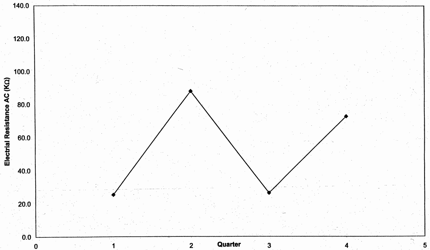
Fig. 4.28: Wyckoff Road Eastbound Average Electrical Resistance AC (KΩ)
