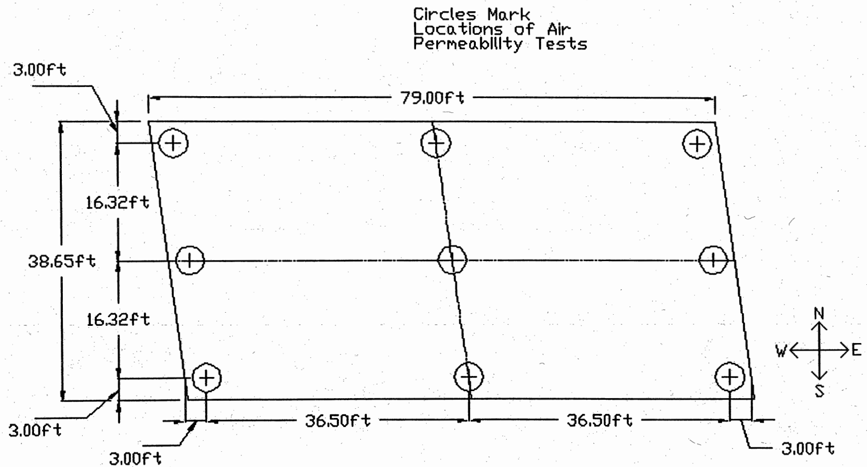
Fig. 3.36: Locations of Surface Air Flow Field Permeability Indicator Readings North Main Street Westbound
