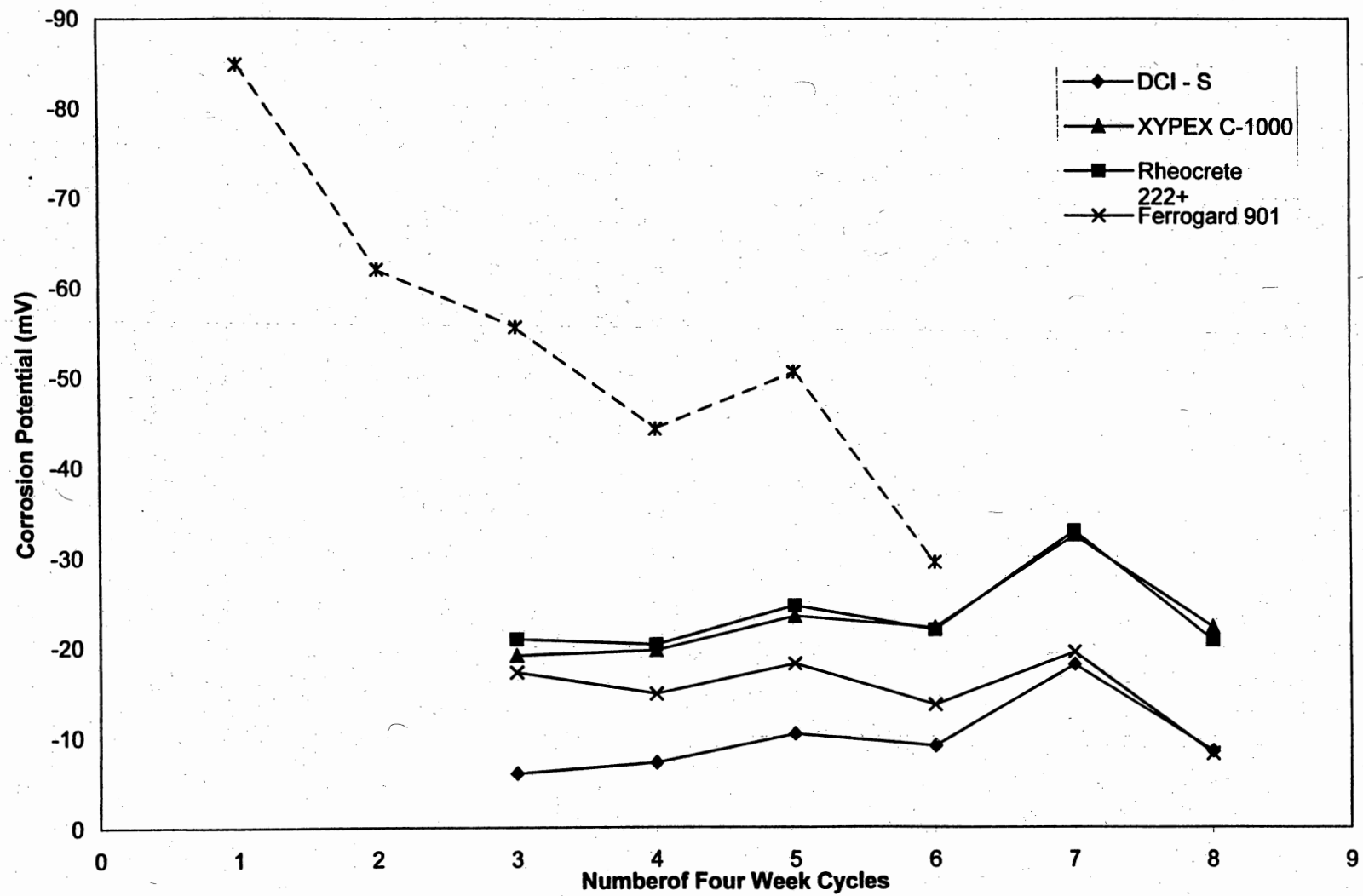
Fig. 4.37: Comparison of Corrosion Inhibitors Minideck Average Corrosion Potential (mV)
