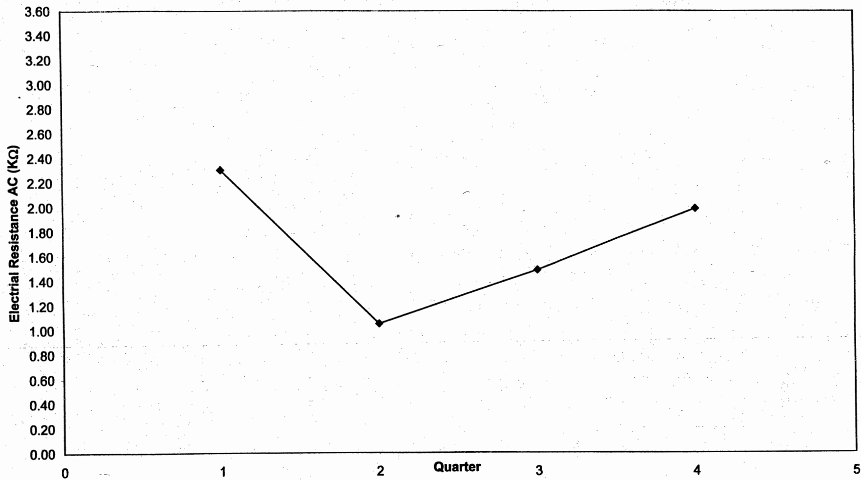
Fig. 4.26: Wyckoff Road Eastbound GECOR 6 Average Electrical Resistance AC (KΩ)
