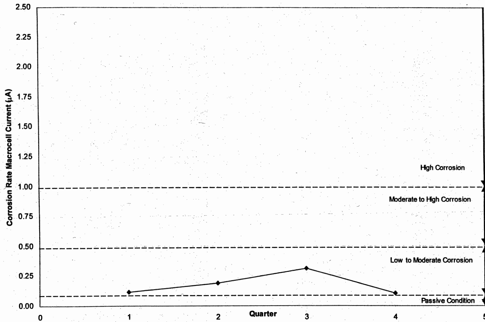
Fig. 4.24: Wyckoff Road Eastbound GECOR 6 Average Corrosion Rate Macrocell Current (μA)
