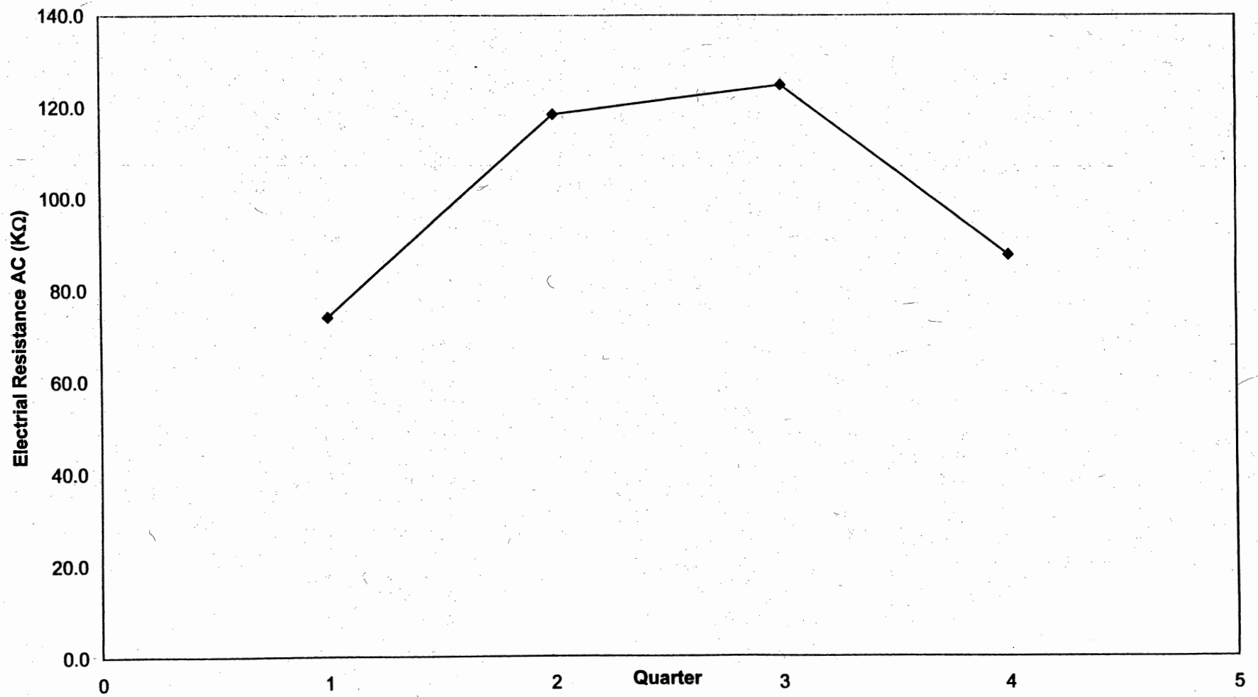
Fig. 4.7: North Main Street Westbound Average Electrical Resistance AC (KΩ)
