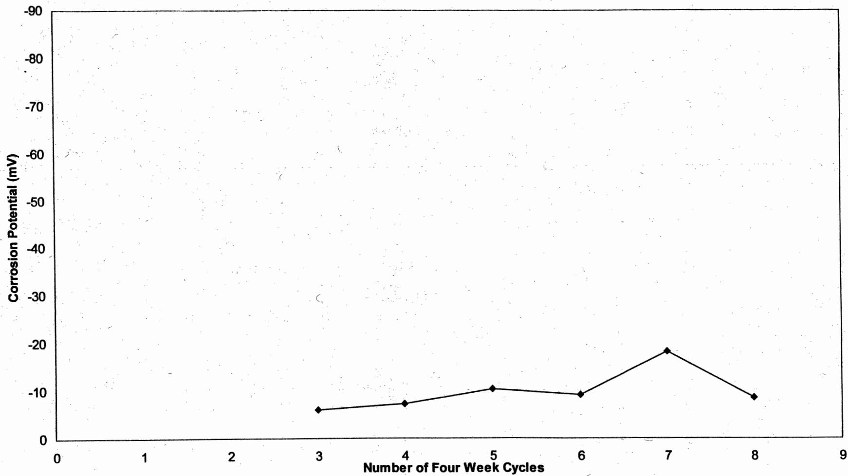
Fig. 4.2: Minideck A - Average Corrosion Potential (mV)
