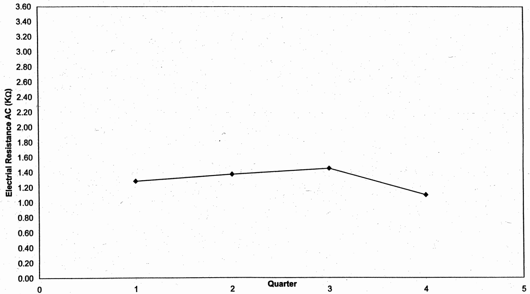
Fig. 4.5: North Main Street Westbound GECOR 6 Average Electrical Resistance AC (KΩ)
