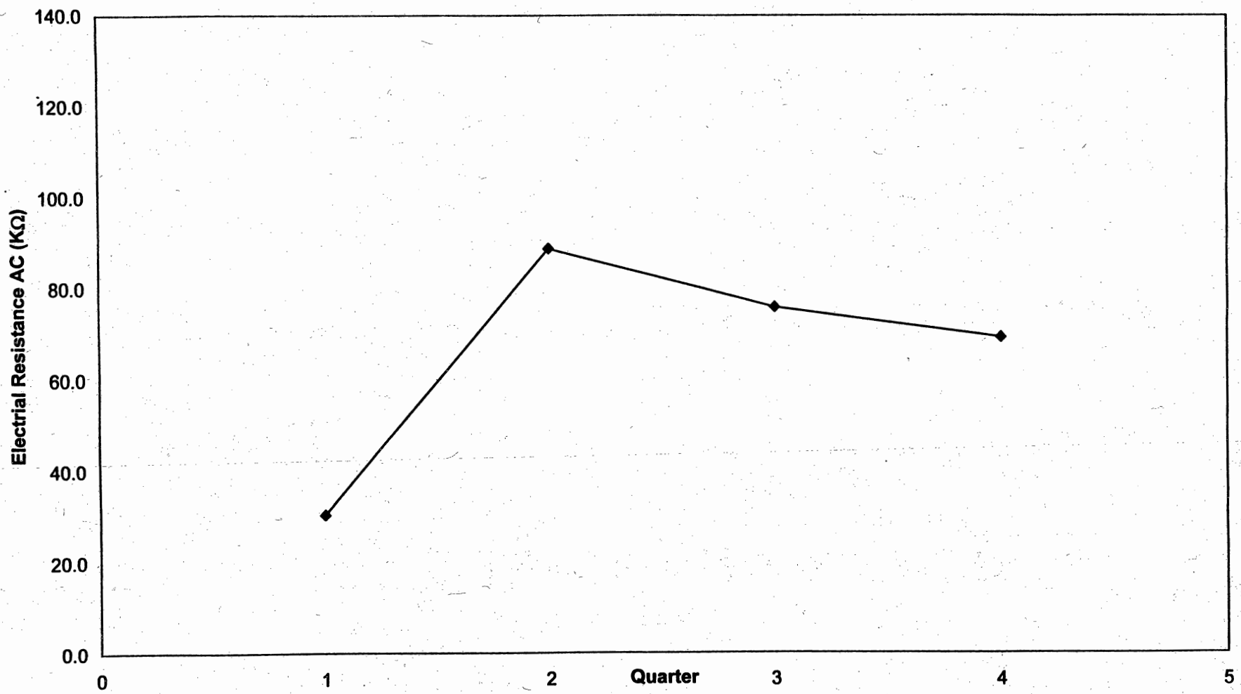
Fig. 4.35: Route 130 Westbound Average Electrical Resistance AC (KΩ)
