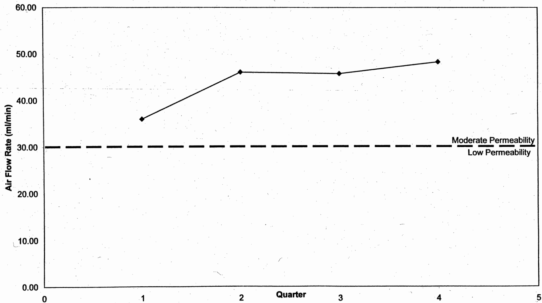
Fig. 4.34: Wyckoff Road Westbound Average Air Flow Rate (ml/min)
