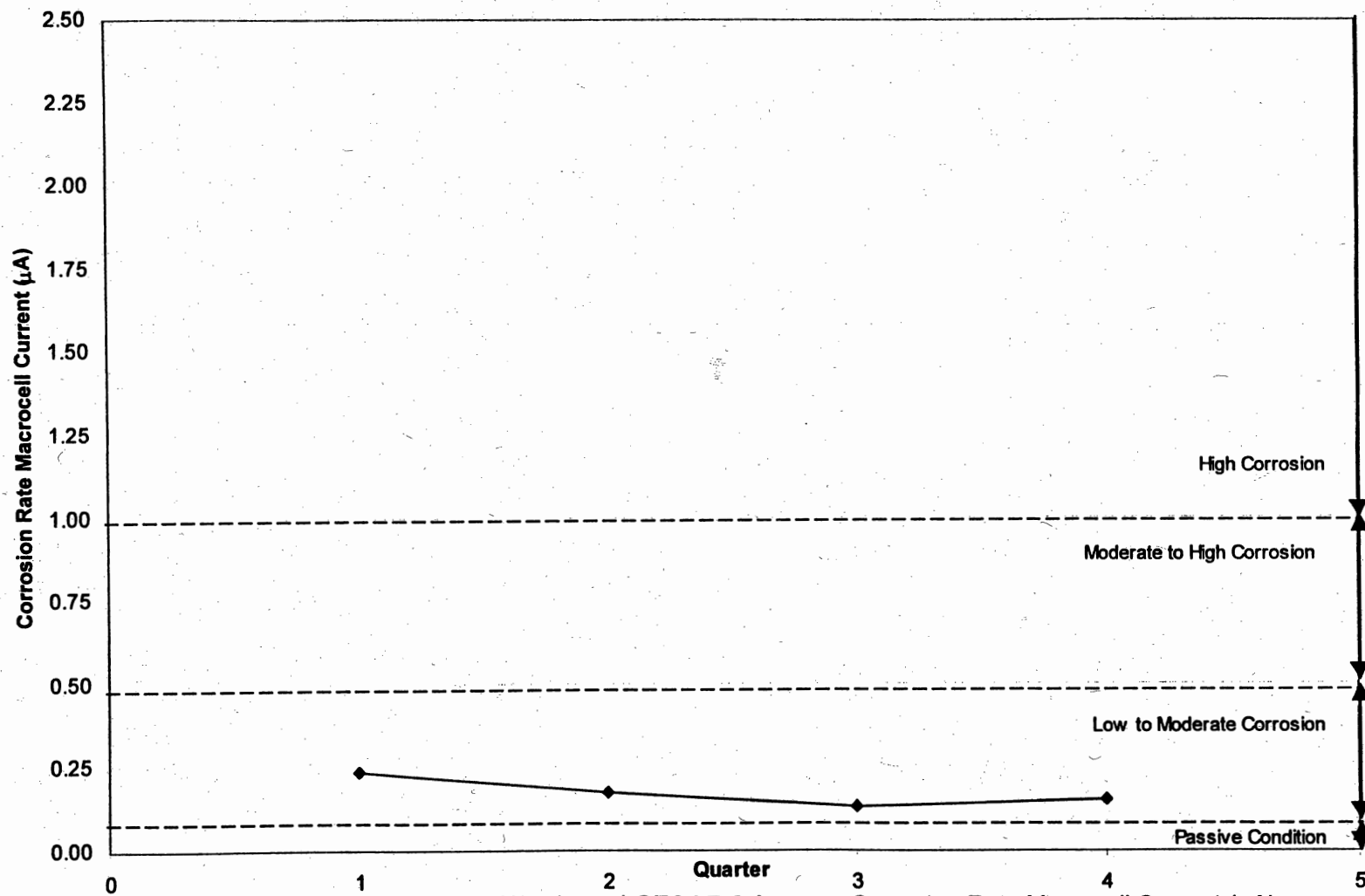
Fig. 4.3: North Main Street Westbound GECOR 6 Average Corrosion Rate Macrocell Current (μA)
