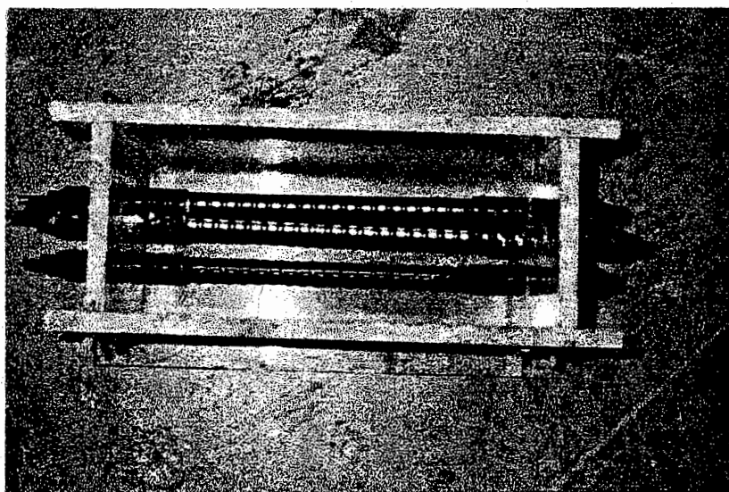
Fig. 3.46: Prepared Minideck Mold
