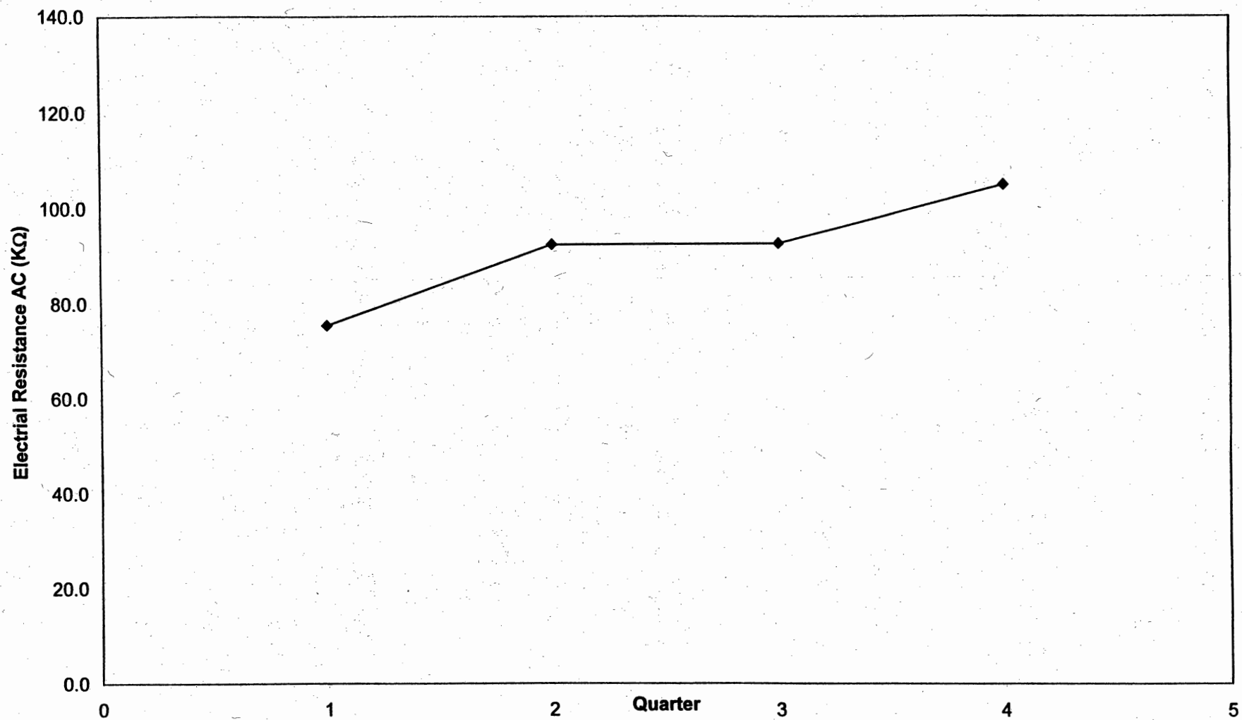
Fig. 4.21: Wyckoff Road Westbound Average Electrical Resistance AC (KΩ)
