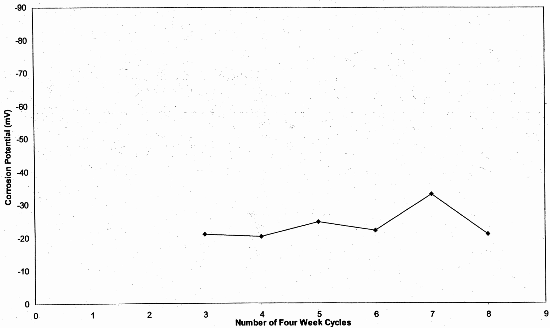
Fig. 4.16: Minideck C - Average Corrosion Potential (mV)
