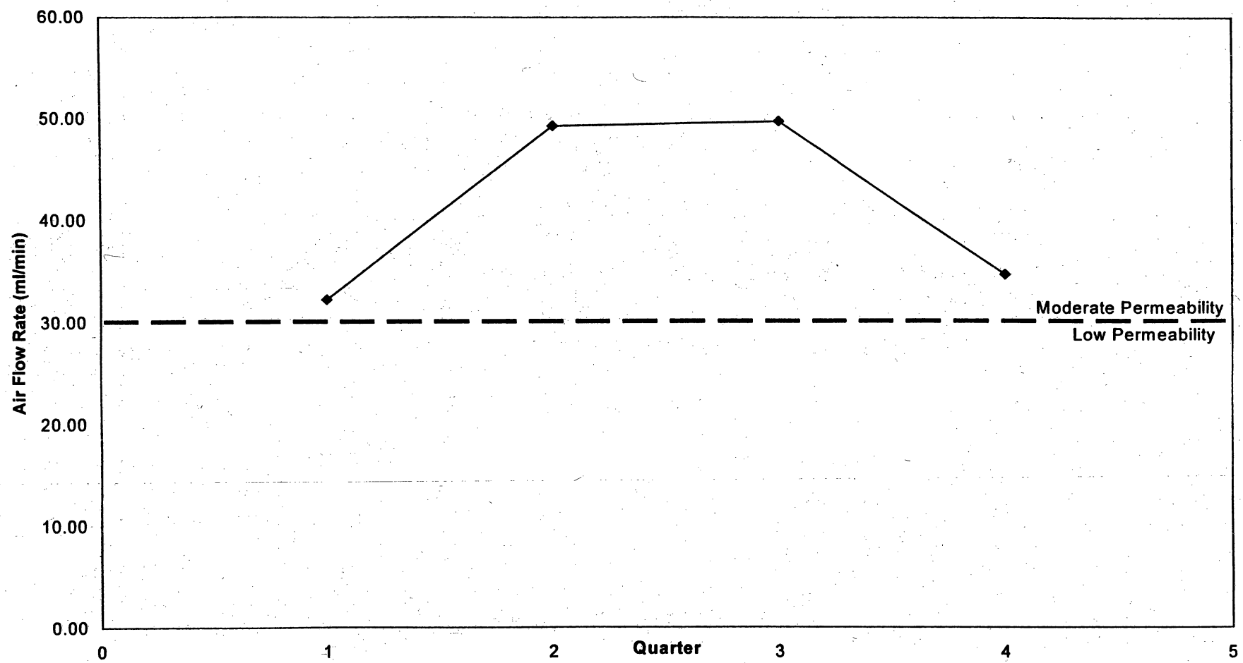
Fig. 4.6: North Main Street Westbound Average Air Flow Rate (ml/min)
