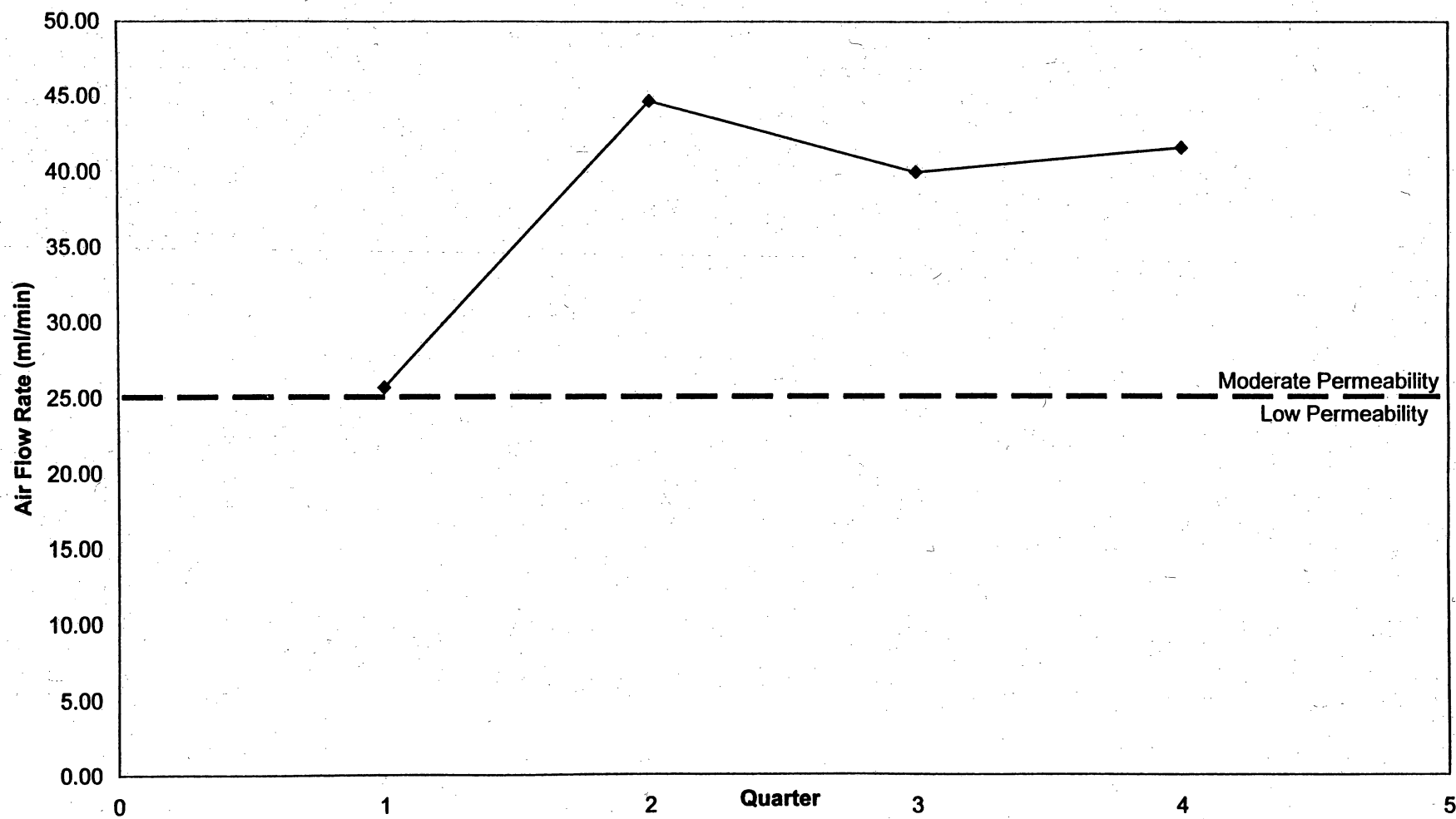
Fig. 4.27: Wyckoff Road Westbound Average Air Flow Rate (ml/min)
