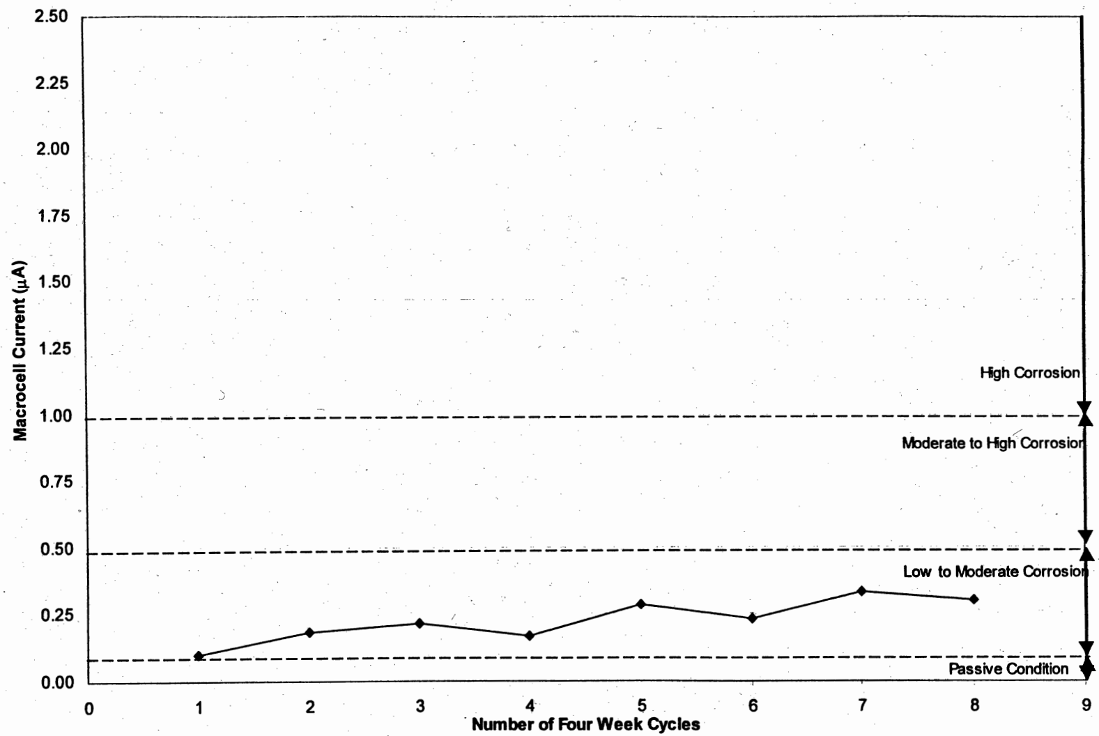
Fig. 4.8: Minideck B - Average Corrosion Rate Macrocell Current (µA)
