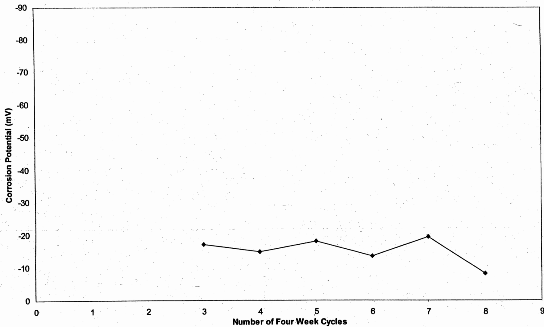
Fig. 4.23: Minideck D - Average Corrosion Potential (mV)
