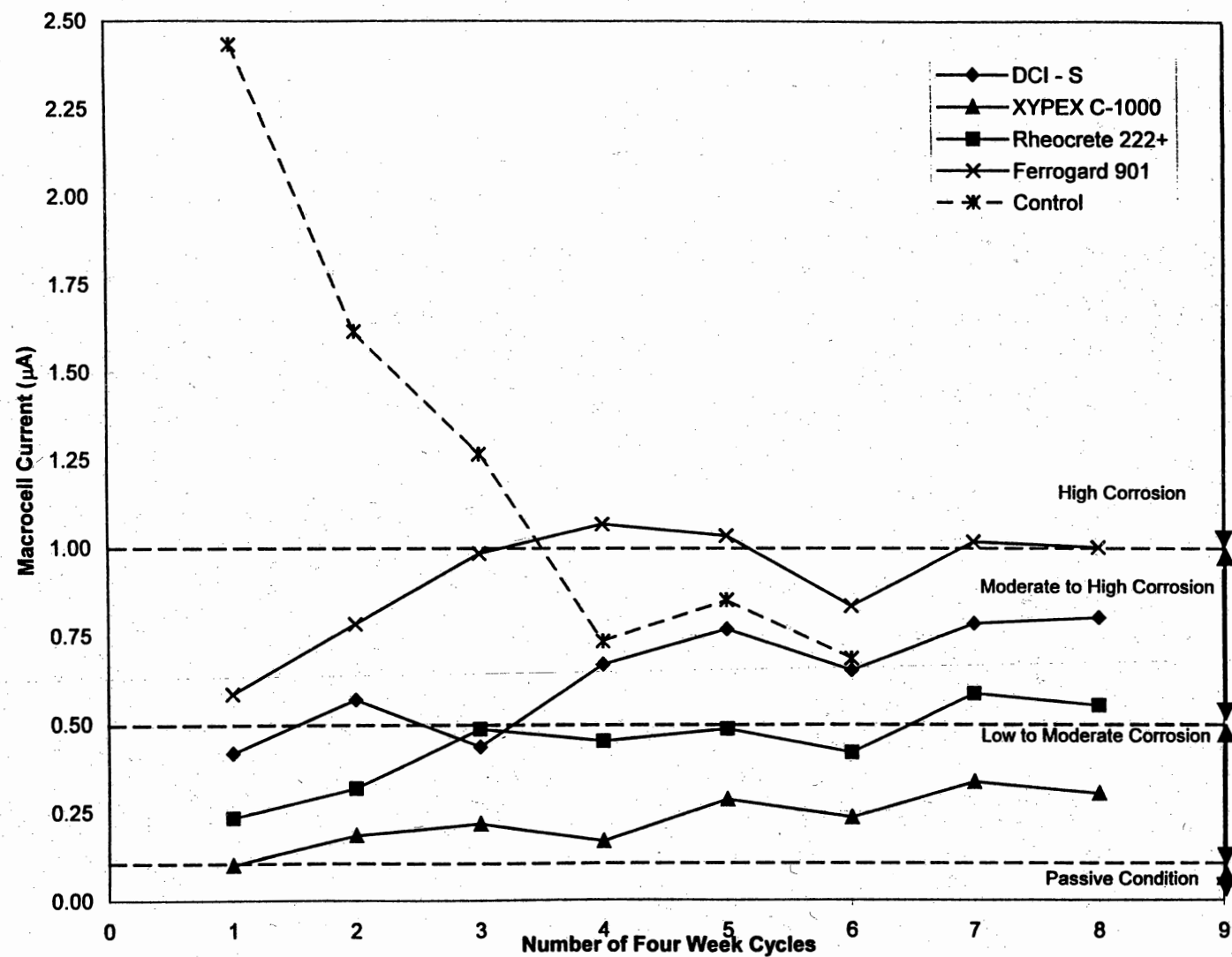
Fig. 4.36: Comparison of Corrosion Inhibitors Minideck Average Corrosion Rate Macrocell Current ( \mu\text{A} )
