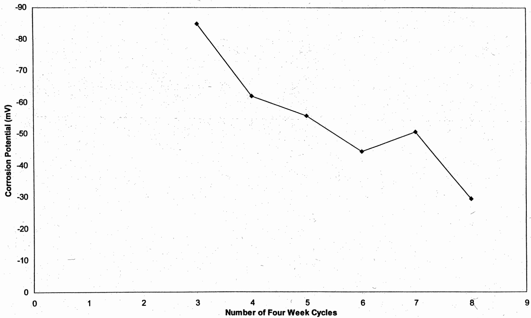
Fig. 4.30: Minideck E - Average Corrosion Potential (mV)
