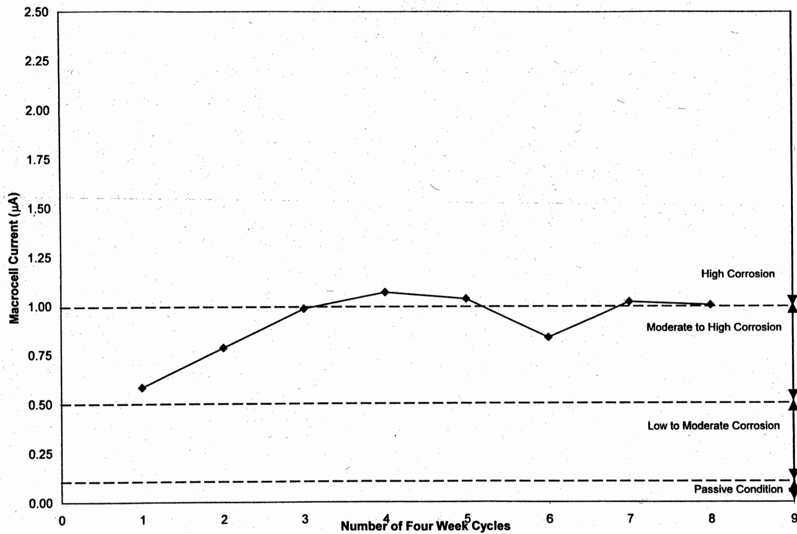
Fig. 4.22: Minideck D - Average Corrosion Rate Macrocell Current ( \mu\text{A} )
