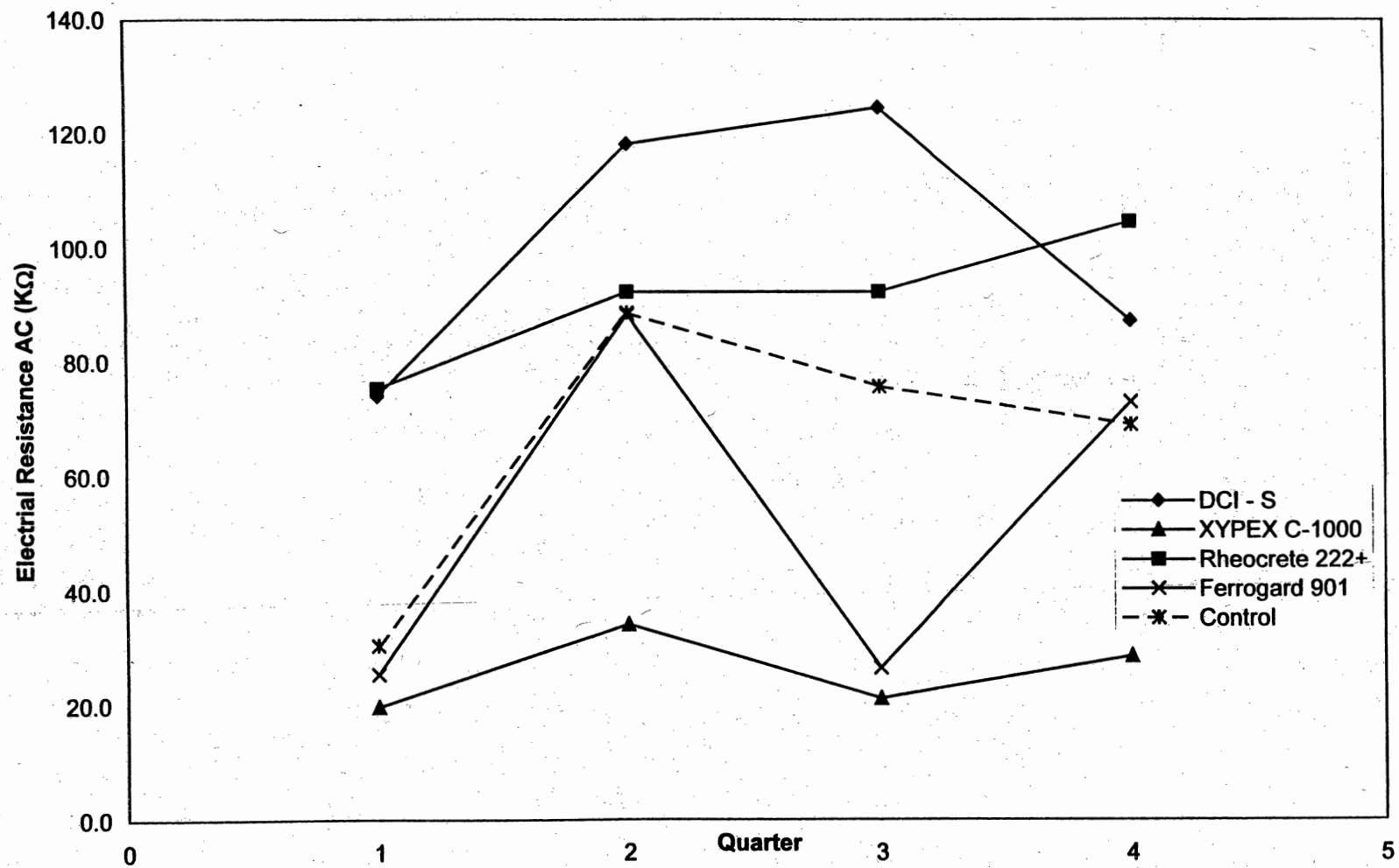
Fig. 4.42: Comparison of Corrosion Inhibitors Average Electrical Resistance AC (KΩ)
