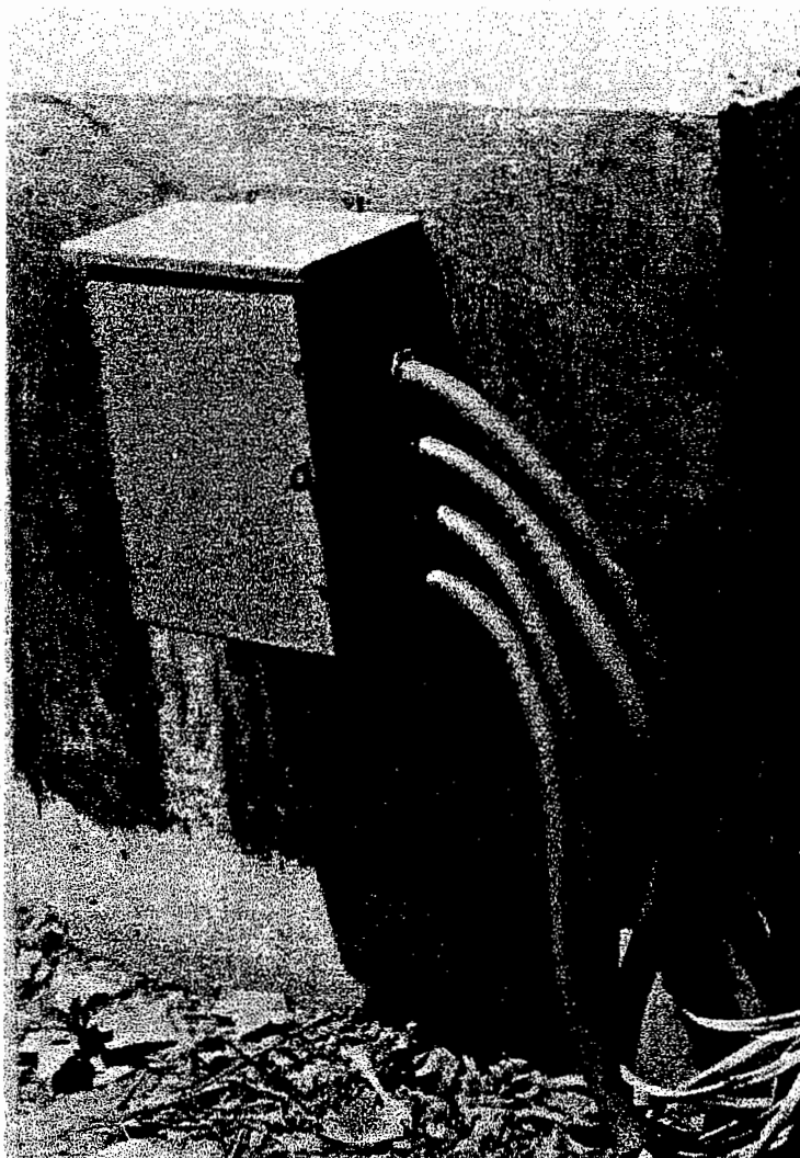
Fig. 3.27: Conduits and Enclosure – Route 130 Westbound
