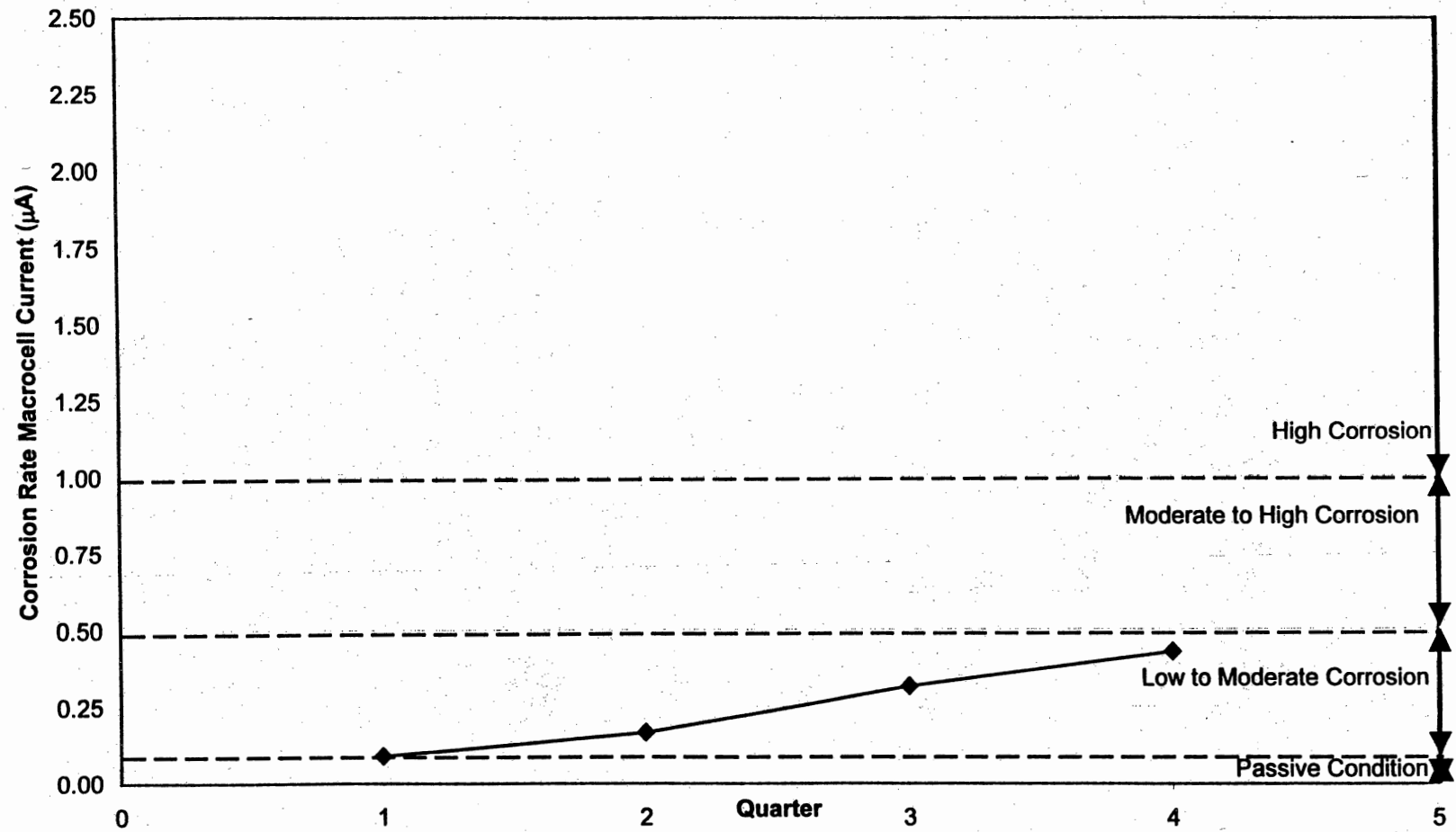
Fig. 4.10: North Main Street Eastbound Average Corrosion Rate Macrocell Current (µA)
