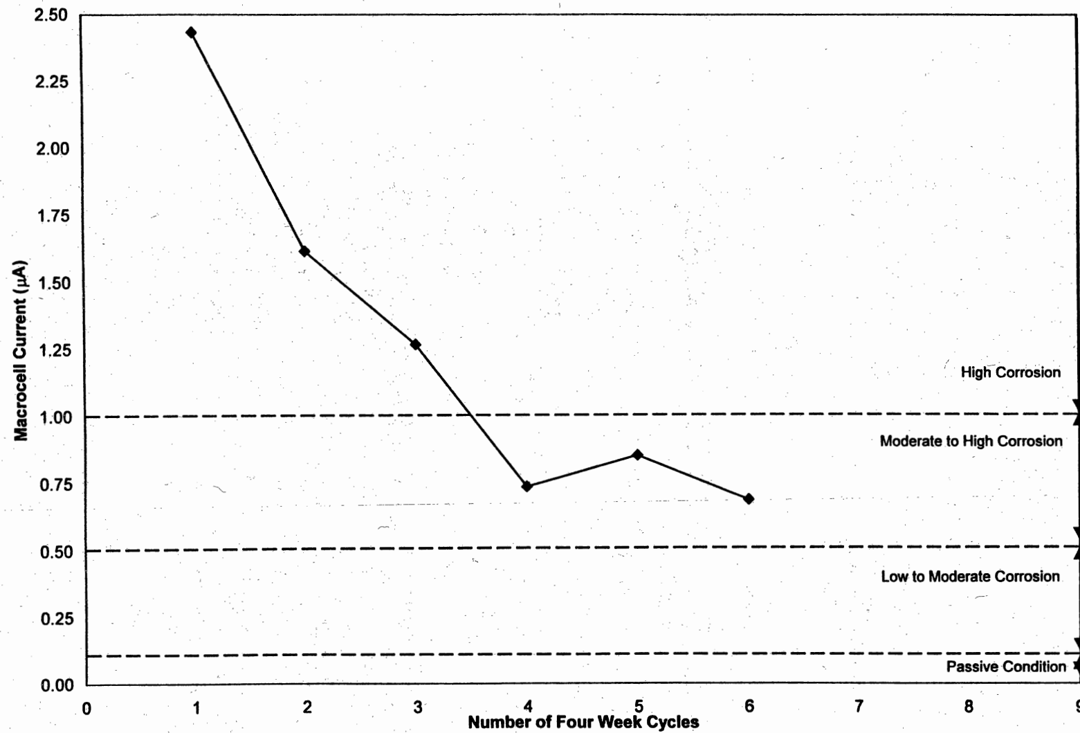
Fig. 4.29: Minideck E - Average Corrosion Rate Macrocell Current ( \mu\text{A} )
