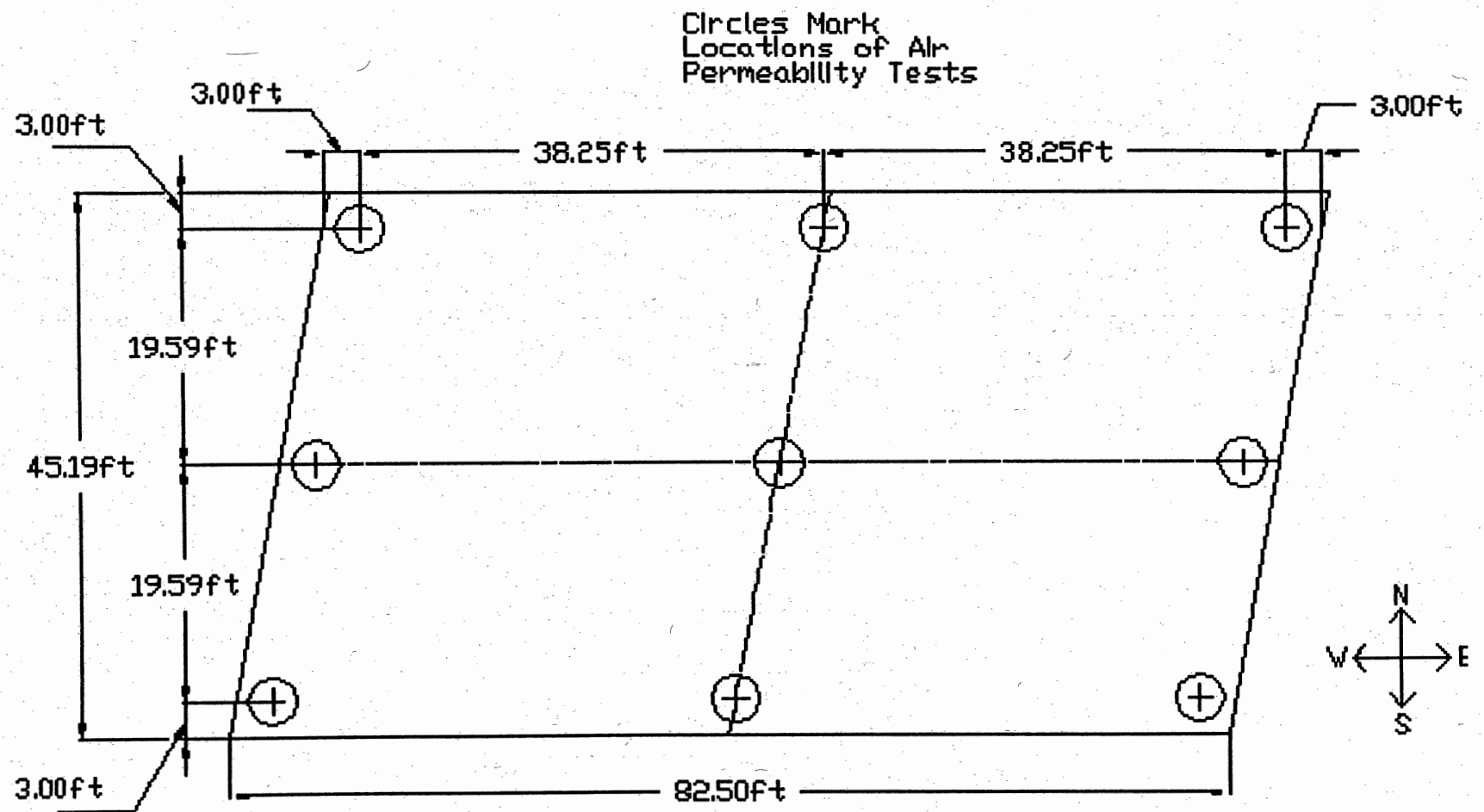
Fig. 3.39: Locations of Surface Air Flow Permeability Readings Wyckoff Road Eastbound
