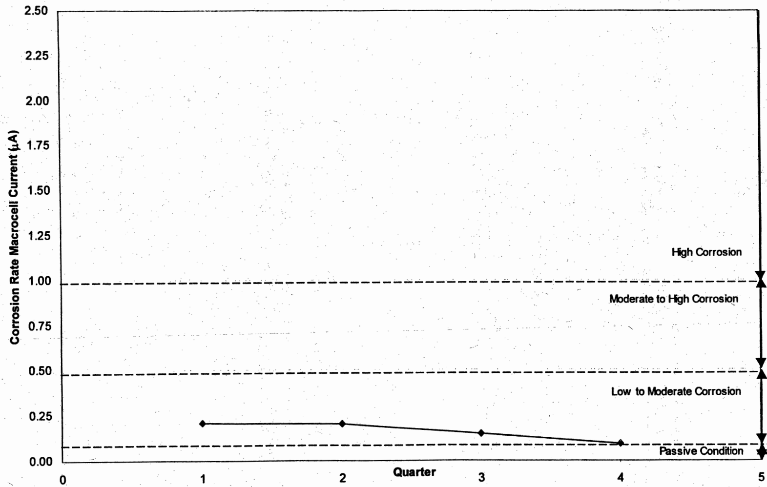
Fig. 4.31: Route 130 Westbound GECOR 6 Average Corrosion Rate Macrocell Current (μA)
