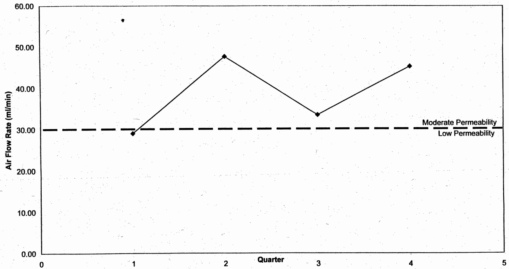
Fig. 4.20: Wyckoff Road Westbound Average Air Flow Rate (ml/min)
