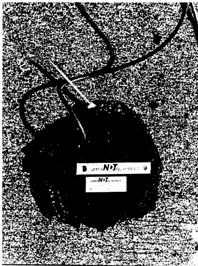
Fig. 3.2: GECOR 6 Corrosion Rate Meter Sensor with Sponge
