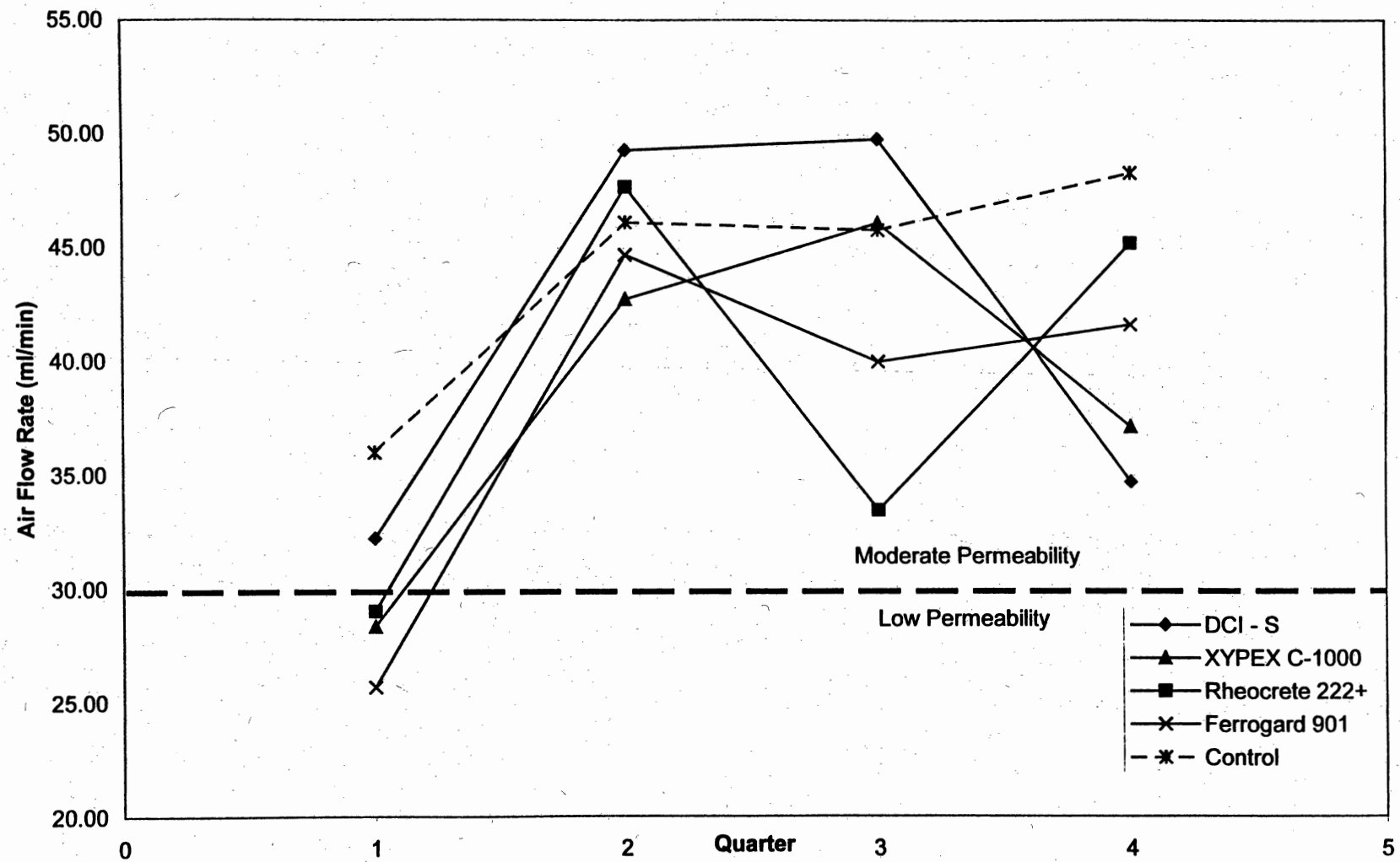
Fig. 4.41: Comparison of Corrosion Inhibitors Average Air Flow Rate (ml/min)
