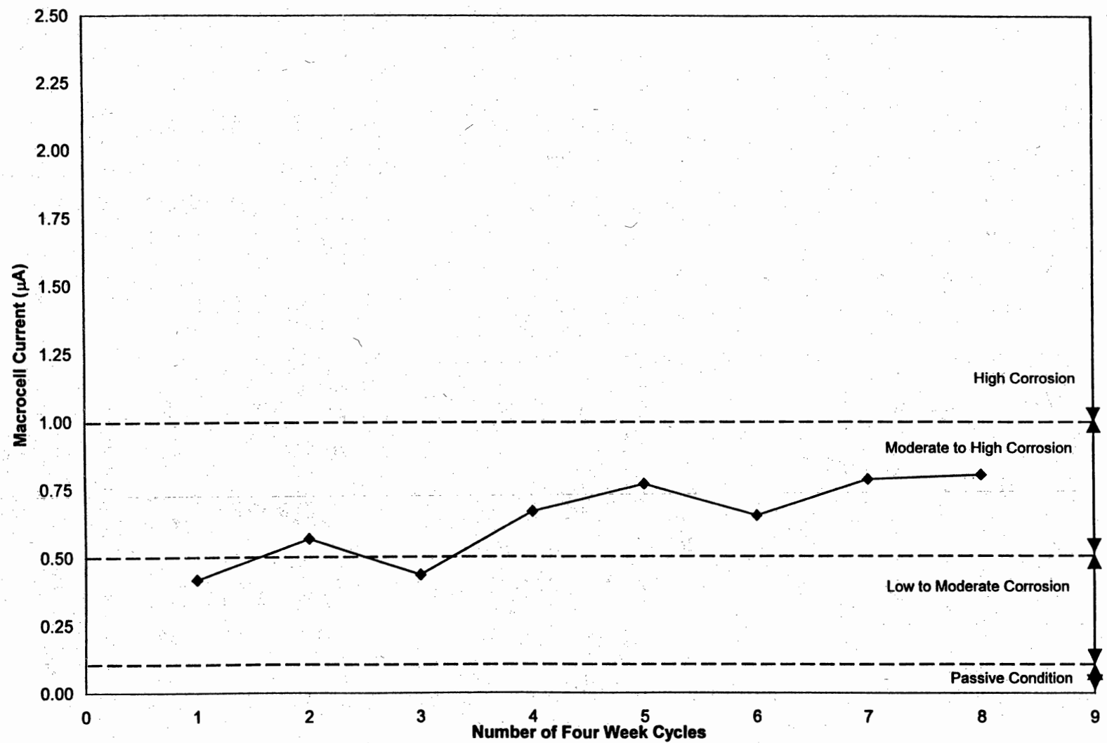
Fig. 4.1: Minideck A - Average Corrosion Rate Macrocell Current (µA)
