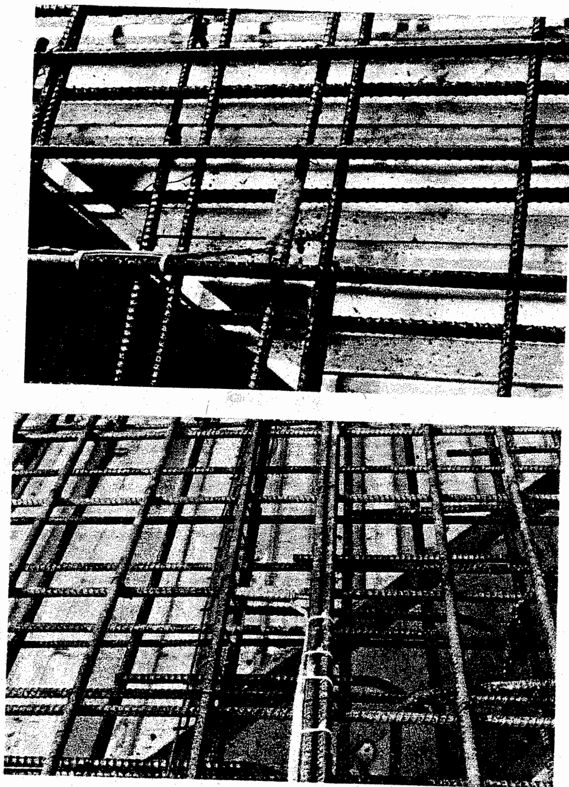
Fig. 3.21: Connection to Wyckoff Road Eastbound
