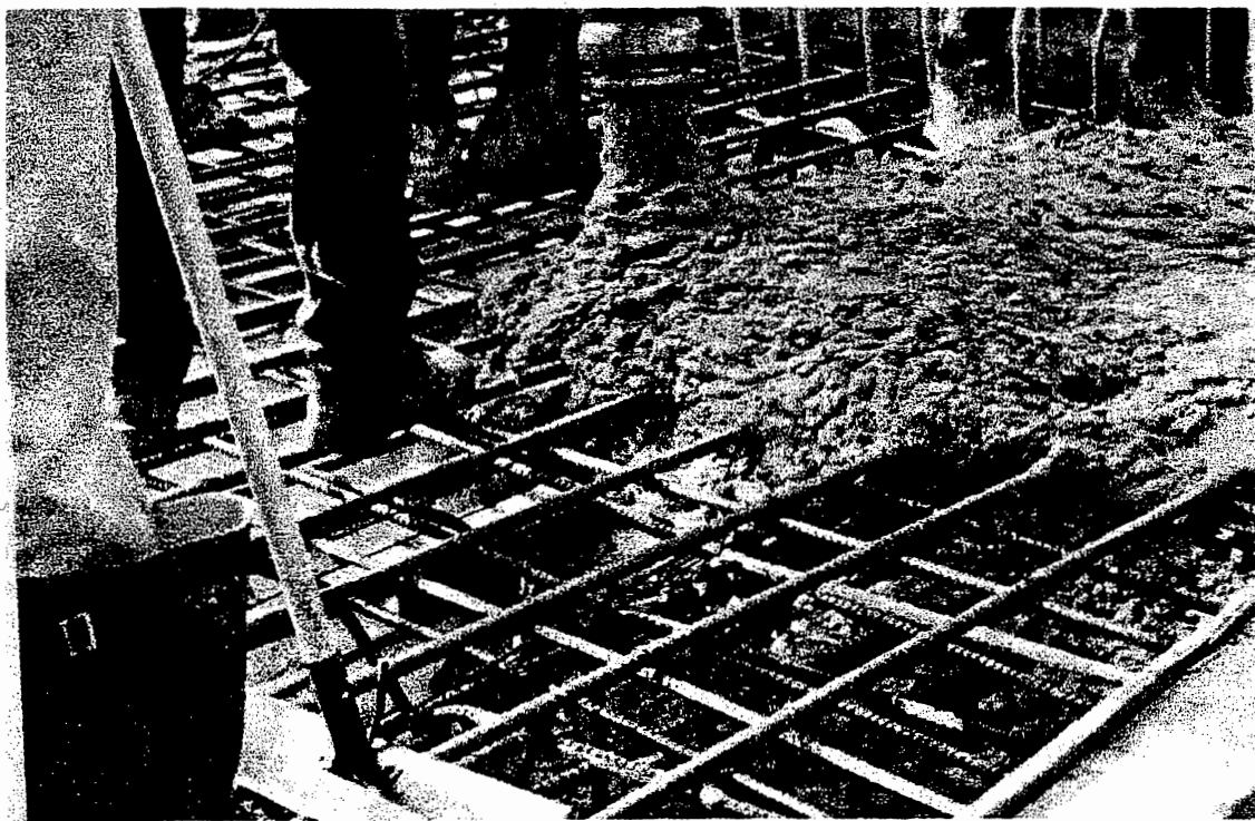
Fig. 3.29: Placement on Fresh Concrete at North Main Street Westbound
