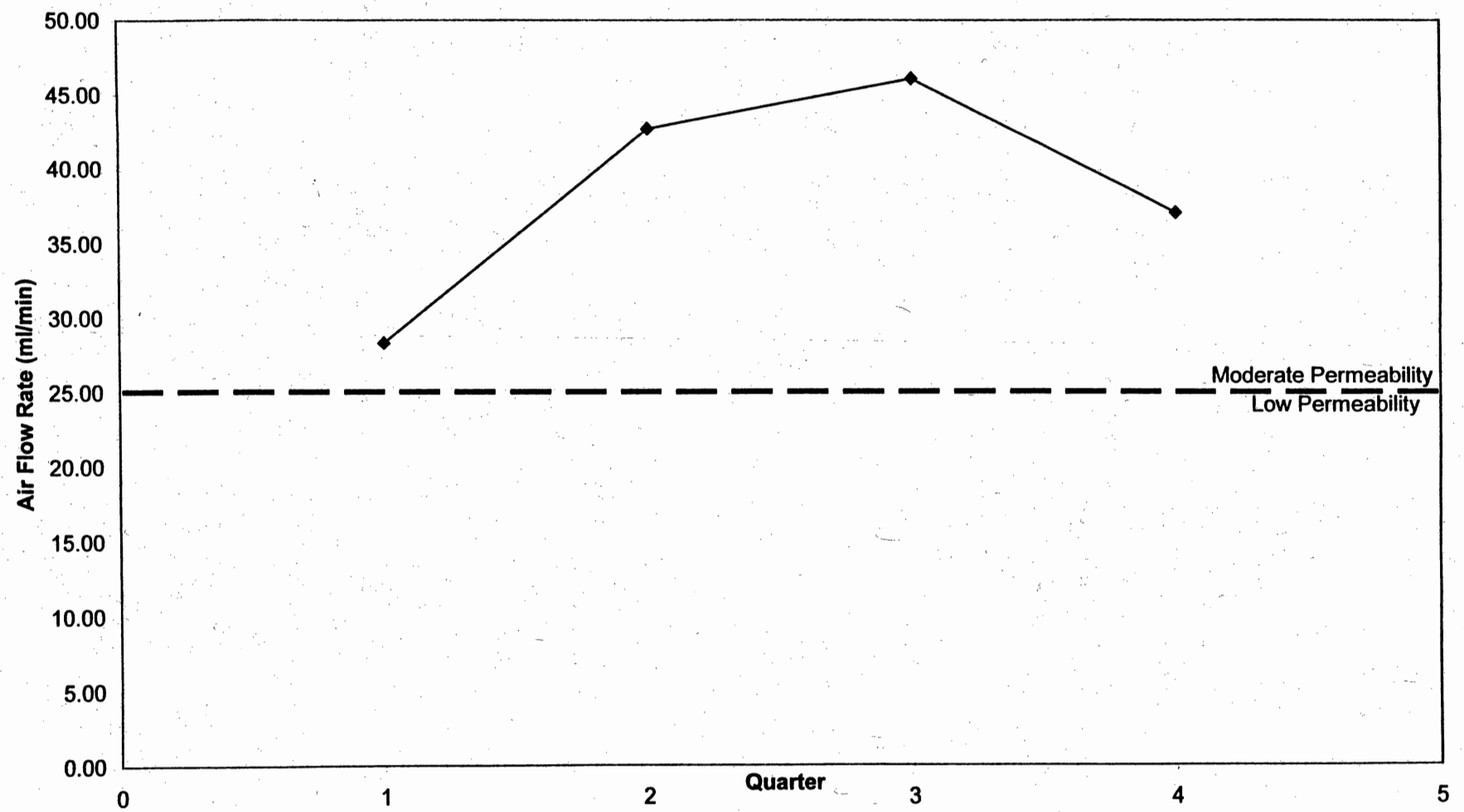
Fig. 4.13: North Main Street Eastbound Average Air Flow Rate (ml/min)
