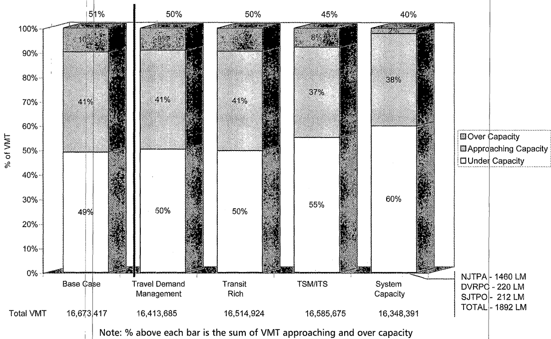
Figure VIII.7 Vehicle Miles Traveled by Level of Service 2025 PM Peak Hour Statewide
