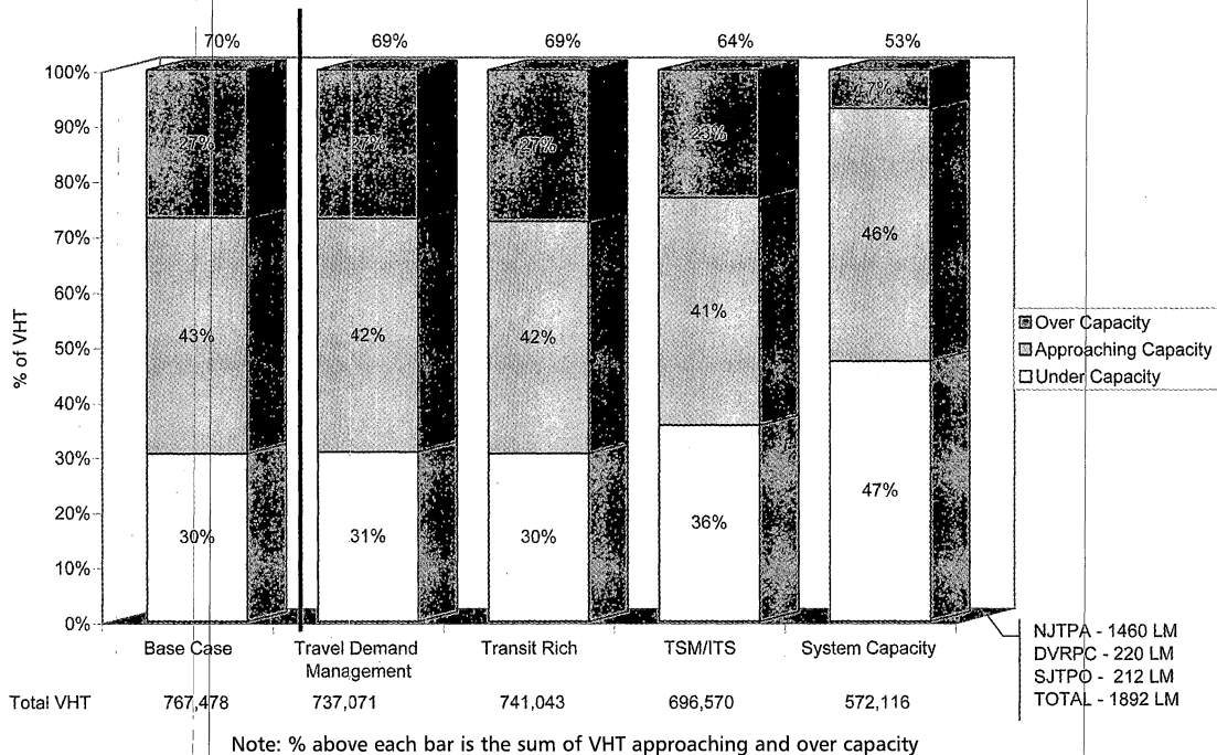
Figure VIII.8 Vehicle Hours Traveled by Level of Service 2025 PM Peak Hour Statewide
