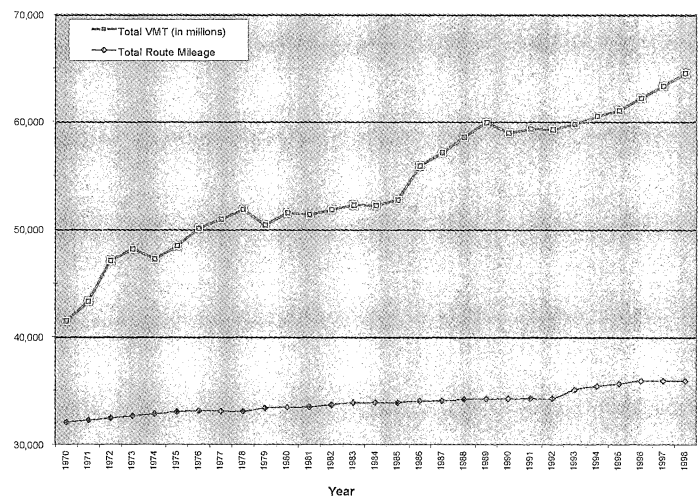
Figure III.3 Growth in VMT vs. Route Mileage, New Jersey 1970-1998
