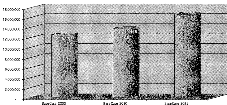
Figure VIII.6 Vehicle Hours Traveled PM Peak Hour Statewide
