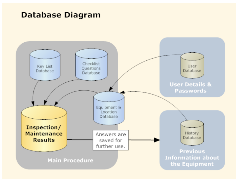
Figure 12. Database Diagram
