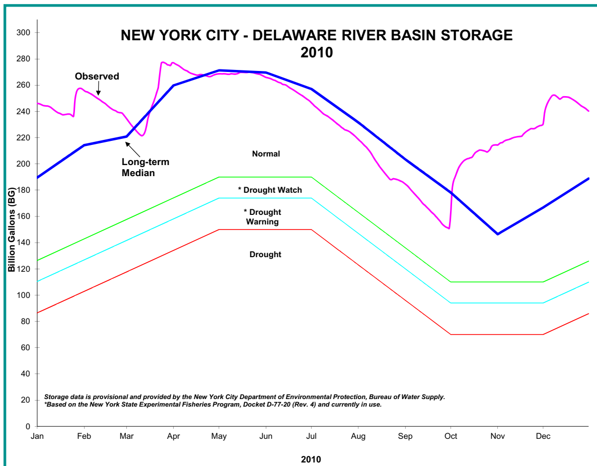
This graph shows the observed combined water storage in the NYC-Delaware Basin reservoirs (Cannonsville, Pepacton, and Neversink) during 2010, as well as the long-term median and drought rating curves. The period of record represented by the long-term median values is June 1967 to November 1998.
