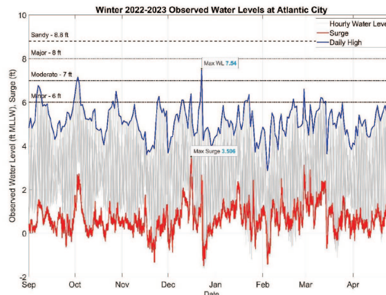
Figure 1: Winter 2022-23 water levels measured at Atlantic City.
