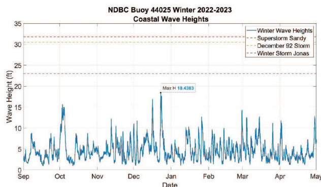
Figure 3: Winter 2022-23 wave heights measured off Long Branch.
