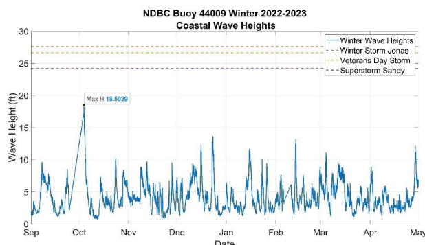
Figure 2: Winter 2022-23 wave heights measured off Cape May.
