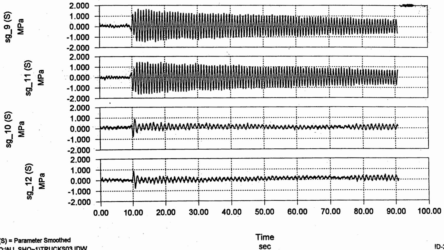
Figure 3-32 Comparison of Structure in "Twisting" and "Hatchet" Modes.
