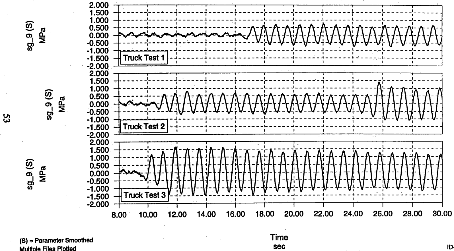
Figure 3-28 Comparison of Column Response in All Three Truck Tests.
