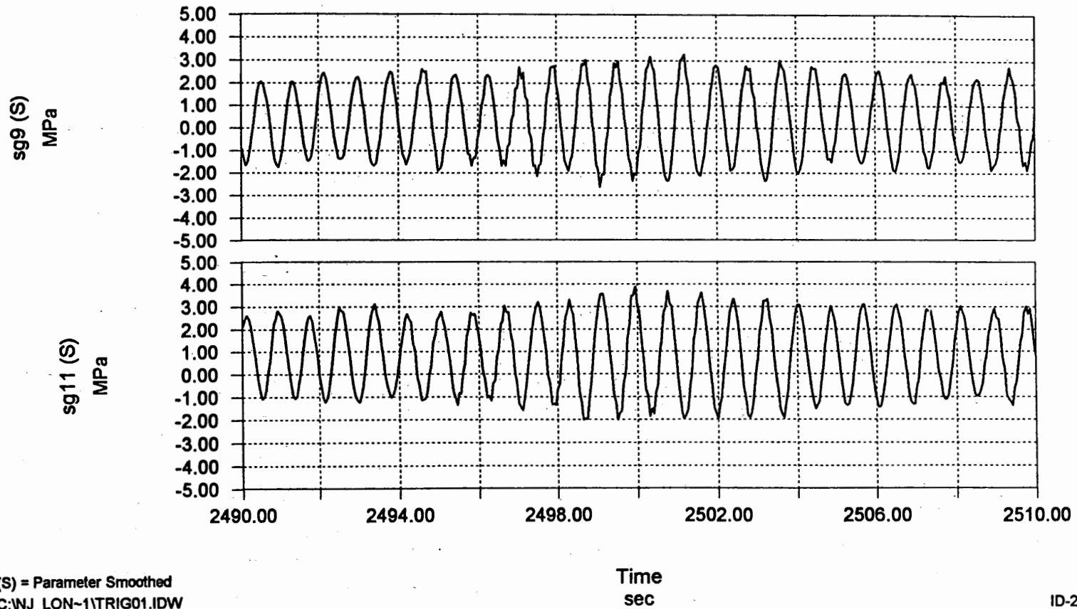
Figure 3-36 Close Up of Long Term Data.
