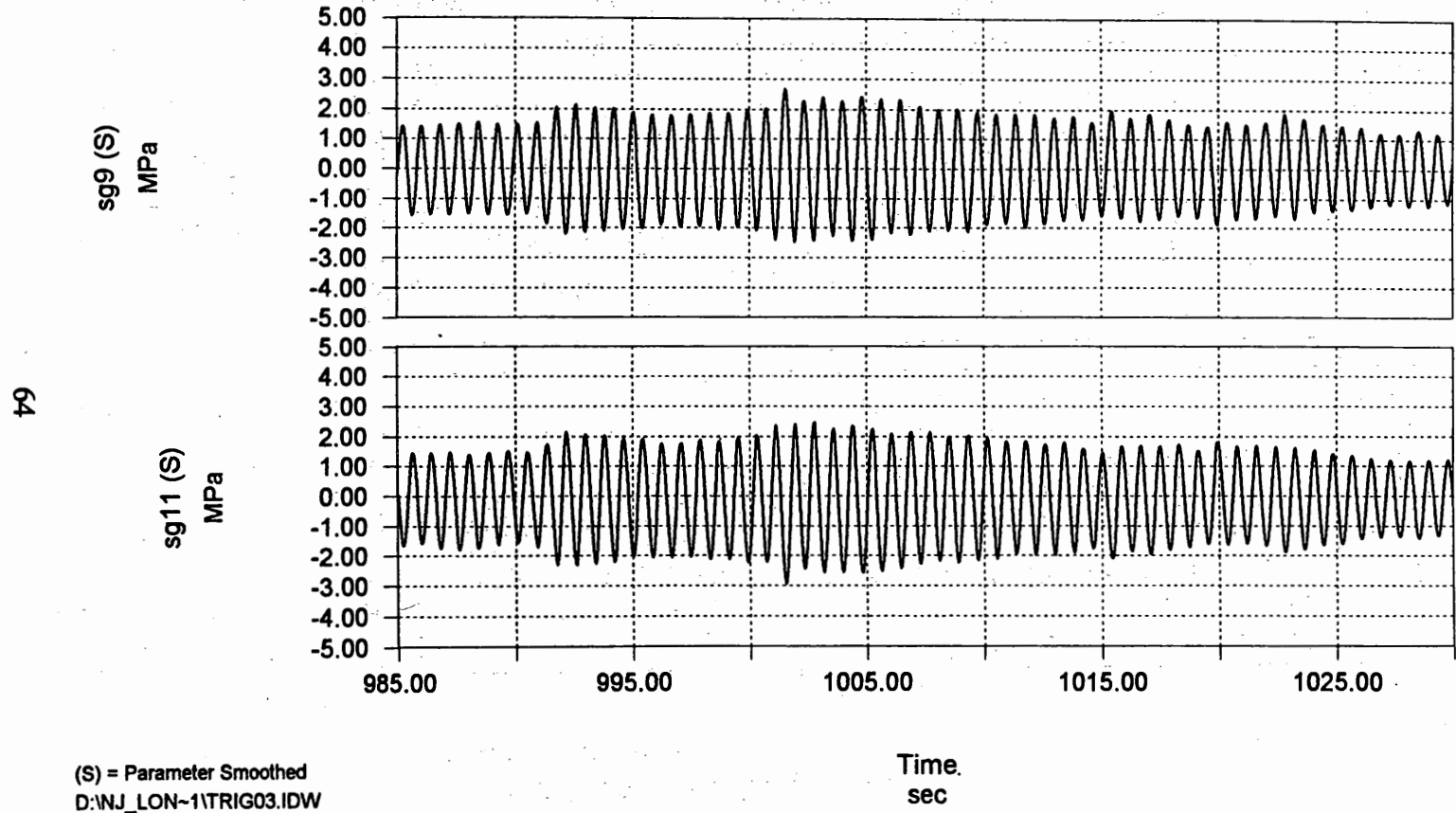
Figure 3-39 Close Up of Long Term Data
