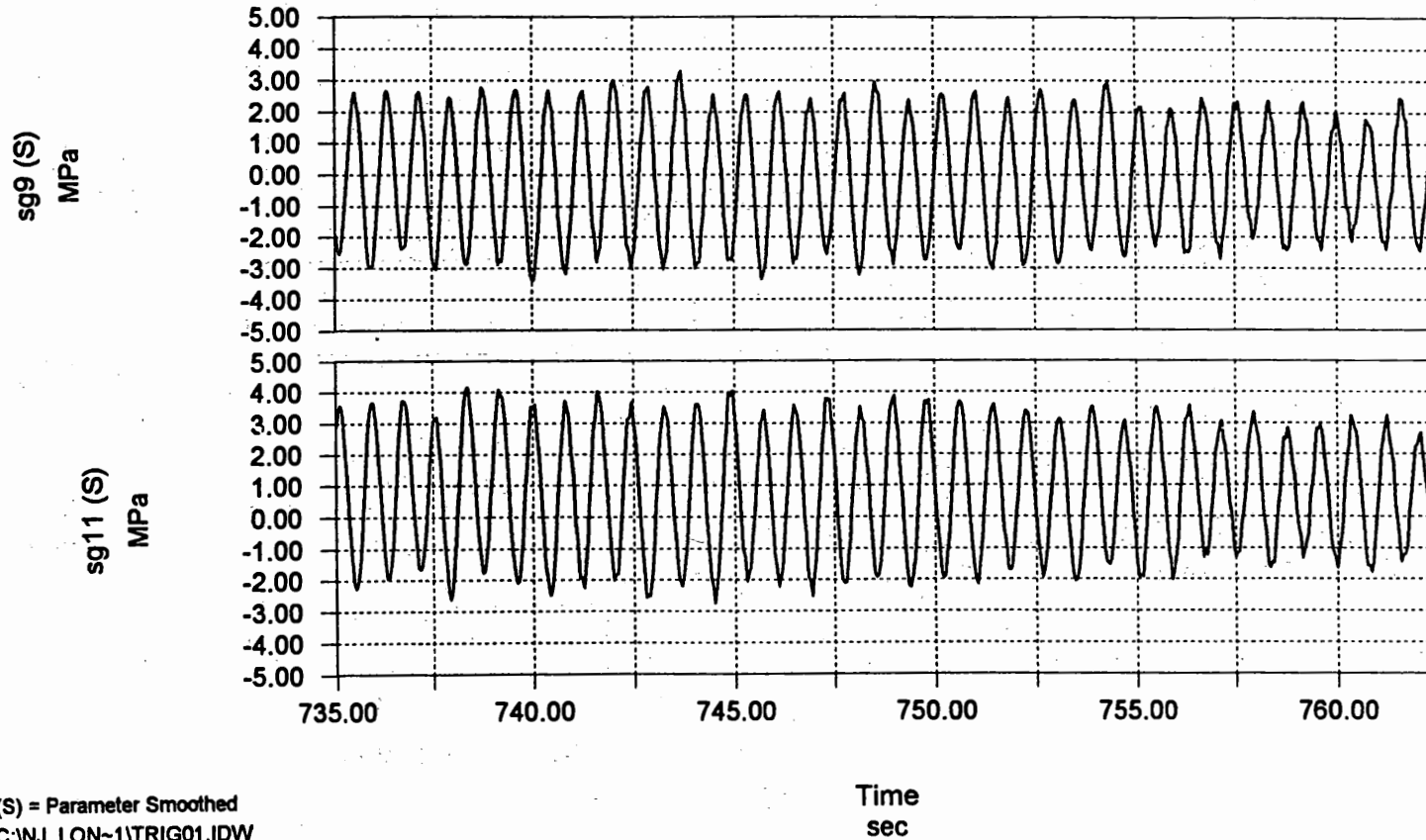
Figure 3-34 Close Up of Long Term Data.
