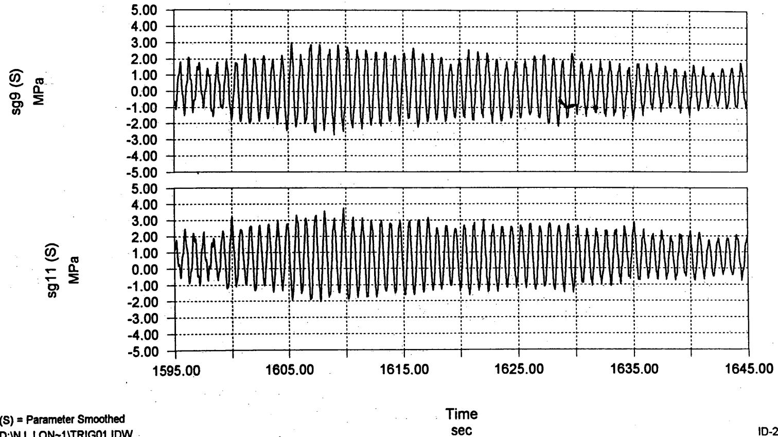
Figure 3-35 Close Up of Long Term Data.
