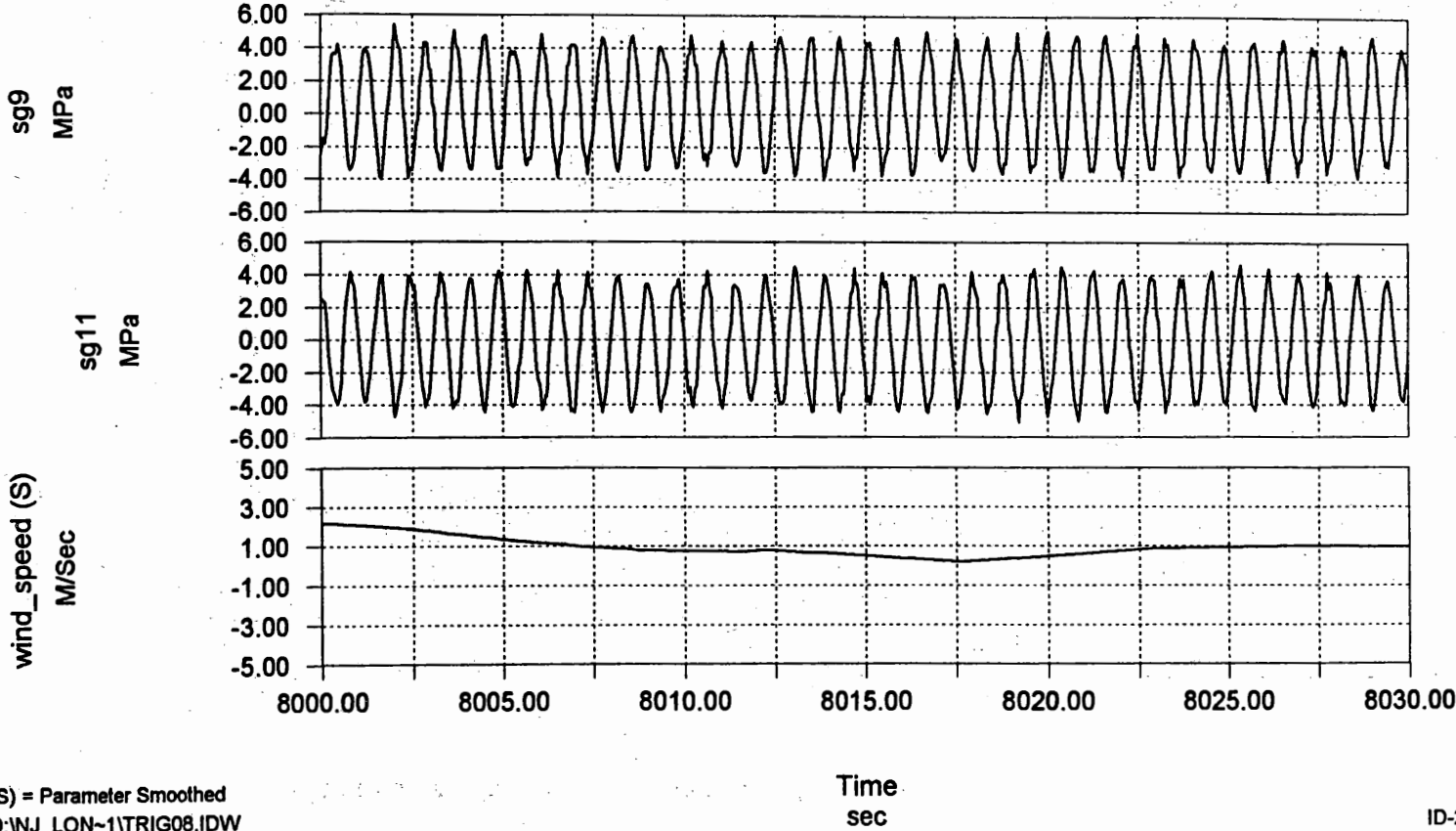
Figure 3-41 Maximum Recorded Stress Ranges in Column and Natural Wind Speed.
