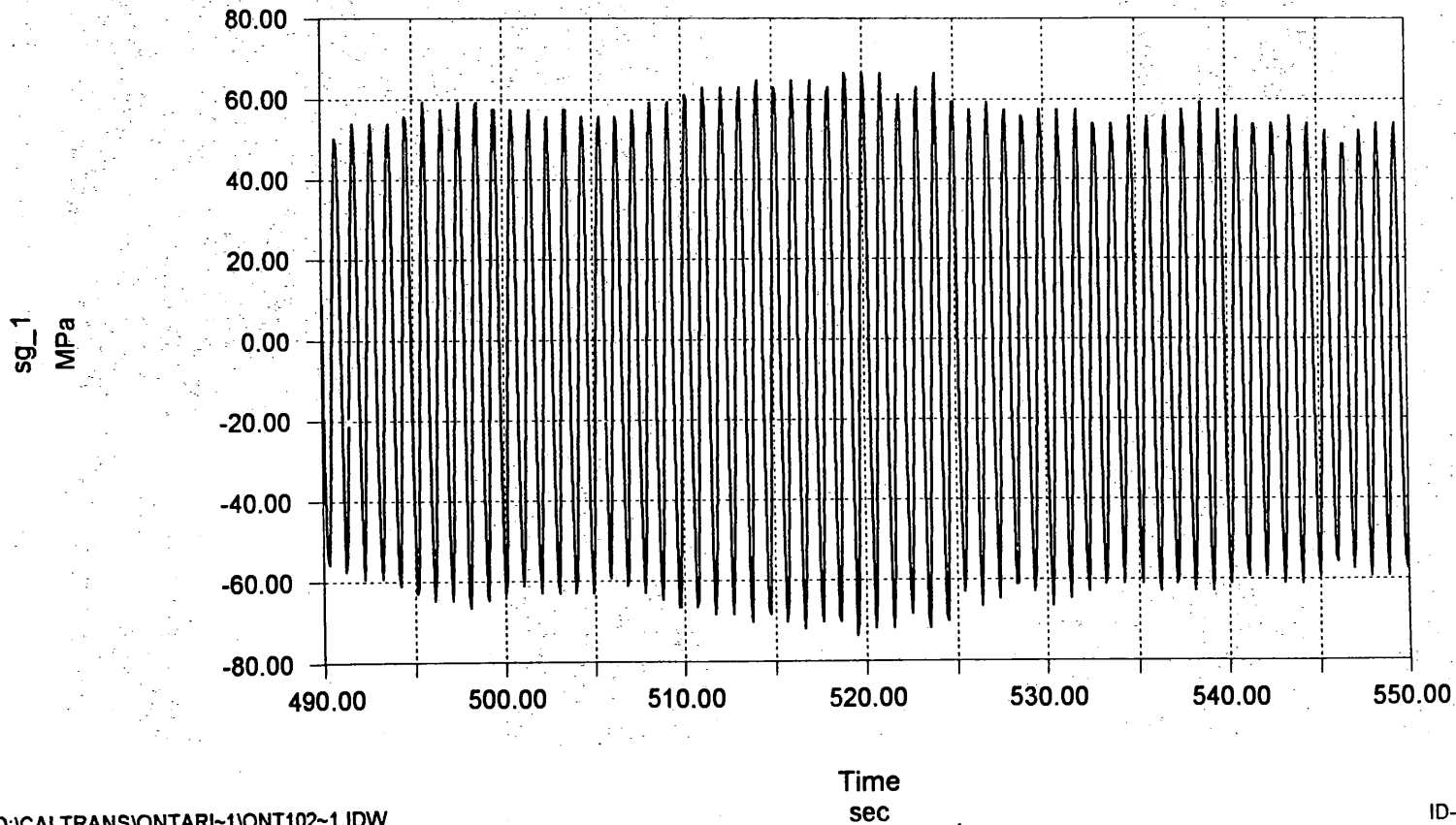
Figure 2-1 Stress Range in a Caltrans Monotube VMS Sign Support Structure.
