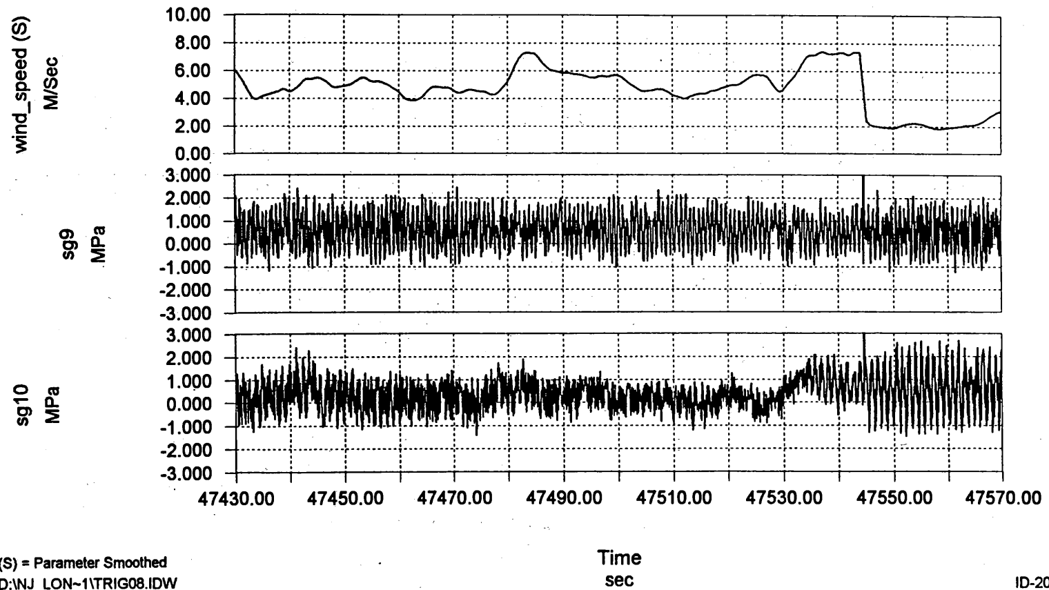
Figure 3-44 Maximum Wind Speed and Column Response.
