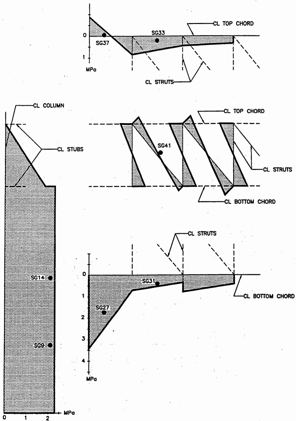
Figure 3-23 Stress in Structure from a 1 kN Load
