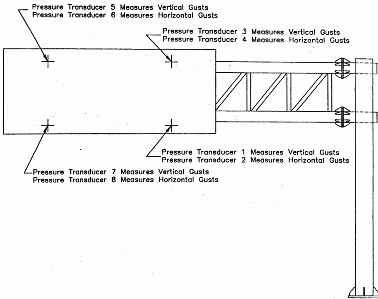
Figure 3-13 Pressure Transducer Numbering Scheme.
