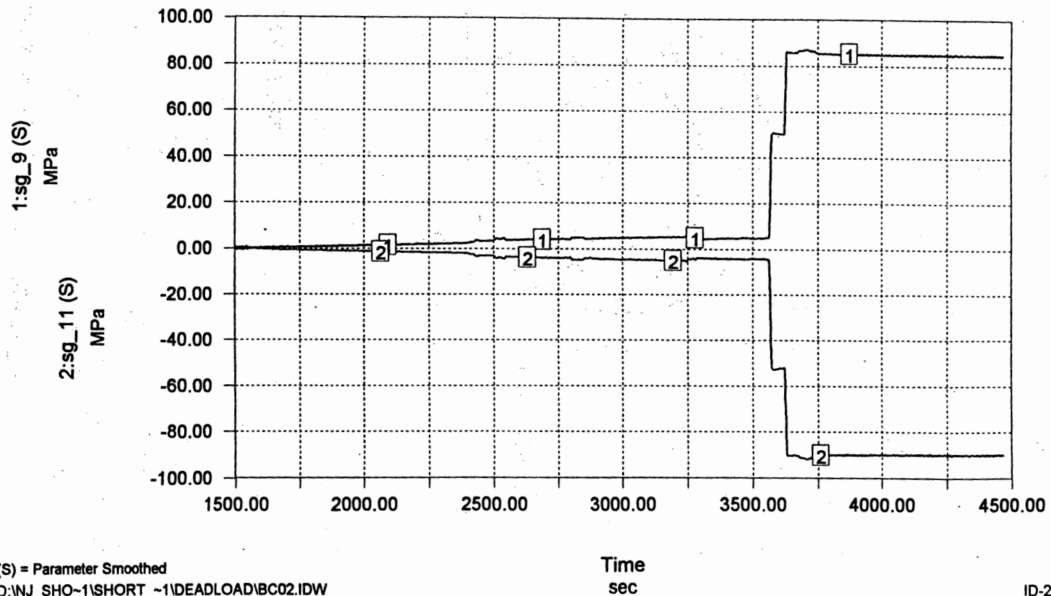
Figure 3-8 Dead Load Stress in Column.
