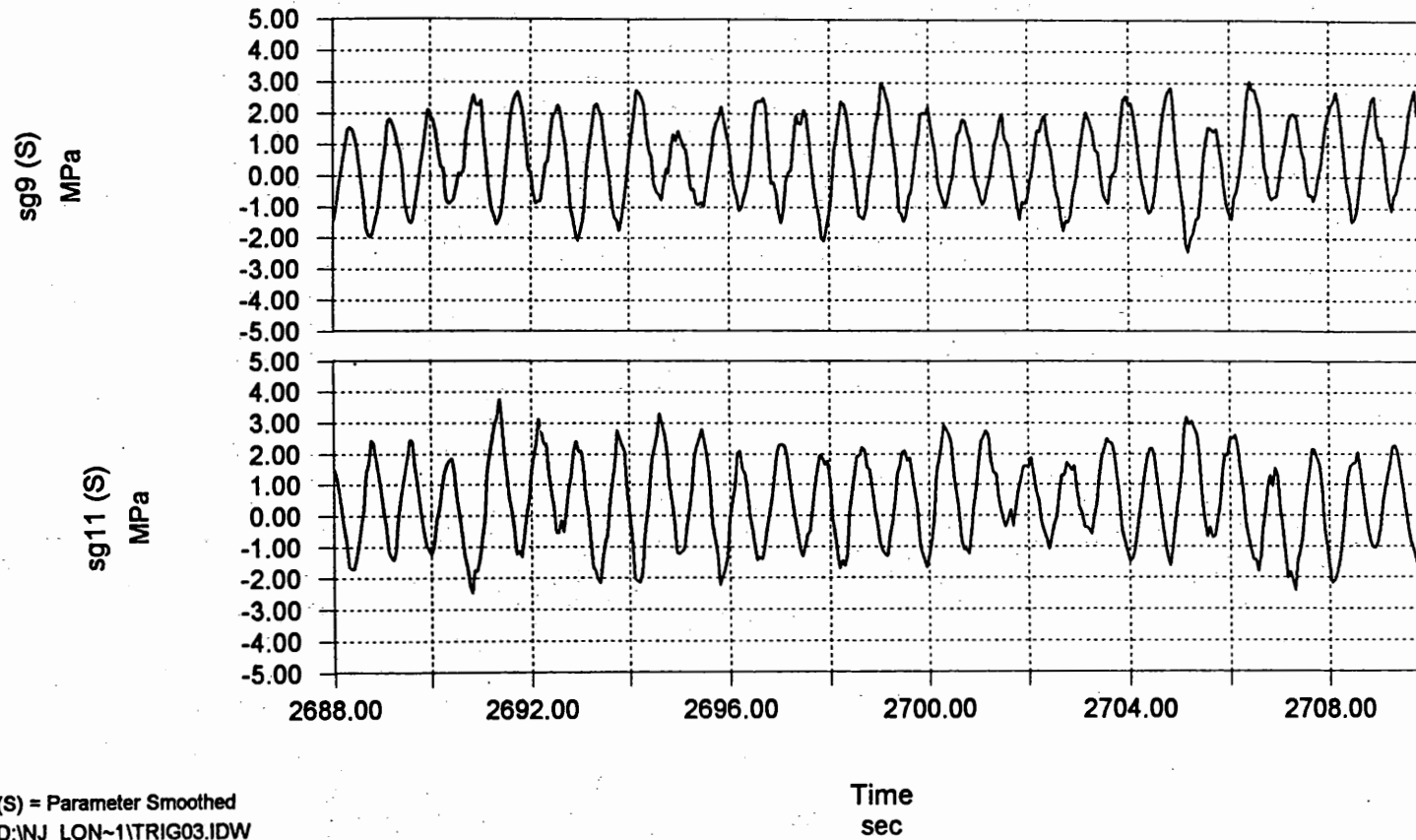
Figure 3-40 Close Up of Long Term Data
