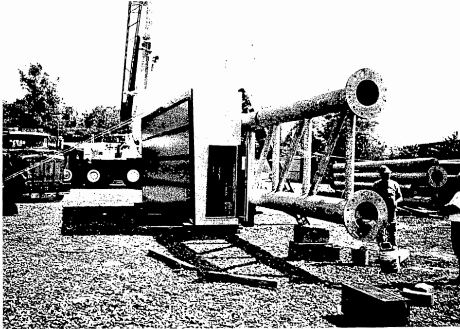
Figure 3-3 VMS Connected to Truss in Storage Yard.
