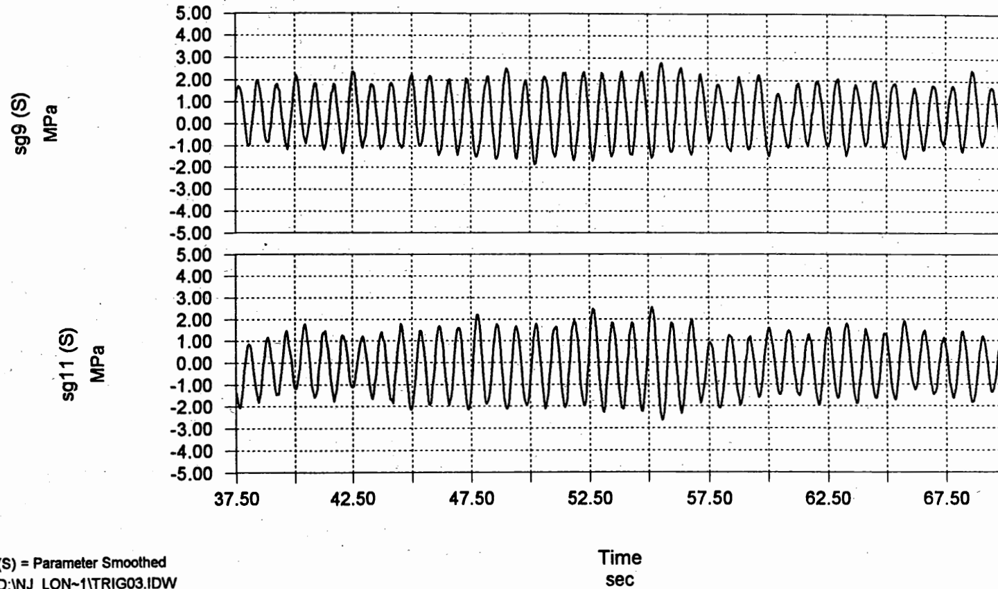
Figure 3-38 Close Up of Long Term Data.
