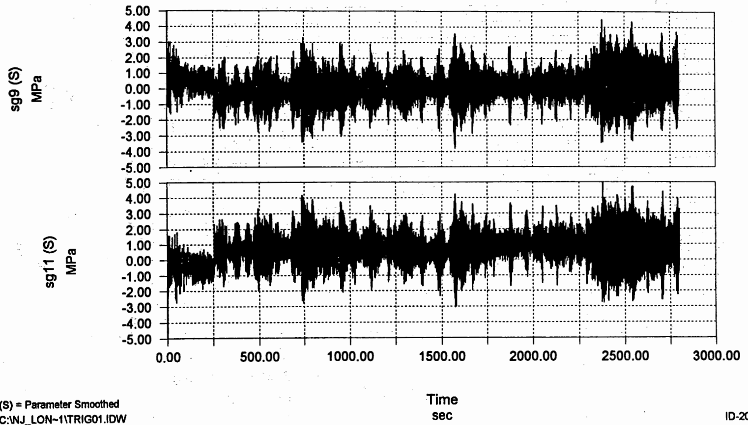
Figure 3-33 Random Data File from Long Term Monitoring.
