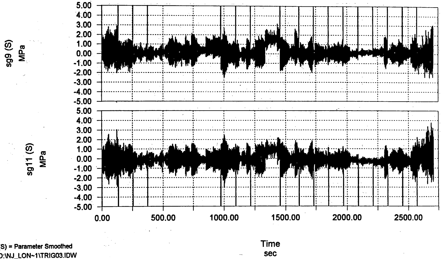
Figure 3-37 Random Data File from Long Term Monitoring.
