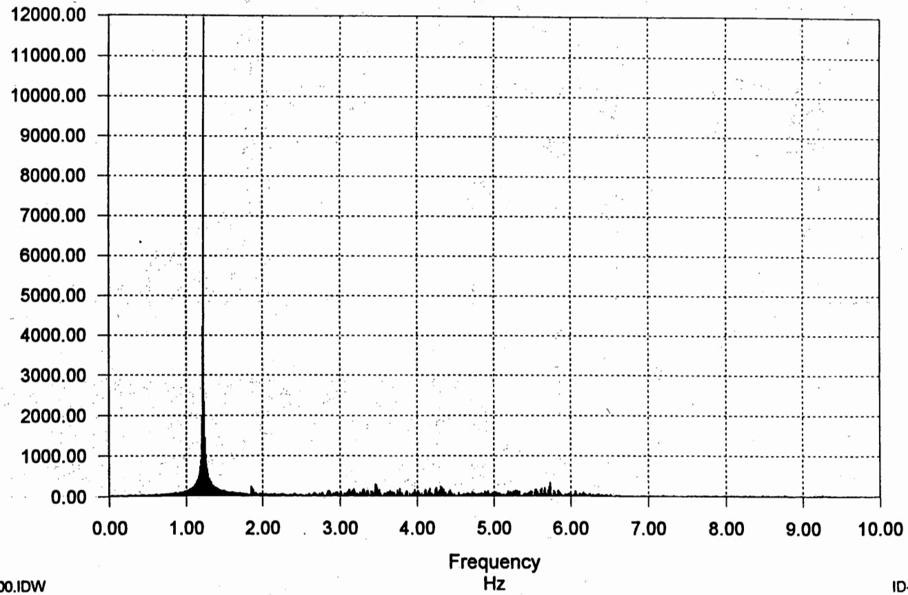
Figure 3-22 FFT Indicating Natural Frequency in the "Hatchet Mode".
