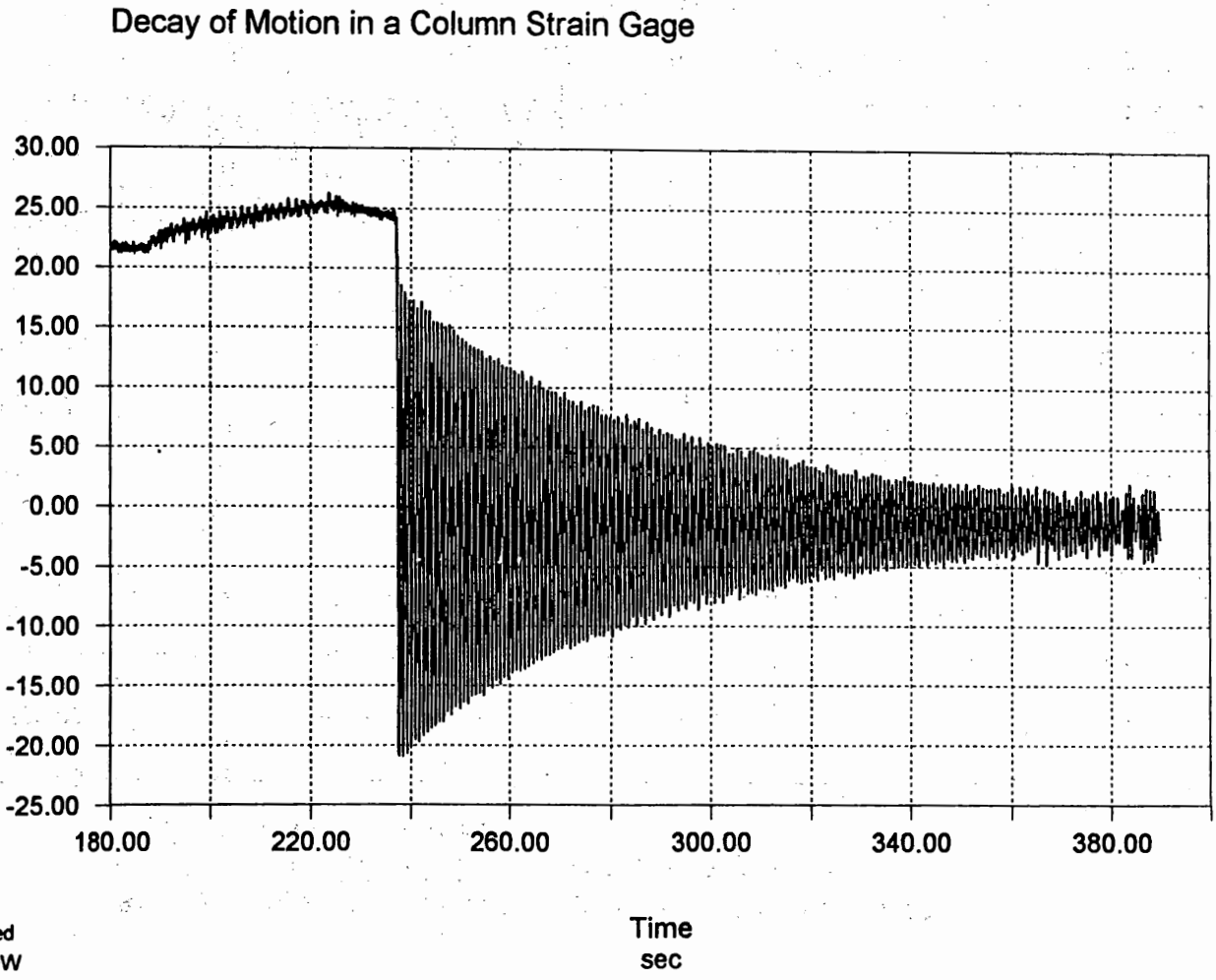
Figure 3-20 Damping of Motion in a Column Strain Gage.
