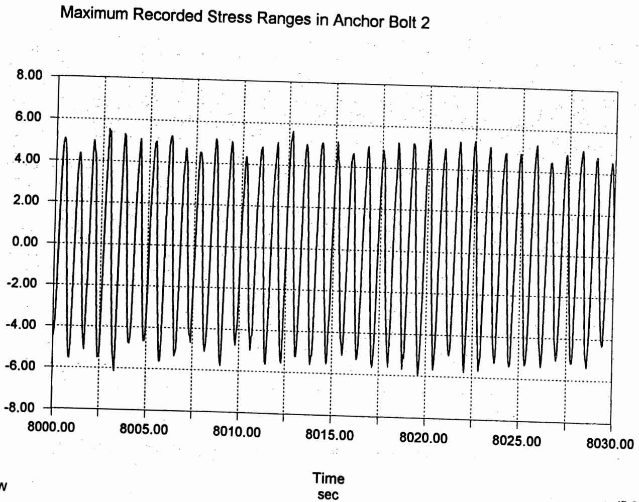
Figure 3-43 Maximum Recorded Axial Stress Ranges in Anchor Bolts.
