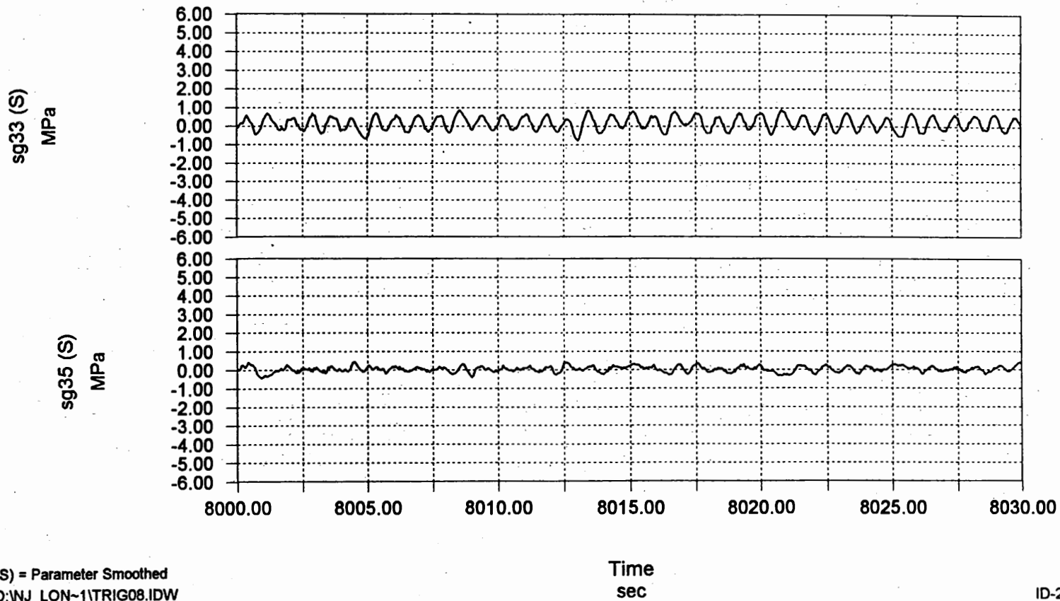
Figure 3-42 Maximum Recorded Stress Ranges in Top Chord.
