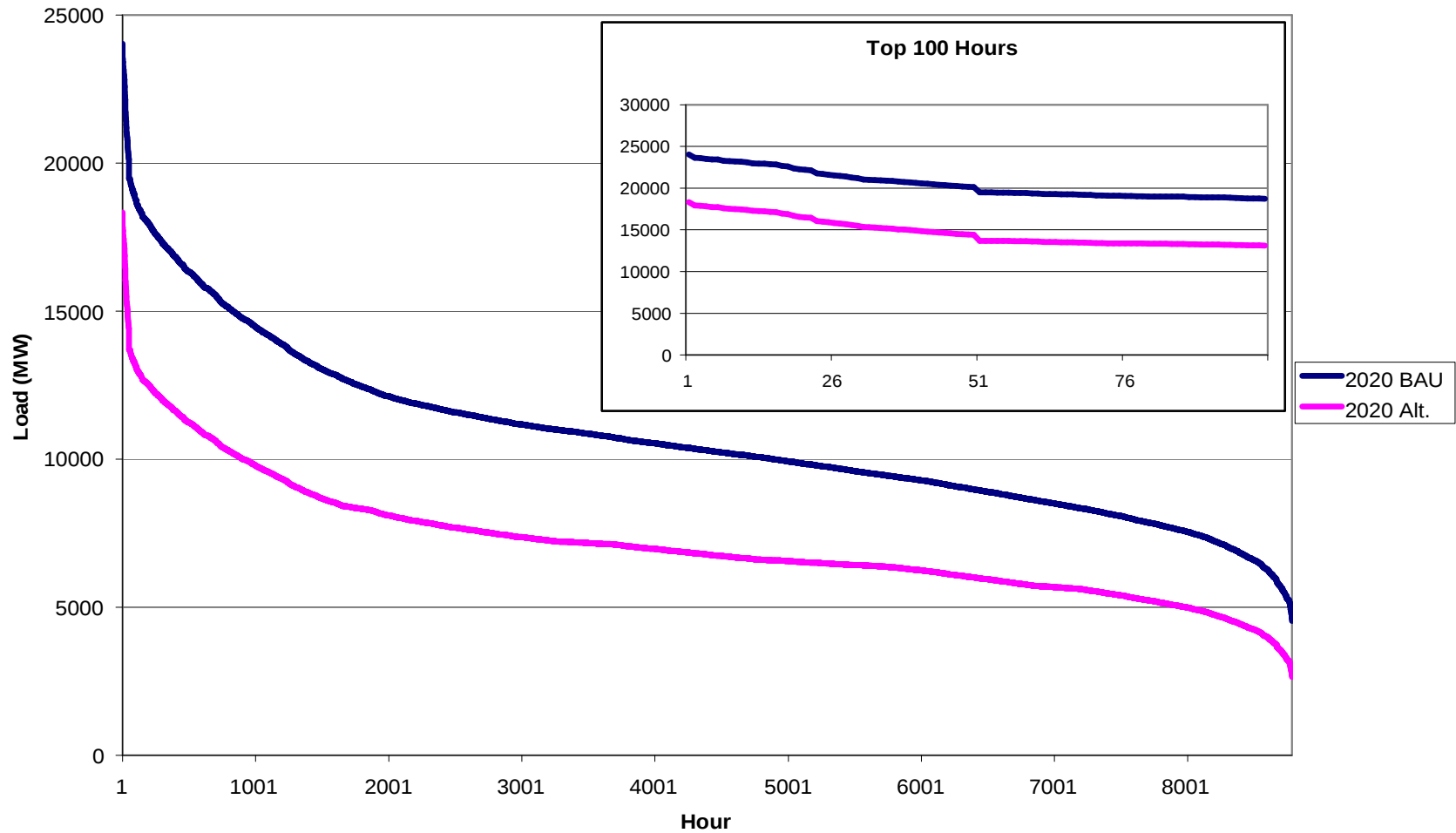
2020 BAU and Alternative Load Duration Curves
