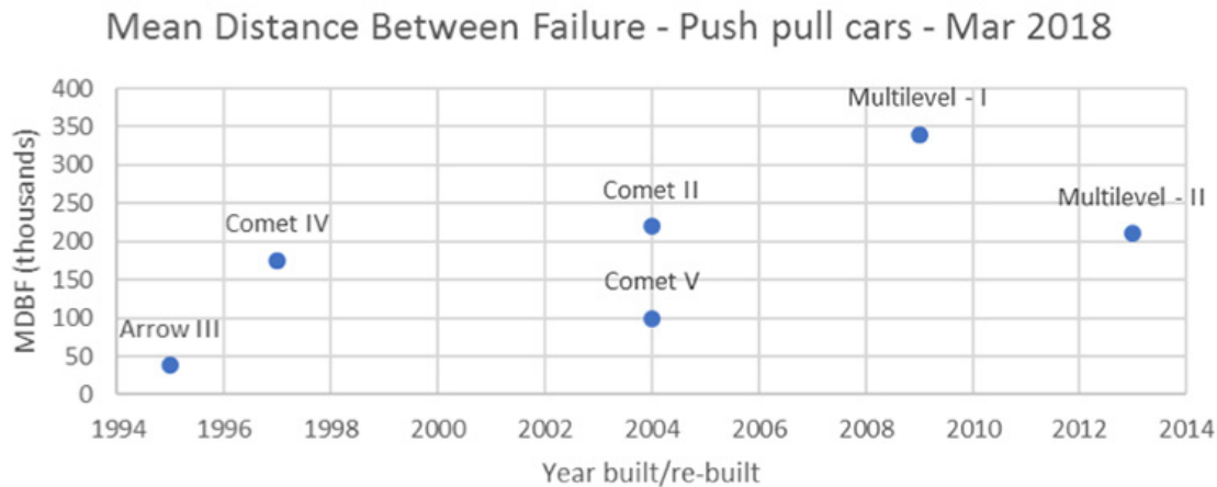
Figure 9-6: MDBF Against Age March 2018
