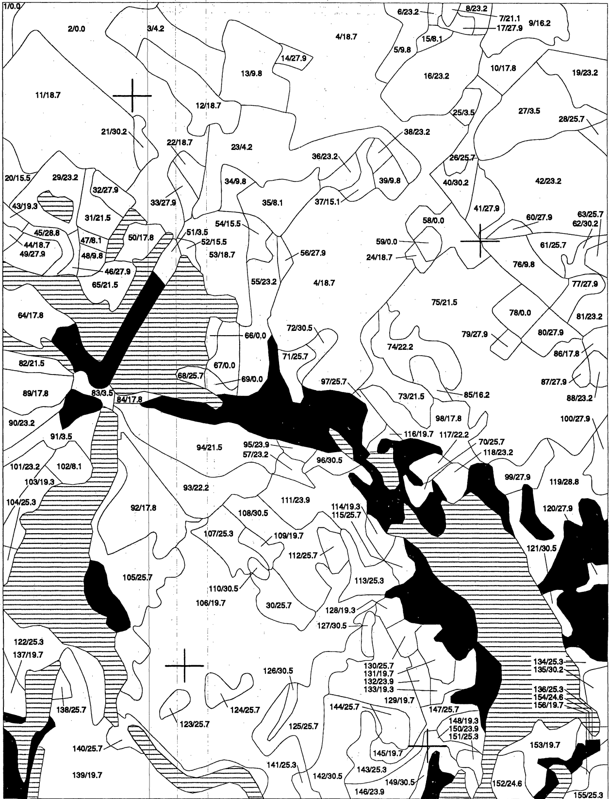
Figure 23. Step 6: Recharge base map. Number at left of slash is polygon code. Number at right of slash is recharge (in.yr). Shaded areas are the same as in figure 21.
