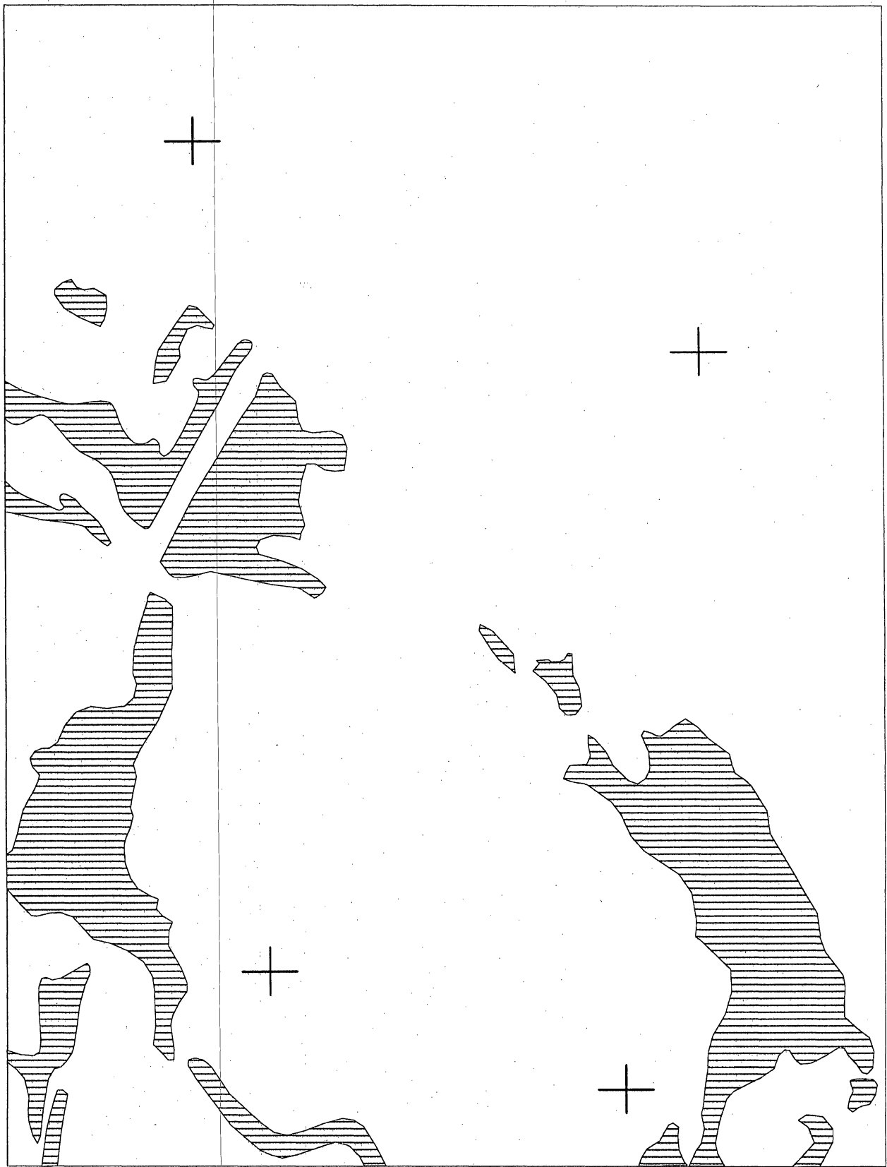
Figure 15. Step 2: Mylar template. Shading indicates surface water and wetlands (> 5 acres).
