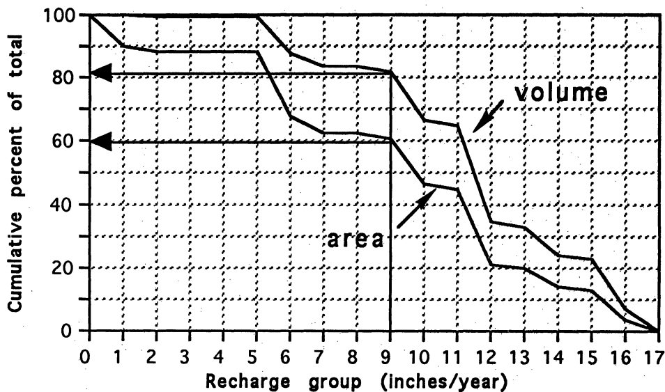
Figure 40. Cumulative volume and area vs. recharge group, NJGS test case.
