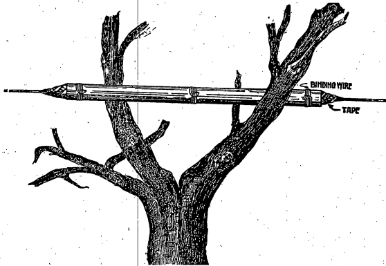
Fig 16. Abrasion moulding - used to protect trees and wires. (Courtesy of National Electric Light Assn.)
