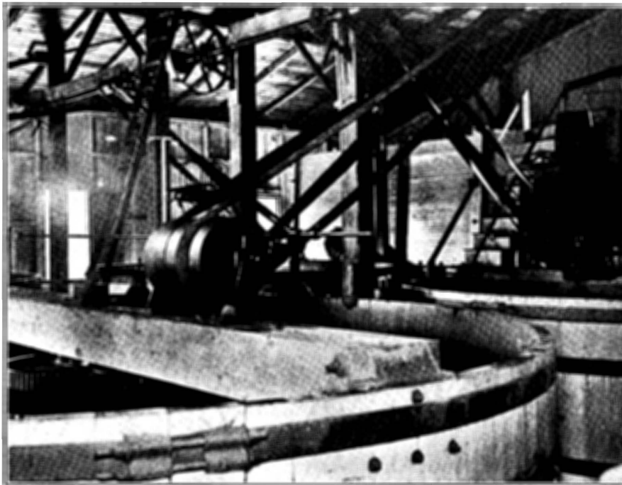
MILLVILLE: Water Filters and Hypochlorite Plant.
