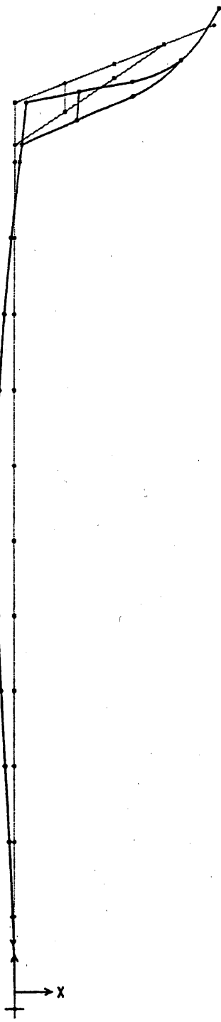
Figure 2-10 Cantilevered Support Standard Sixth Mode Shape.
