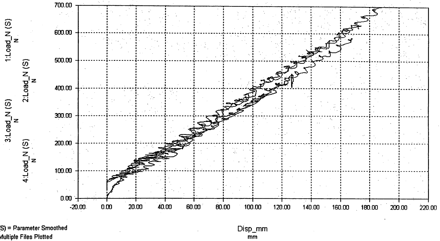
Figure 3-5 Stiffness of Cantilevered Support
