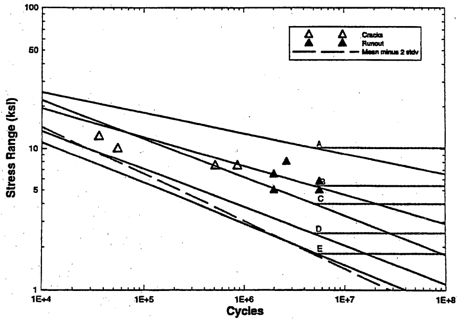
Figure 3-20 S-N Curve for Through-Thickness Cracks Including the Runouts.
