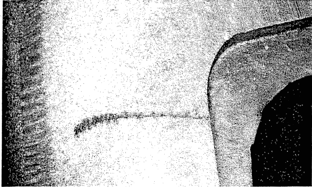
Figure 3-13 Fatigue Crack in Transformer Base of Specimen S-3
