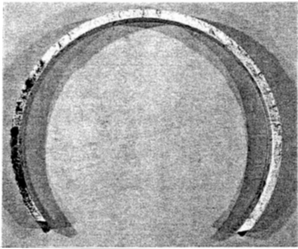
Figure 3-18 Typical Through-Thickness Weld Toe Crack.
