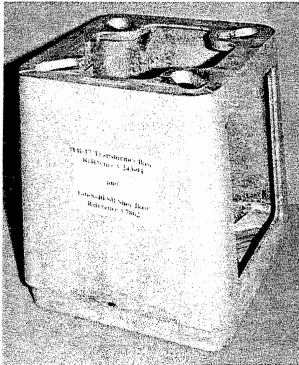
Figure 3-1 Cracked Transformer Base from Route 147.
