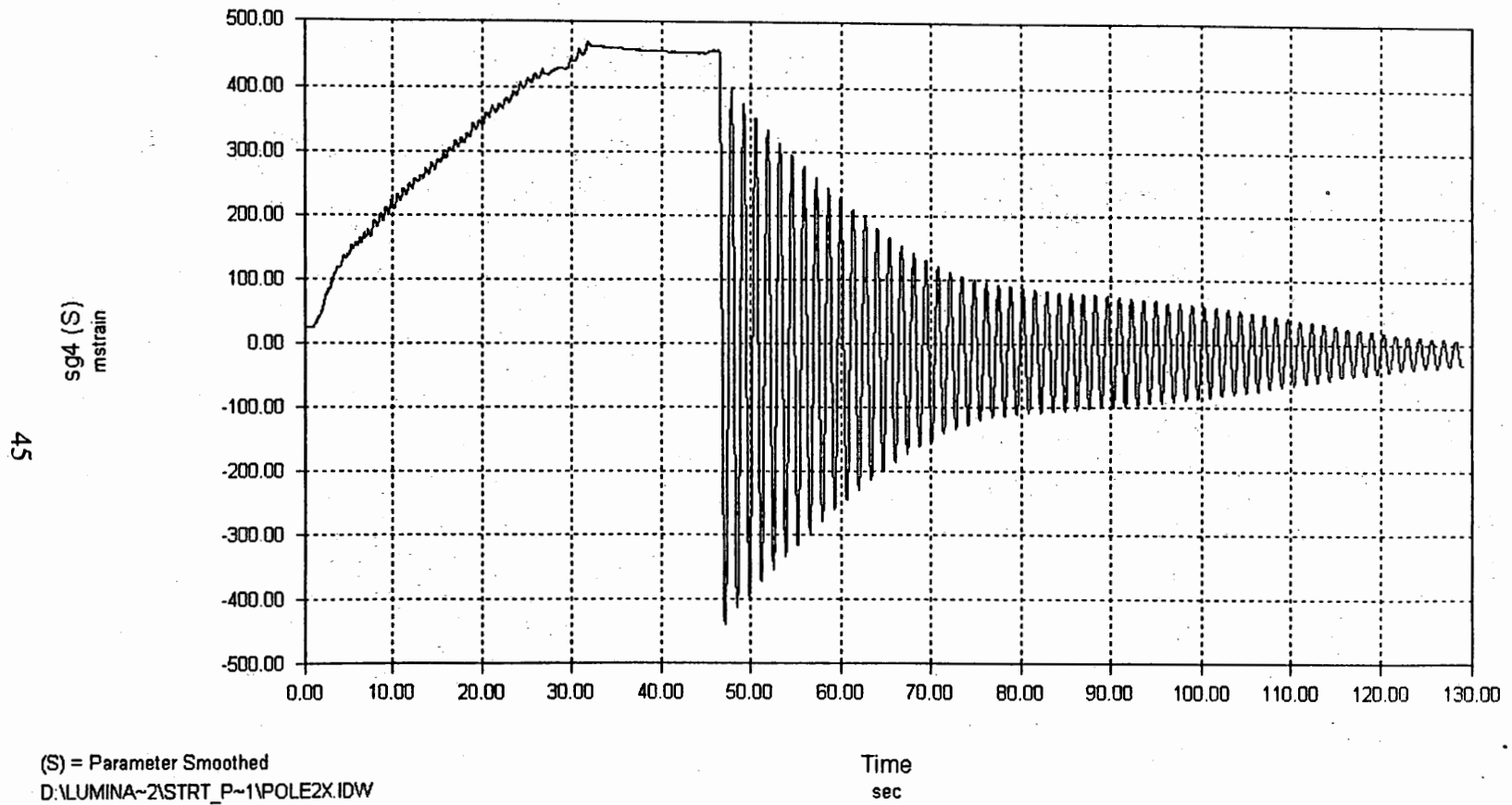
Figure 3-10 Damping of Motion in a Straight Support
