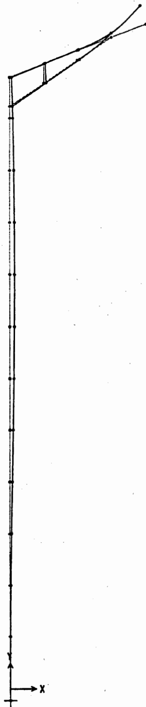
Figure 2-8 Cantilevered Support Standard Fourth Mode Shape.
