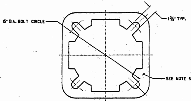
PLAN VIEW OF BASE N.T.S.
