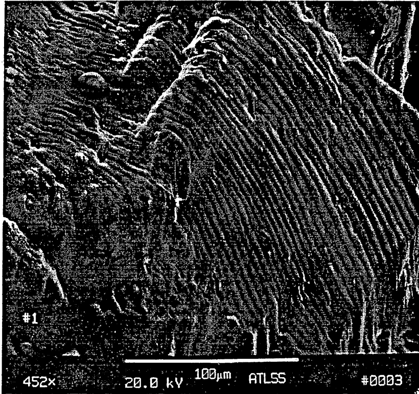
Figure 3-25 Striations from Cracked Pole on Route 147.
