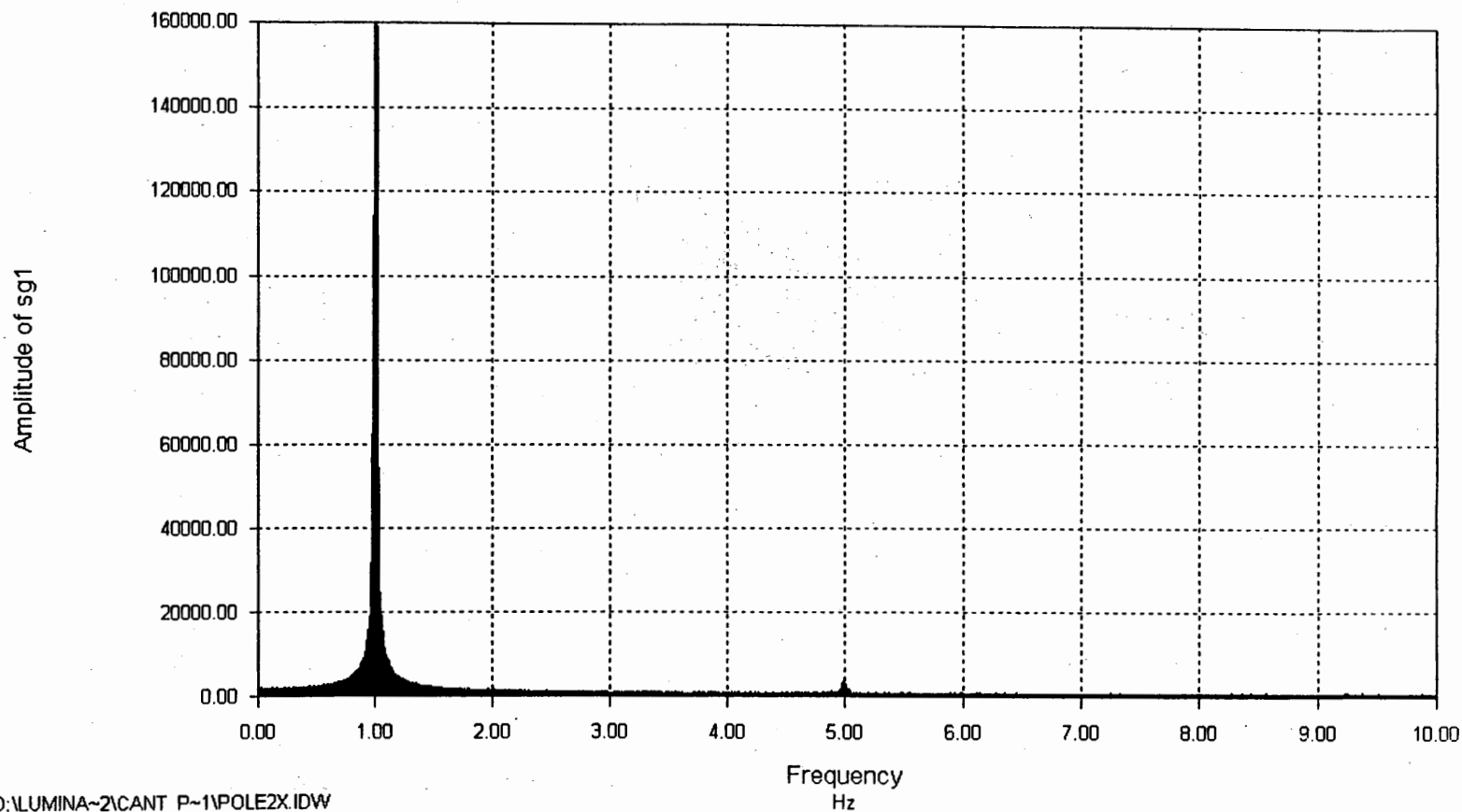
Figure 3-6 Natural Frequency of Cantilevered Support
