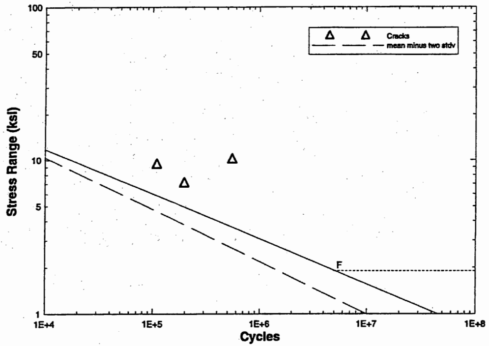
Figure 3-23 S-N Curve for Shear Stress Range Induced Cracks
