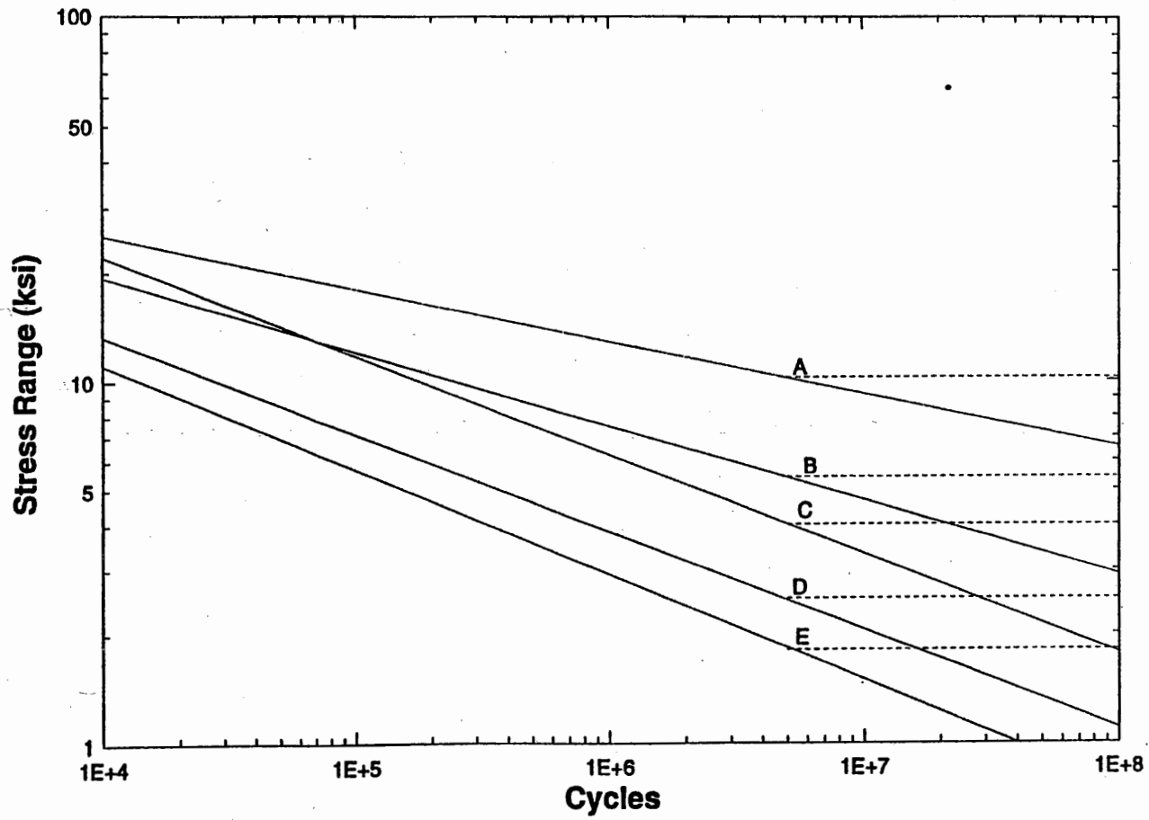
Figure 2-13 S-N Curves for Aluminum.
