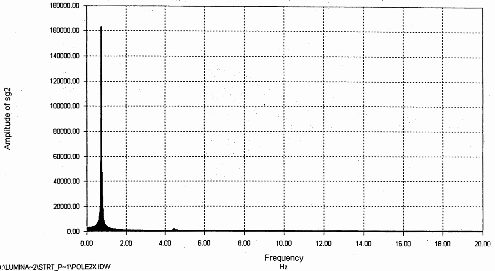
Figure 3-9 Natural Frequency of Straight Support
