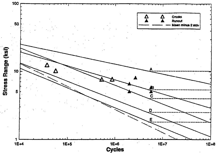
Figure 3-19 S-N Curve for Through-Thickness Cracks Not Including the Runouts.
