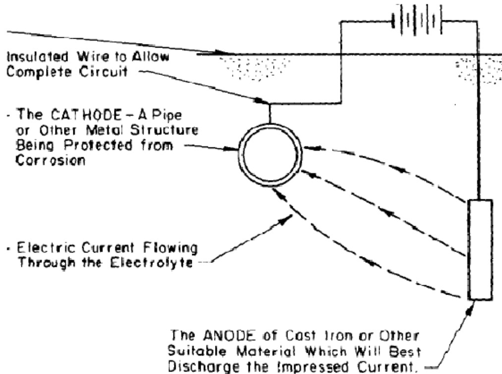
Figure 15: Impressed Current System
