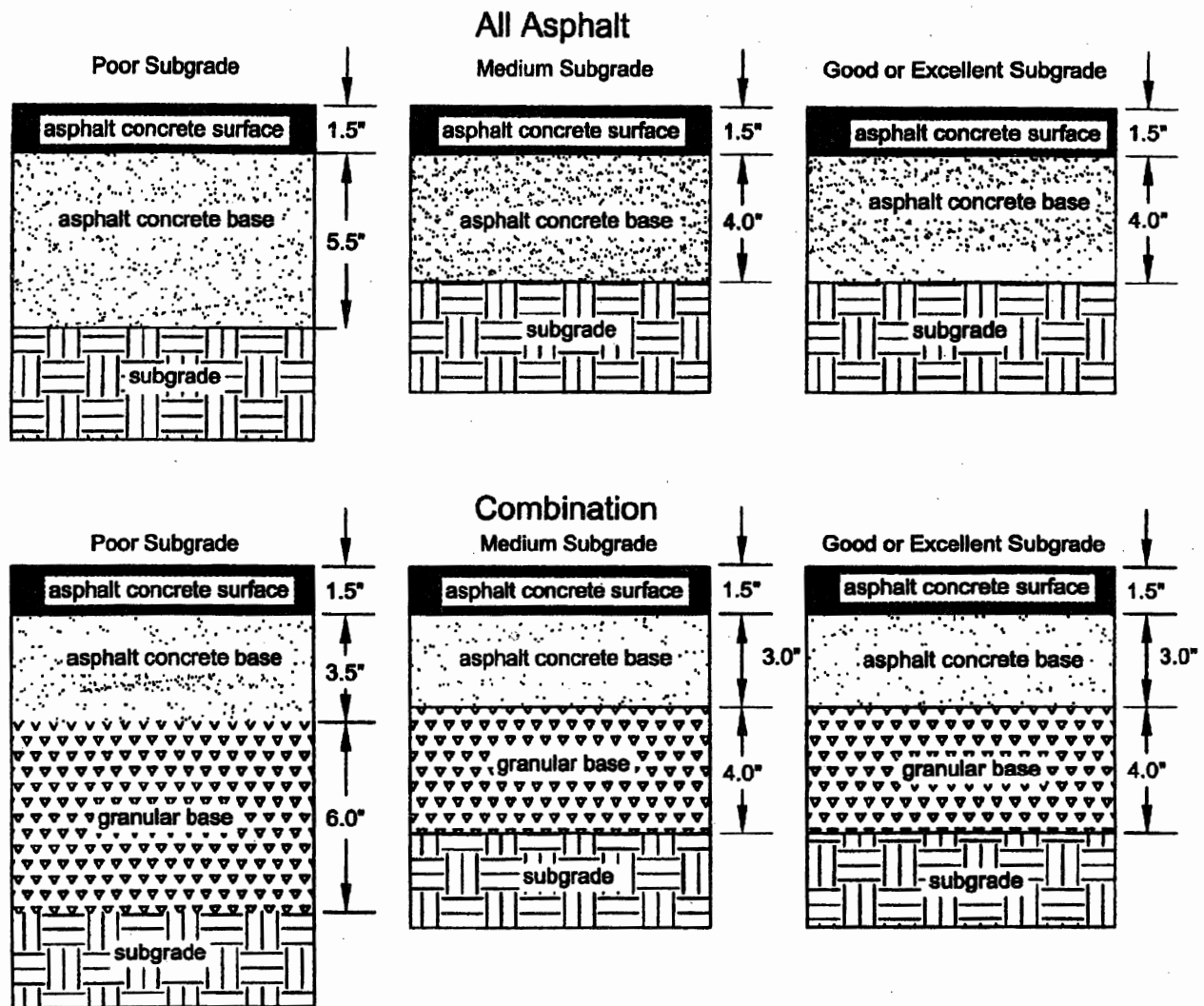
Figure 4.2 Pavement Sections for Rural Residential Lanes, Rural Streets, Cul-de-Sacs, and Alleys (ADT \leq 500) (EAL \leq 30,000)
