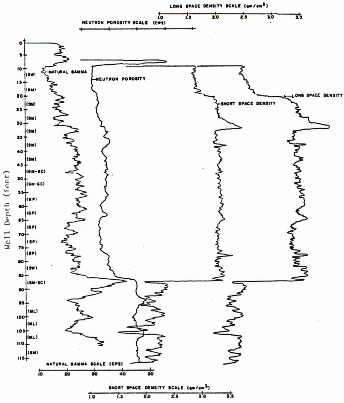
Geophysical logs of Test Well TW-8.
