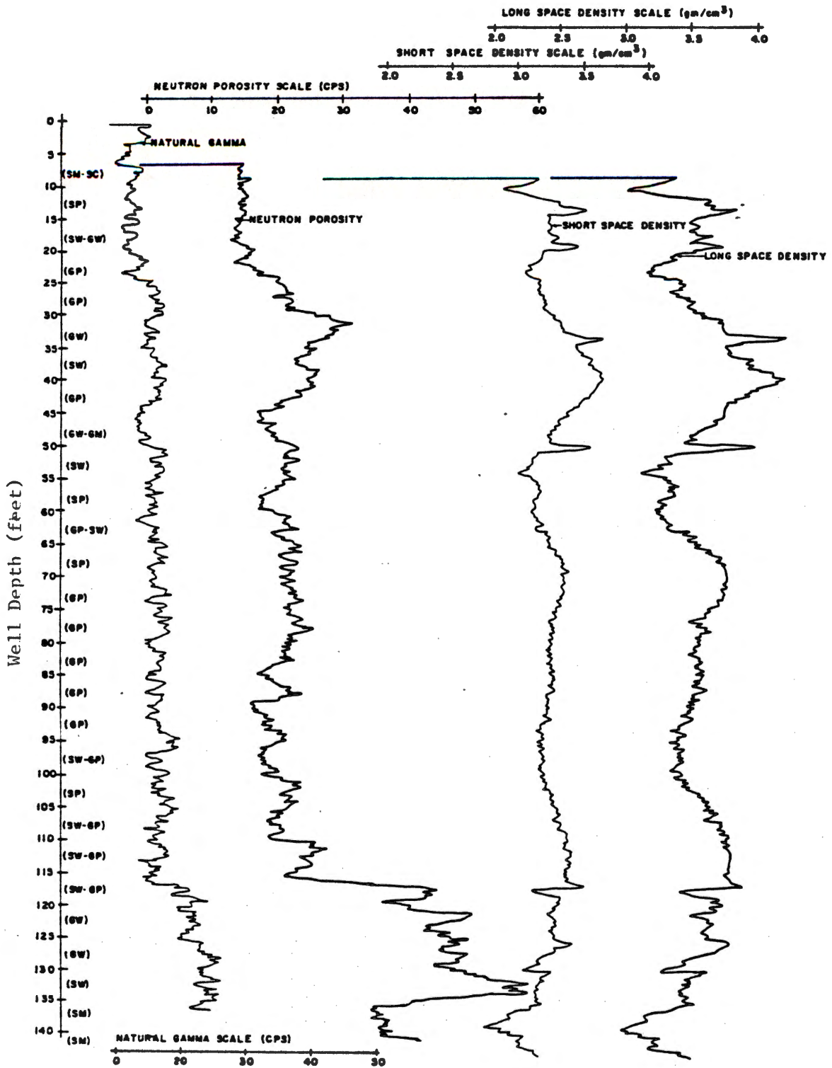
Geophysical logs of Test Well TW-5.
