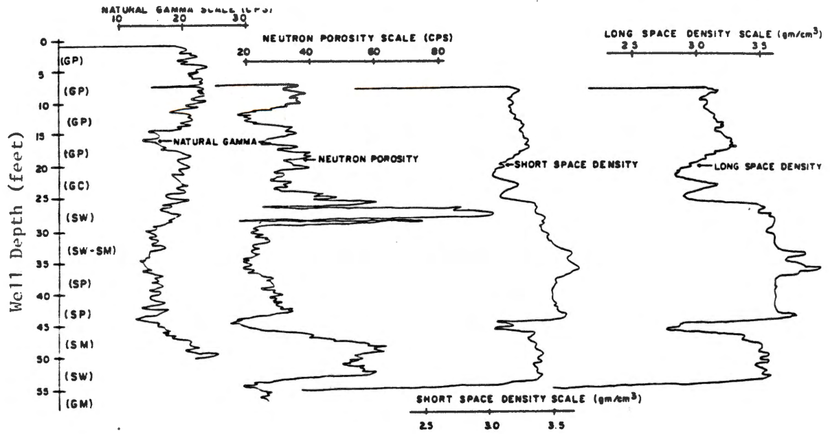
Geophysical logs of Test Well TW-11.
