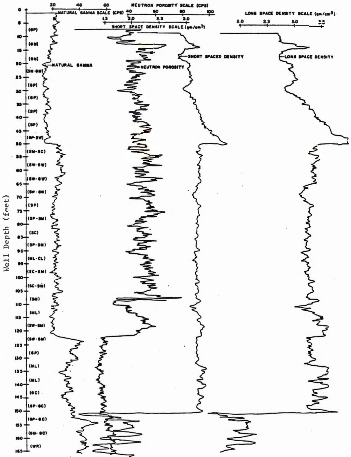
Geophysical logs of Test Well TW-1.
