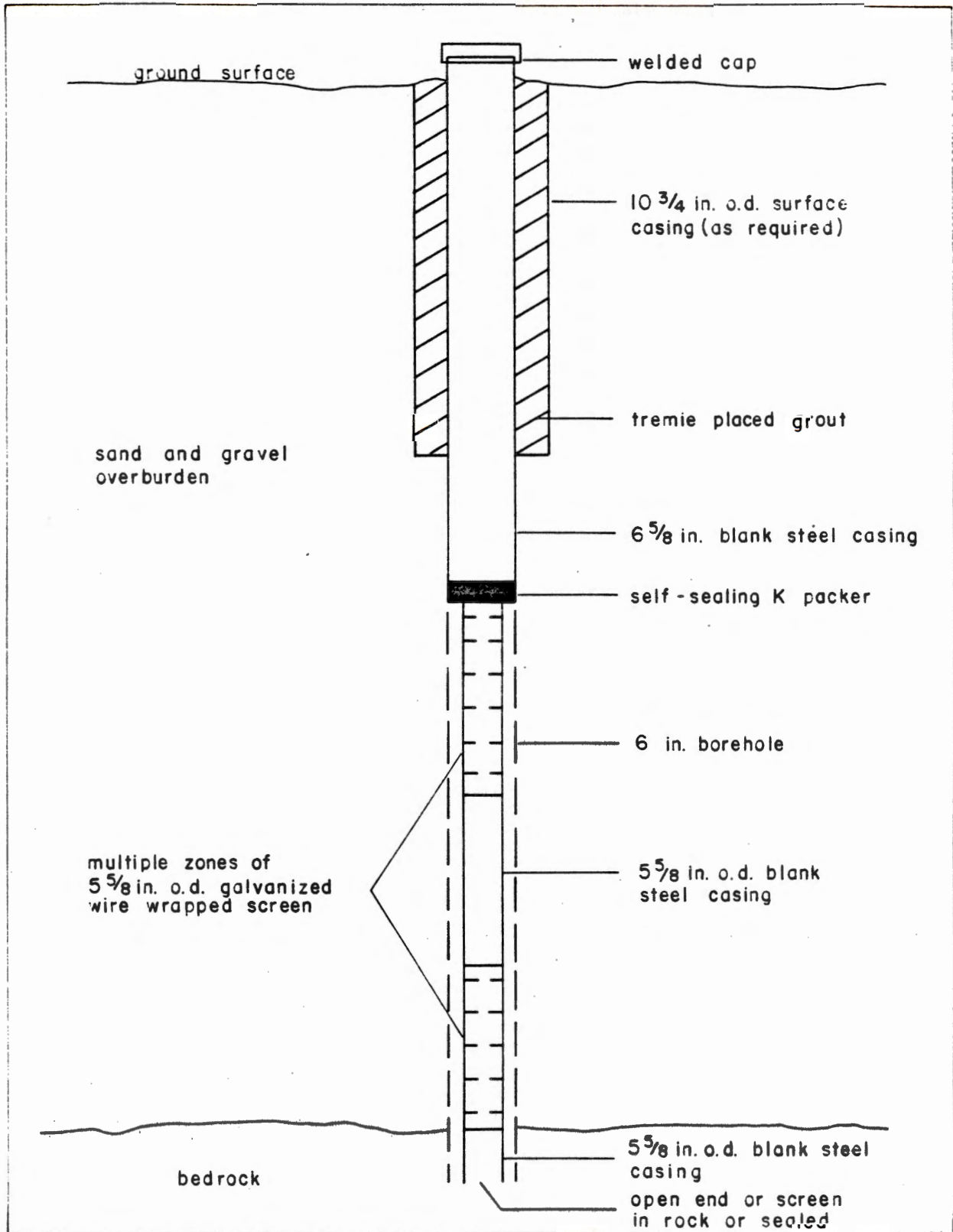
Figure 11. Construction of test wells used in the study.
