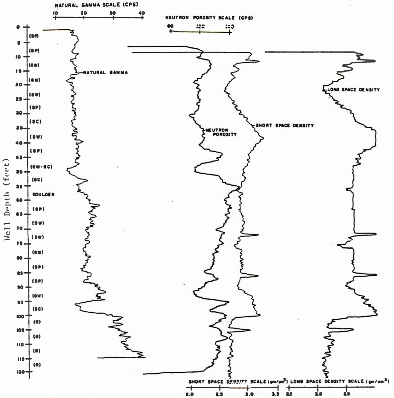
Geophysical logs of Test Well TW-10.
