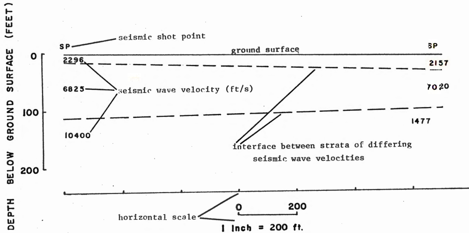
Explanation of cross sections from seismic traverses. Locations shown on Plate 2.
