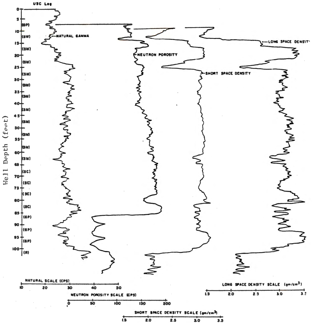
Geophysical logs of Test Well TW-9.
