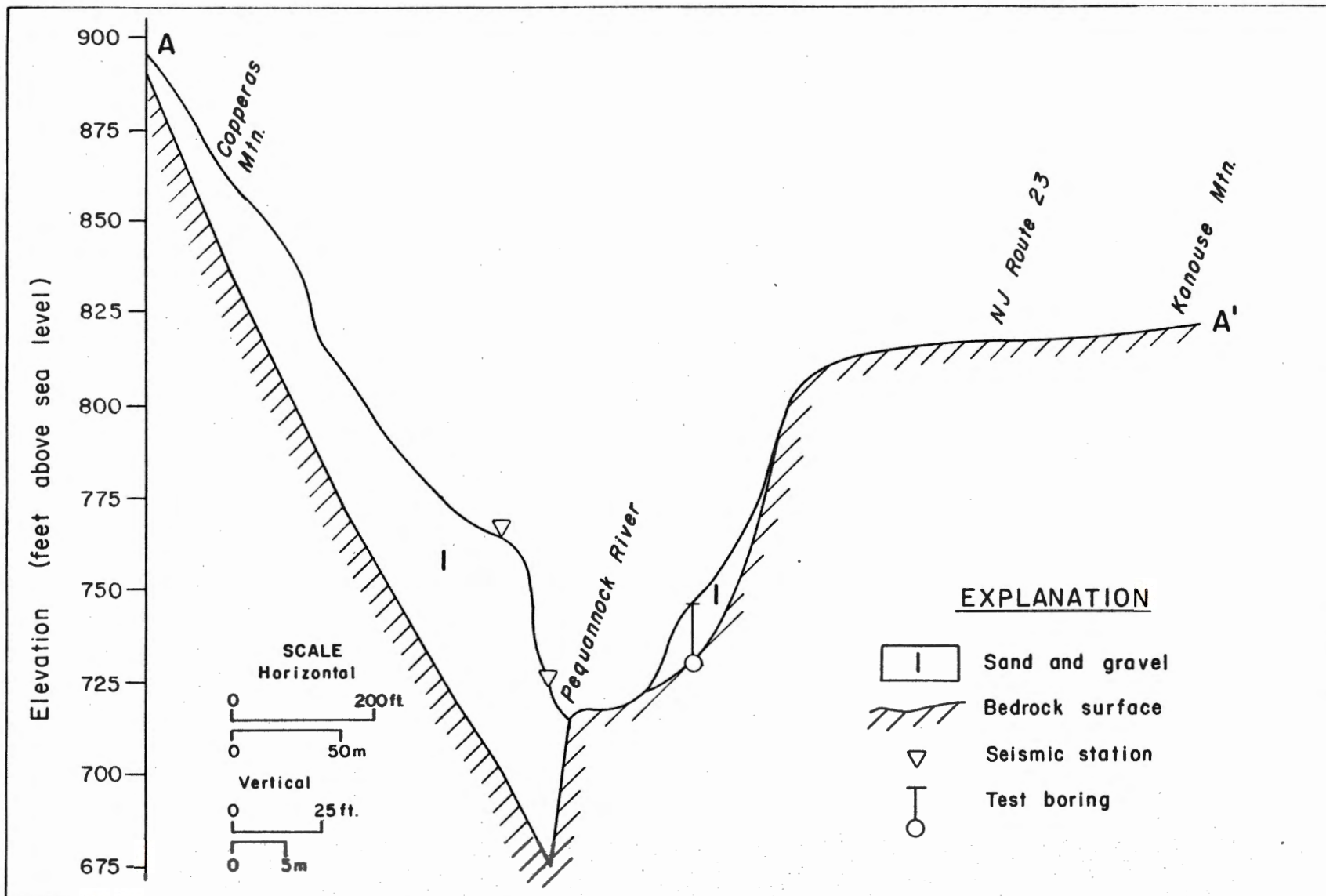
Figure 3. Profile of bedrock surface at gap between Copperas and Kanouse Mountains from reflection and refraction seismology and test boring.
