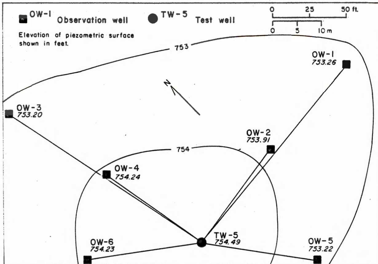
Figure 5. Array of observation wells for TW-5 aquifer test in Area 1, and piezometric surface before pumping.
