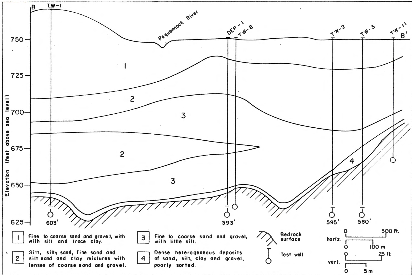
Figure 4. Cross section of valley fill deposits along the Pequannock River in Area 1, Jefferson and Rockaway Townships.
