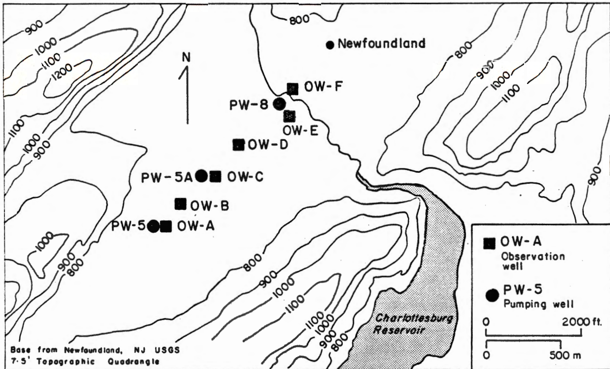
Figure 6. Map of pumping wells and observation wells in TIP Simulation at Area 1.
