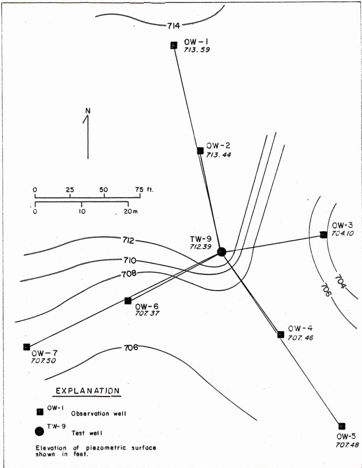
Figure 10. Array of observation wells for TW-9 aquifer test in Area 4, and piezometric surface before pumping.
