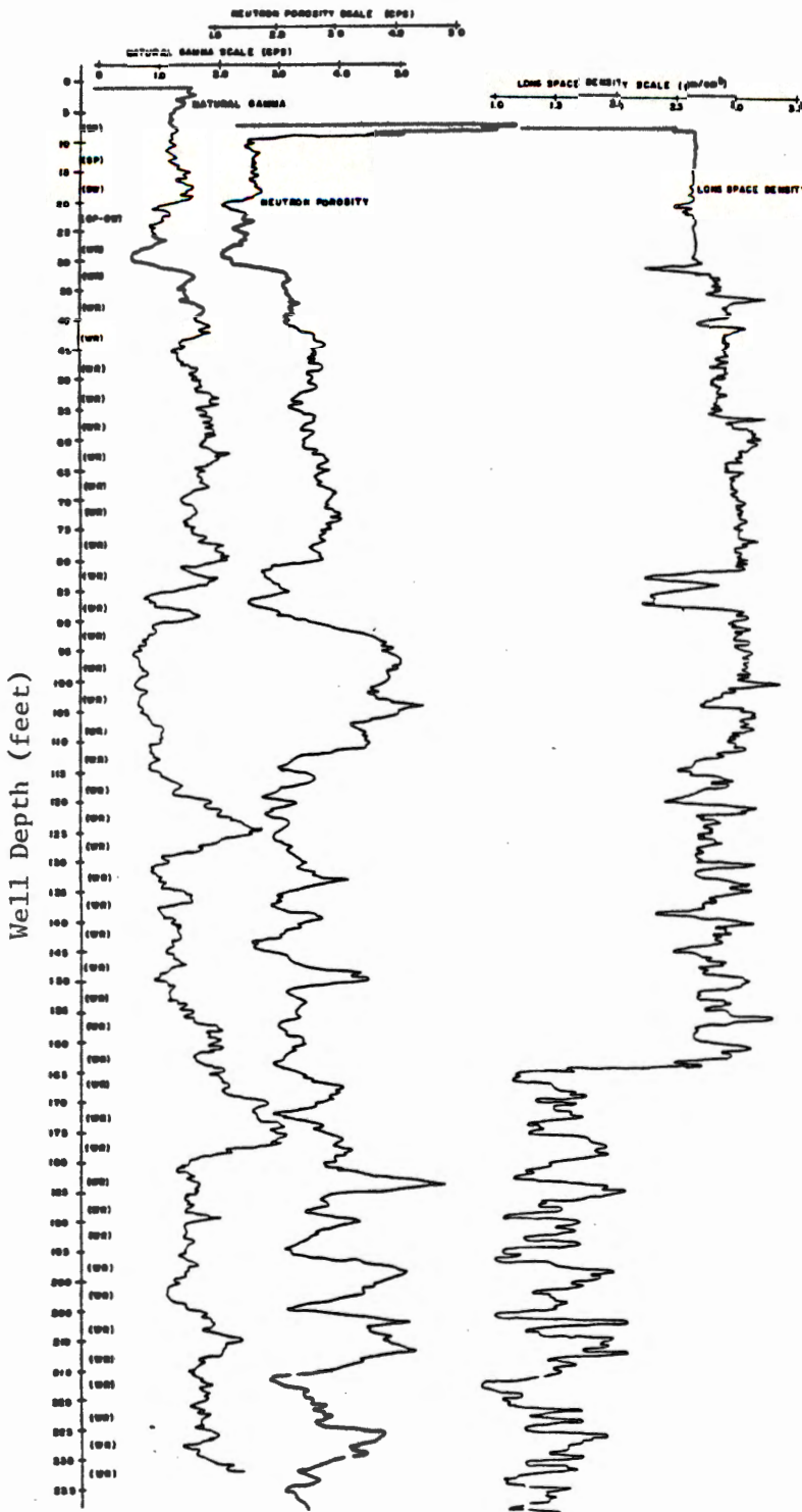
Geophysical logs of Test Well TW-6.
