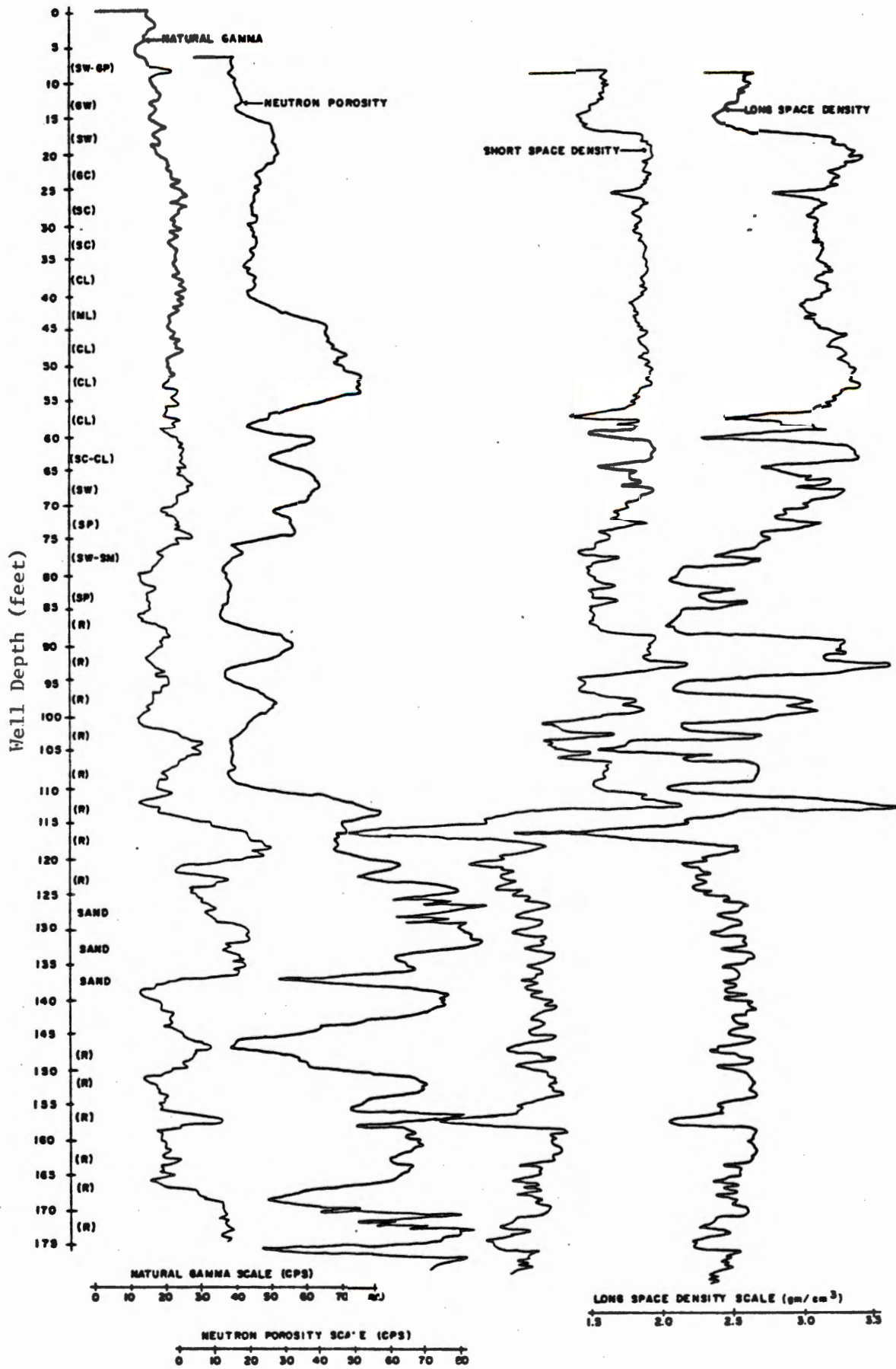
Geophysical logs of Test Well TW-3.
