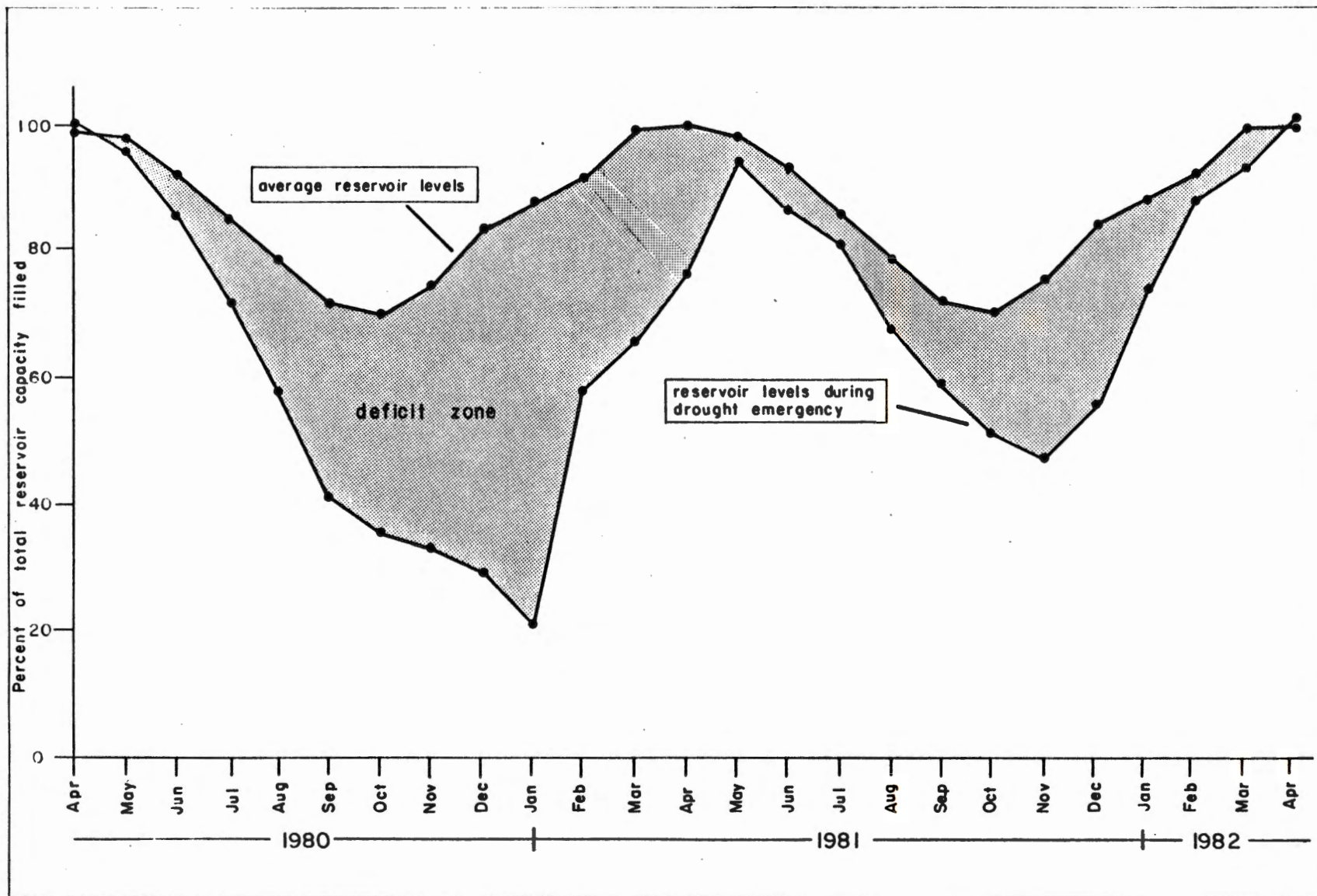
Figure 1. Graph comparing reservoir capacity filled, 1980-82 to long-term average filled capacity. Includes Boonton, Canistear, Charlottesville, Clinton, Oak Ridge, Oradell, Split Rock and Wanaque Reservoirs, Echo and Woodcliff Lakes, Lake DeForest and Lake Tappan.
