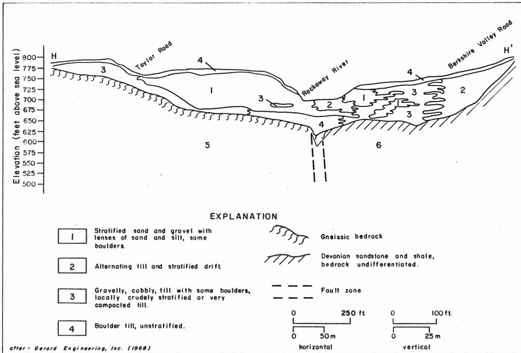
Figure 9. Cross section of bedrock surface and valley fill deposits in Berkshire Valley, Area 4.
