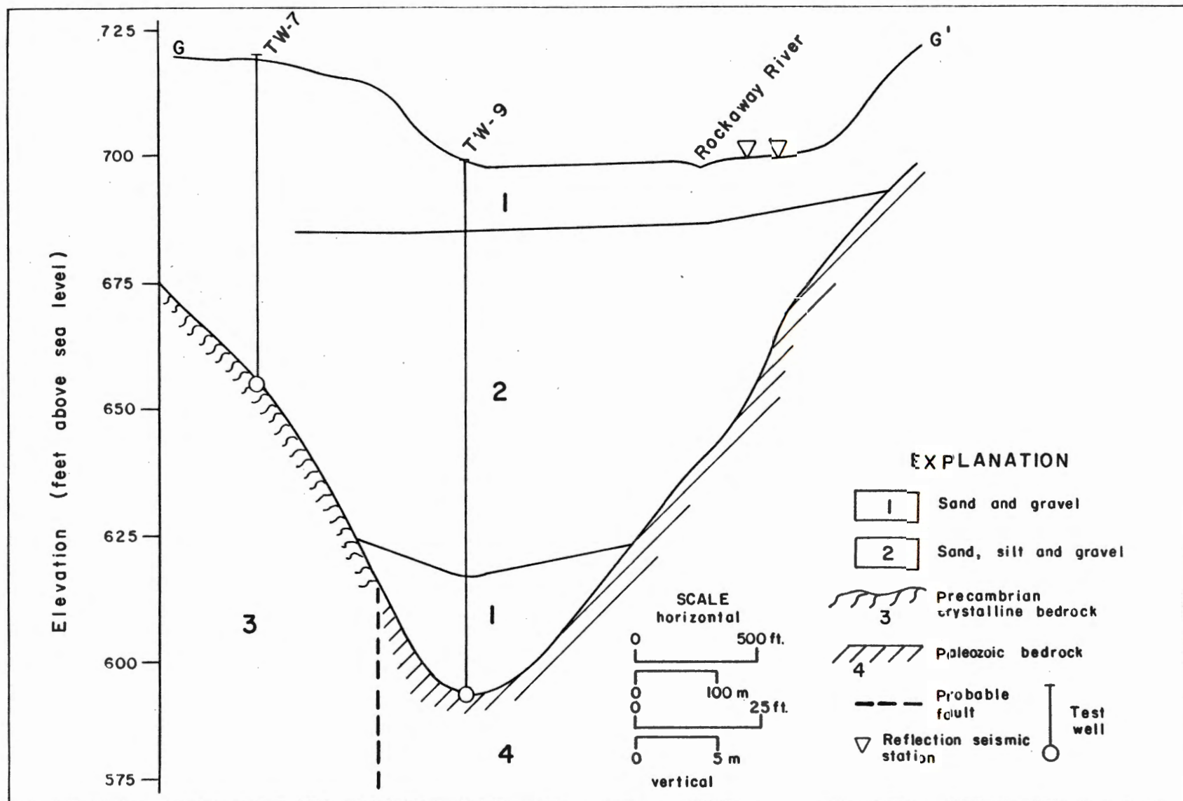
Figure 8. Cross section of valley fill deposits in Lower Berkshire Valley, Area 4, Jefferson Township.
