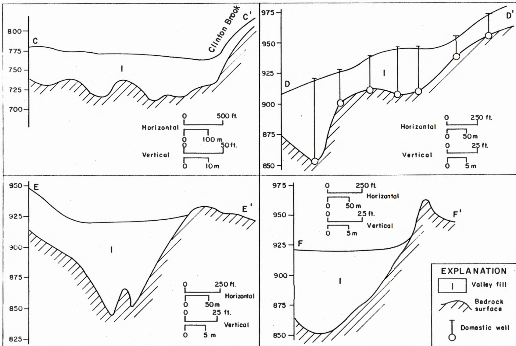
Figure 7. Profiles of bedrock surface in Area 2, West Milford Township. Elevations are in feet above sea level. C-C': Along LaRue Road as interpreted from reflection seismology. D-D': Along Gould Road as interpreted from domestic water well logs. E-E': Across bog North of Echo Lake as interpreted from reflection seismology. F-F': Along Wooley Road as interpreted from reflection seismology.
