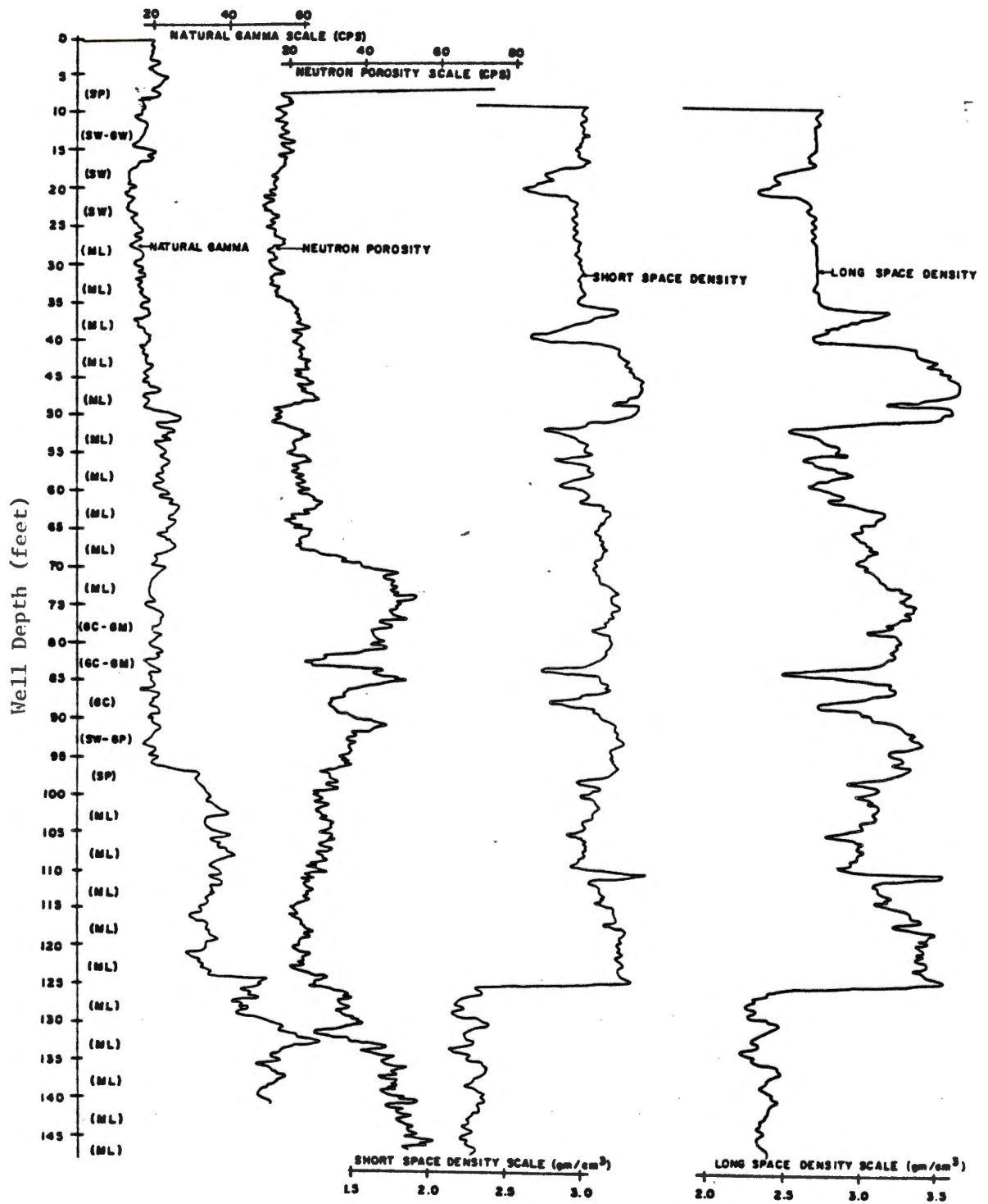
Geophysical logs of Test Well TW-2.
