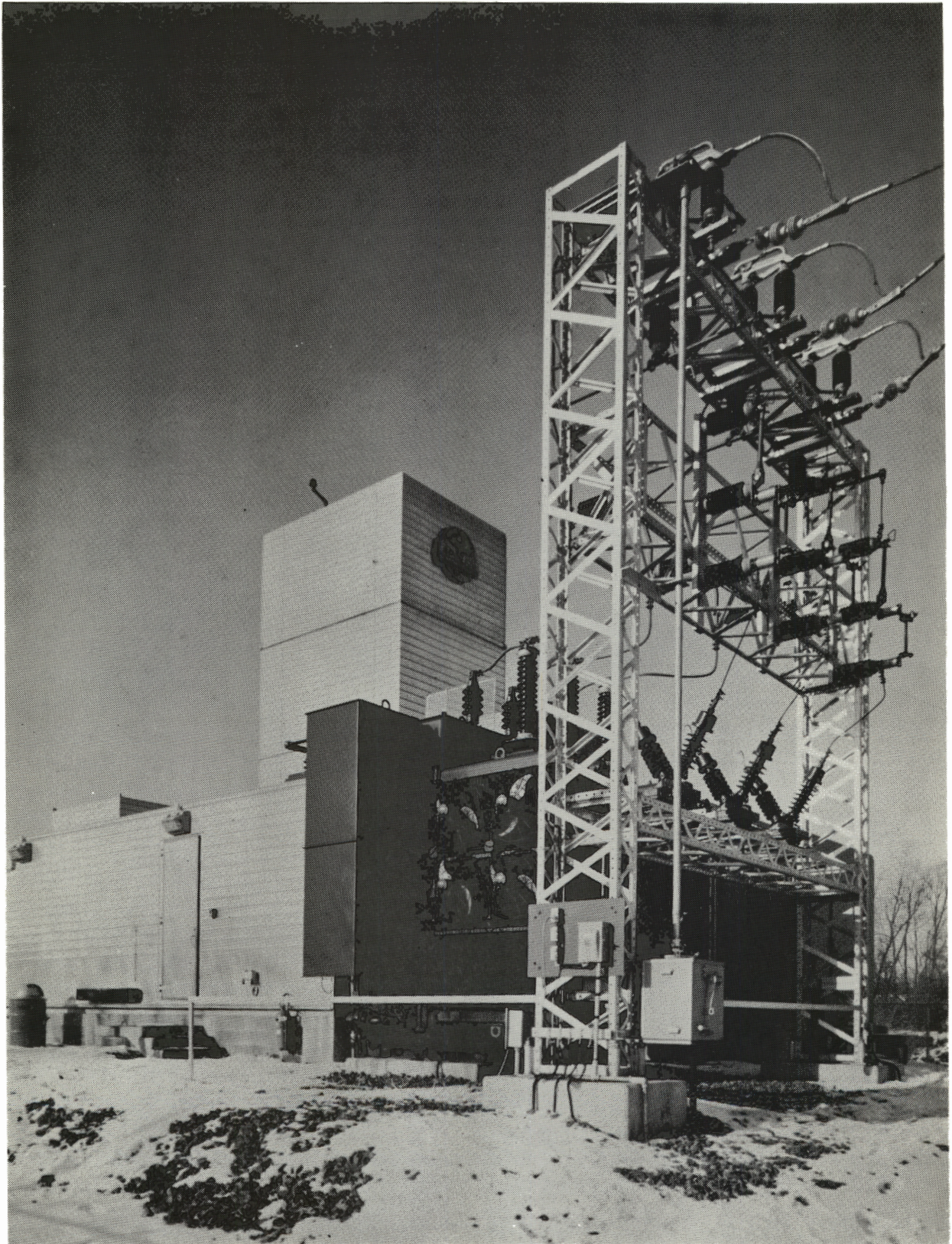
Public Service Electric and Gas Company's 20,000 kilowatt gas-turbine generator in Gloucester County.
