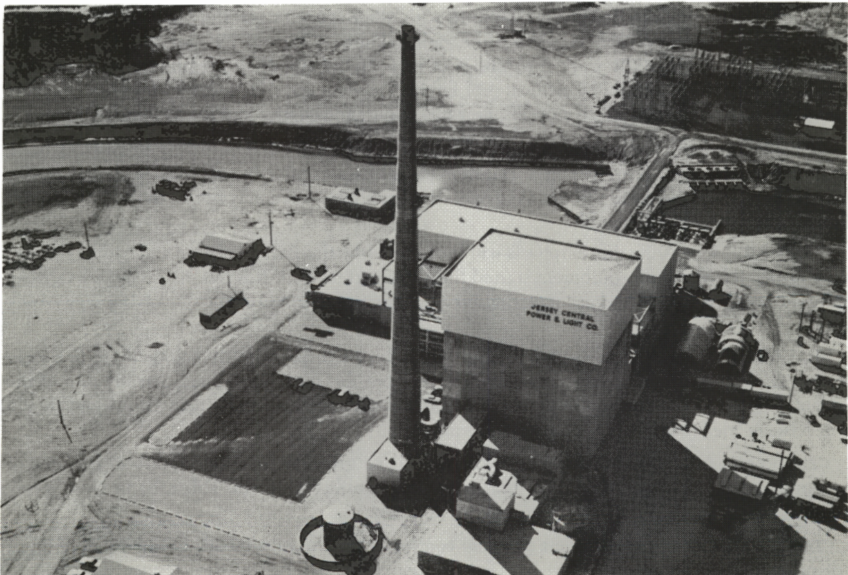
The Oyster Creek Nuclear Generating Station in Lacey Township, Ocean County, is New Jersey's only atomic-powered generating plant. It is owned by the Jersey Central Power and Light Company.
