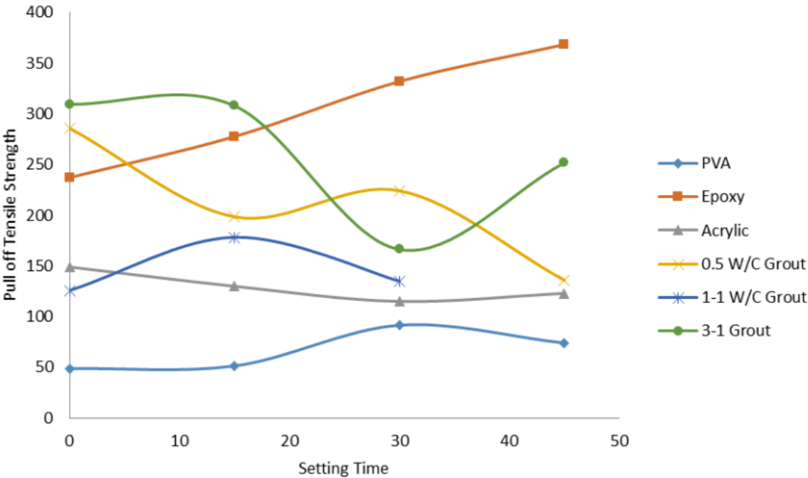
Figure 9. Pull-off tensile strength of repair material for various bonding agents for different setting times after 5 months (13)
