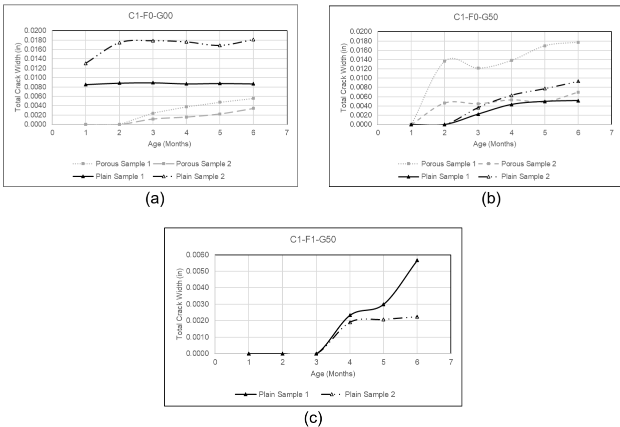
Figure 35. Growth of total crack width over time for C1 samples: (a) C1-F0-G00; (b) C1-F0-G50; (c) C1-F1-G50
