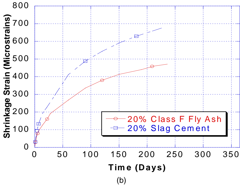
Figure 17 Plot of (a) the Specific Creep and (b) Shrinkage of SCC Containing 20% slag cement and 20% Class F Fly Ash
