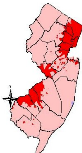
Figure 3 NATA PREDICTED CONCENTRATIONS IN NEW JERSEY FOR 1996
