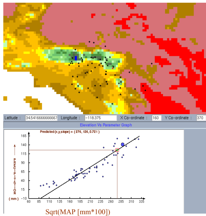
Figure 5. PRISM graphical user interface showing: (a) 1-hour index flood precipitation vs mean annual precipitation ( \text{sqrt}(\text{MAP}) ); and (b) 24-hour index flood precipitation vs \text{sqrt}(\text{MAP}) , San Bernardino Mountains, CA. Size of dot indicates relative weight of station in regression function.
