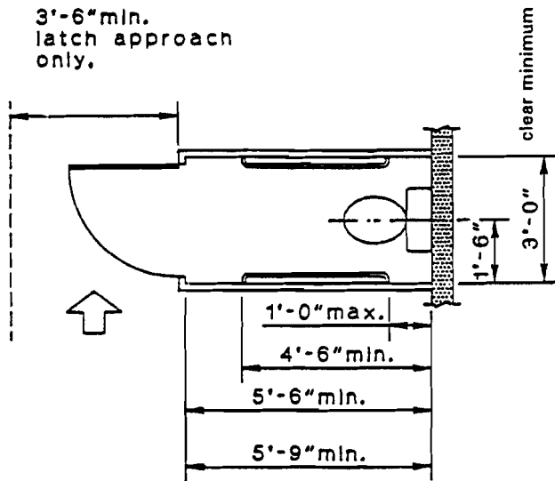
Figure 7.56b Alternate Stall
