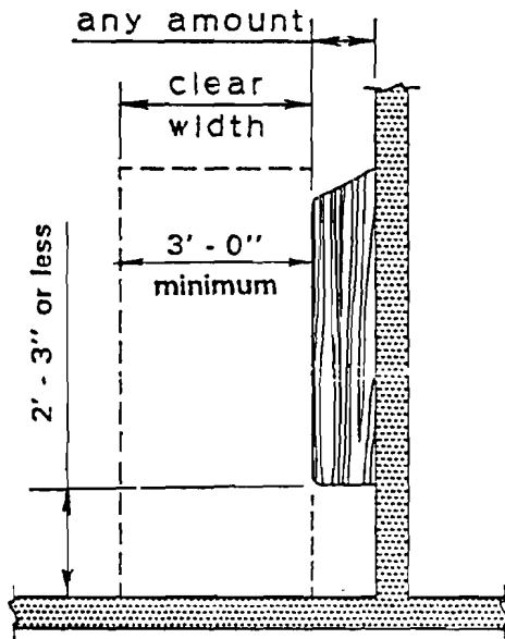
Figure 7.20c Clear Width
