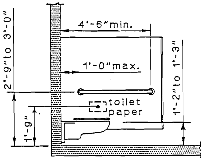
Figure 7.56d Side Wall
