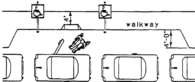
Figure 7.13c Parking Spaces
