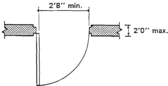
Figure 7.42b Sliding Door
