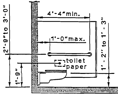
Figure 7.55d Side Wall
