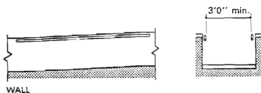
Figure 7.30c Ramp with Vertical Guards
