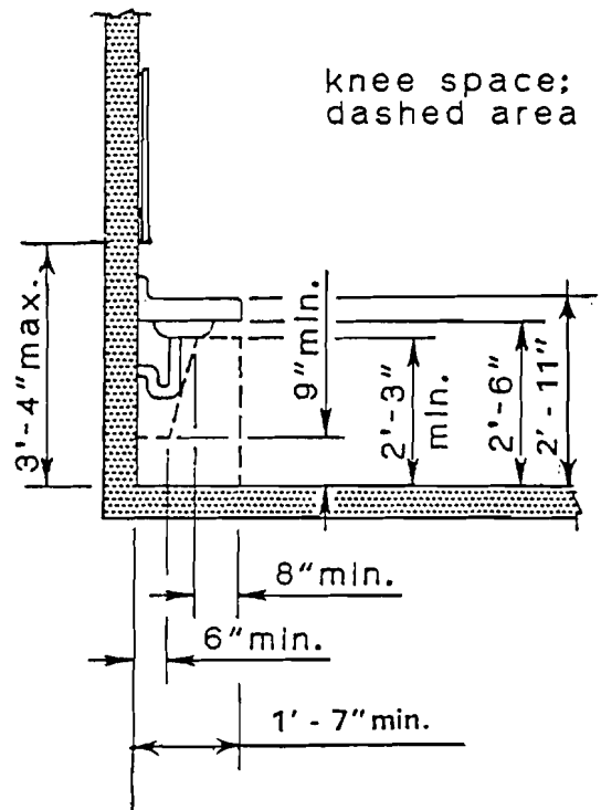
Figure 7.58a Lavatory
