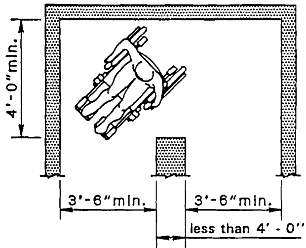
Figure 7.19c Turn-Maneuvering Clearance
