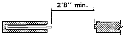
Figure 7.42c Folding Door
