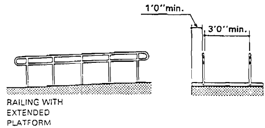
Figure 7.30d Ramp with Extended Platform
