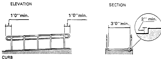
Figure 7.30b Ramp with Wall
