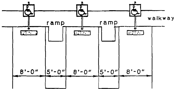
Figure 7.13b Parking Spaces
