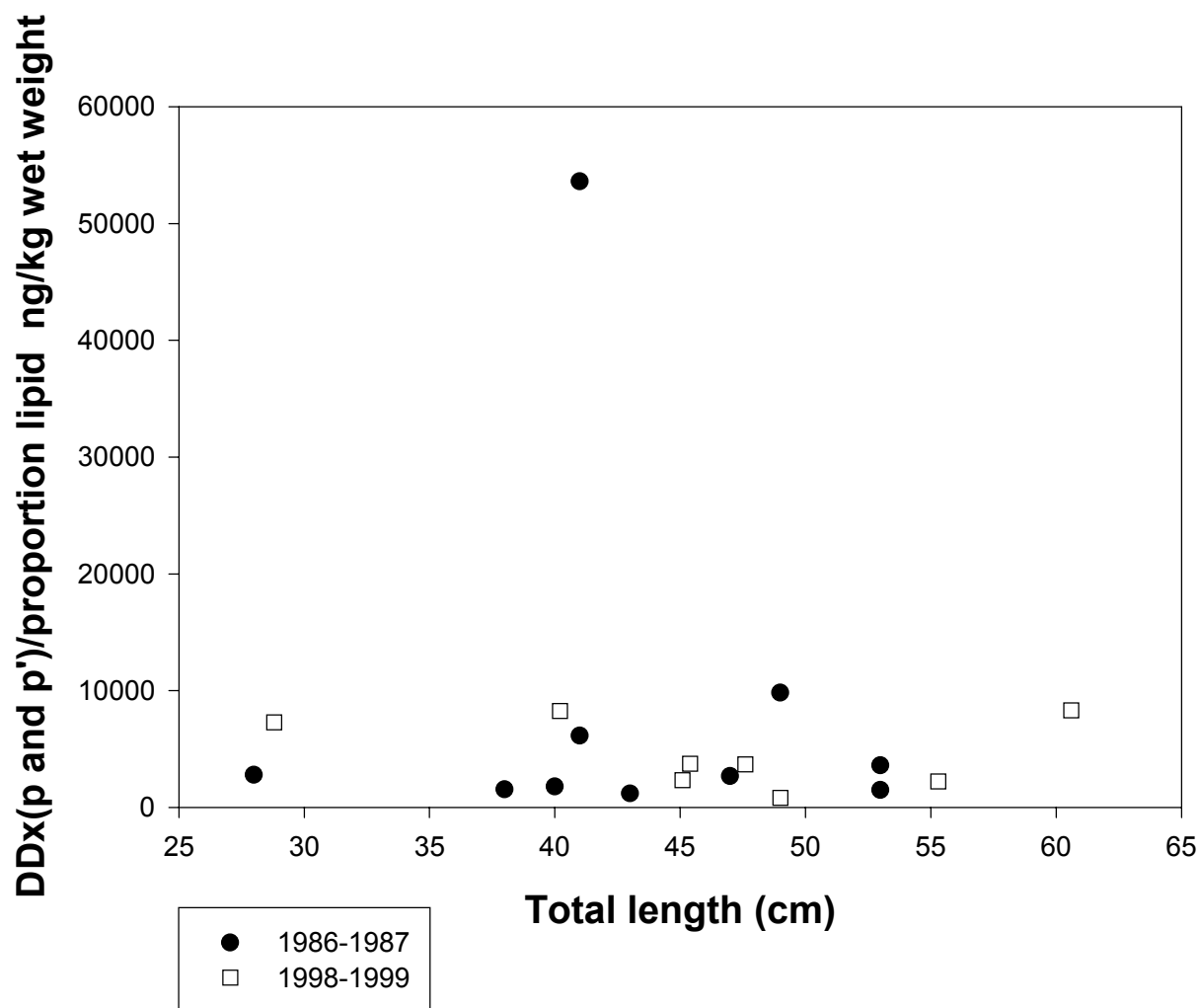
Figure 16. Relationship between lipid normalized DDX concentrations and length for American eel from Northeastern sites from 1986-87 and 1998-99.
