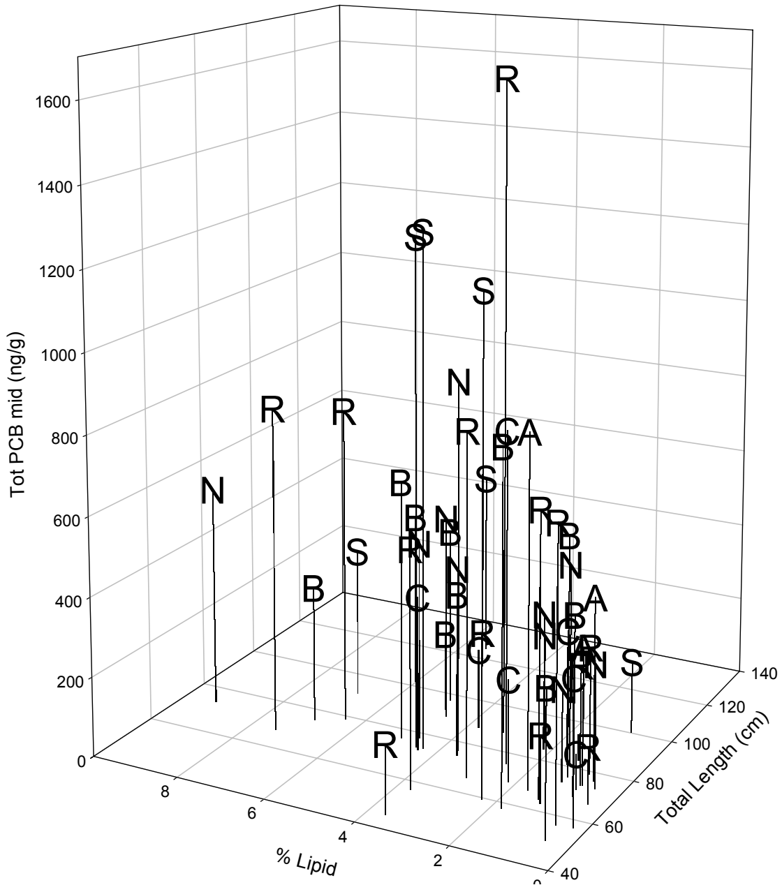
Figure 7. Relationship between total PCB concentration (ng/g wet weight), lipid content (%) and total length (cm) in striped bass.
