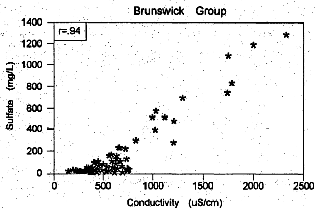
Figure 4. Scatter diagram showing dissolved sulfate and conductivity for ground water samples from the sedimentary rocks of the Brunswick Group, New Jersey.
