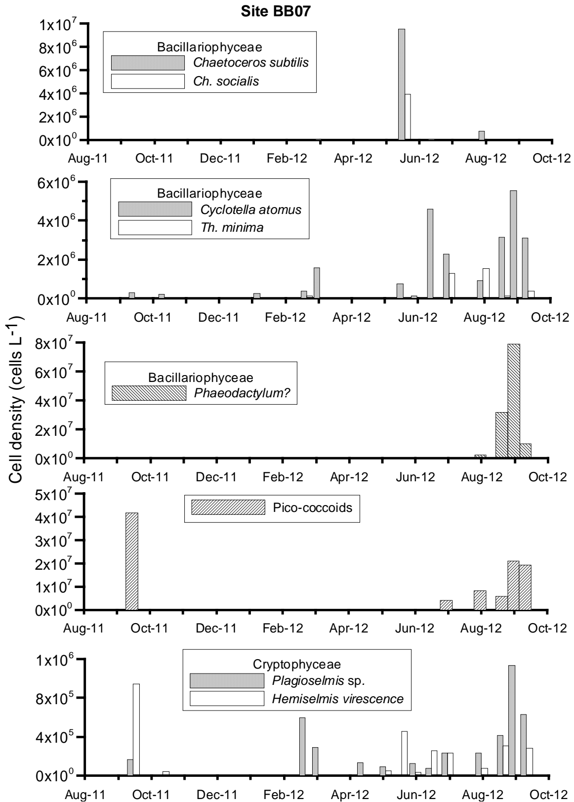
Fig. 10. Abundance and seasonal changes of some dominant species at site BB07 (BB07a) from August 2011 to September 2012.
