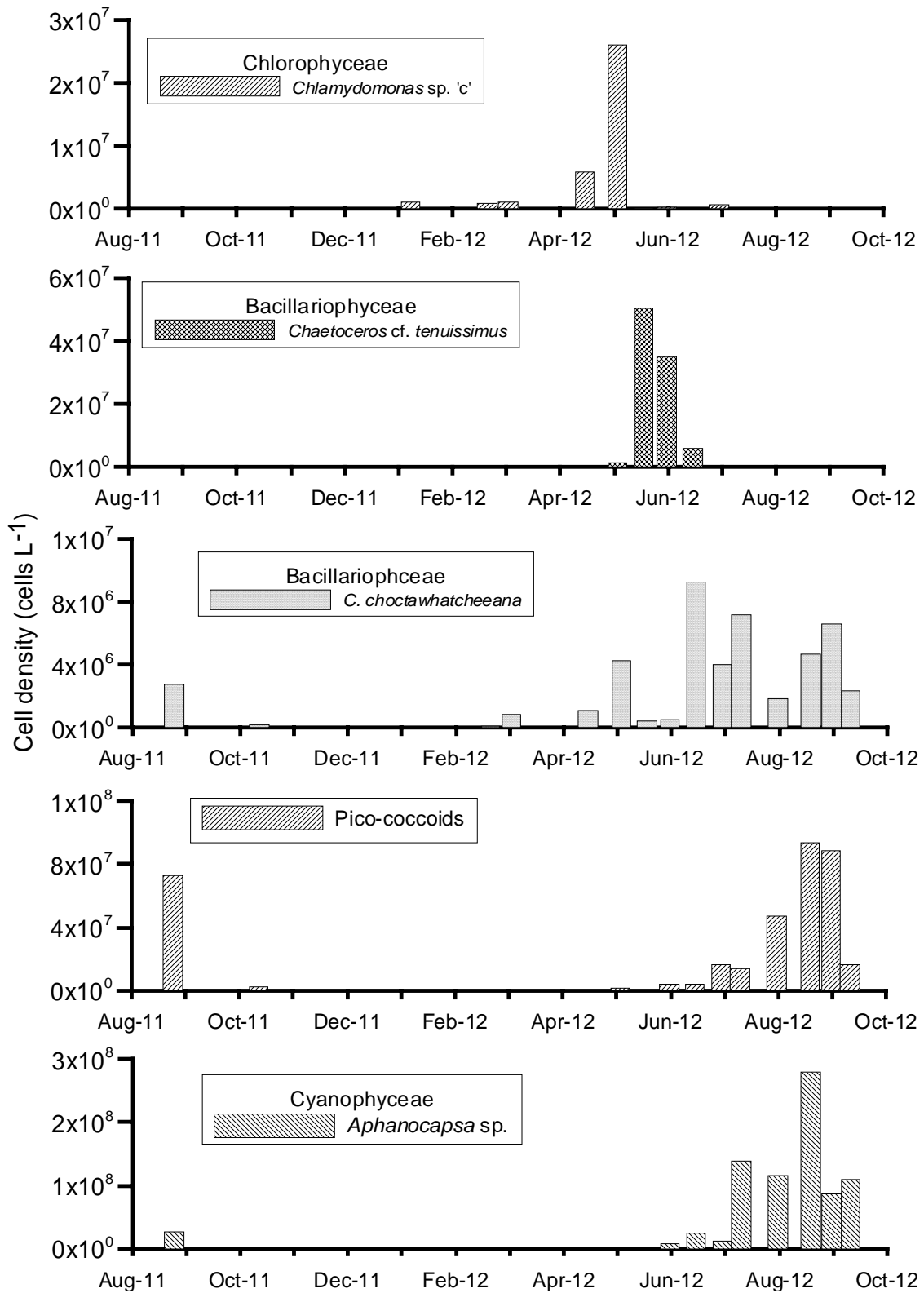
Fig. 6. Abundance and seasonal changes of some dominant species at site BB01 from August 2011 to September 2012.
