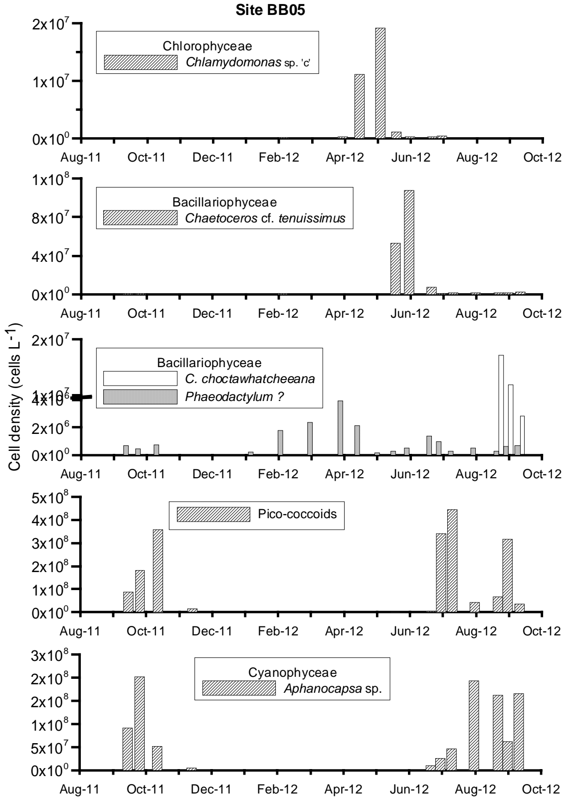
Fig. 9. Abundance and seasonal changes of some dominant species at site BB05 (BB05a) from August 2011 to September 2012. Note: Y-axis in panel 3 break from 4 \times 10^6 to 1 \times 10^7 .
