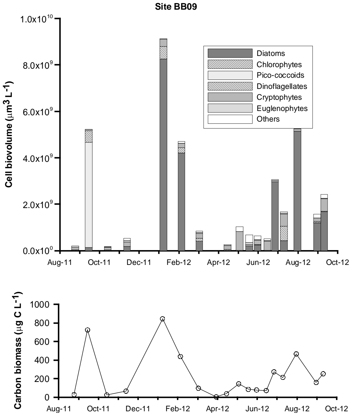
Fig. 19. Biovolume calculation and carbon biomass estimation of phytoplankton at site BB09 from August 2011 to September 2012.
