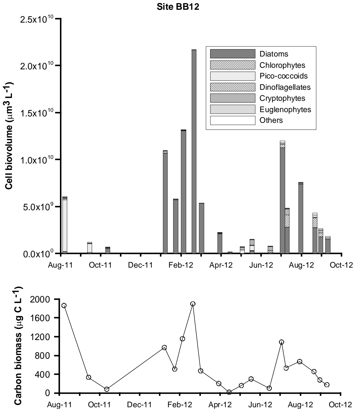
Fig. 20. Biovolume calculation and carbon biomass estimation of phytoplankton at site BB12 from August 2011 to September 2012.
