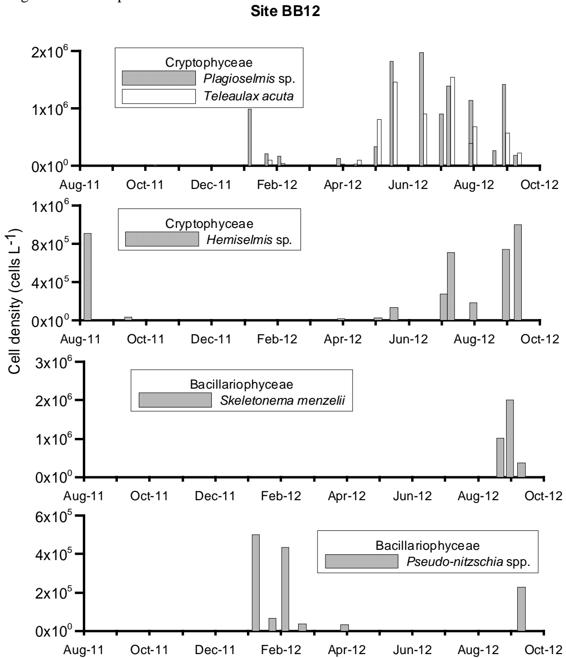
Fig. 12 (Cont.). Abundance and seasonal changes of some dominant species at site BB12 from August 2011 to September 2012.
