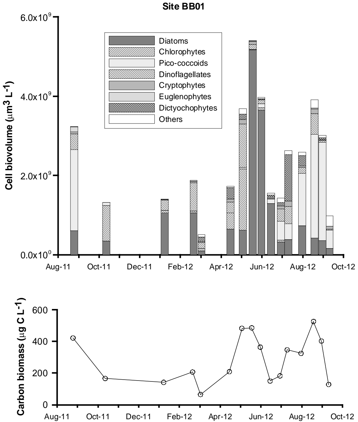
Fig. 14. Biovolume calculation and carbon biomass estimation of phytoplankton at site BB01 from August 2011 to September 2012.
