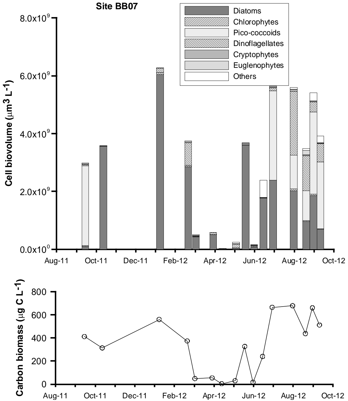
Fig. 18. Biovolume calculation and carbon biomass estimation of phytoplankton at site BB07 from August 2011 to September 2012.
