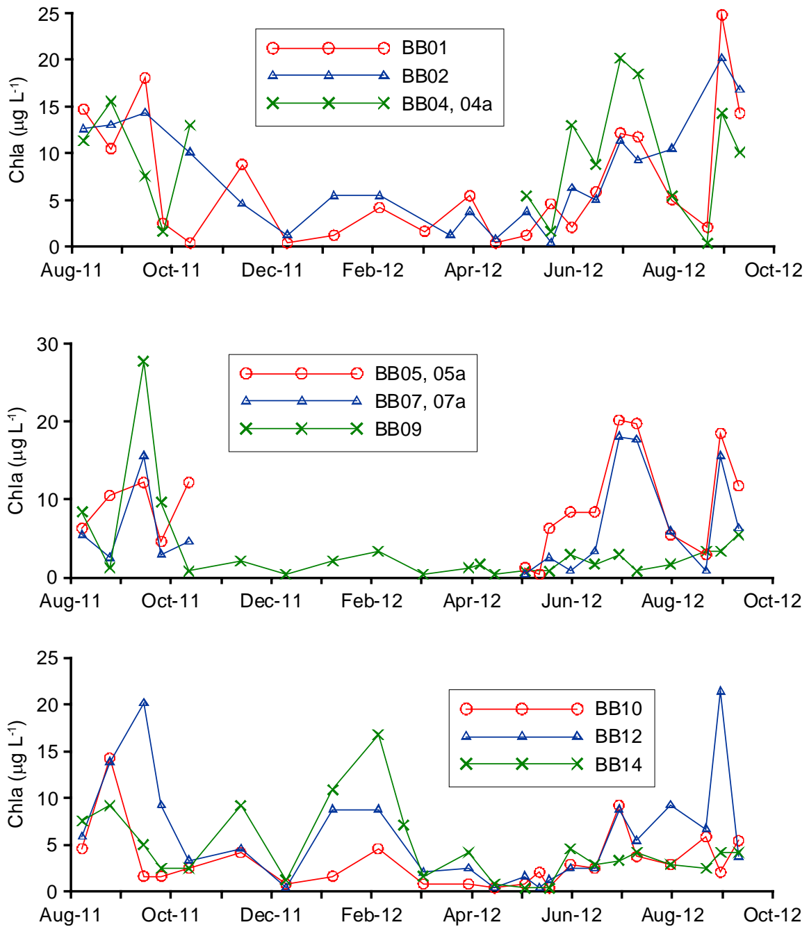
Fig. 5. Change of chlorophyll a at phytoplankton collection sites in BB-LEH from August 2011 to September 2012. Data from NJDEP water quality monitoring, http://www.nj.gov/dep/barnegatbay/bbmapviewer.htm .
