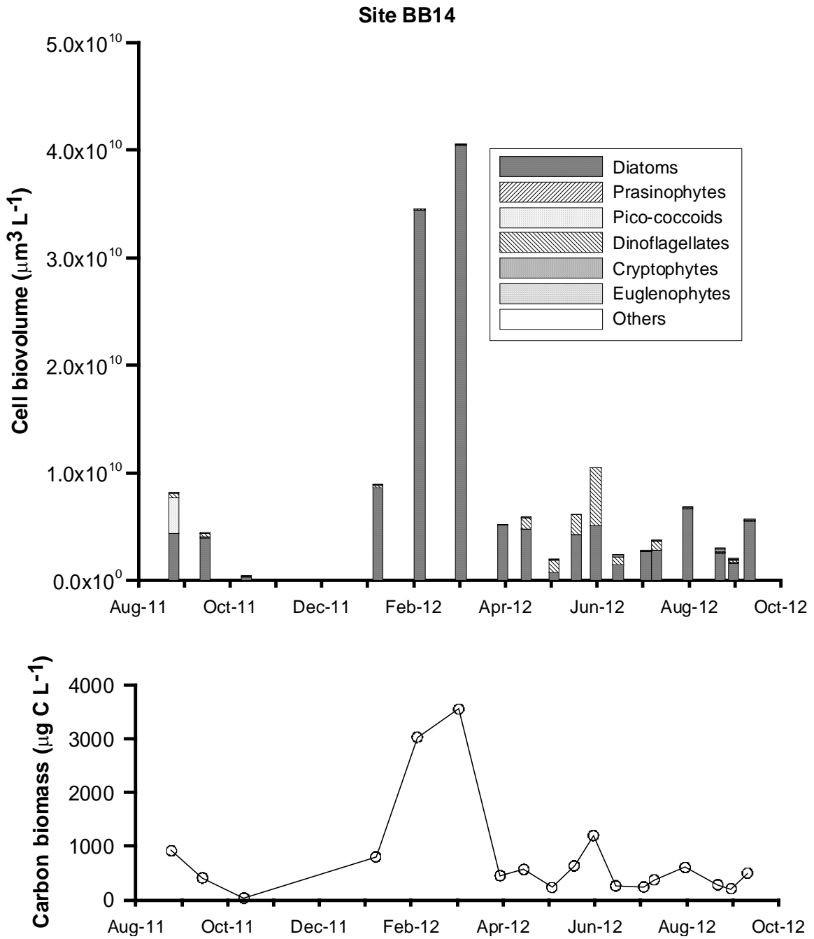
Fig. 21. Biovolume calculation and carbon biomass estimation of phytoplankton at site BB14 from August 2011 to September 2012.
