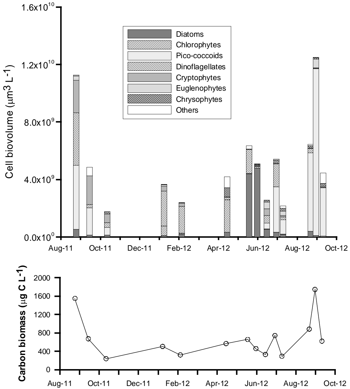
Fig. 15. Biovolume calculation and carbon biomass estimation of phytoplankton at site BB02 from August 2011 to September 2012.
