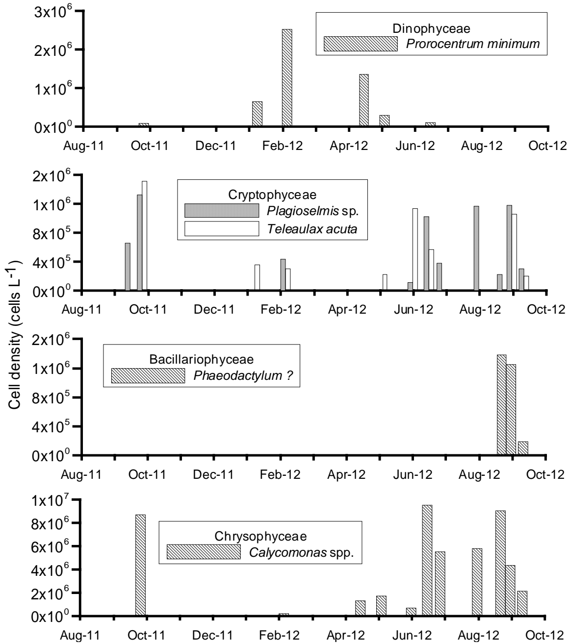
Fig. 8 (Cont.). Abundance and seasonal changes of some dominant species at site BB04 (BB04a) from August 2011 to September 2012.
