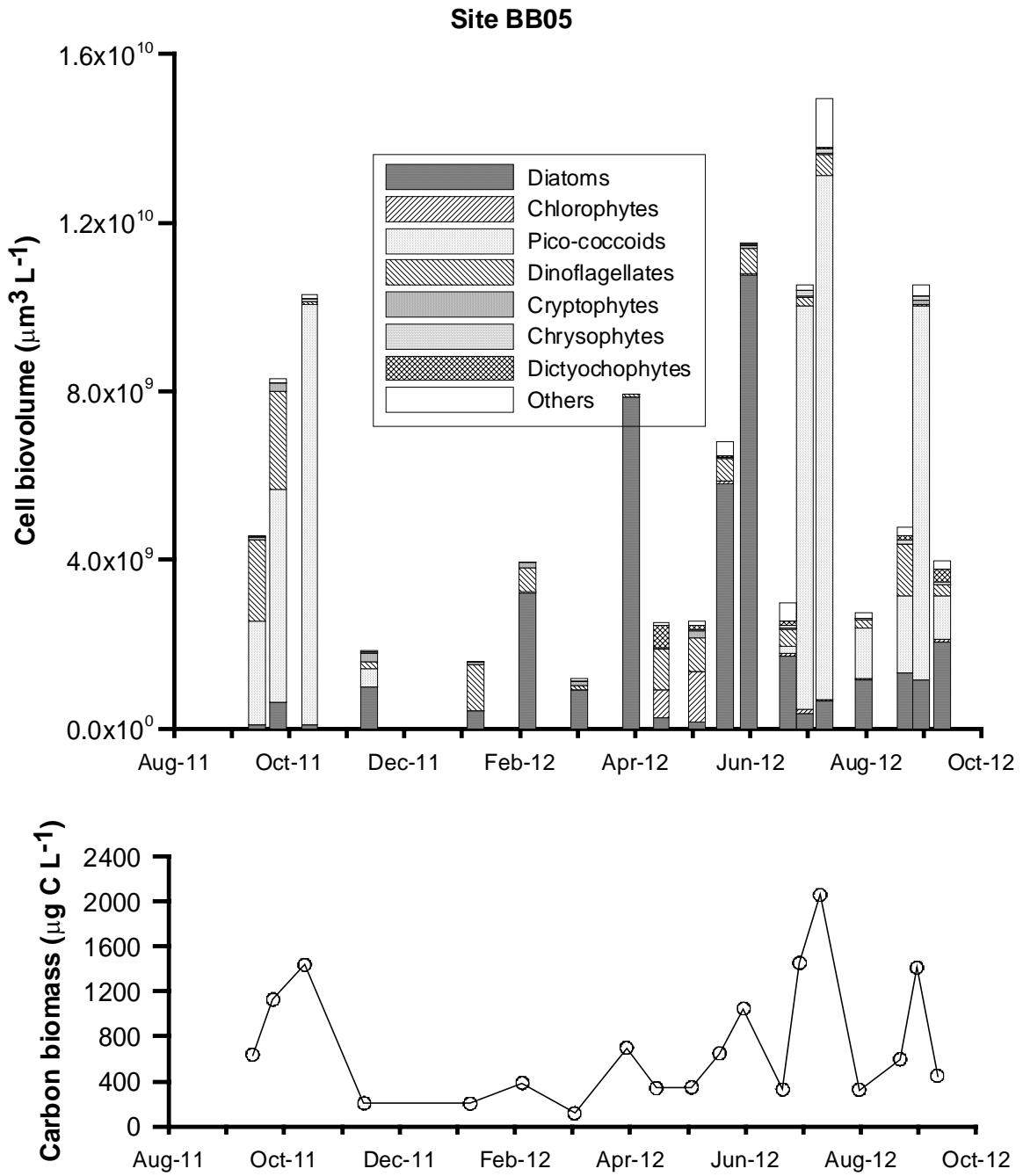
Fig. 17. Biovolume calculation and carbon biomass estimation of phytoplankton at site BB05 from August 2011 to September 2012.
