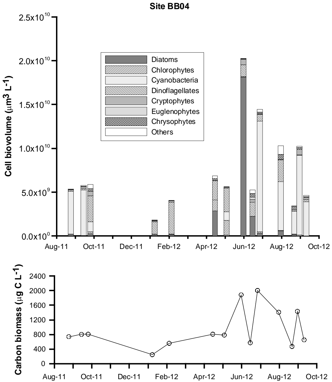
Fig. 16. Biovolume calculation and carbon biomass estimation of phytoplankton at site BB04 from August 2011 to September 2012.
