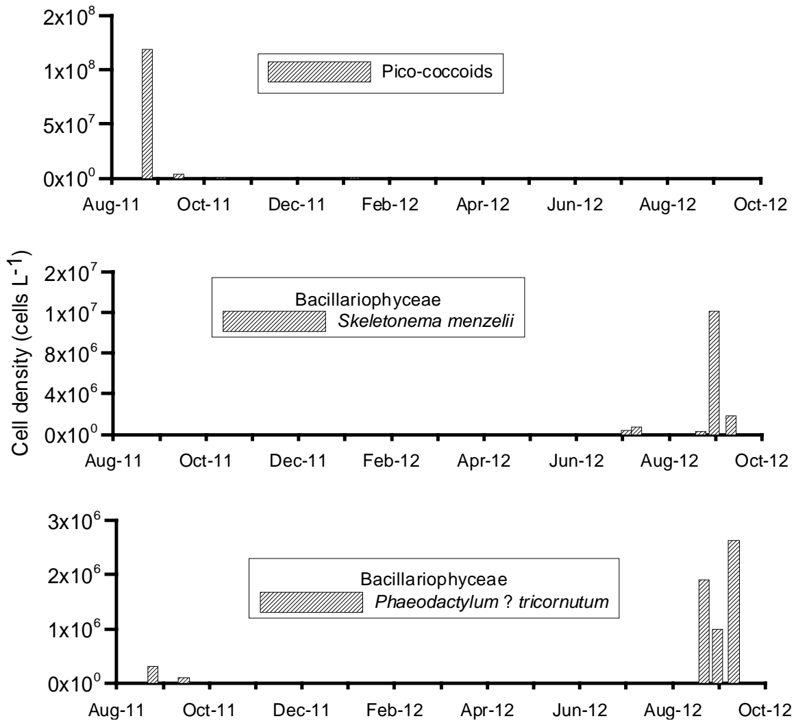
Fig. 13 (Cont.). Abundance and seasonal changes of some dominant species at site BB14 from August 2011 to September 2012.
