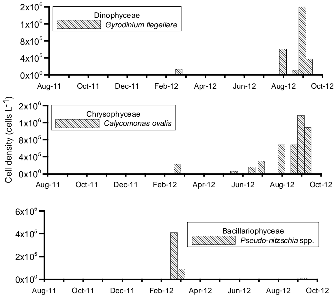
Fig. 10 (Cont.). Abundance and seasonal changes of some dominant species at site BB07 (BB07a) from August 2011 to September 2012.
