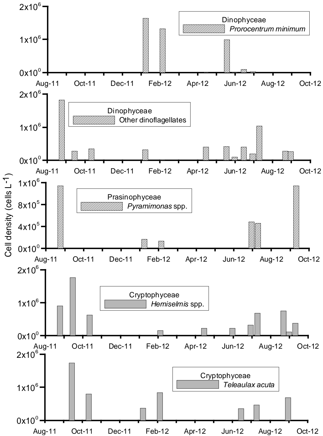
Fig. 7 (Cont.). Abundance and seasonal changes of some dominant species at site BB02 from August 2011 to September 2012.
