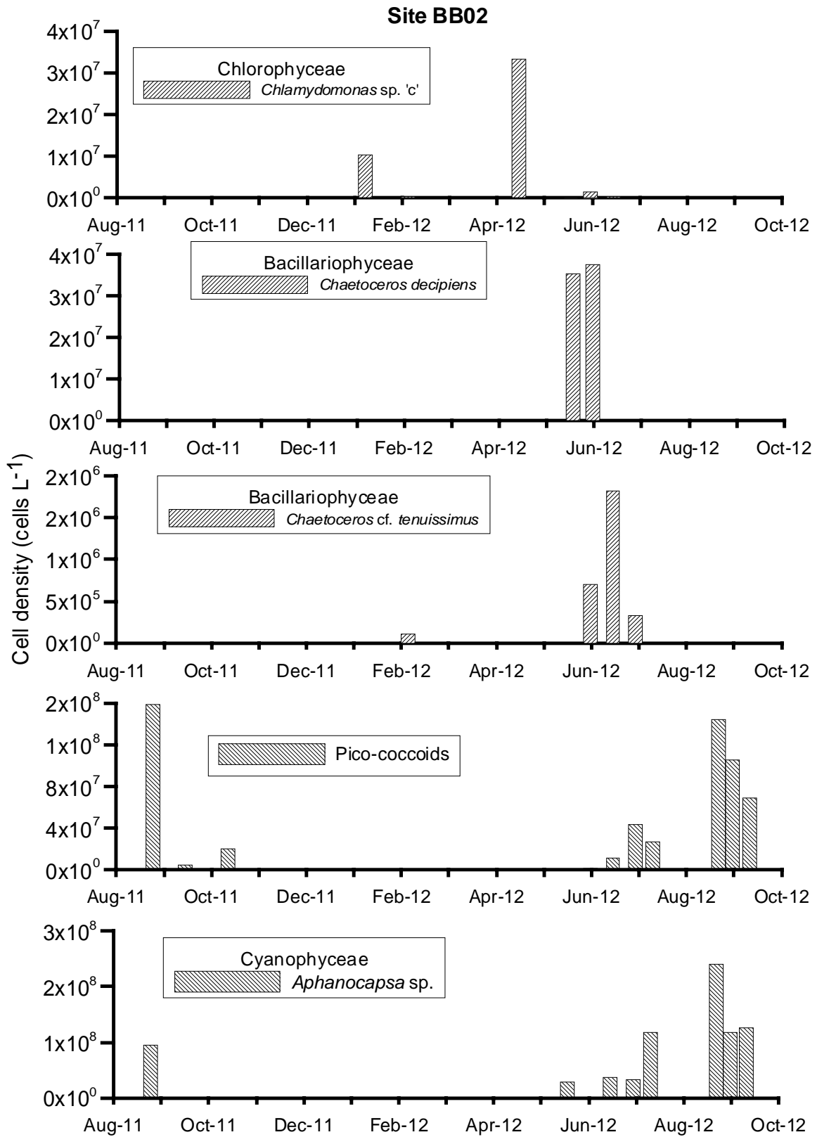
Fig. 7. Abundance and seasonal changes of some dominant species at site BB02 from August 2011 to September 2012.
