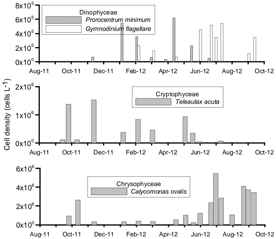
Fig.9 (Cont.). Abundance and seasonal changes of some dominant species at site BB05 (BB05a) from August 2011 to September 2012.
