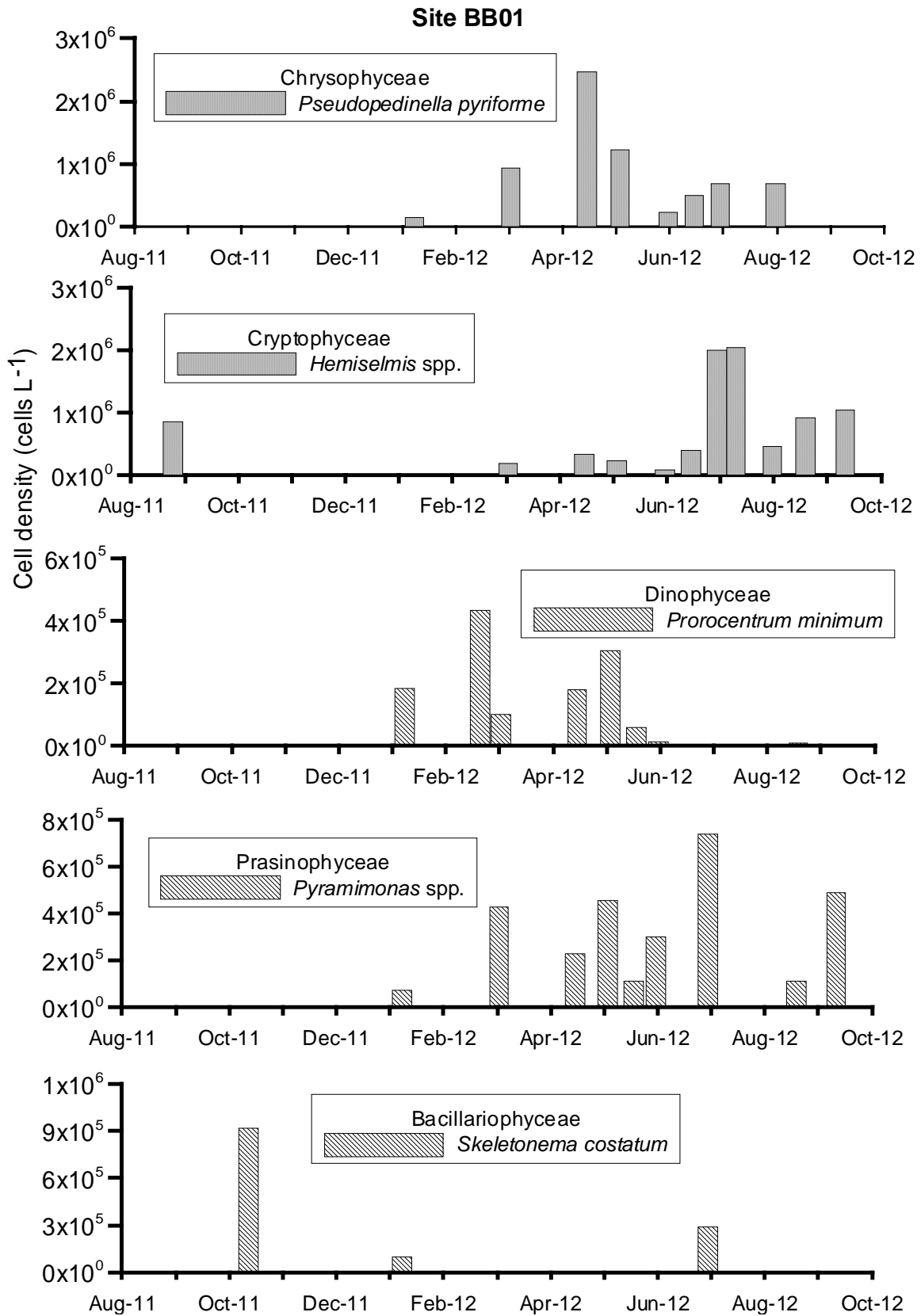
Fig. 6 (Cont.). Abundance and seasonal changes of some dominant species at site BB01 from August 2011 to September 2012.
