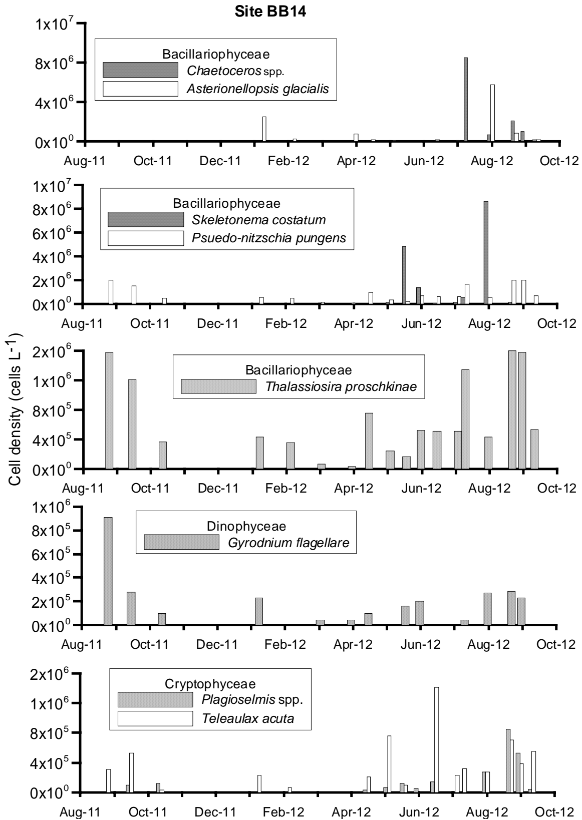
Fig. 13. Abundance and seasonal changes of some dominant species at site BB14 from August 2011 to September 2012.
