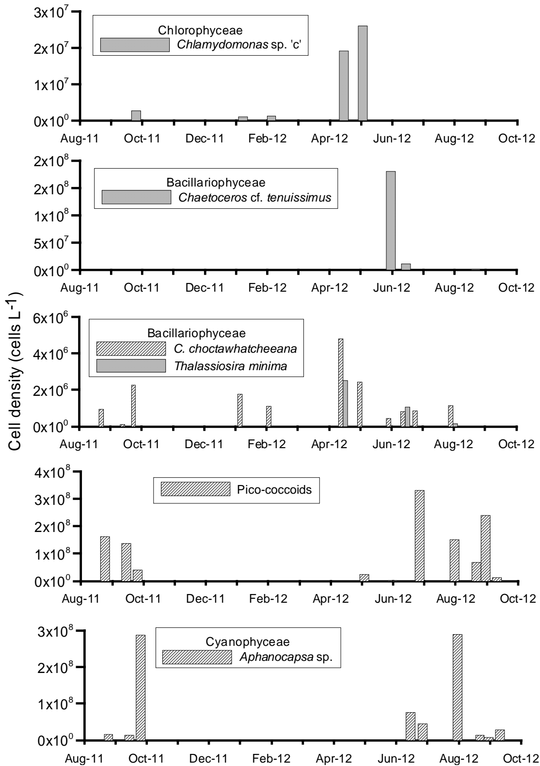
Fig. 8. Abundance and seasonal changes of some dominant species at site BB04 (BB04a) from August 2011 to September 2012.
