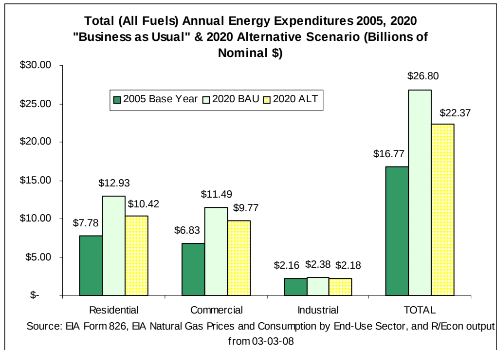
Figure 19: Total Annual Energy Expenditures for all Sectors.
