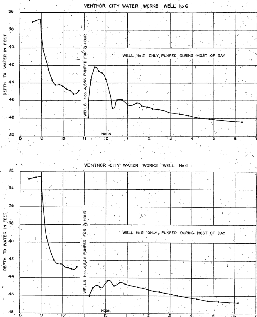
Fig. 11.—Graph showing fluctuation of water level in wells Nos. 4 and 6 at Ventnor Water Works during pumping of well No. 5, January 15, 1925.
