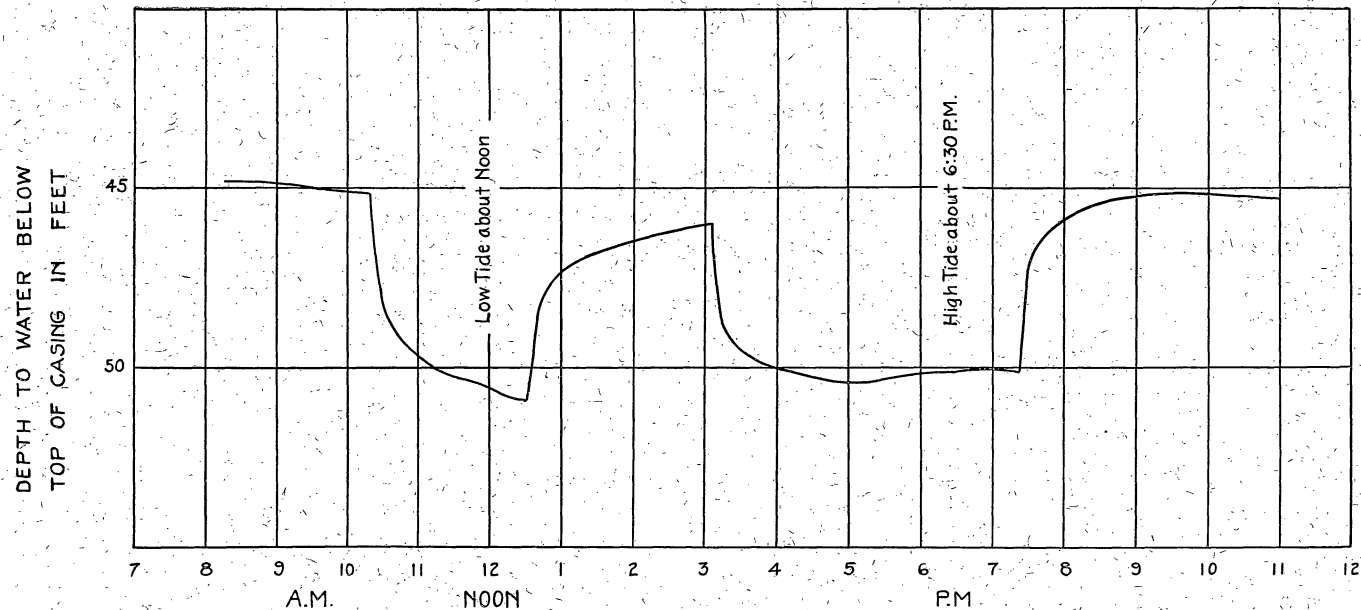
FIG. 7.—Graph showing fluctuation of water level in new well at Margate City Water Works, August 28, 1924.
