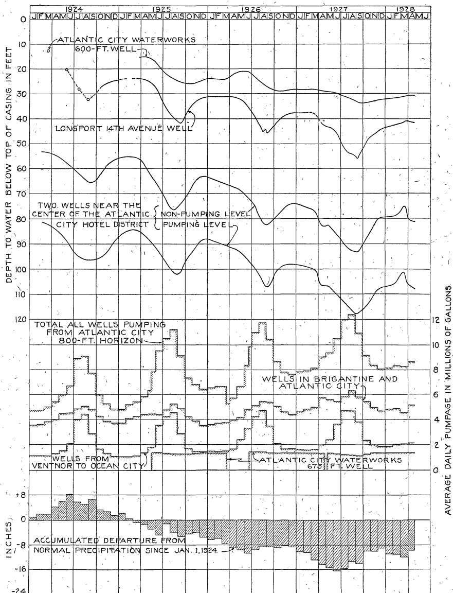
FIG. 14.—Diagram showing fluctuation of water level in, and pumpage from, wells tapping Atlantic City 800-foot sand in the area between Brigantine, Pleasantville and Ocean City, and accumulated departure from normal precipitation in southern interior section of New Jersey since January 1, 1924.
