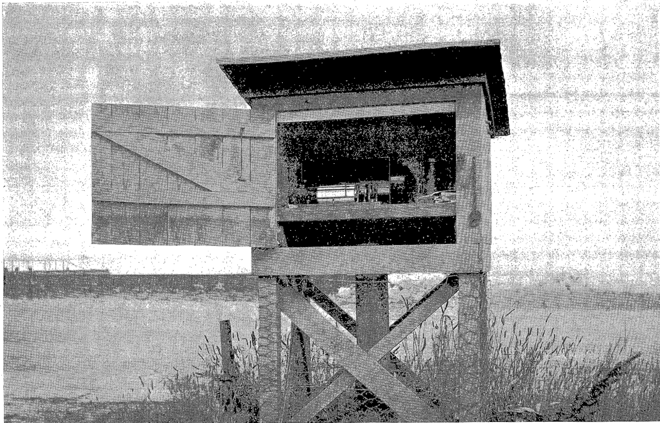
Installation of water-level recorder on 14th Street 800-foot well of Borough of Longport.
