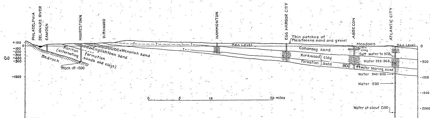
FIG. 4.—Generalized cross section from Philadelphia to Atlantic City showing principal water-bearing horizons.
