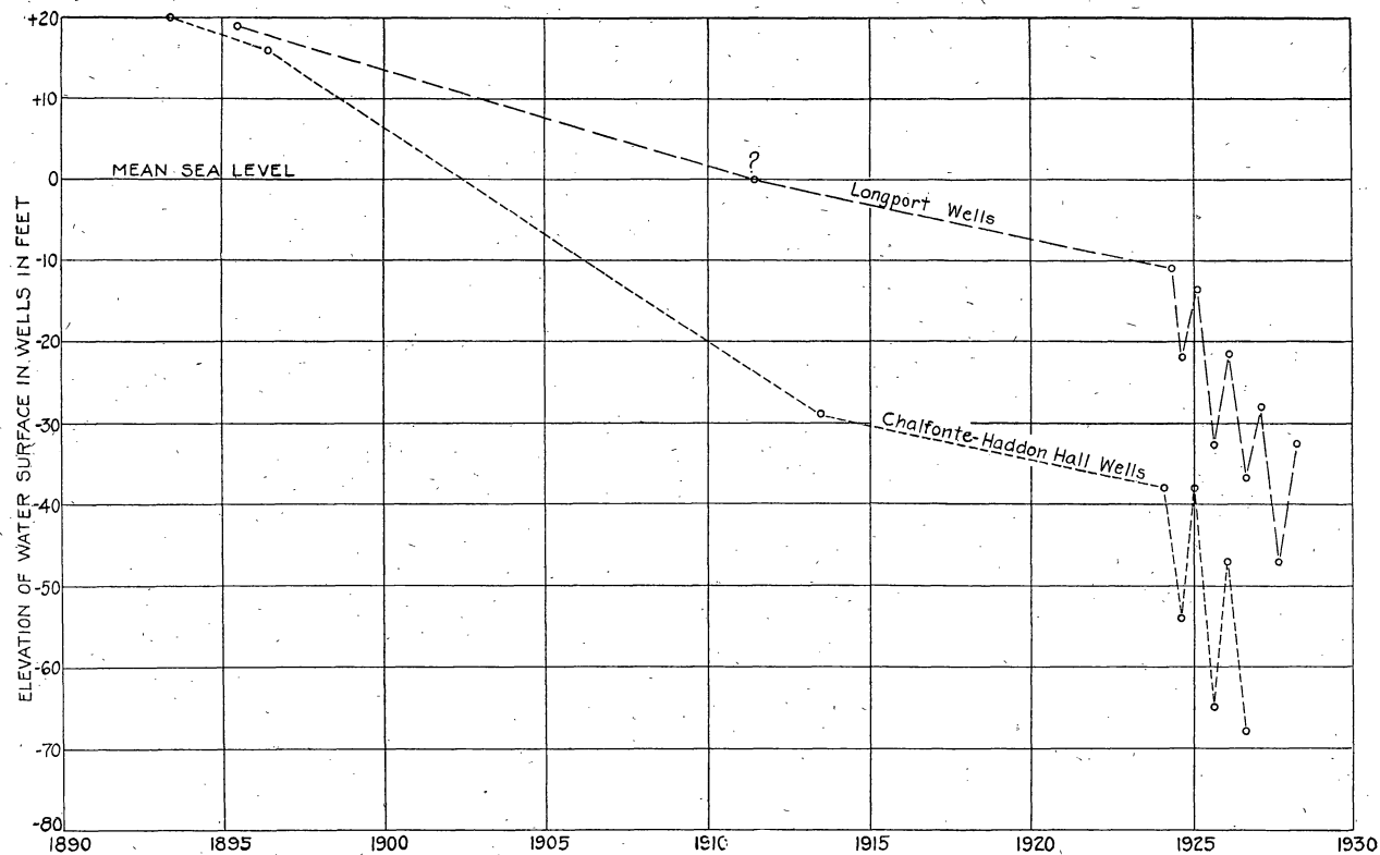
FIG. 16.—Graph showing rate of lowering of static water level in wells at Haddon Hall and Chalfonte Hotel and at Longport, 1893 to 1928.
