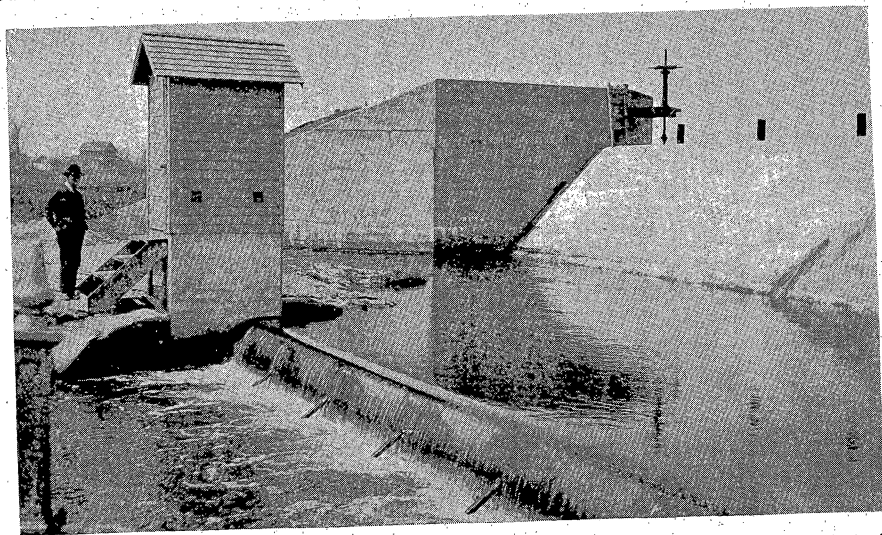
Weir and gaging station below Absecon dam, maintained by New Jersey Department of Conservation and Development and U. S. Geological Survey to measure flow of Absecon Creek.
