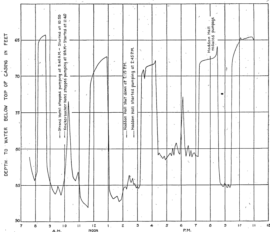
FIG. 8.—Graph showing fluctuation of water level in well at Chalfonte Hotel, August 28, 1924.
