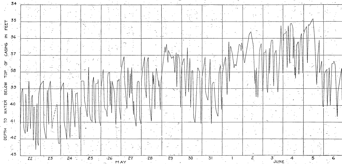
Fig. 6.—Graph showing fluctuation of water level in new well at Atlantic City Electric Company, May 21 to June 7, 1924.
