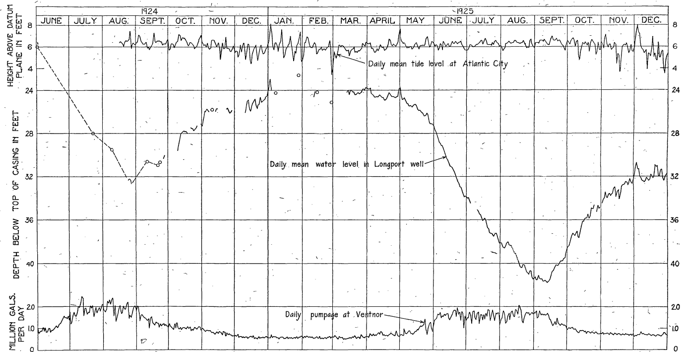
FIG. 13.—Graph showing daily mean water level in 14th Avenue well, Longport, mean tide level at Steel Pier, Atlantic City, and daily pumpage at Ventnor.
