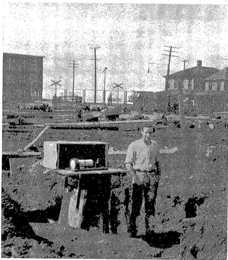
Temporary installation of water-level recorder on new well of Atlantic City Electric Co., May, 1924.
