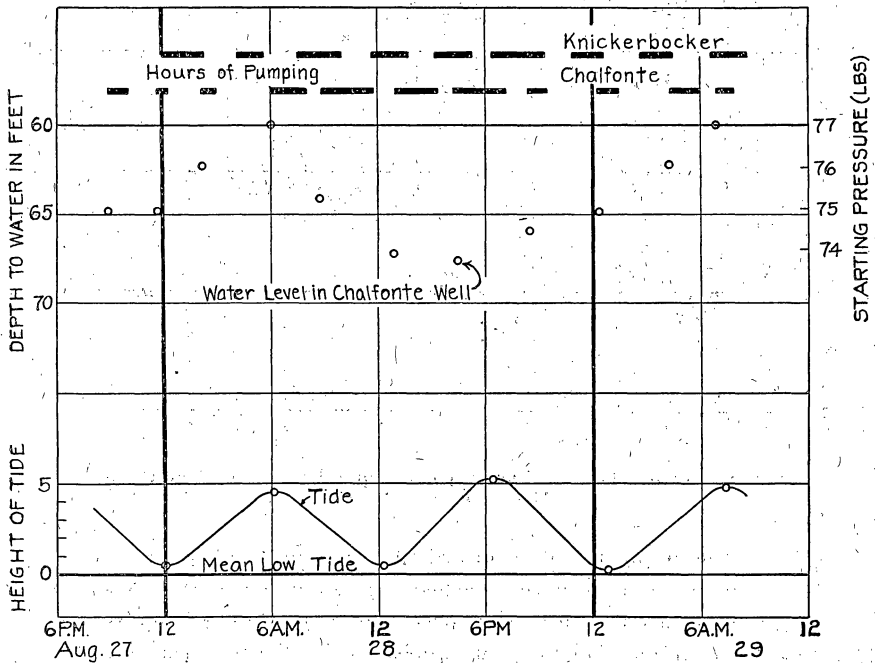
FIG. 9.—Graph showing depth to water in Chalfonte Hotel well at times of starting pump; hours of pumping from wells at Chalfonte and Knickerbocker Hotels, and fluctuation of tide, August 27 to 29, 1924.
