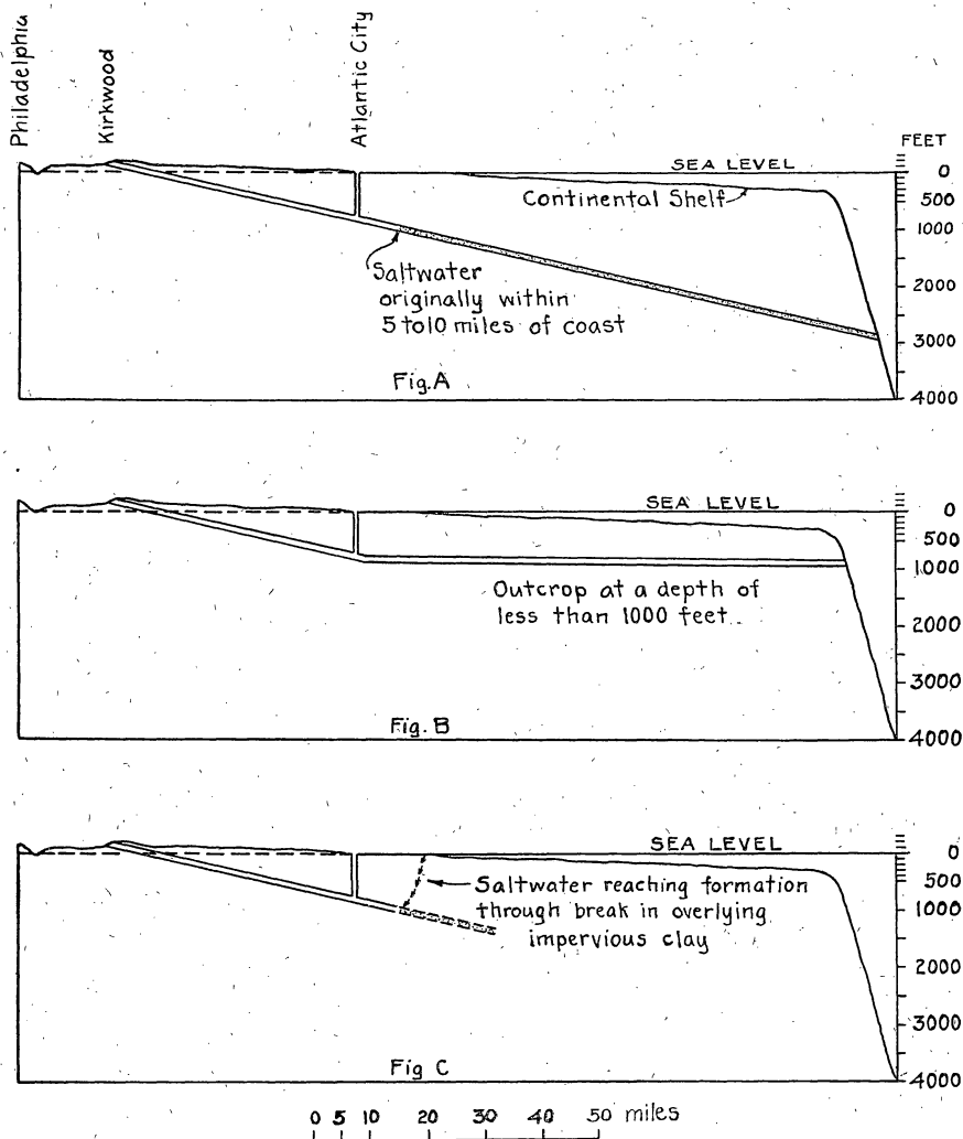
FIG. 21.—Diagrams showing possible alternative conditions that would account for a head of 25 feet on the 800-foot sand at Atlantic City.
