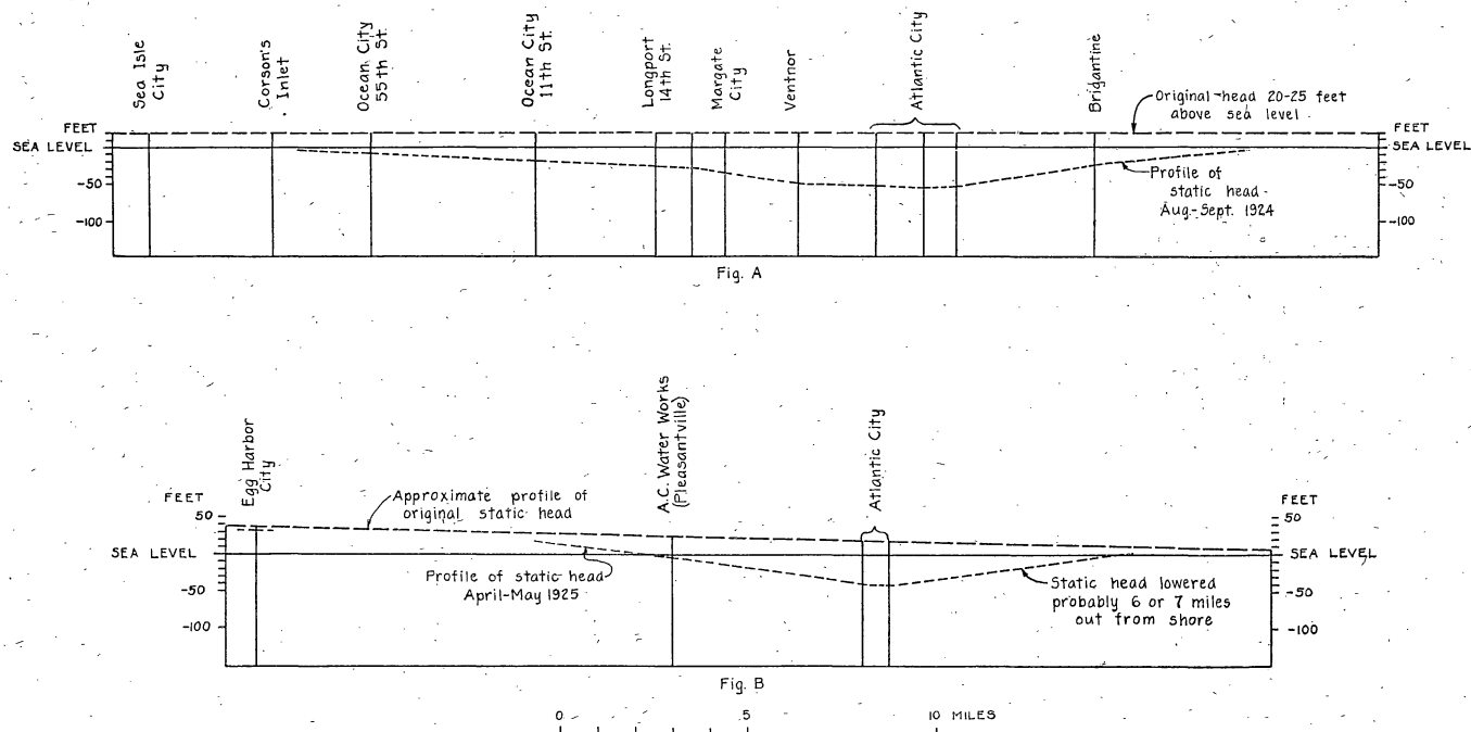
FIG. 15.—Profiles of piezometric surface of 800-foot horizon in the Atlantic City region. A.—Profile parallel to coast. B.—Profile at right angles to coast.
