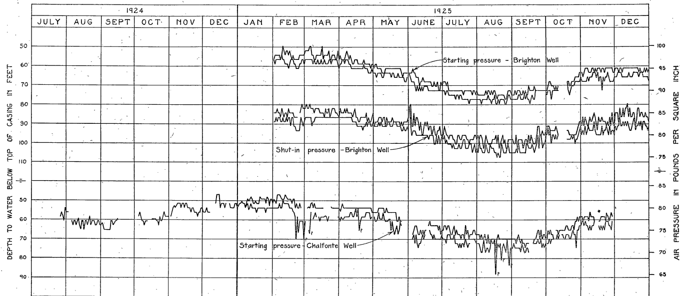
FIG. 12.—Graph showing highest and lowest starting and shut-in pressures on Brighton Hotel well and highest and lowest starting pressures on Chalfonte Hotel well, 1924-1925.
