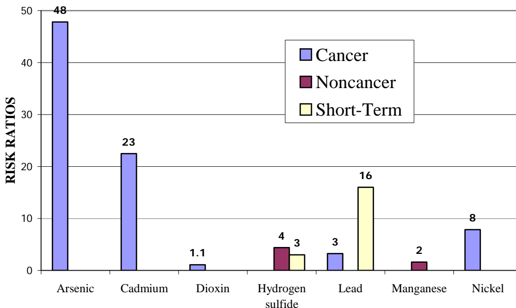
Figure 3: Risk Ratios Greater Than 1 Camden Waterfront South Air Toxics Pilot Project Final Risk Assessment
