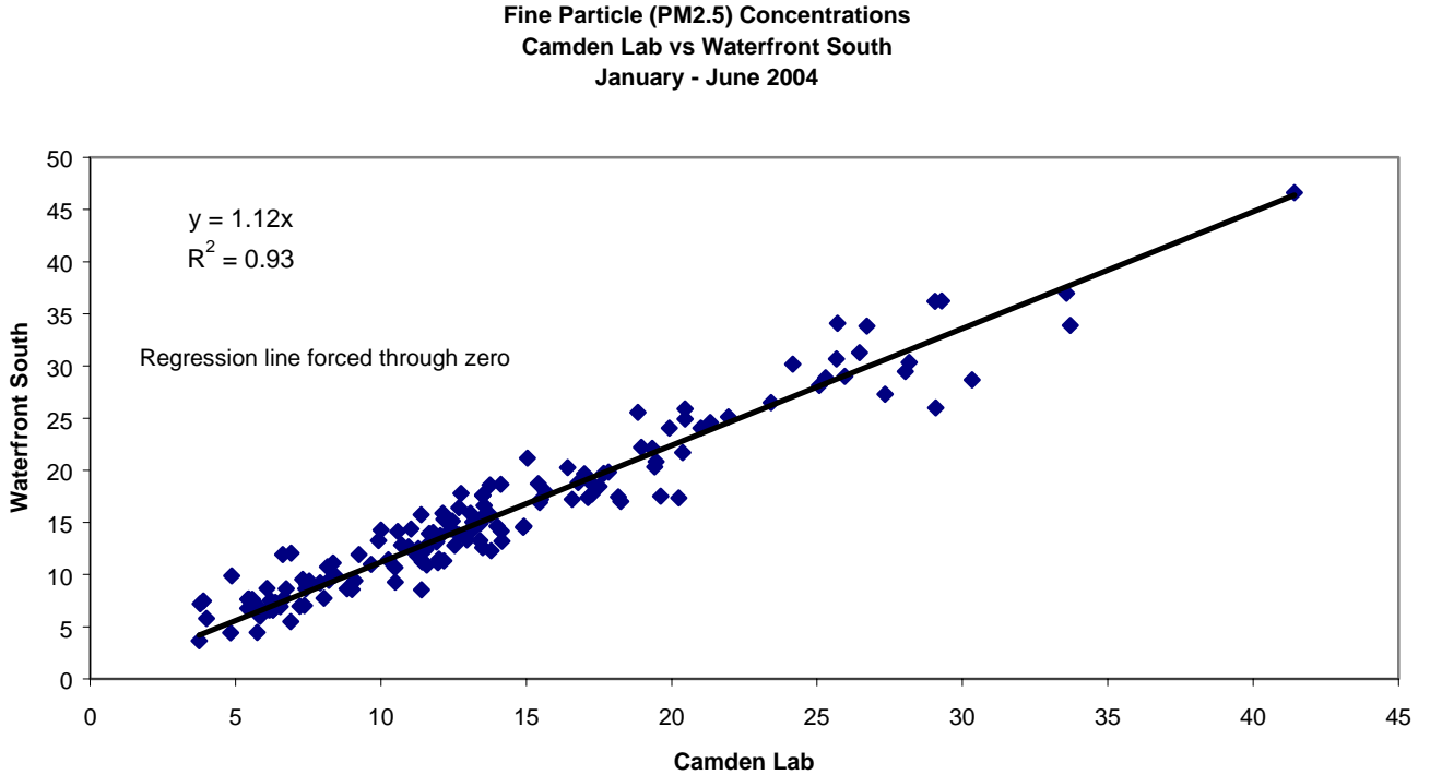
Figure 12: Comparison of PM 2.5 measured at Waterfront South and the Camden Lab with a regression line
