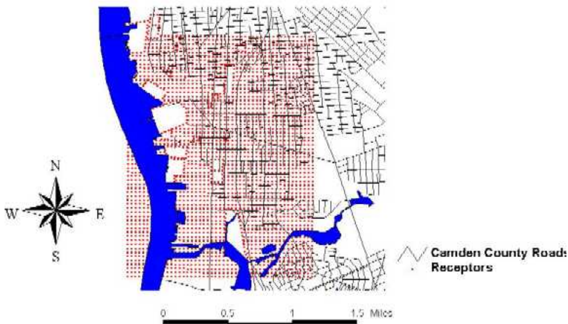
Figure 2: Distribution of Air Quality Receptors across Waterfront South Each dot on the map represents a point where air concentrations were predicted by the ISC model.
