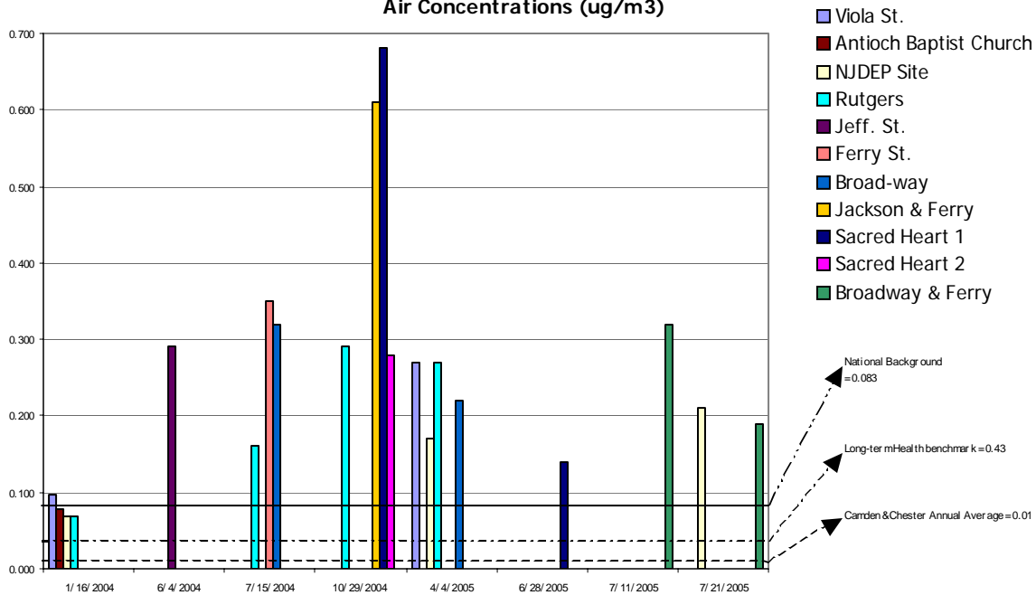
Figure 12: Camden Bucket Brigade - Chloroform Results Air Concentrations (ug/m3)
