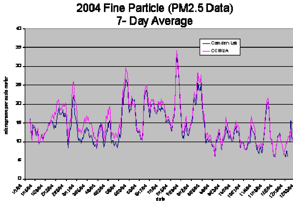
Figure 11: Particulate (PM2.5) Concentrations for 2004 in micrograms per cubic meter 7-day average
