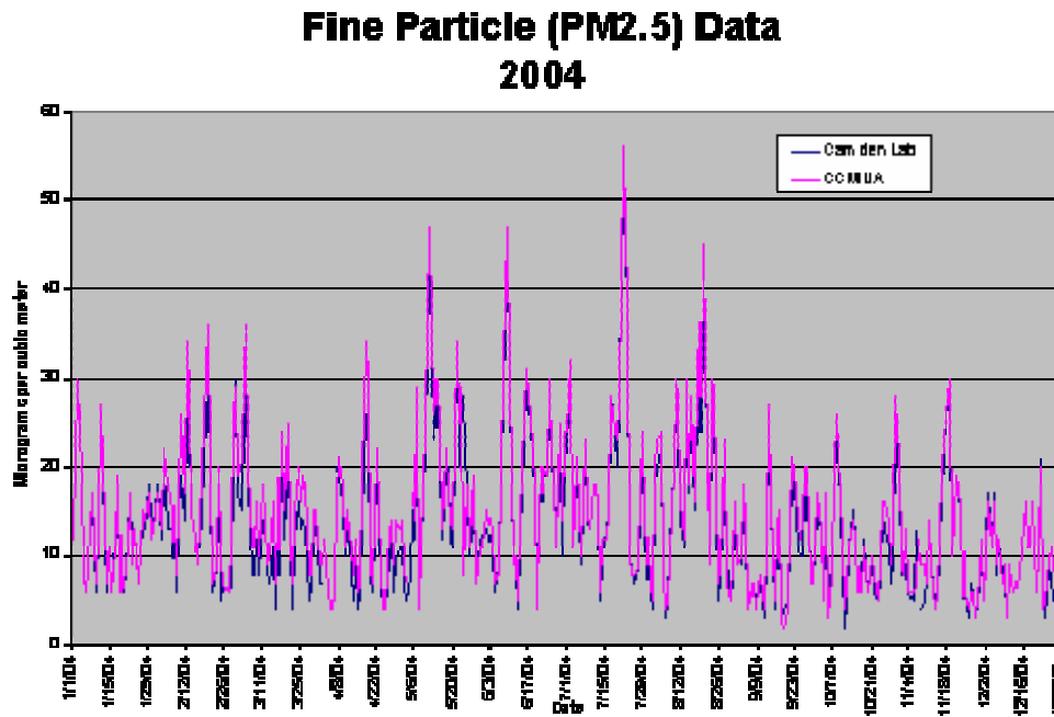
Figure 10: Particulate (PM2.5) Concentrations for 2004 in micrograms per cubic meter
