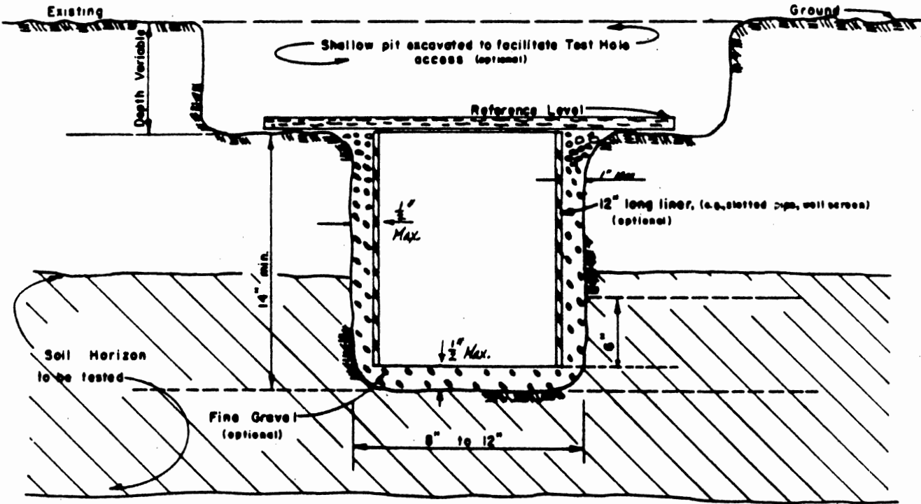
Figure 7. Percolation Test
