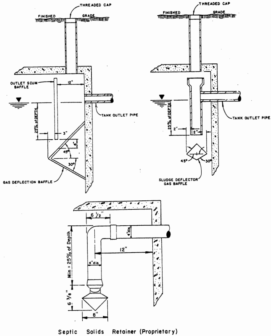
Figure 12. Gas Deflection Baffles
