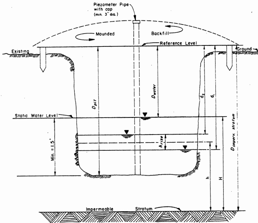
Figure 7. Percolation Test
