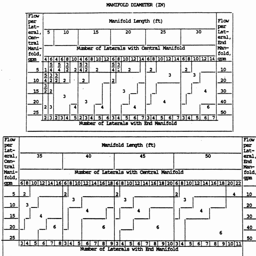
Figure 15. Required Manifold Diameters For Various Manifold Lengths, Number of Laterals and Lateral Discharge Rates
