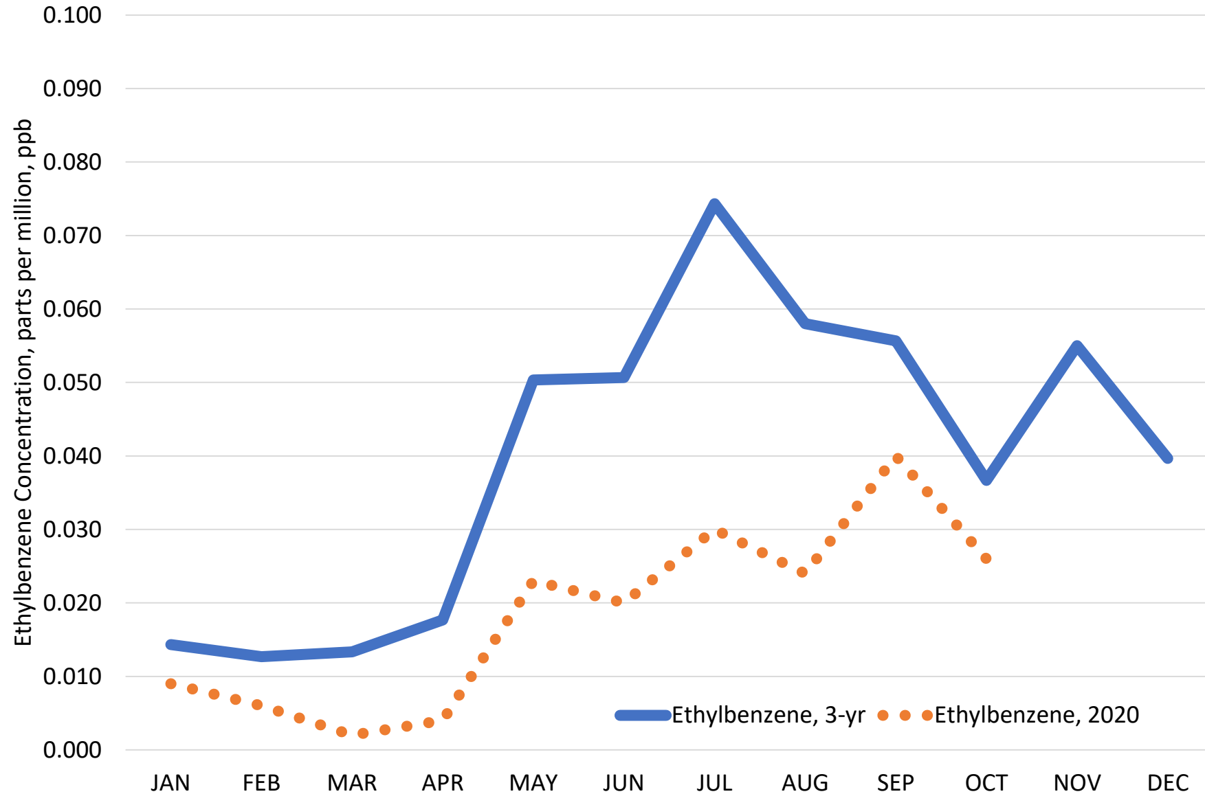
Comparison of 3-Year Average (2015, 2016, 2019) Monthly Ethylbenzene Concentrations with 2020 Monthly Ethylbenzene Concentrations at Bayonne
