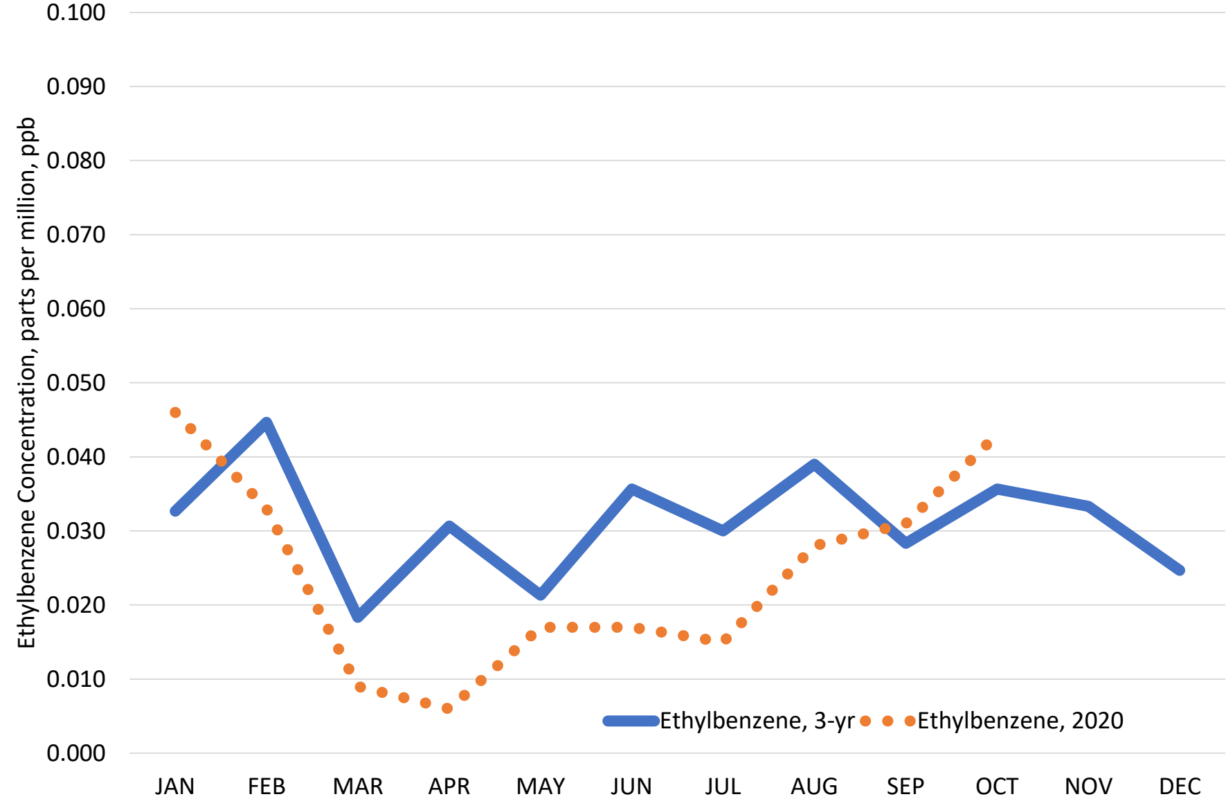
Comparison of 3-Year Average (2017, 2018, 2019) Monthly Ethylbenzene Concentrations with 2020 Monthly Ethylbenzene Concentrations at Camden
