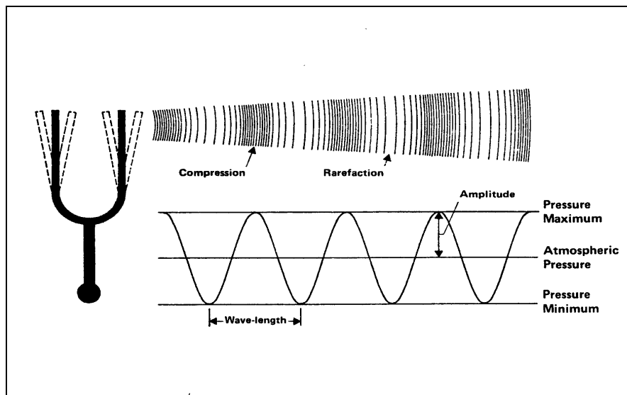
Figure A-1 Acoustics of a Pure Tone
