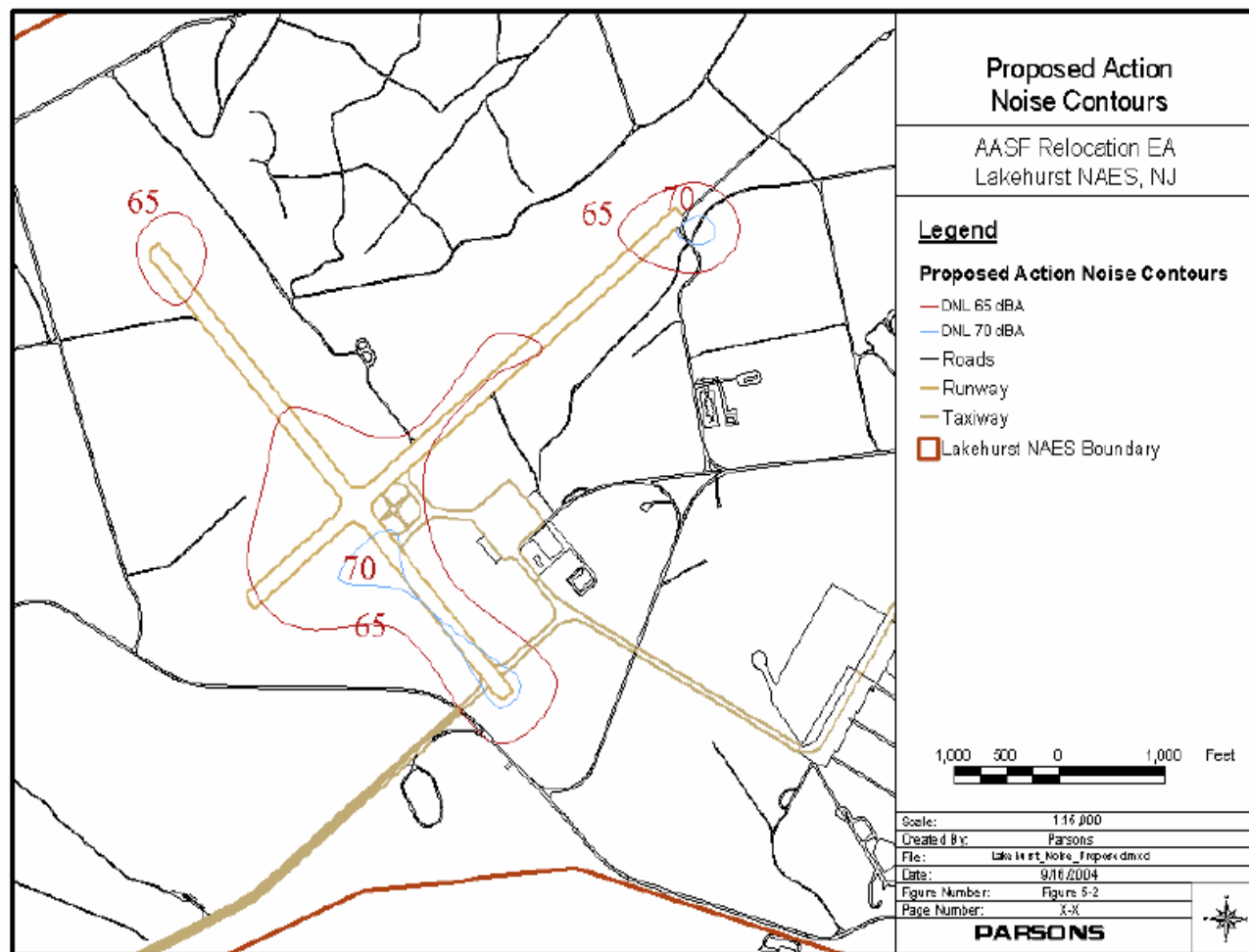
Figure 5-7 NAES Lakehurst Noise Contours with Proposed AASF Operations
